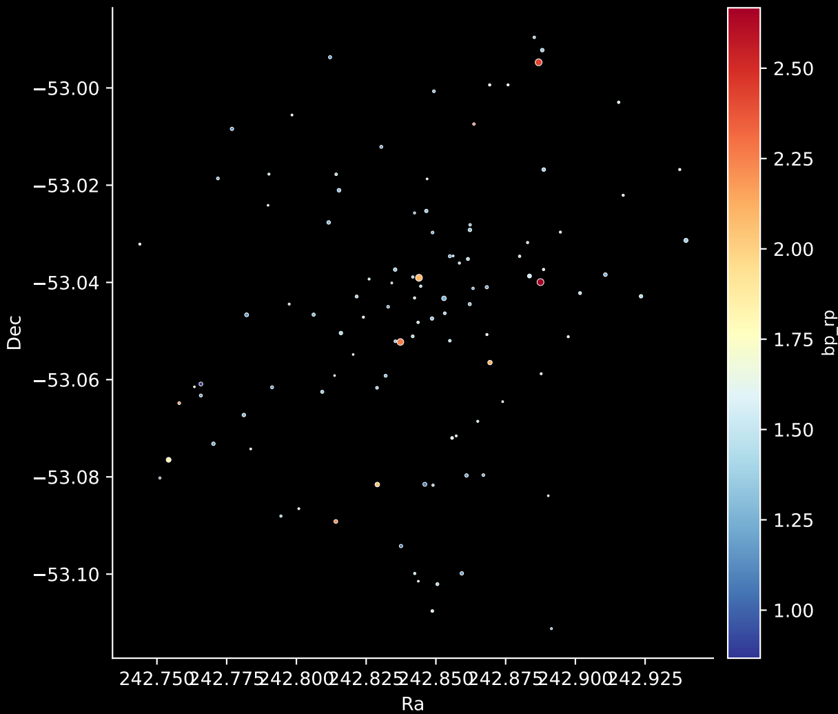
Gaia Cluster: [BH_72] Stars: 106
