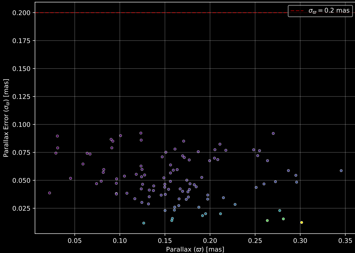
Gaia Cluster: [BH_72] Parallax Quality (n= 106)
