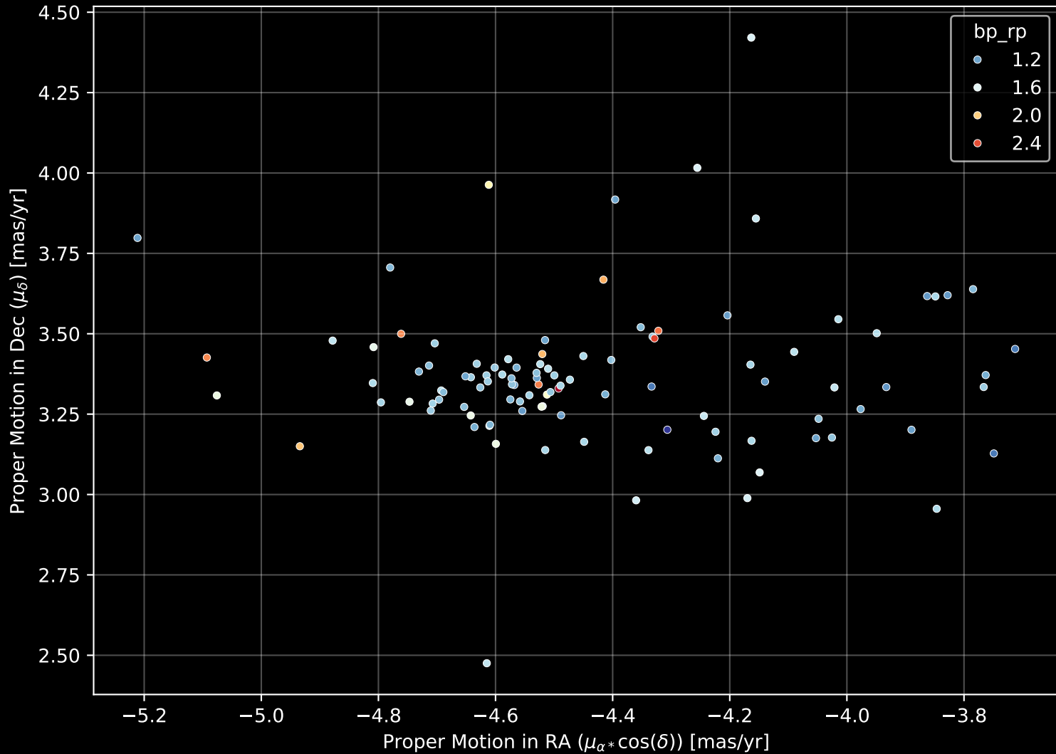
Gaia Cluster: [BH_72] Proper Motion Diagram (n= 106)
