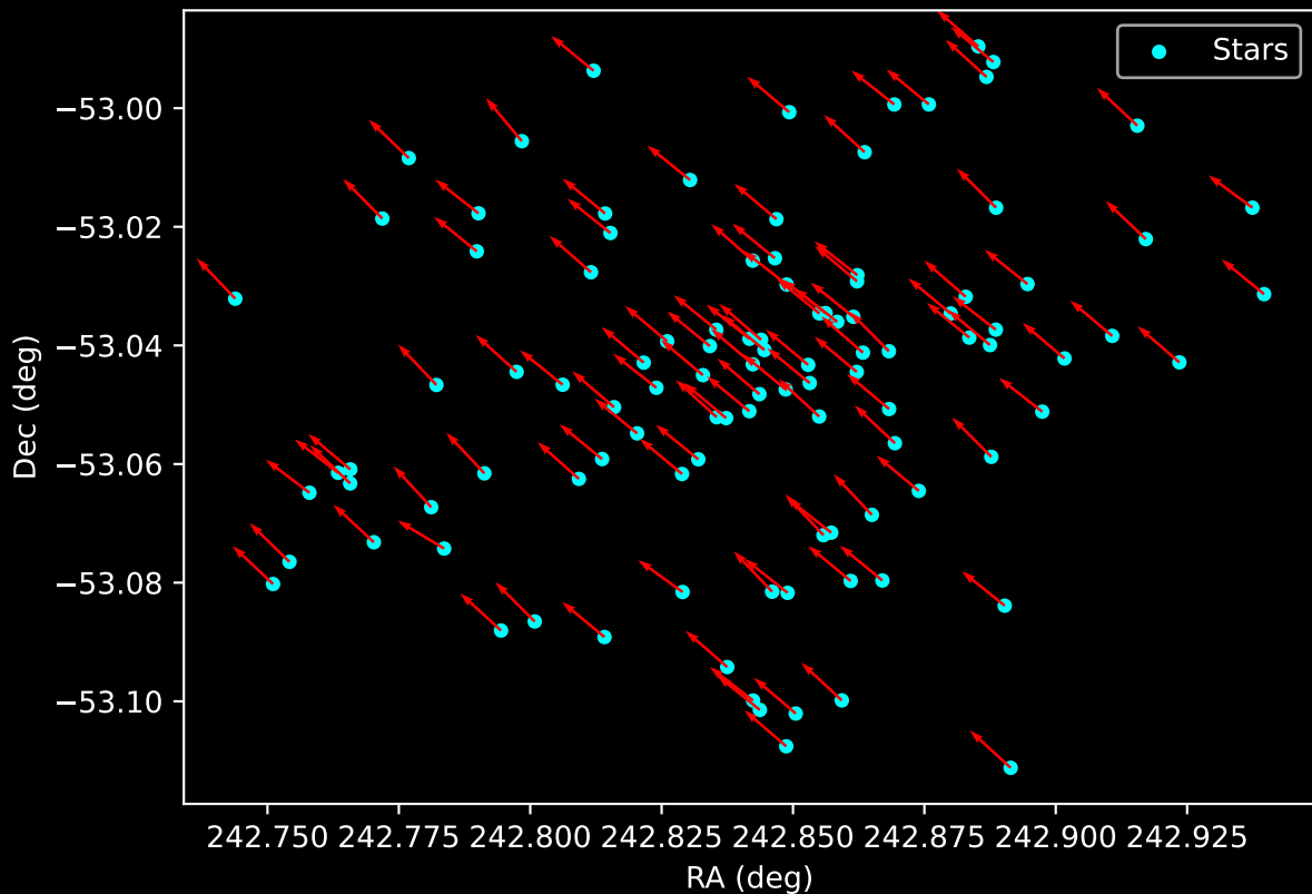
Gaia Cluster: [BH_72] Proper Motion Vectors for Gaia Star Field (n= 106)
