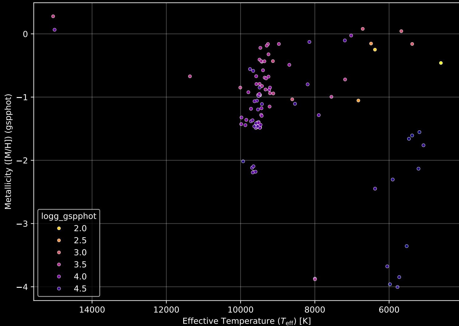
Gaia Cluster: [BH_72] Stellar Population Parameters (n= 106)
