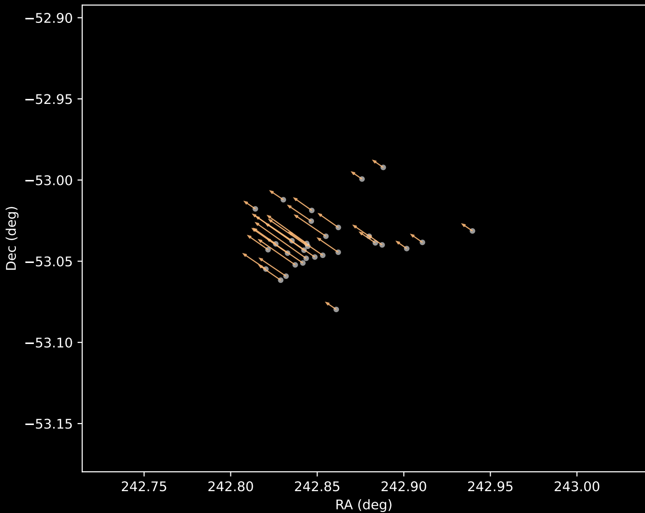
Gaia DR3 Cluster 3 Proper Motion Vectors (n=31)
