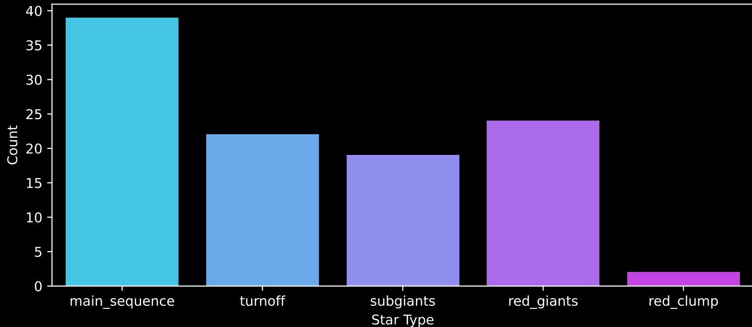
Gaia Cluster: [BH_72] Count plot of Star Type
