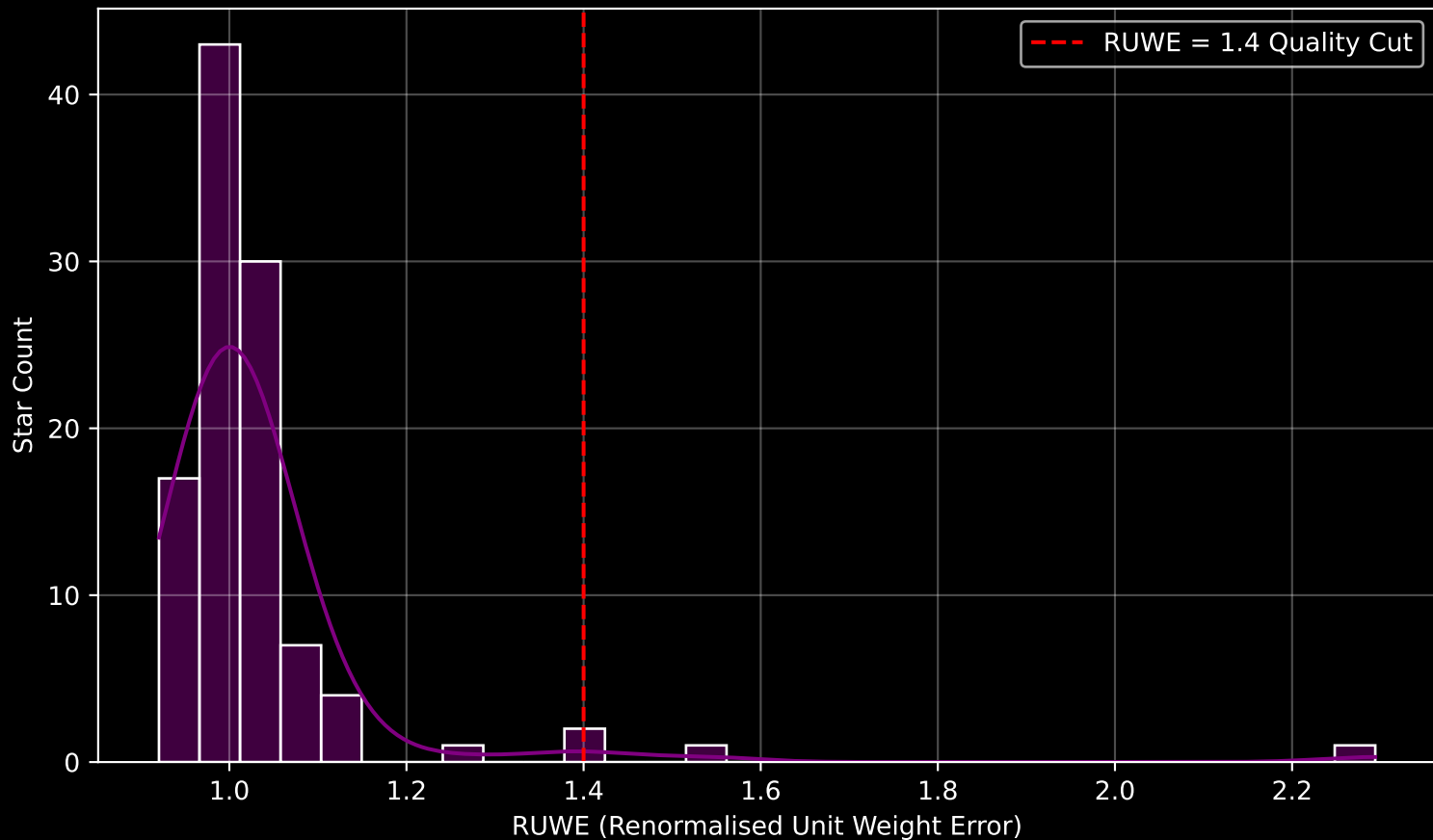
Gaia Cluster: [BH_72] RUWE Distribution (n= 106)
