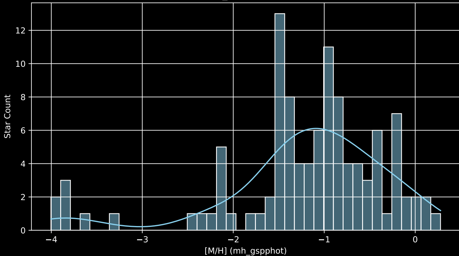
Gaia Cluster: [BH_72 [M/H] (mh_gspphot) (n= 106)
