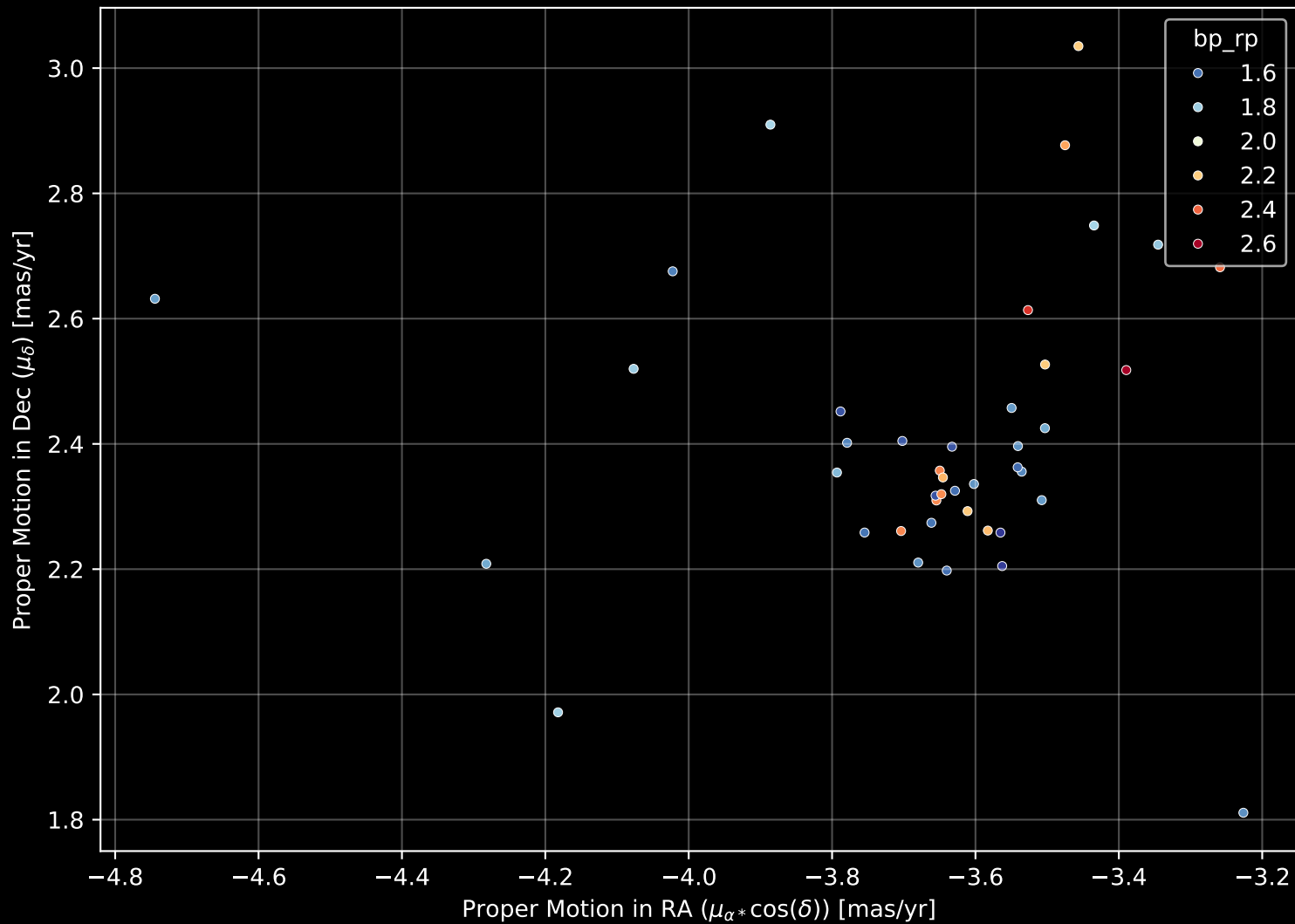
Gaia Cluster: [BH_73] Proper Motion Diagram (n= 42)
