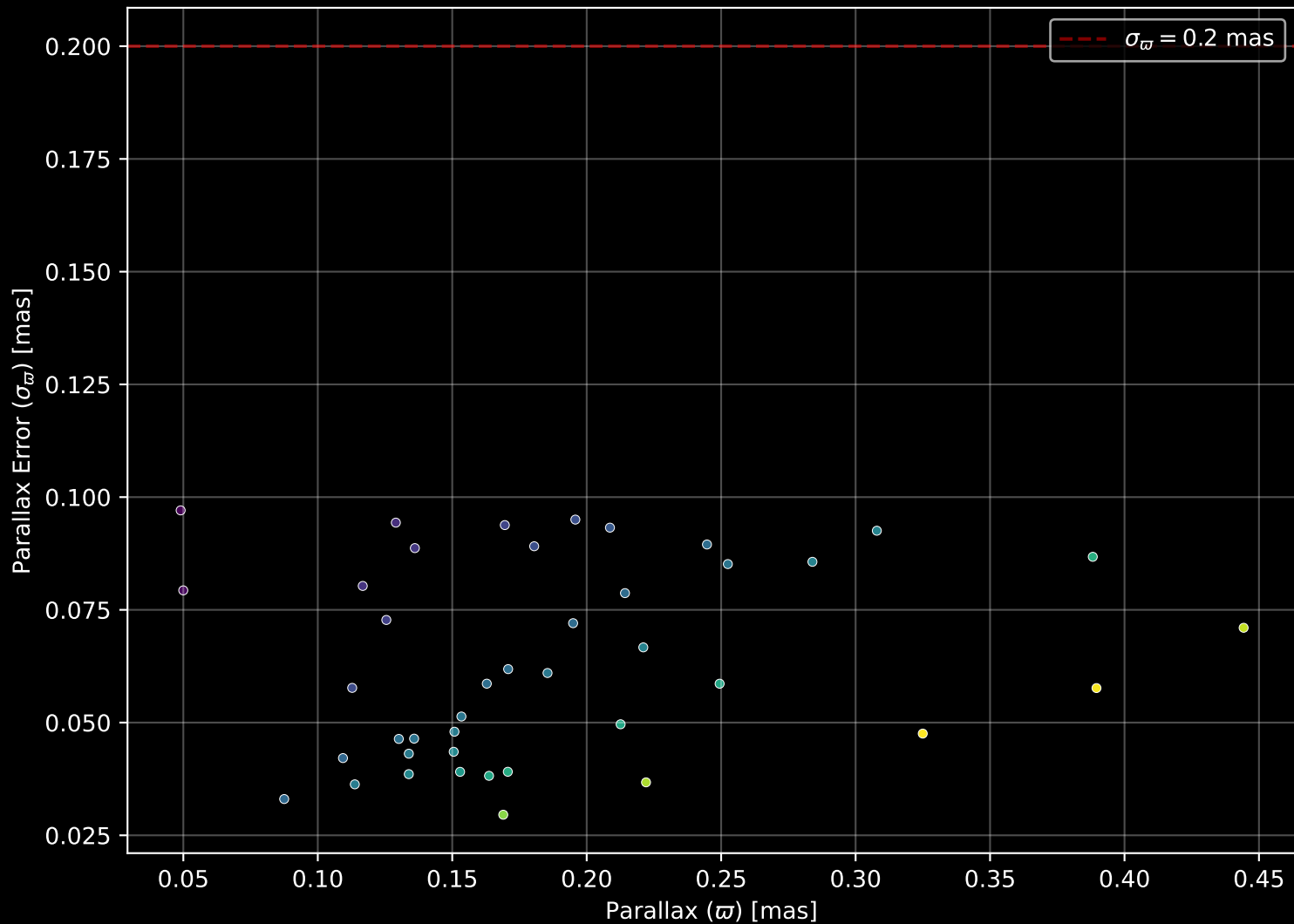
Gaia Cluster: [BH_73] Parallax Quality (n= 42)
