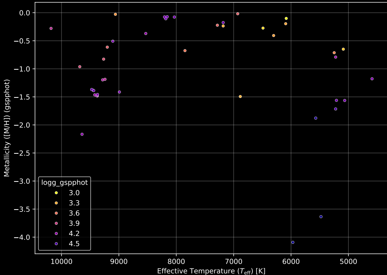
Gaia Cluster: [BH_73] Stellar Population Parameters (n= 42)
