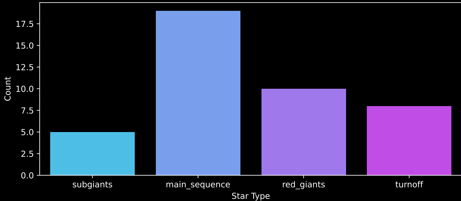
Gaia Cluster: [BH_73] Count plot of Star Type
