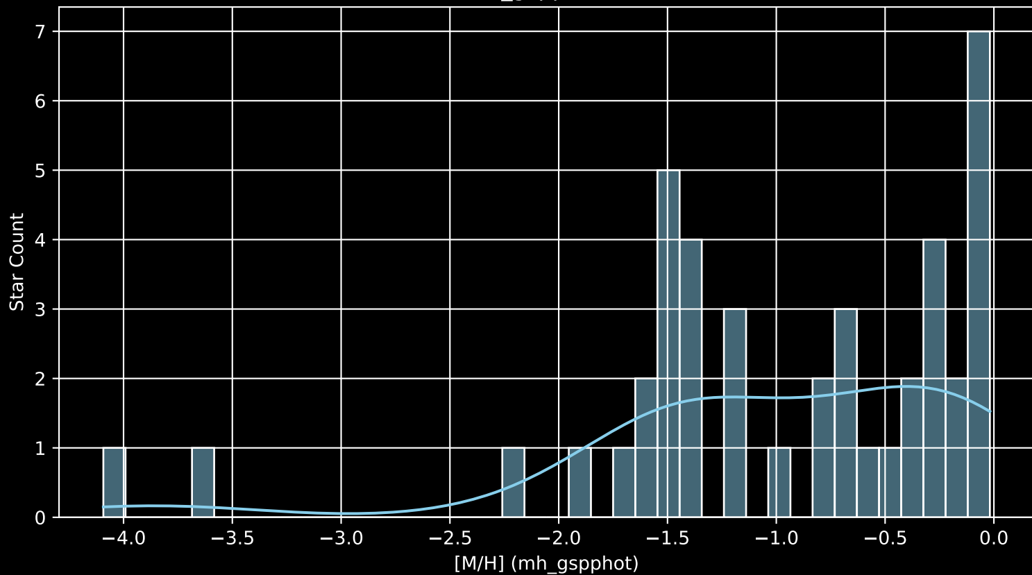
Gaia Cluster: [BH_73 [M/H] (mh_gspphot) (n= 42)
