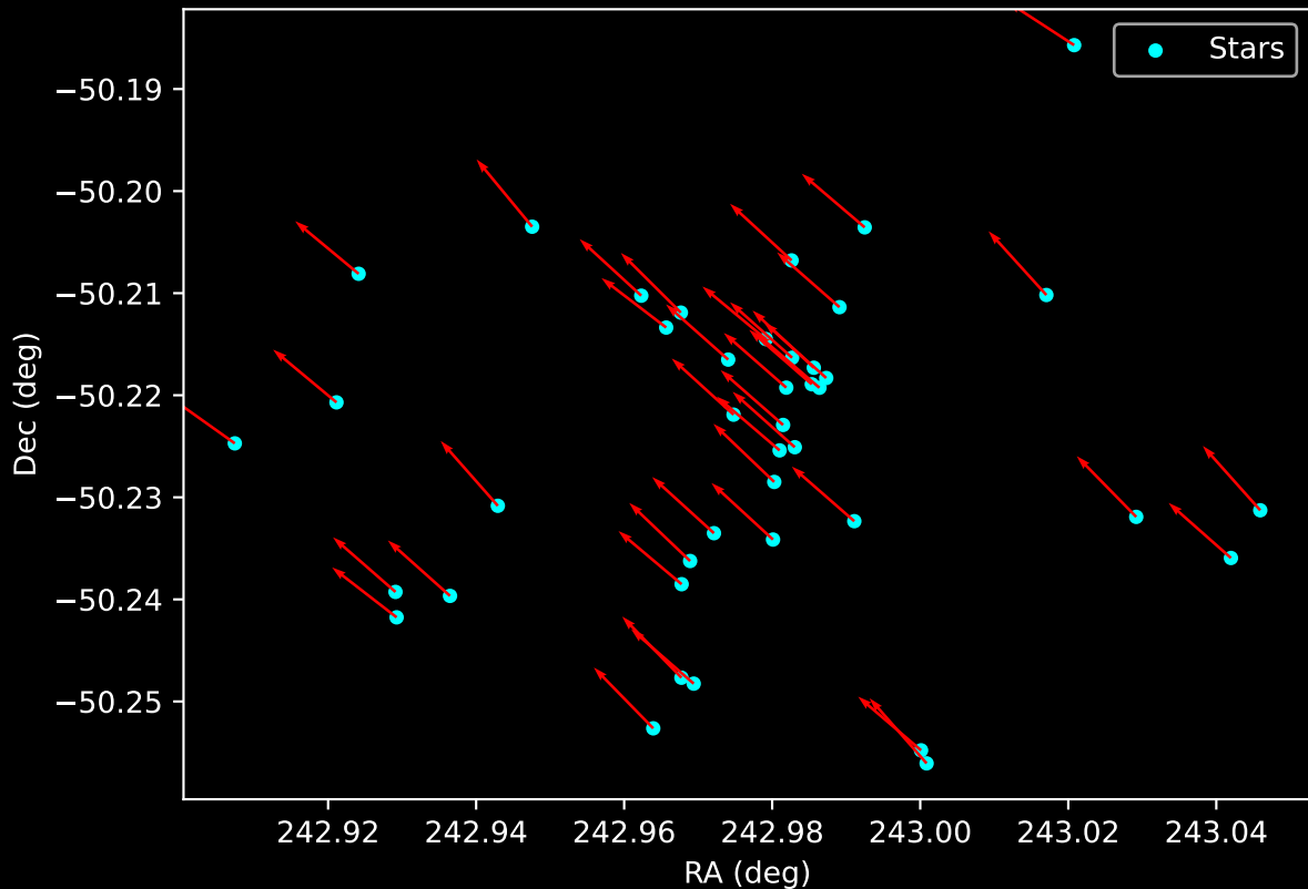
Gaia Cluster: [BH_73] Proper Motion Vectors for Gaia Star Field (n= 42)
