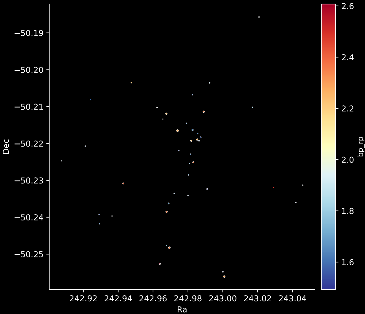
Gaia Cluster: [BH_73] Stars: 42
