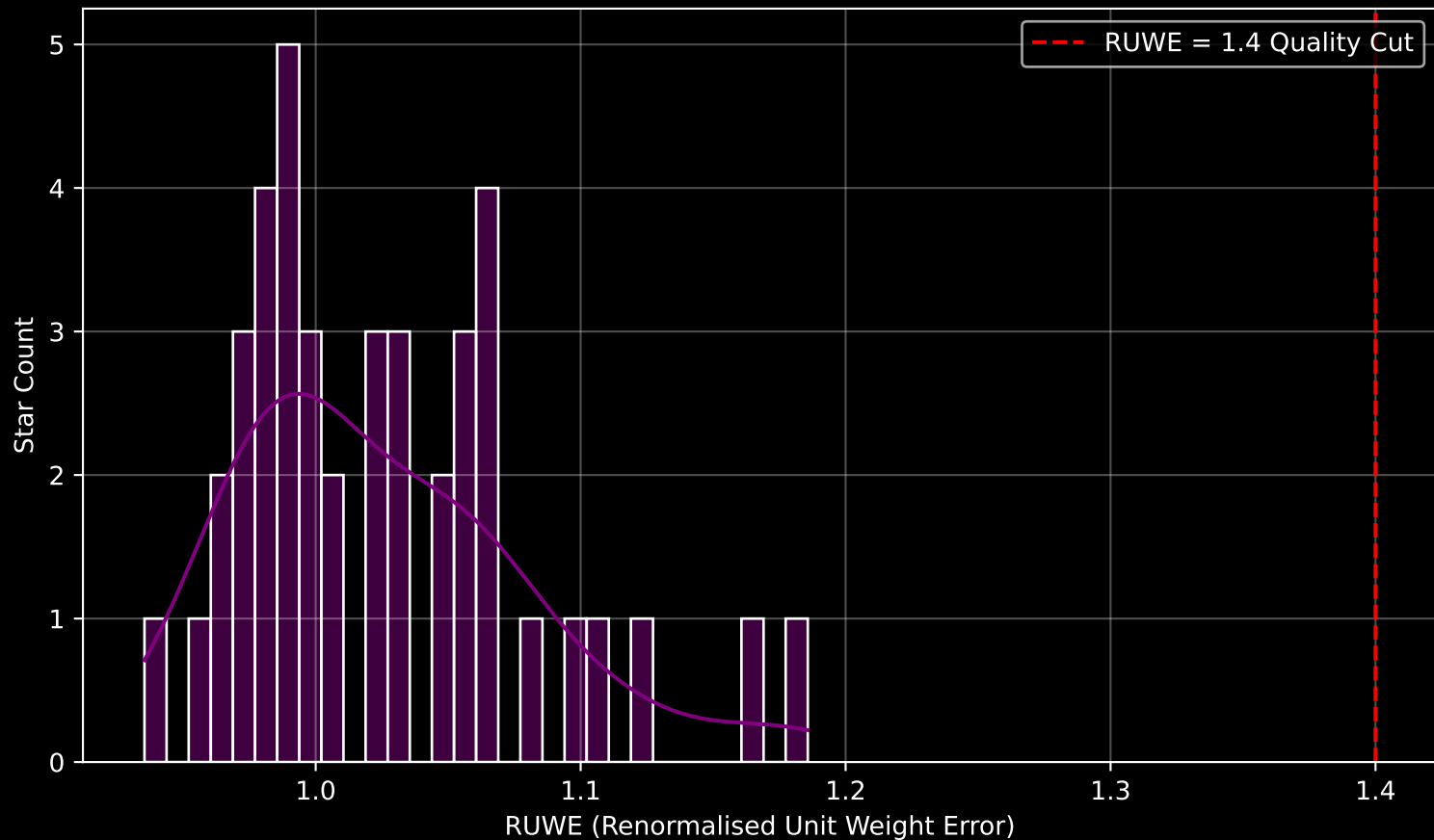
Gaia Cluster: [BH_73] RUWE Distribution (n= 42)
