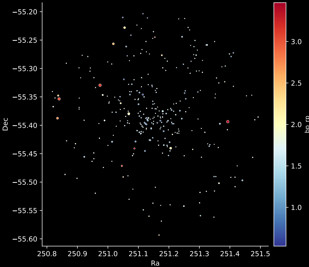
Gaia Cluster: [BH_87] Stars: 307
