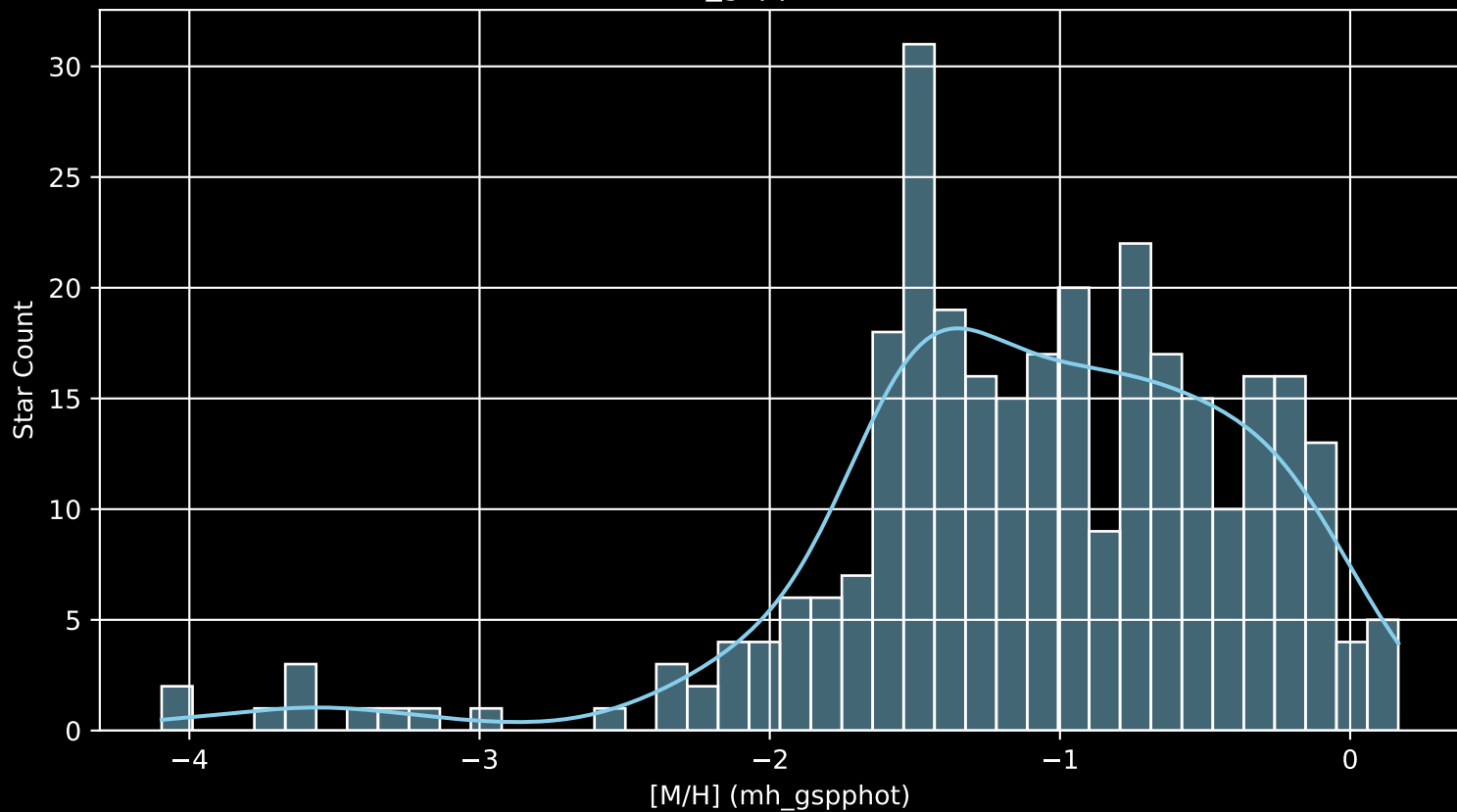
Gaia Cluster: [BH_87 [M/H] (mh_gspphot) (n= 306)
