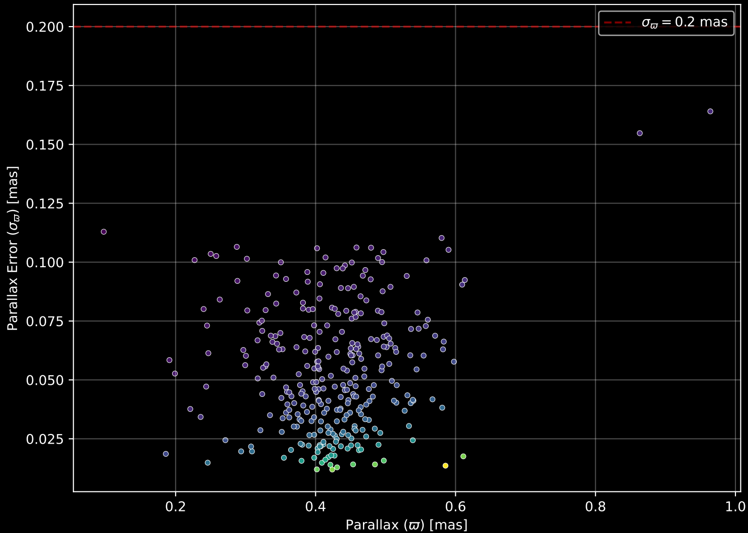
Gaia Cluster: [BH_87] Parallax Quality (n= 307)
