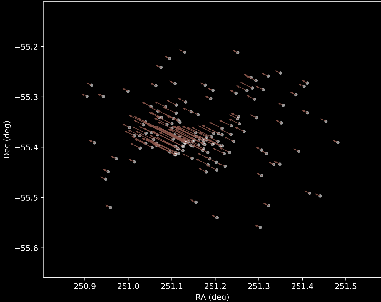
Gaia DR3 Cluster 10 Proper Motion Vectors (n=144)
