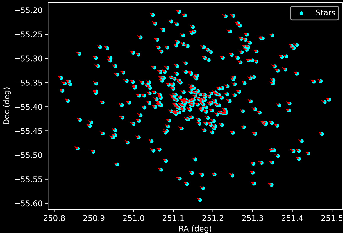
Gaia Cluster: [BH_87] Proper Motion Vectors for Gaia Star Field (n= 307)
