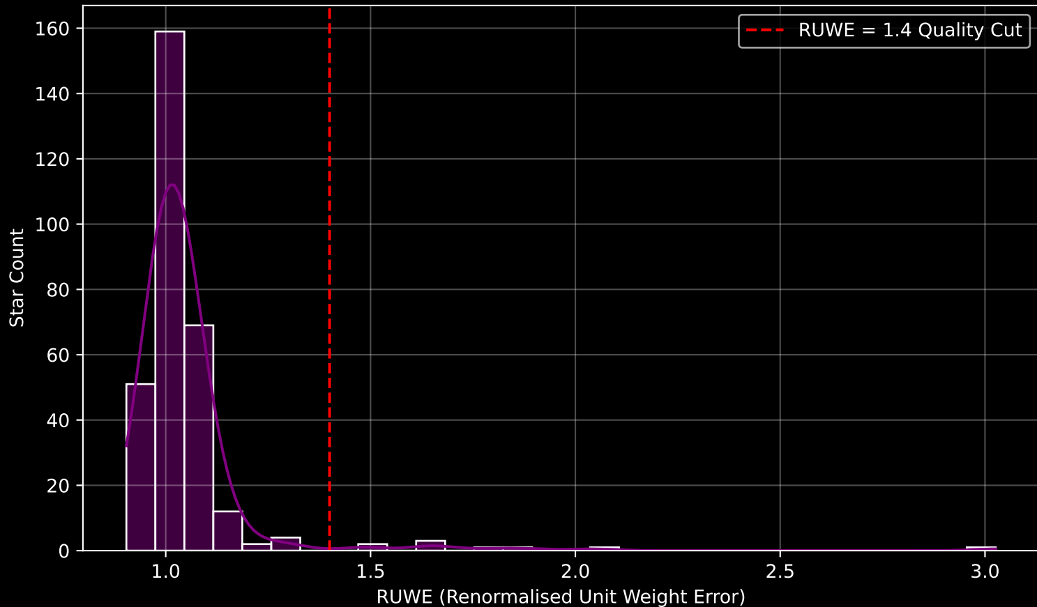
Gaia Cluster: [BH_87] RUWE Distribution (n= 306)
