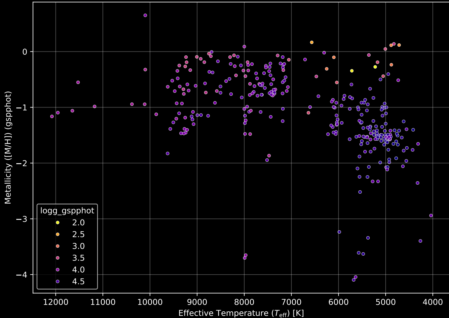
Gaia Cluster: [BH_87] Stellar Population Parameters (n= 307)
