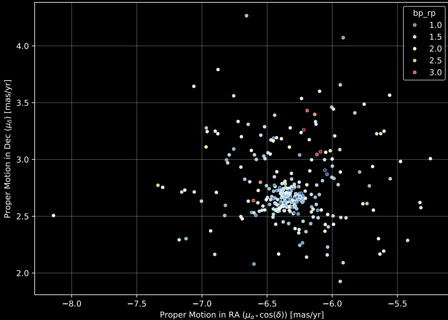
Gaia Cluster: [BH_87] Proper Motion Diagram (n= 307)
