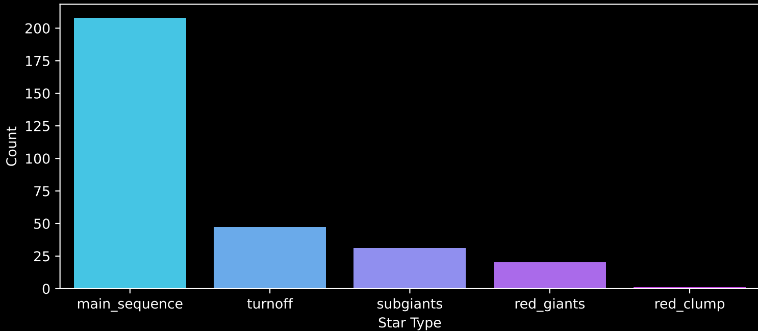
Gaia Cluster: [BH_87] Count plot of Star Type
