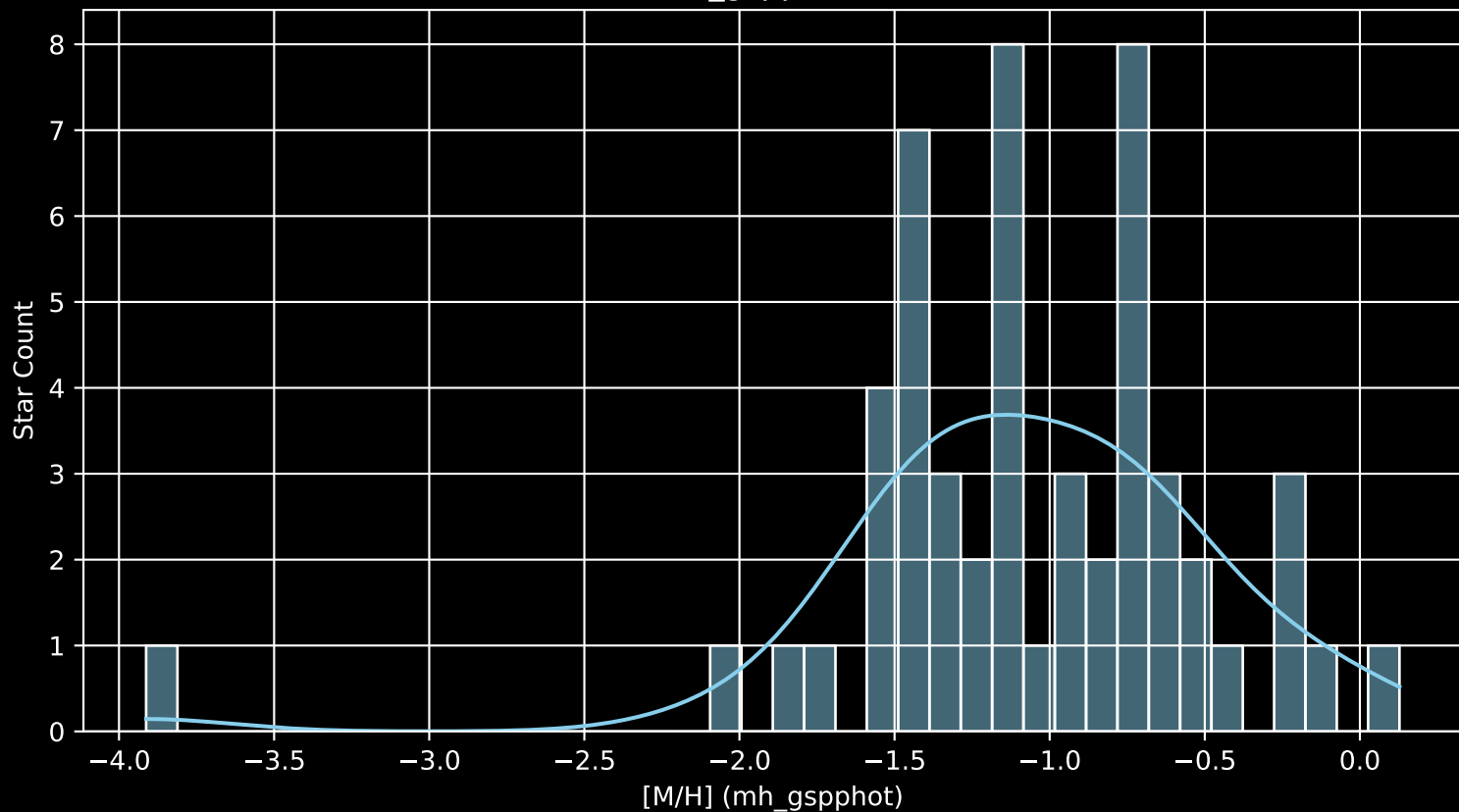
Gaia Cluster: [BH_92 [M/H] (mh_gspphot) (n= 53)
