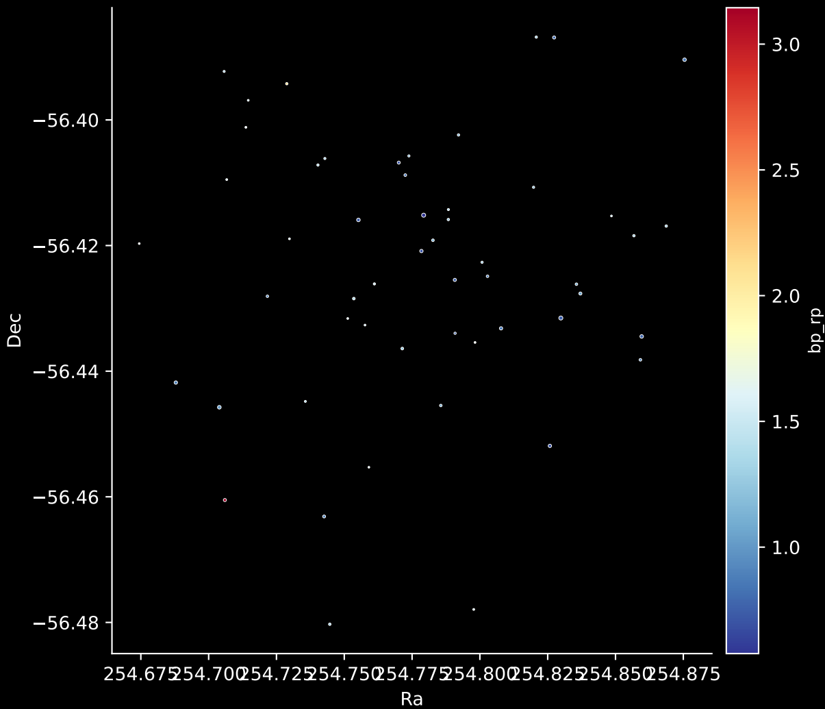
Gaia Cluster: [BH_92] Stars: 53
