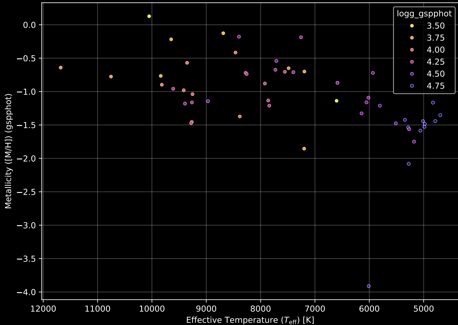
Gaia Cluster: [BH_92] Stellar Population Parameters (n= 53)
