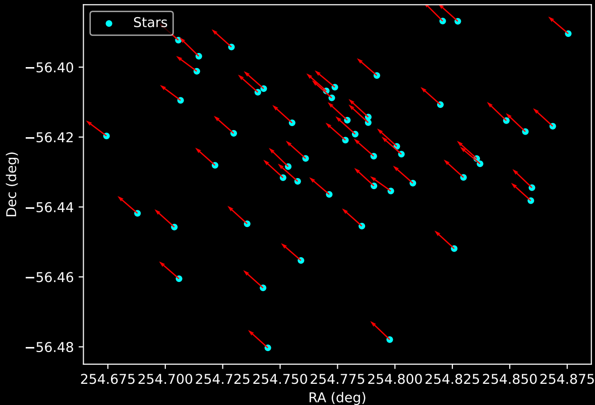
Gaia Cluster: [BH_92] Proper Motion Vectors for Gaia Star Field (n= 53)
