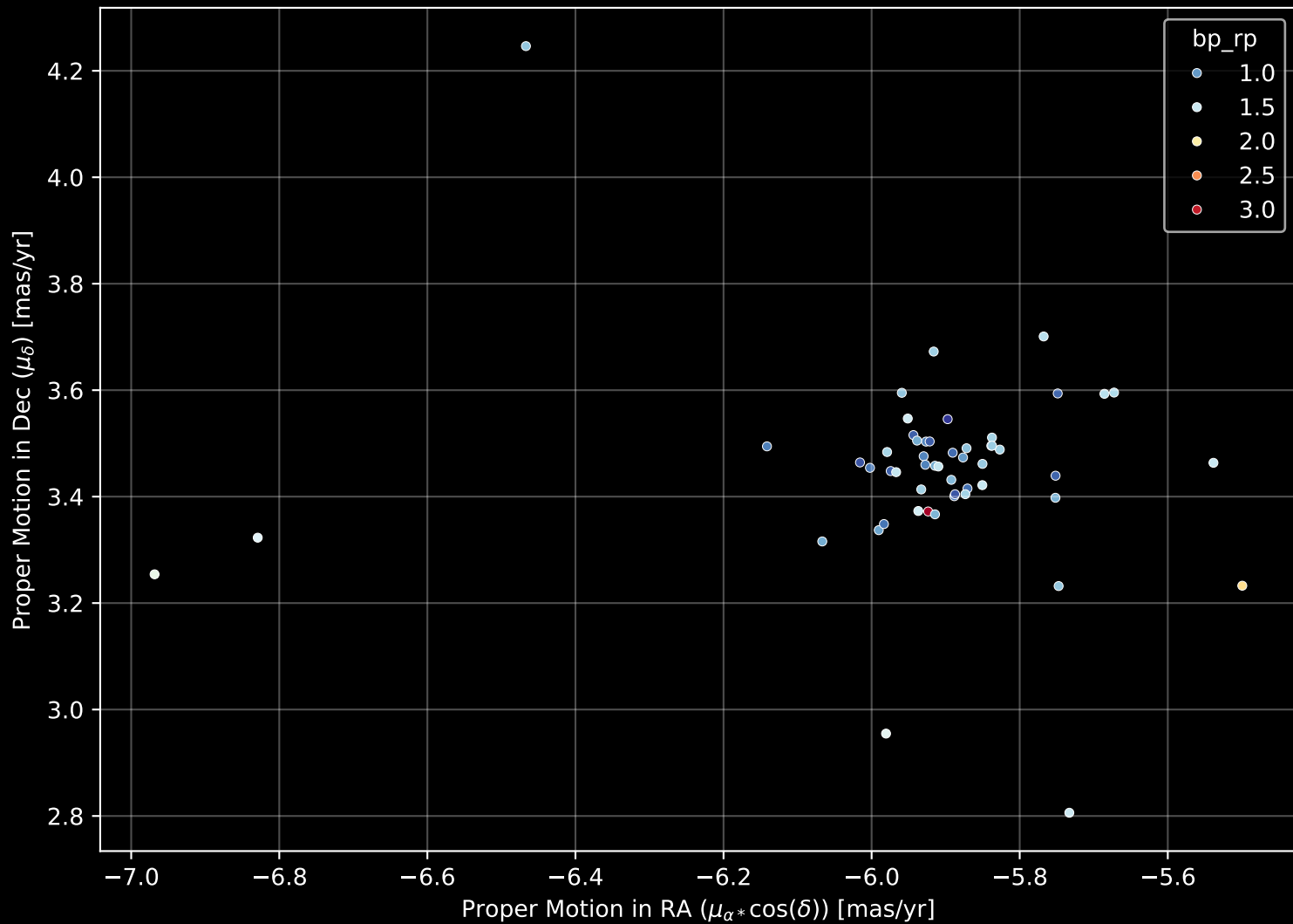
Gaia Cluster: [BH 92] Proper Motion Diagram (n= 53)
