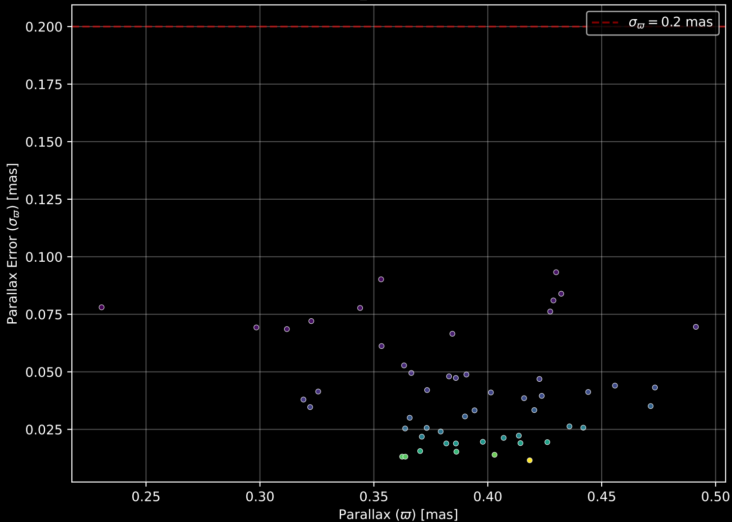
Gaia Cluster: [BH_92] Parallax Quality (n= 53)
