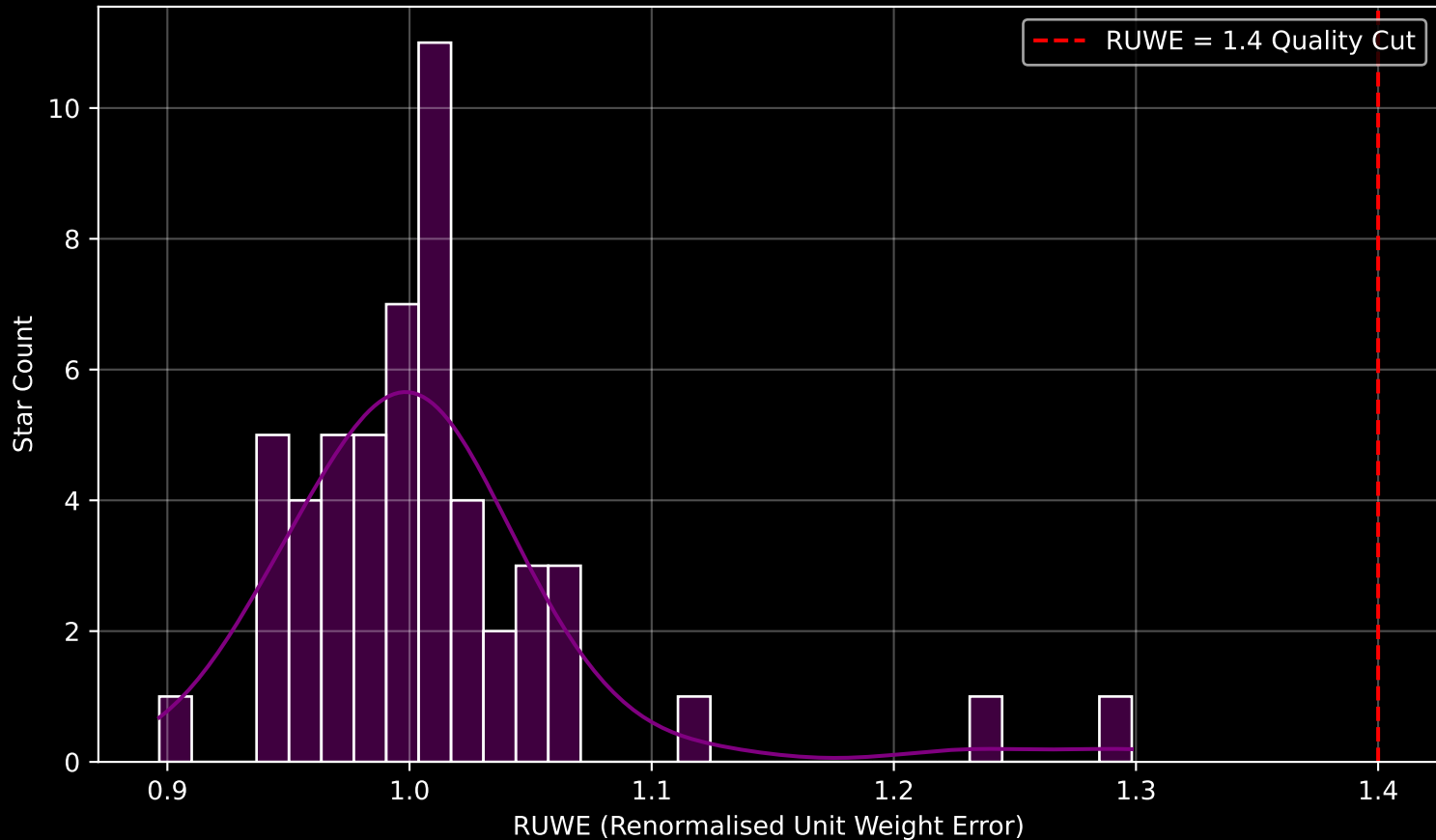
Gaia Cluster: [BH_92] RUWE Distribution (n= 53)
