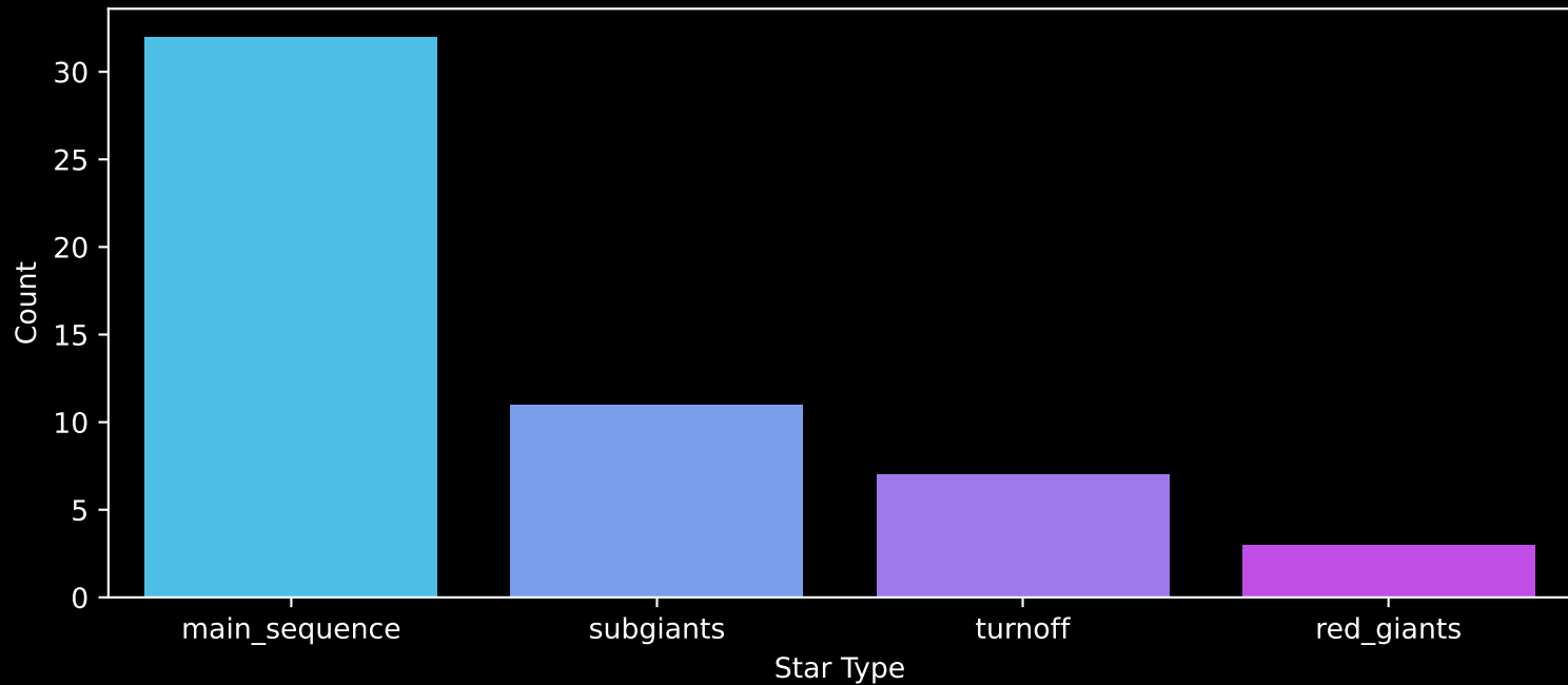
Gaia Cluster: [BH_92] Count plot of Star Type
