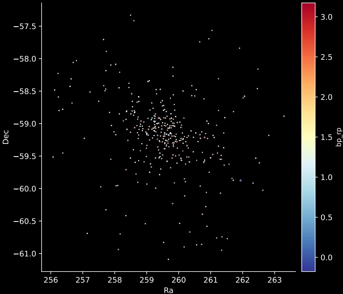
Gaia Cluster: [BH_99] Stars: 356
