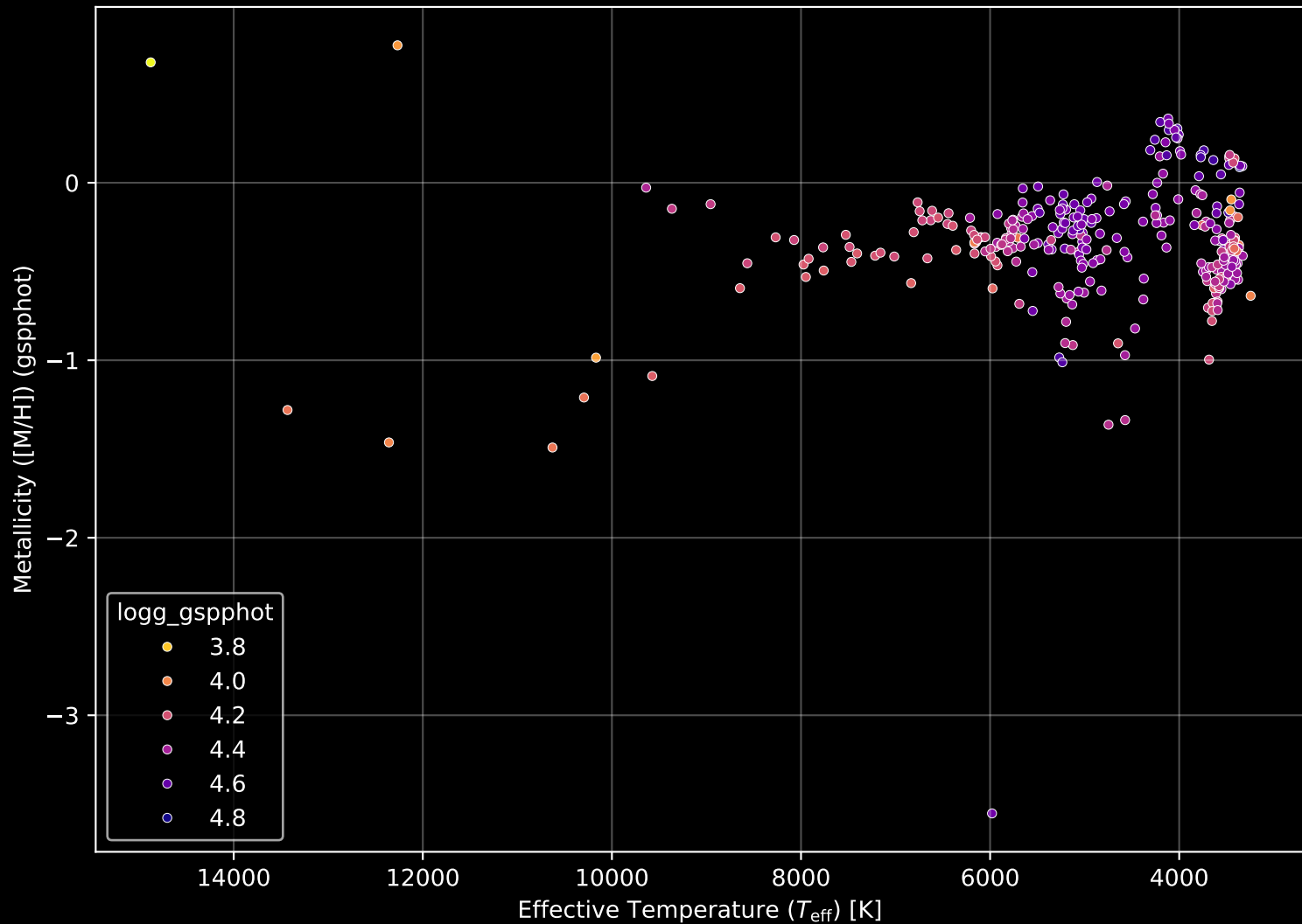
Gaia Cluster: [BH_99] Stellar Population Parameters (n= 356)
