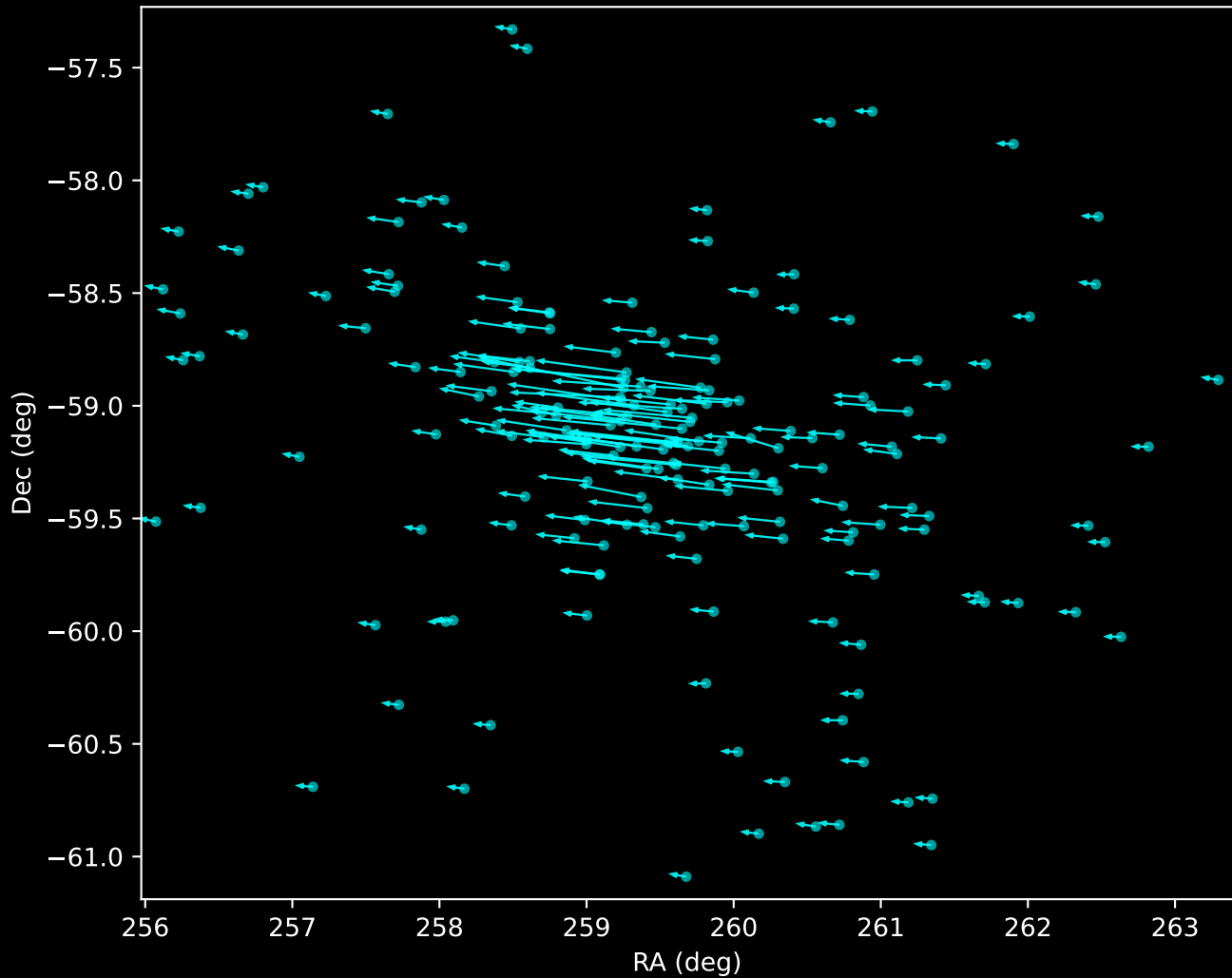
Gaia DR3 Noise Stream Proper Motion Vectors (n=192)
