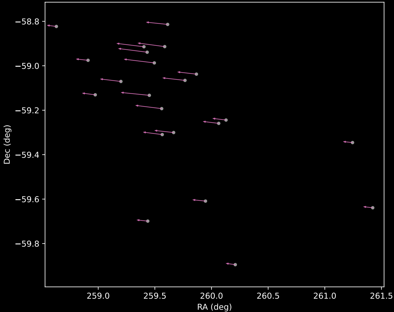
Gaia DR3 Cluster 12 Proper Motion Vectors (n=22)
