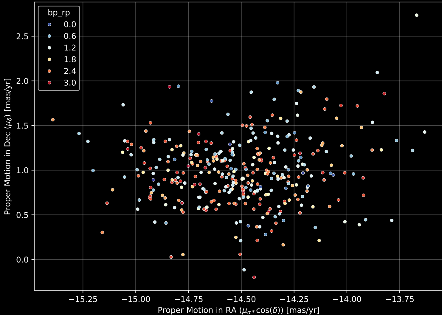
Gaia Cluster: [BH_99] Proper Motion Diagram (n= 356)
