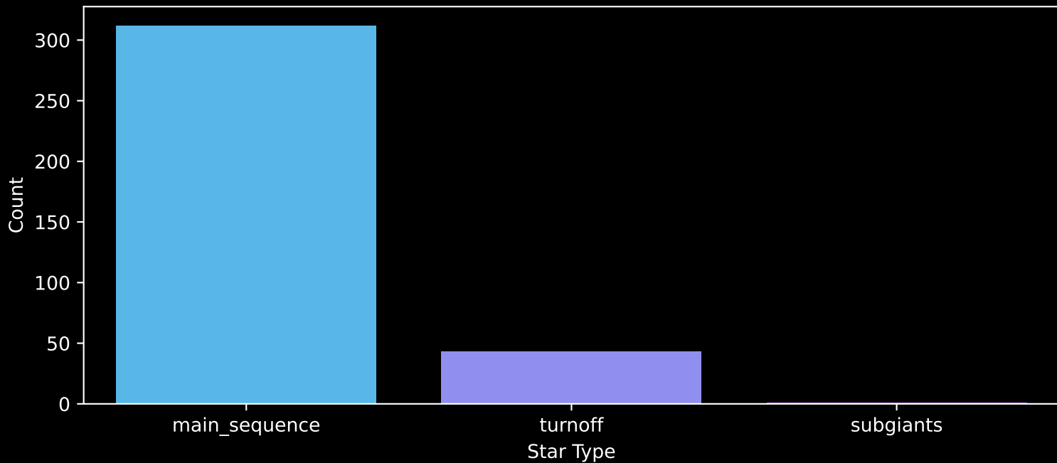
Gaia Cluster: [BH_99] Count plot of Star Type
