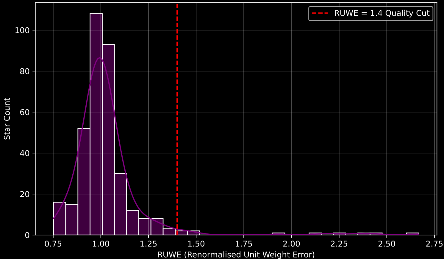
Gaia Cluster: [BH_99] RUWE Distribution (n= 355)
