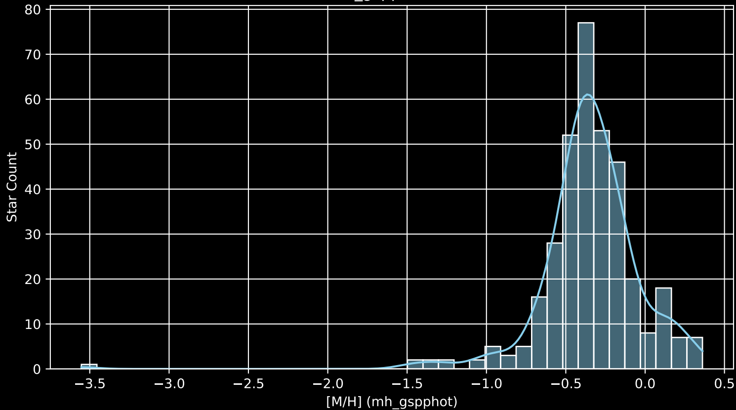
Gaia Cluster: [BH_99 [M/H] (mh_gspphot) (n= 354)
