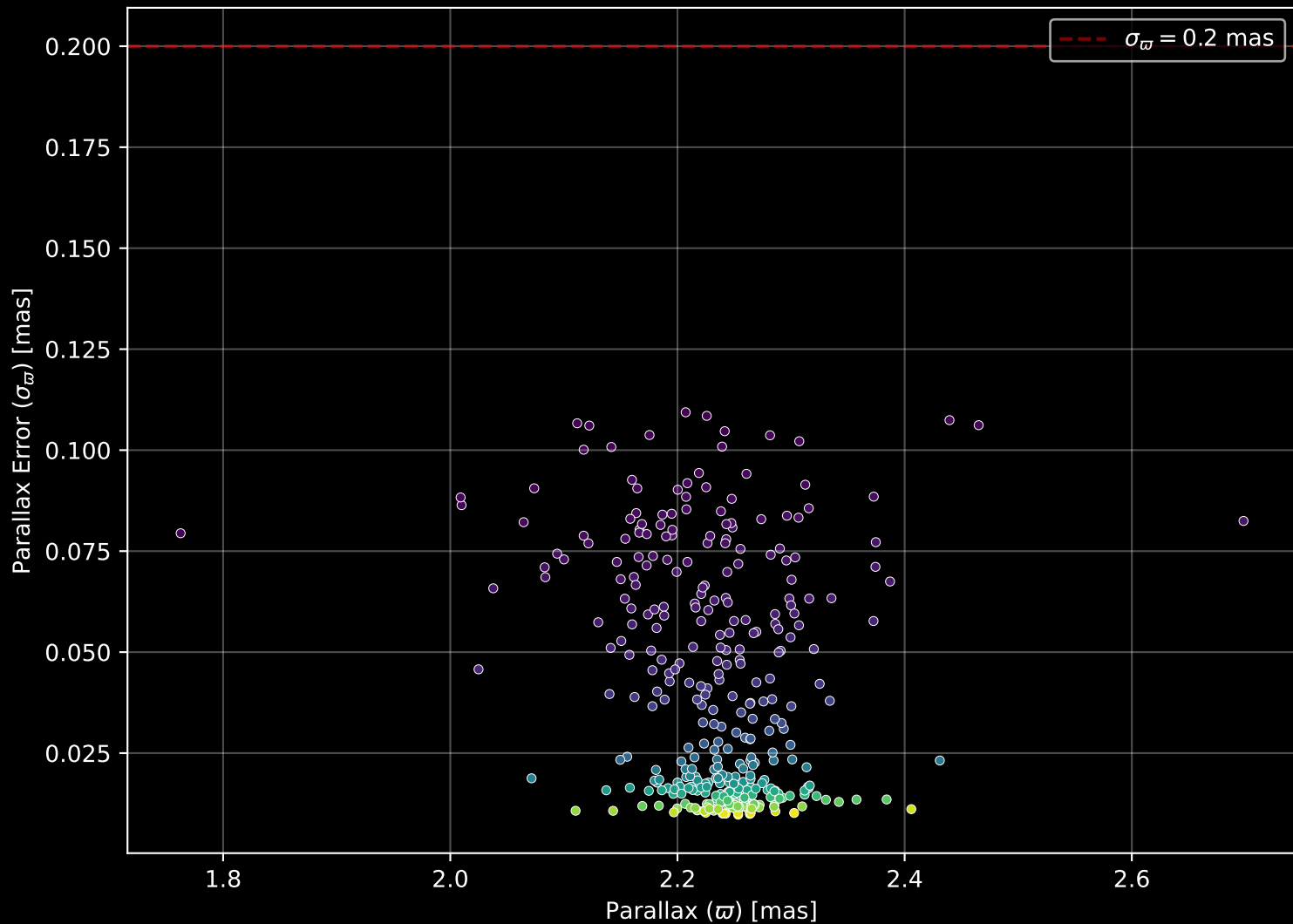
Gaia Cluster: [BH_99] Parallax Quality (n= 356)
