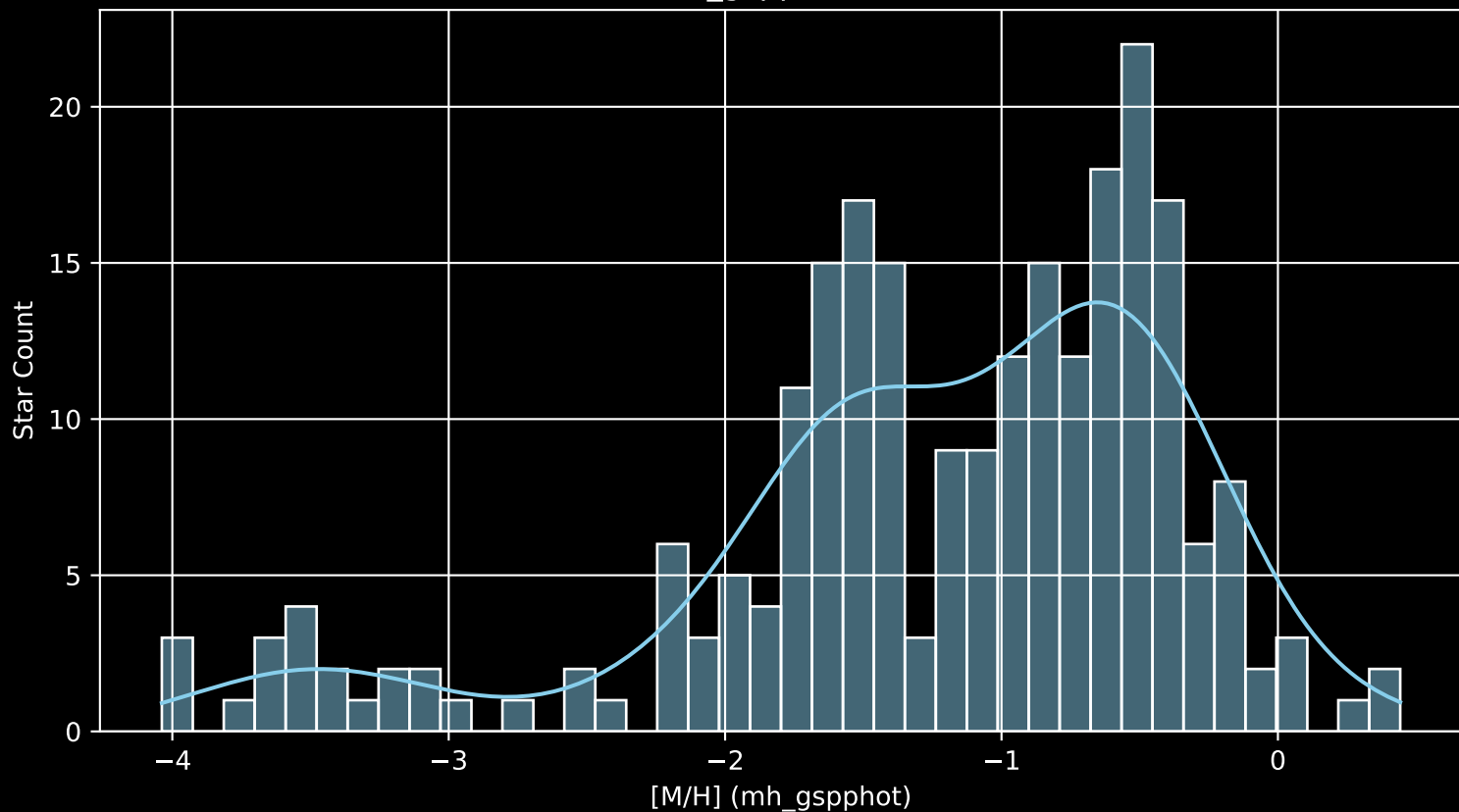
Gaia Cluster: [Basel_17 [M/H] (mh_gspphot) (n= 238)
