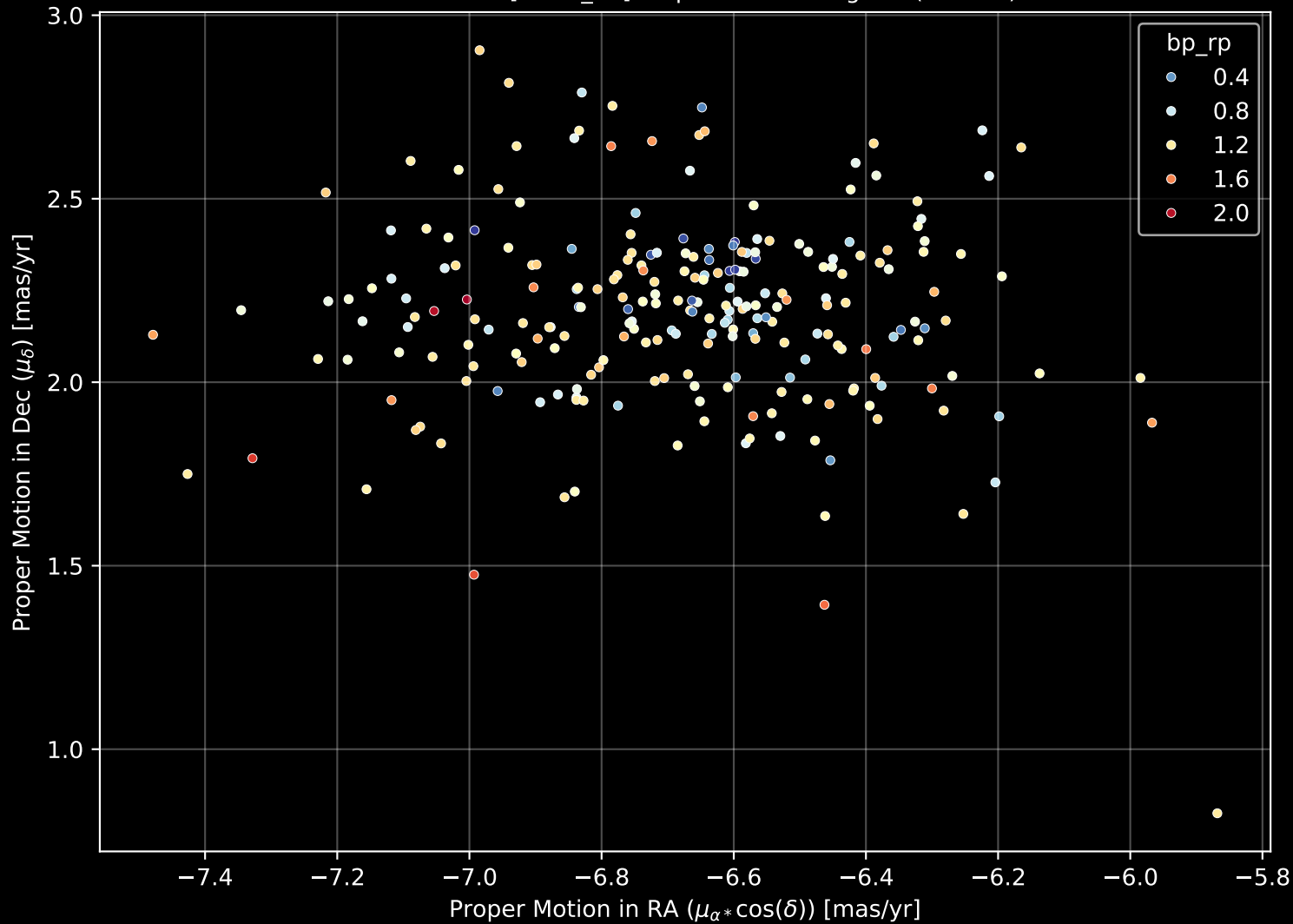
Gaia Cluster: [Basel_17] Proper Motion Diagram (n= 239)
