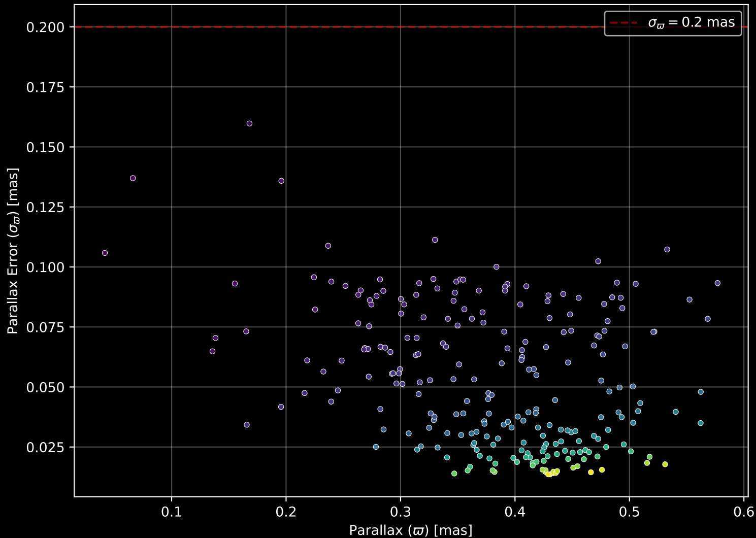
Gaia Cluster: [Basel_17] Parallax Quality (n= 239)
