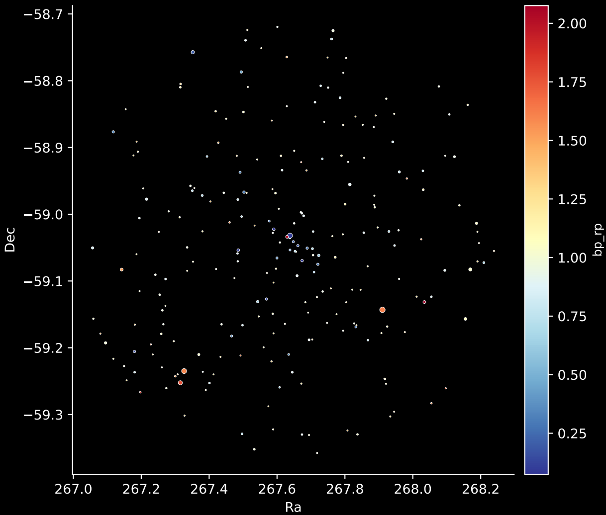
Gaia Cluster: [Basel_17] Stars: 239
