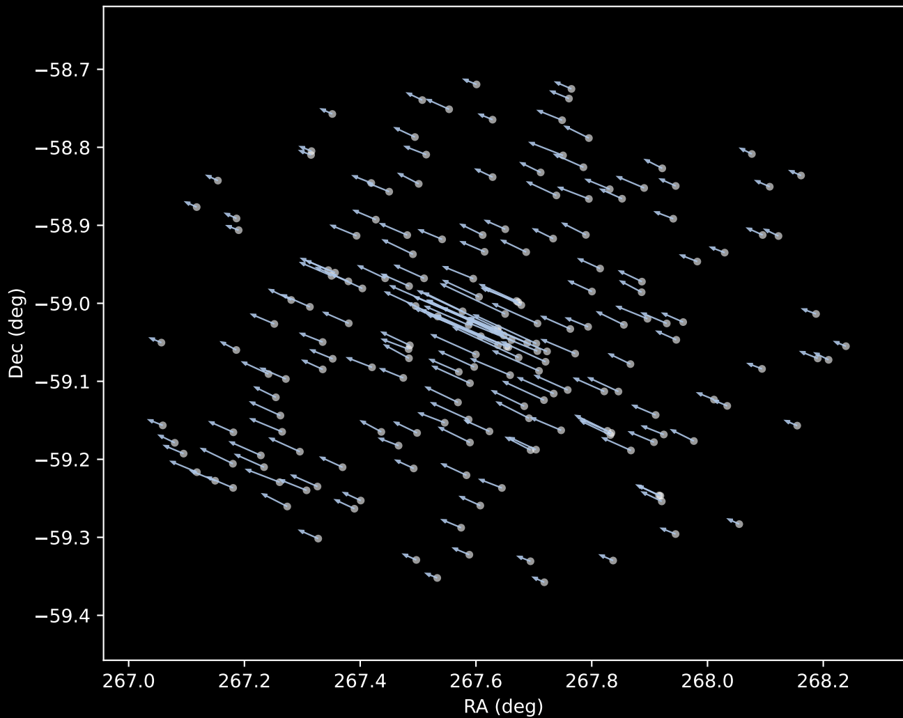
Gaia DR3 Cluster 1 Proper Motion Vectors (n=192)
