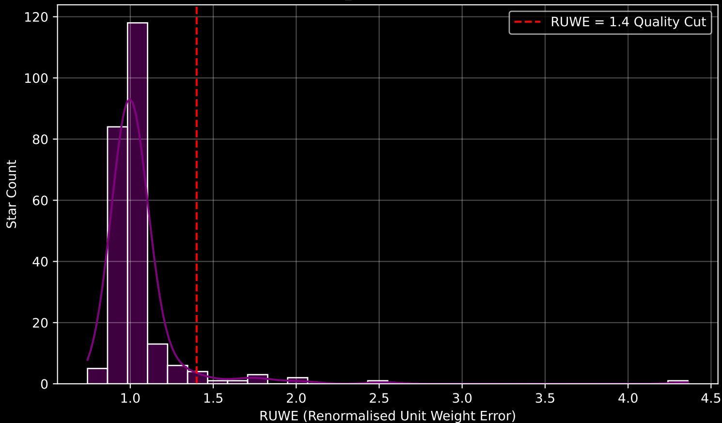
Gaia Cluster: [Basel_17] RUWE Distribution (n= 239)
