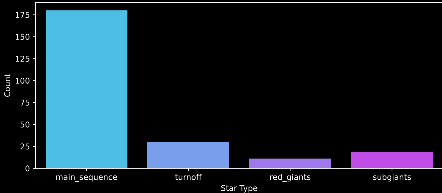
Gaia Cluster: [Basel_17] Count plot of Star Type
