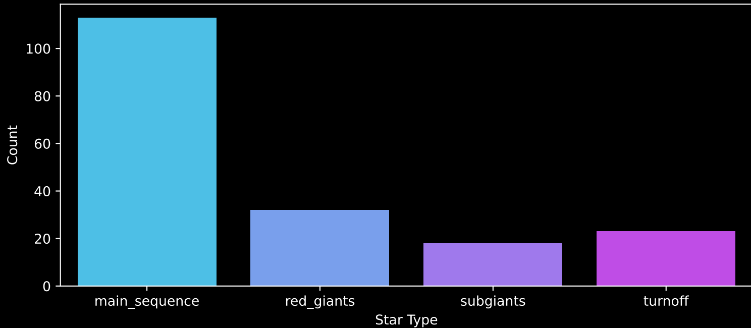
Gaia Cluster: [Berkeley_10] Count plot of Star Type
