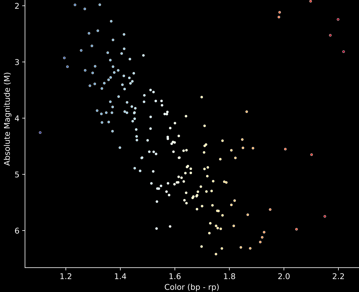
Gaia Cluster: [Berkeley_10] Stars (n= 186) Hertzsprung-Russel Diagram
