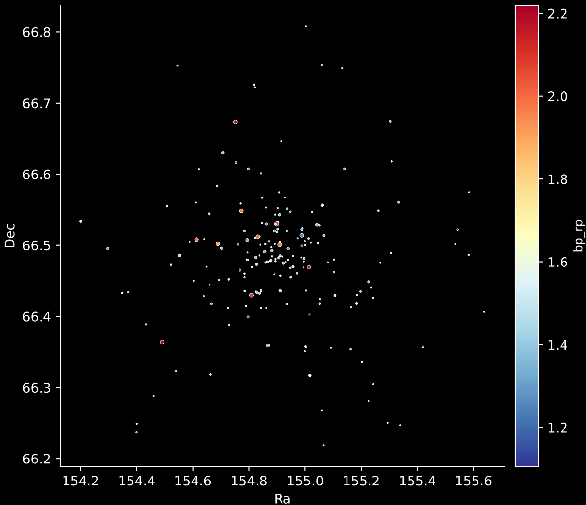
Gaia Cluster: [Berkeley_10] Stars: 186
