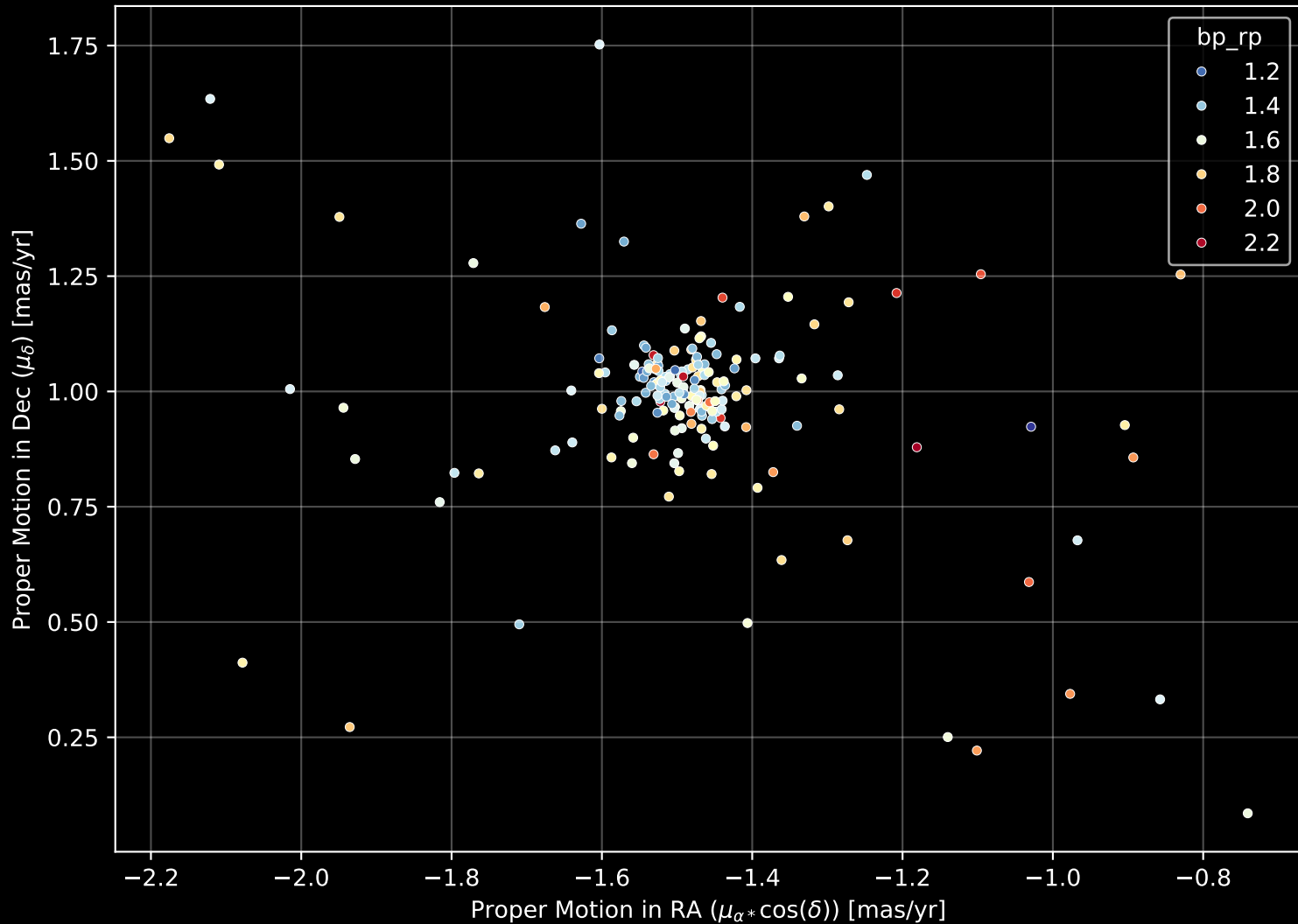
Gaia Cluster: [Berkeley_10] Proper Motion Diagram (n= 186)
