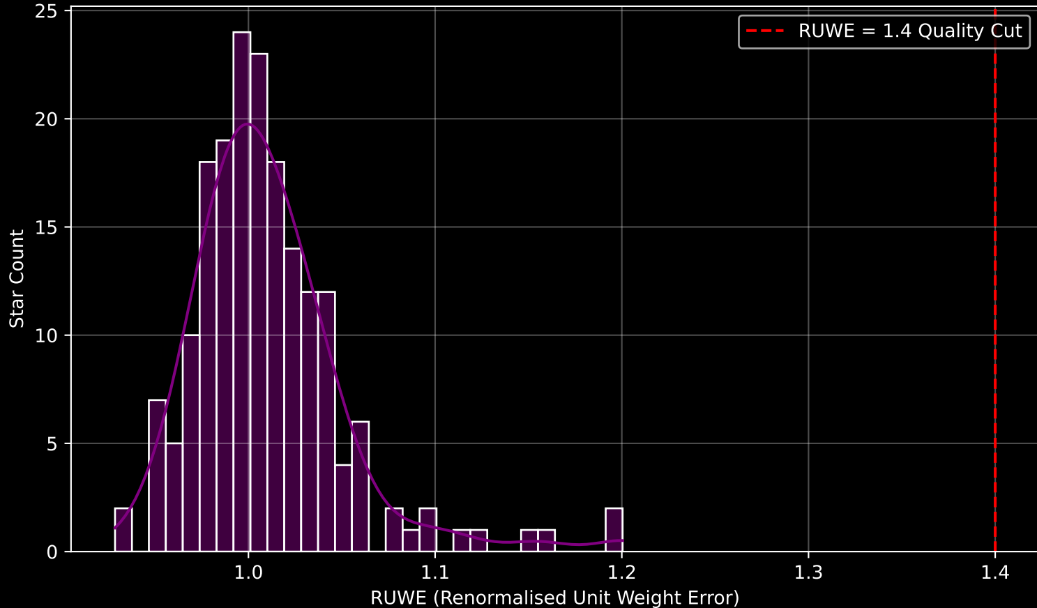
Gaia Cluster: [Berkeley_10] RUWE Distribution (n= 185)
