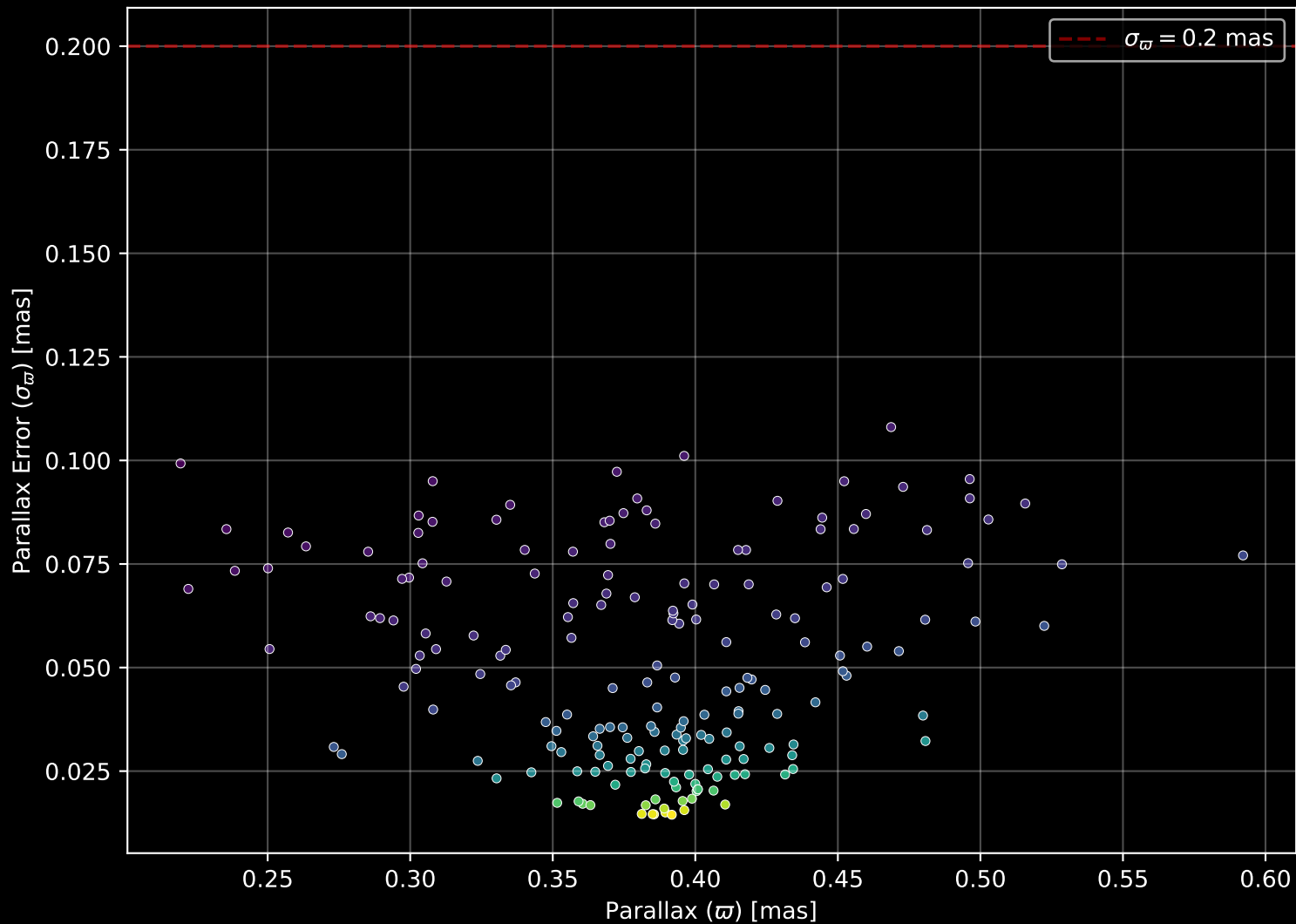
Gaia Cluster: [Berkeley_10] Parallax Quality (n= 186)
