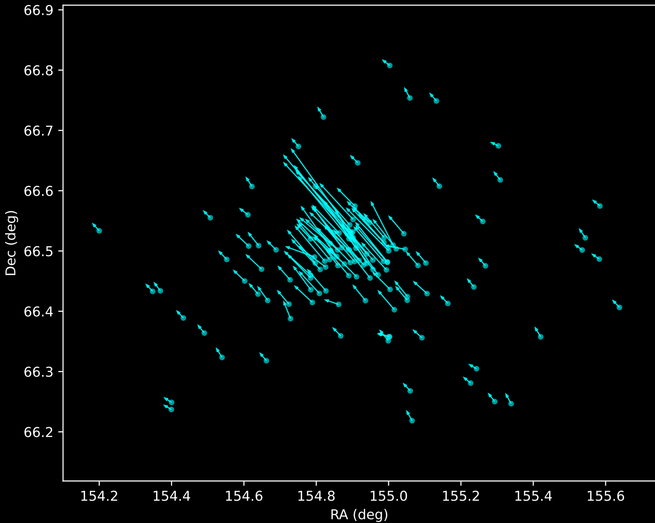
Gaia DR3 Noise Stream Proper Motion Vectors (n=122)
