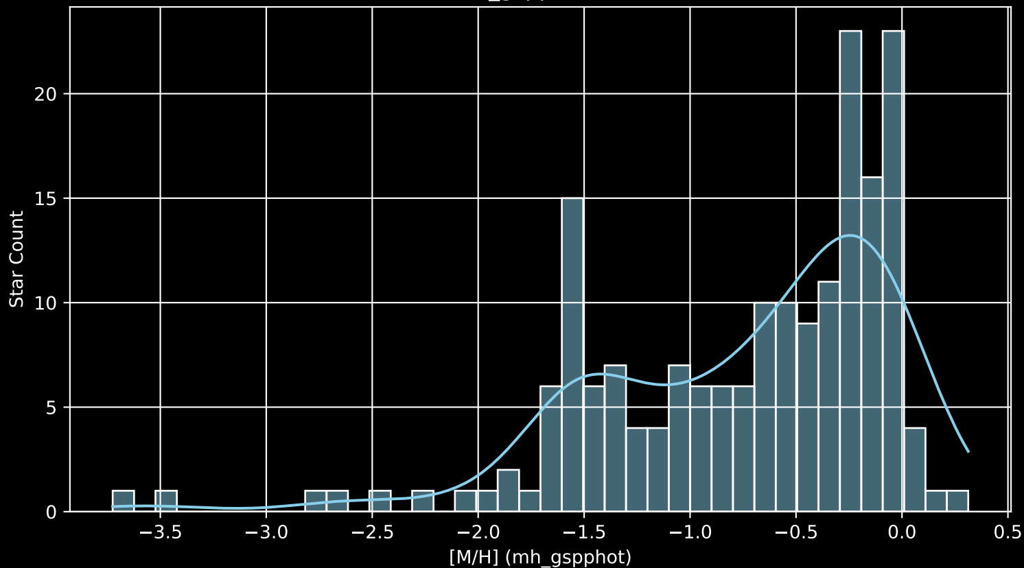
Gaia Cluster: [Berkeley_10 [M/H] (mh_gspphot) (n= 186)
