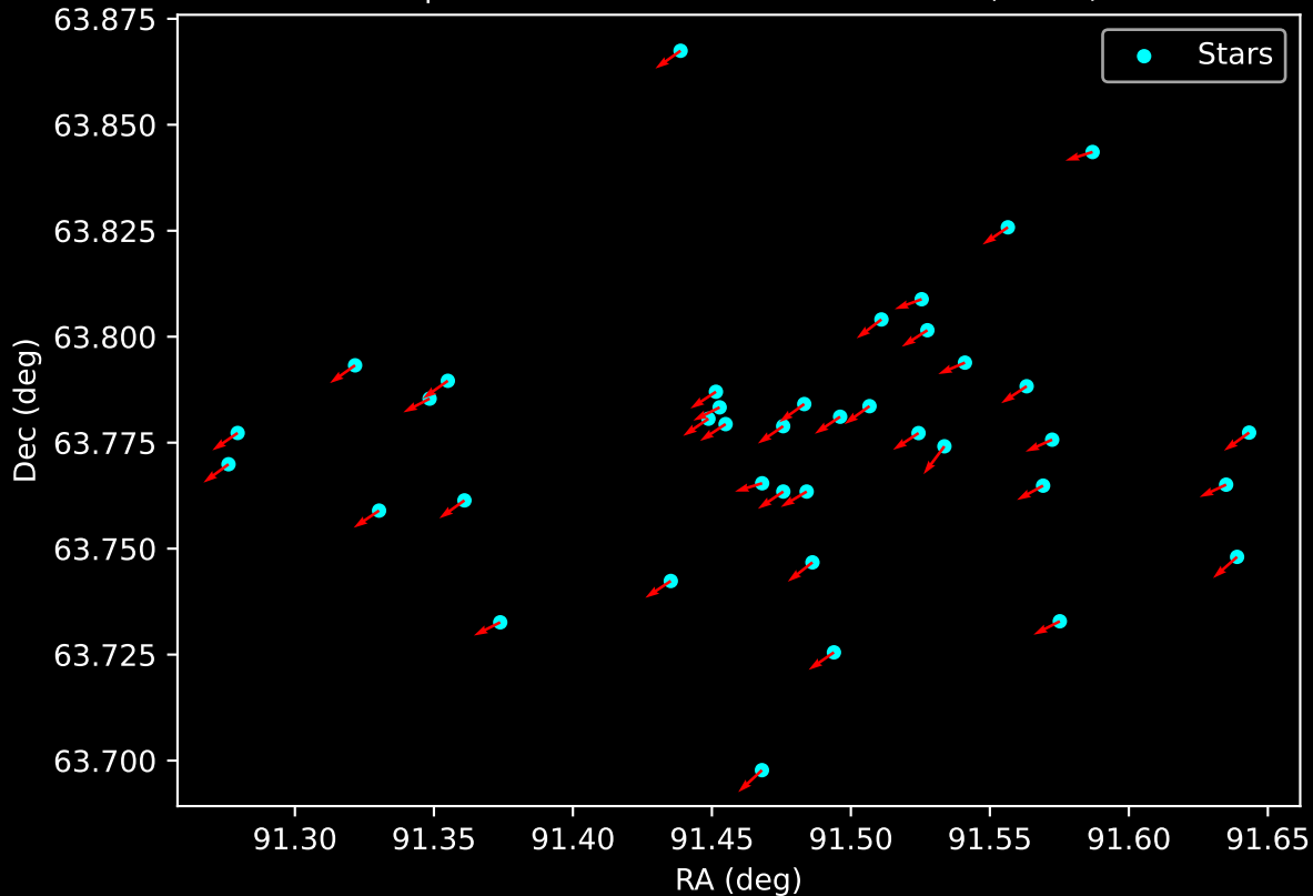
Gaia Cluster: [Berkeley_100] Proper Motion Vectors for Gaia Star Field (n= 39)
