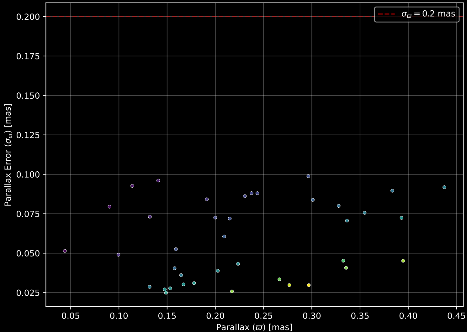
Gaia Cluster: [Berkeley_100] Parallax Quality (n= 39)
