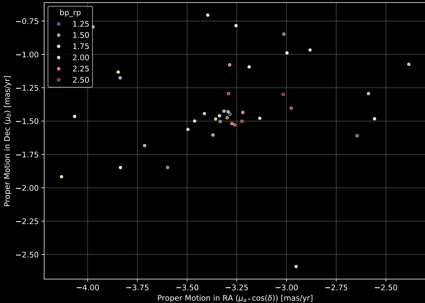
Gaia Cluster: [Berkeley_100] Proper Motion Diagram (n= 39)
