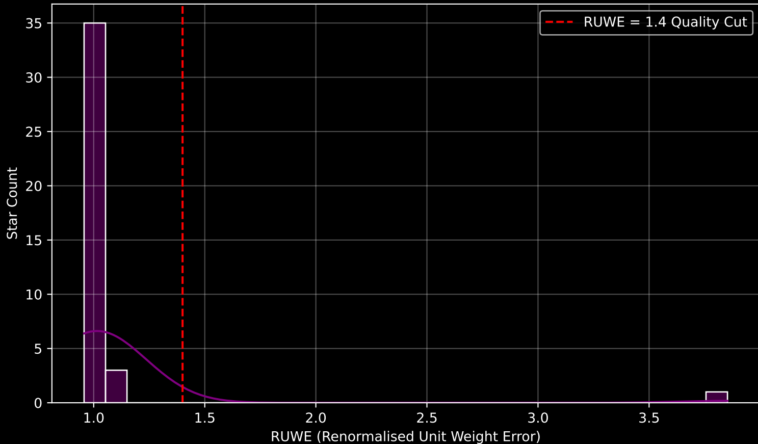
Gaia Cluster: [Berkeley_100] RUWE Distribution (n= 39)
