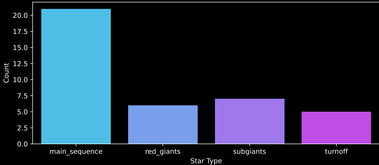
Gaia Cluster: [Berkeley_100] Count plot of Star Type
