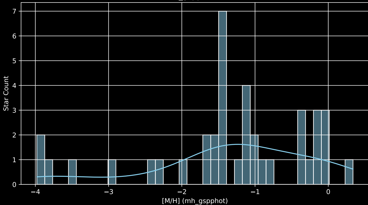
Gaia Cluster: [Berkeley_100 [M/H] (mh_gspphot) (n= 39)
