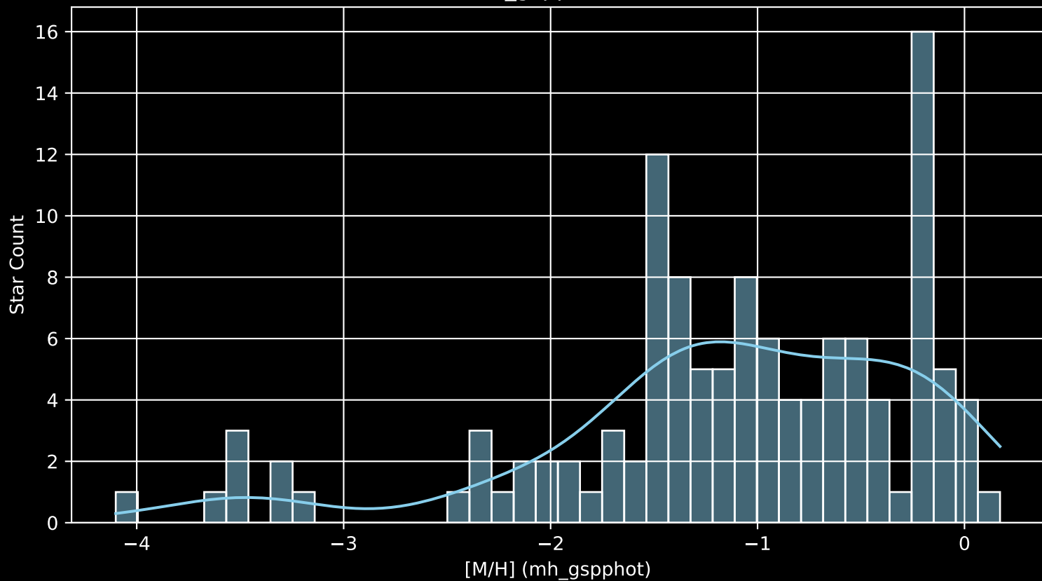
Gaia Cluster: [Berkeley_104 [M/H] (mh_gspphot) (n= 120)
