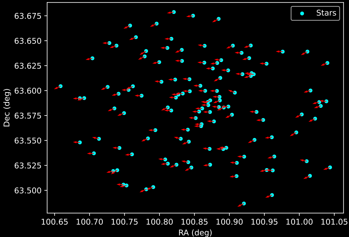
Gaia Cluster: [Berkeley_104] Proper Motion Vectors for Gaia Star Field (n= 121)
