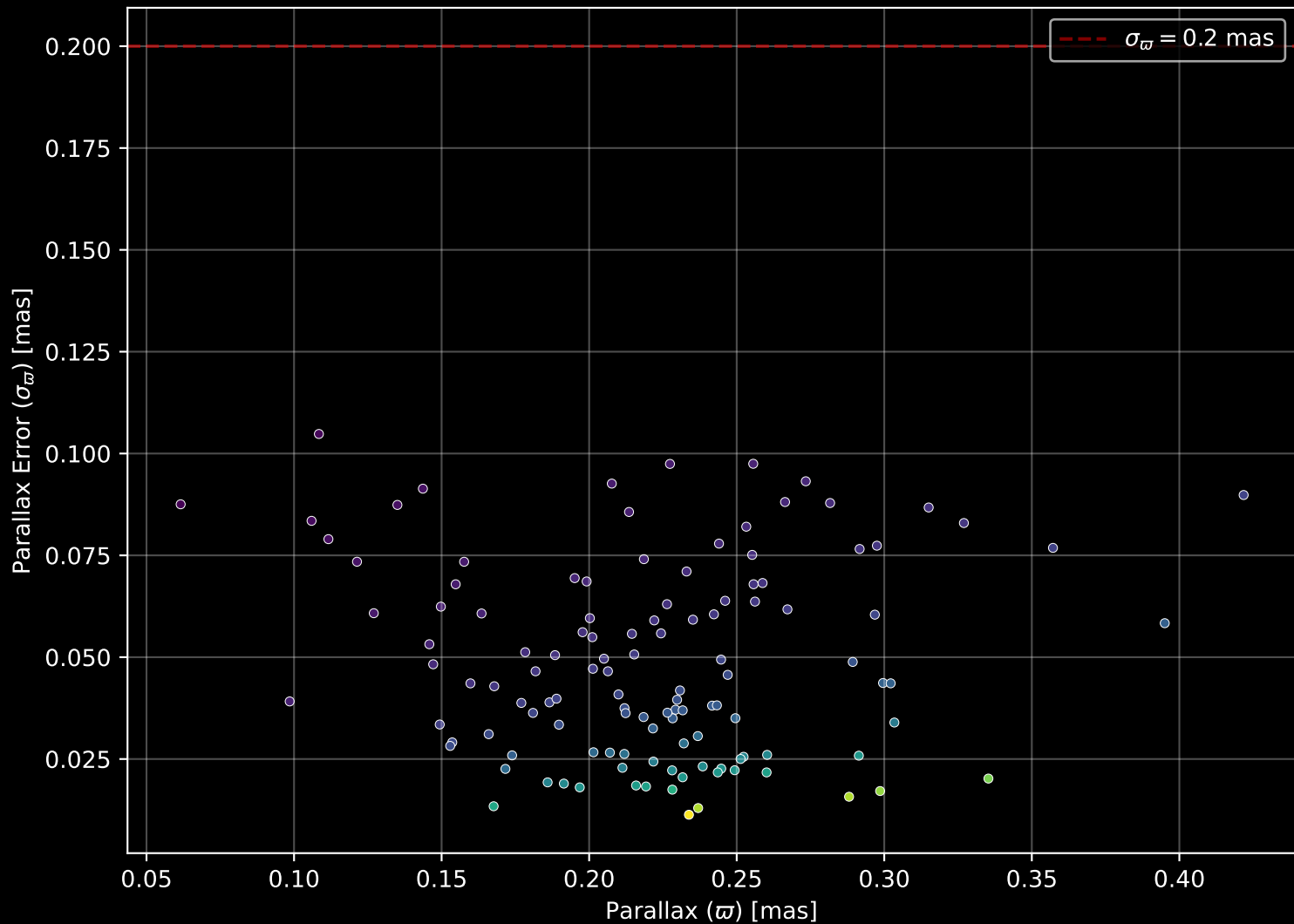
Gaia Cluster: [Berkeley_104] Parallax Quality (n= 121)
