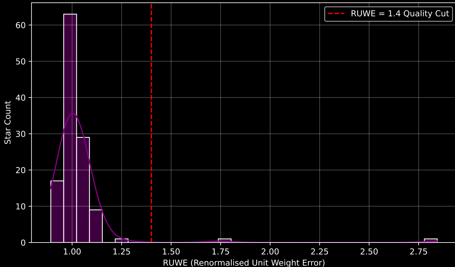
Gaia Cluster: [Berkeley_104] RUWE Distribution (n= 121)
