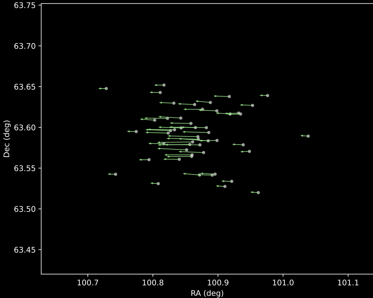
Gaia DR3 Cluster 5 Proper Motion Vectors (n=51)
