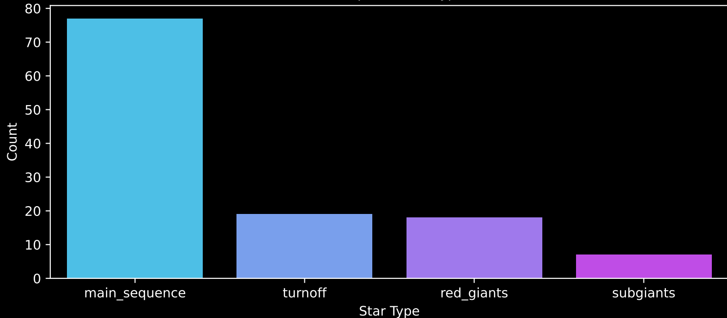
Gaia Cluster: [Berkeley_104] Count plot of Star Type
