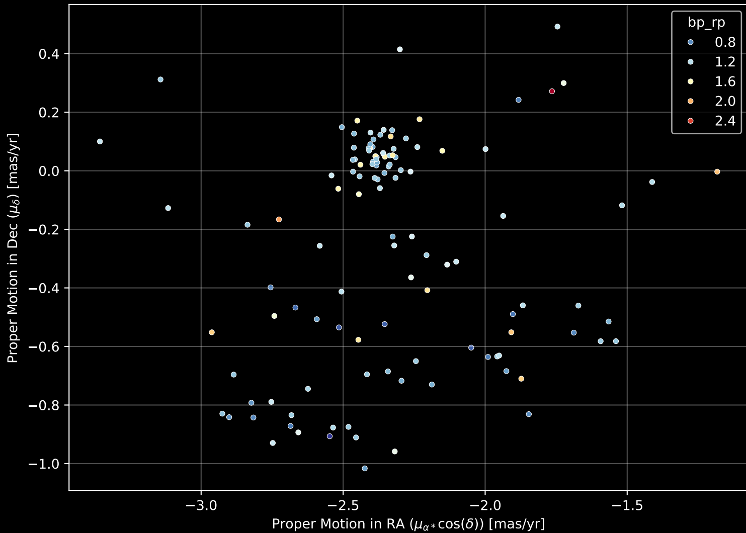
Gaia Cluster: [Berkeley_104] Proper Motion Diagram (n= 121)
