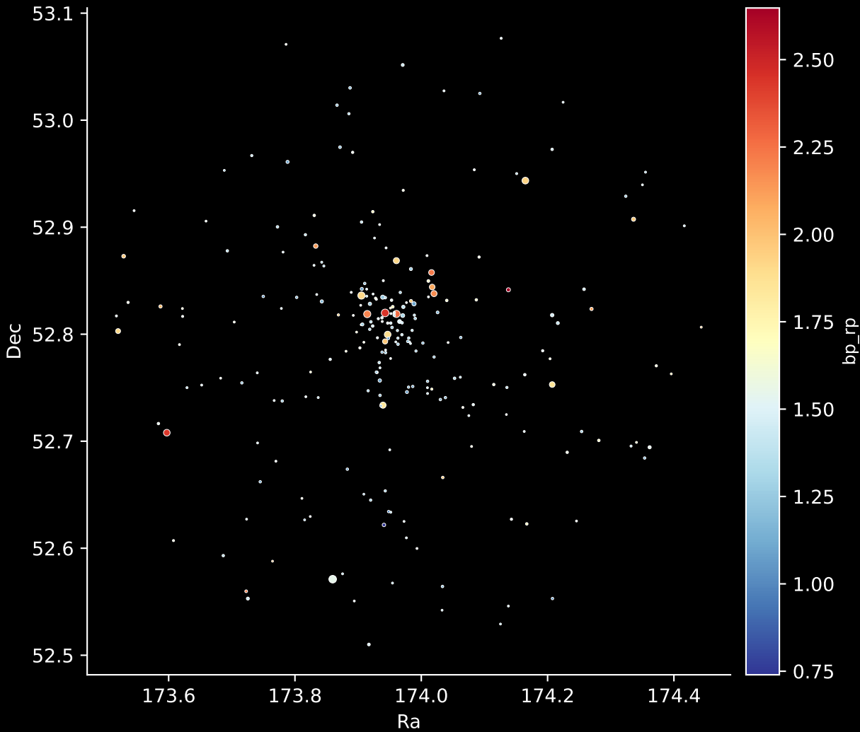
Gaia Cluster: [Berkeley_13] Stars: 237
