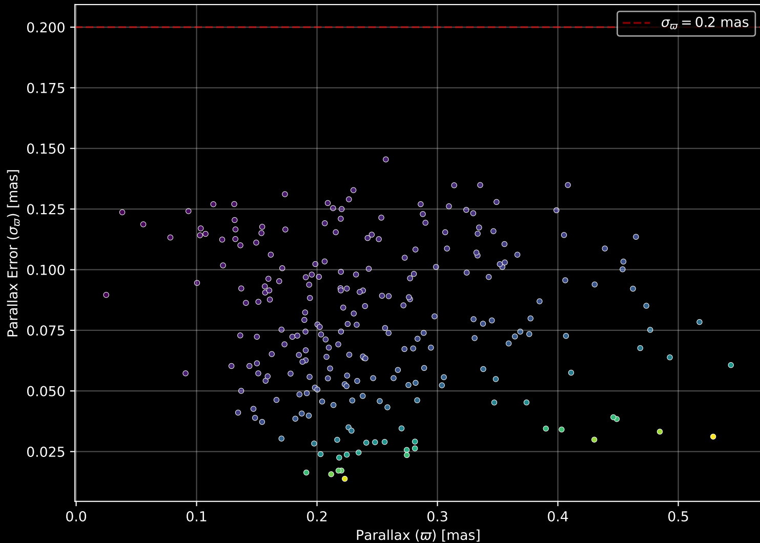
Gaia Cluster: [Berkeley_13] Parallax Quality (n= 237)
