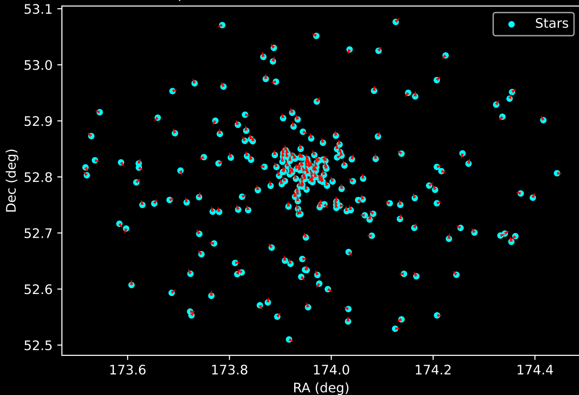
Gaia Cluster: [Berkeley_13] Proper Motion Vectors for Gaia Star Field (n= 237)
