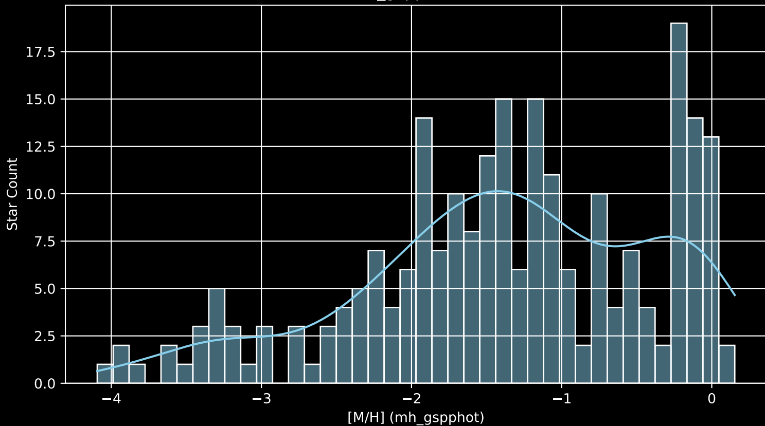
Gaia Cluster: [Berkeley_13 [M/H] (mh_gspphot) (n= 236)
