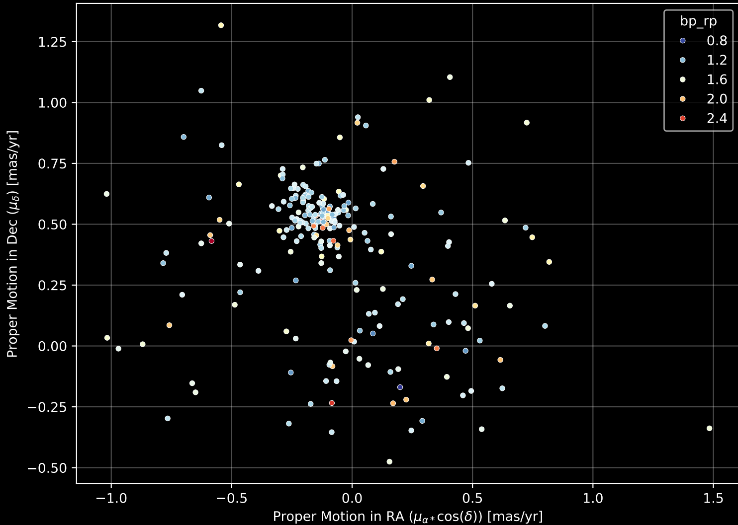
Gaia Cluster: [Berkeley_13] Proper Motion Diagram (n= 237)
