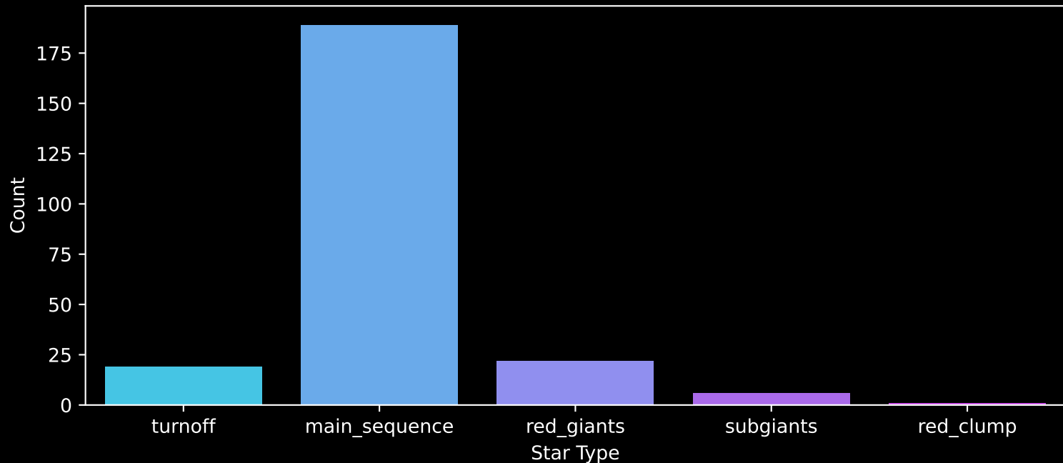
Gaia Cluster: [Berkeley_13] Count plot of Star Type
