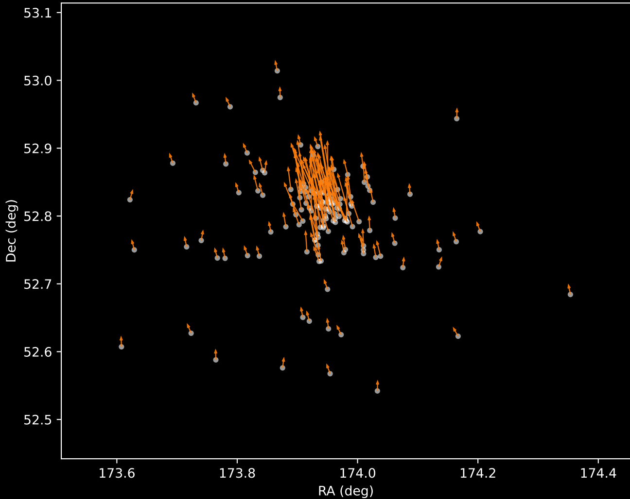
Gaia DR3 Cluster 2 Proper Motion Vectors (n=138)
