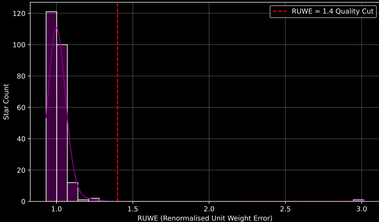
Gaia Cluster: [Berkeley_13] RUWE Distribution (n= 237)
