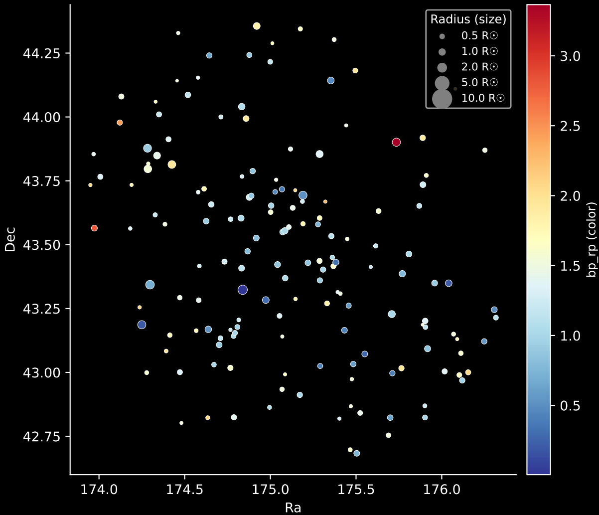
Gaia Cluster: [Berkeley_14A] Stars: 162
