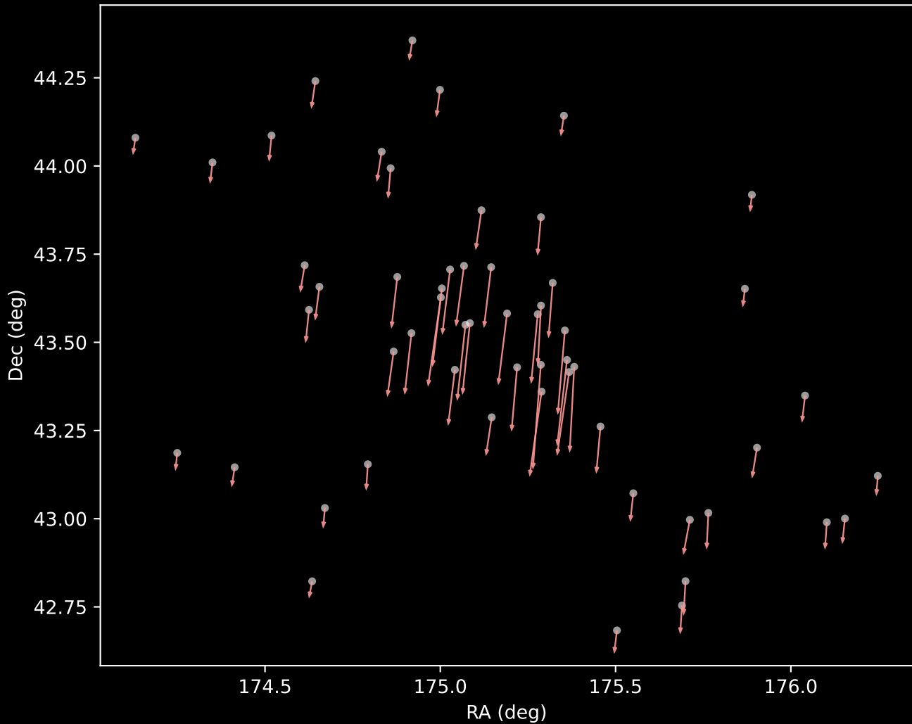
Gaia DR3 Cluster 7 Proper Motion Vectors (n=56)
