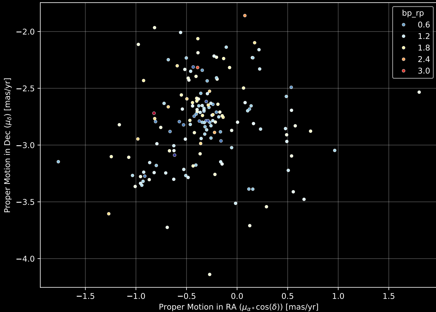
Gaia Cluster: [Berkeley_14A] Proper Motion Diagram (n= 162)
