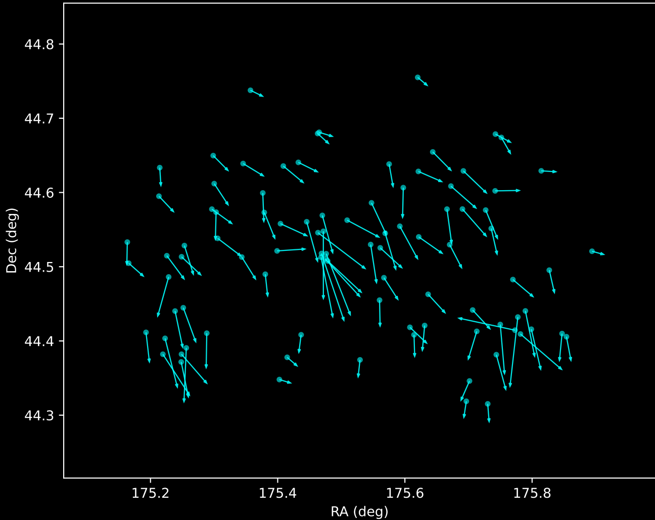
Gaia DR3 Noise Stream Proper Motion Vectors (n=93)
