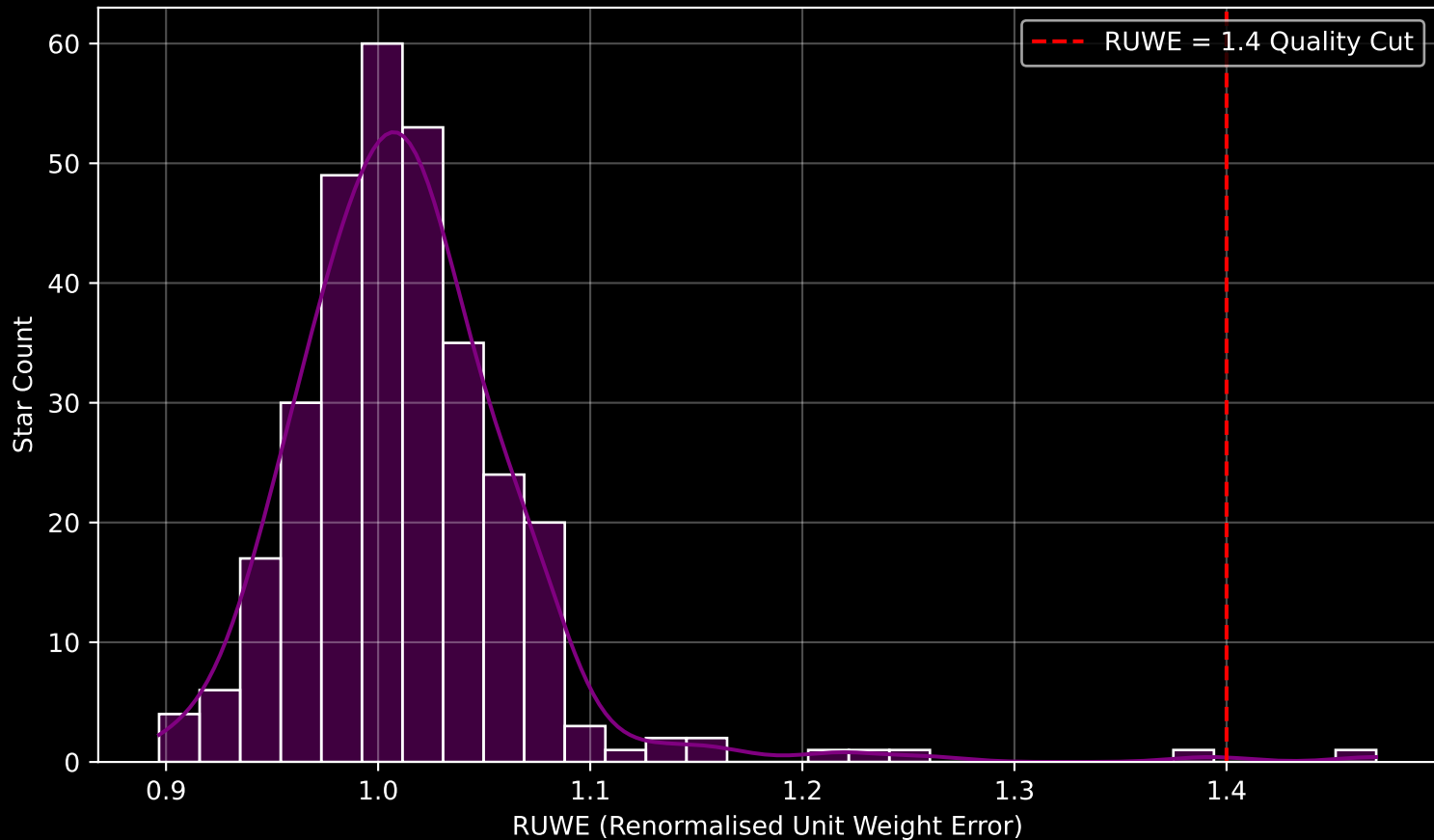
Gaia Cluster: [Berkeley_15] RUWE Distribution (n= 311)
