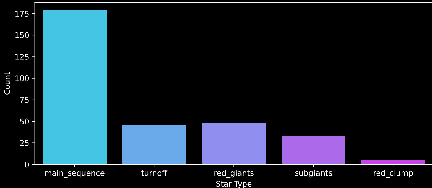
Gaia Cluster: [Berkeley_15] Count plot of Star Type
