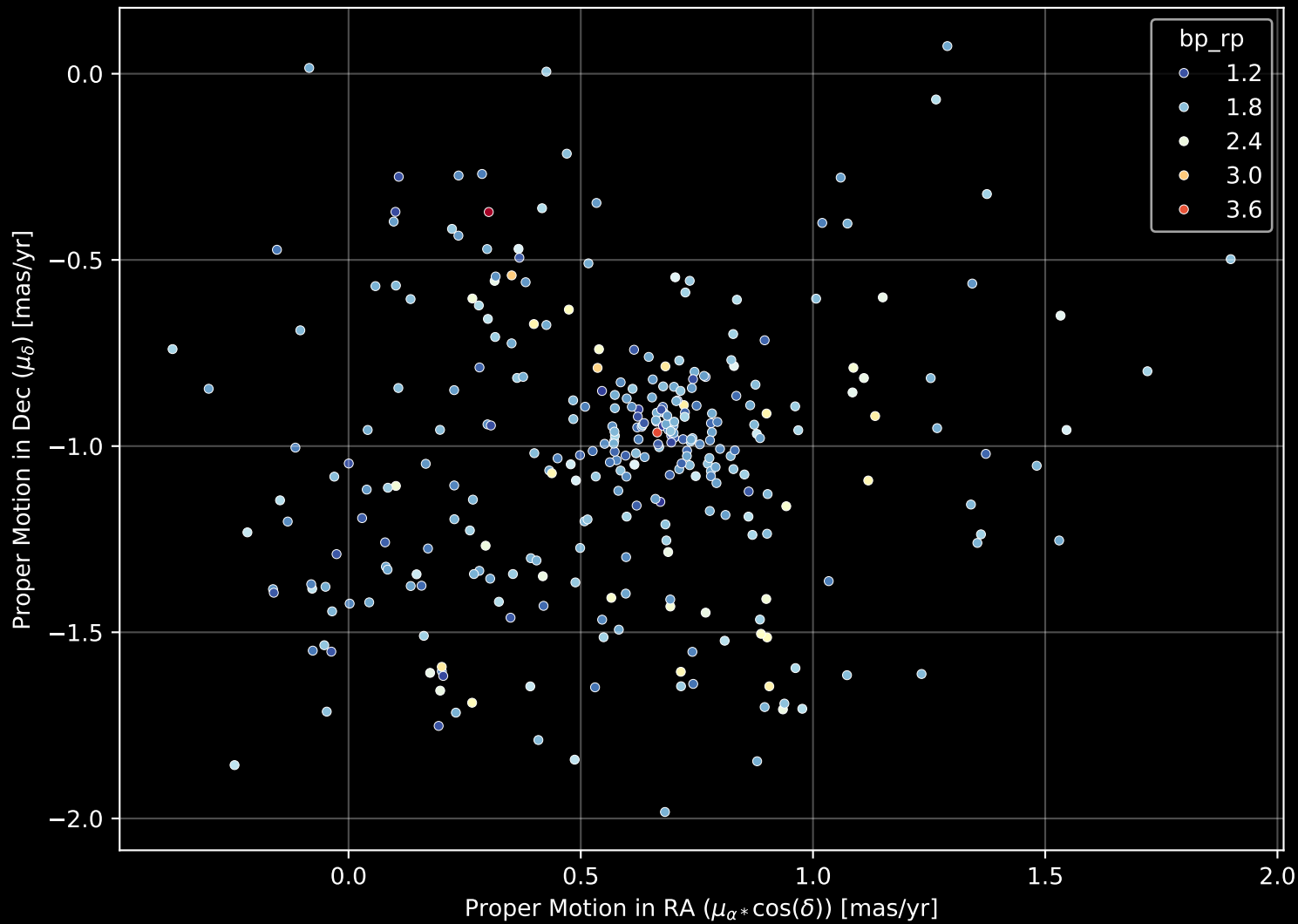
Gaia Cluster: [Berkeley_15] Proper Motion Diagram (n= 311)
