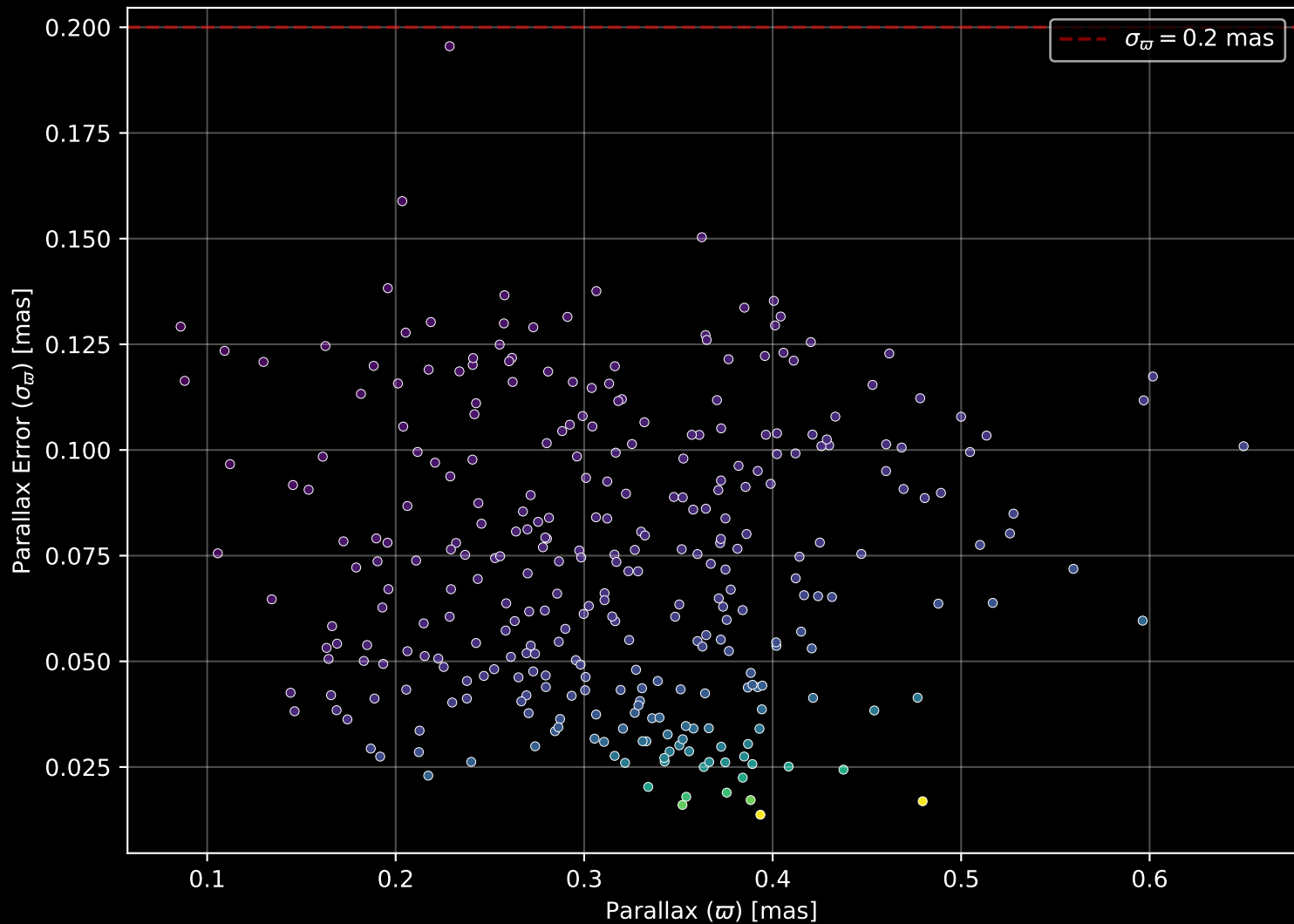
Gaia Cluster: [Berkeley_15] Parallax Quality (n= 311)
