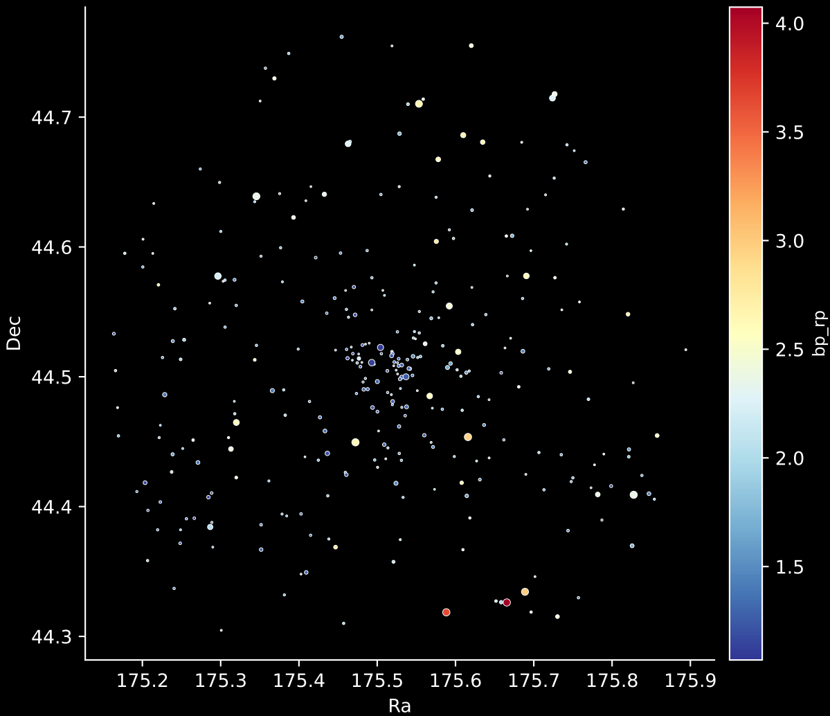
Gaia Cluster: [Berkeley_15] Stars: 311
