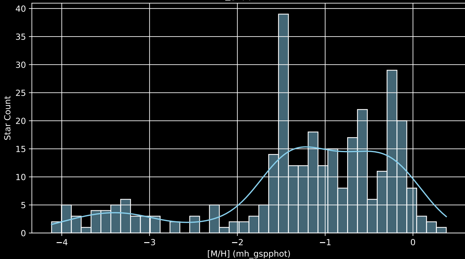
Gaia Cluster: [Berkeley_15 [M/H] (mh_gspphot) (n= 311)
