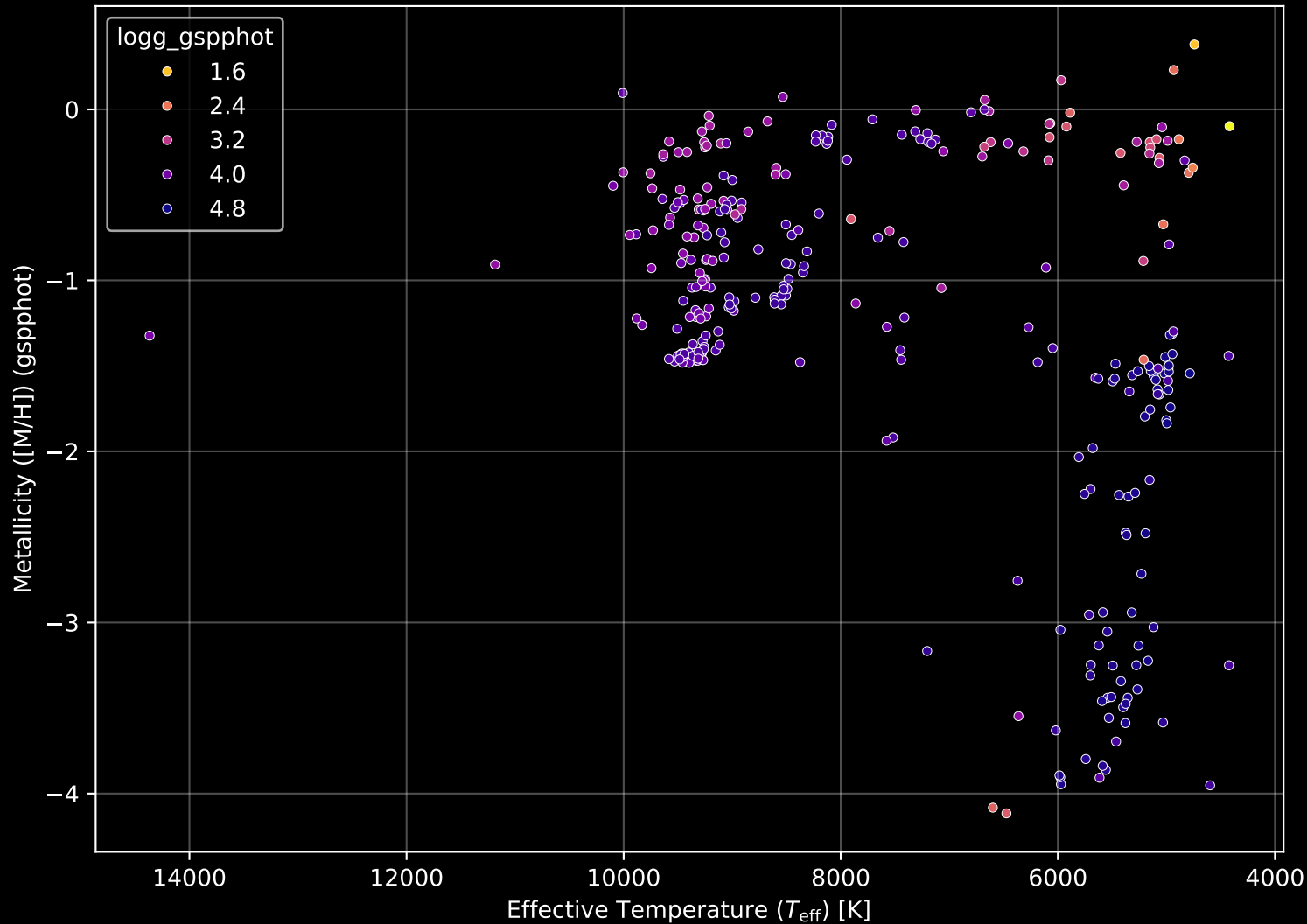
Gaia Cluster: [Berkeley_15] Stellar Population Parameters (n= 311)
