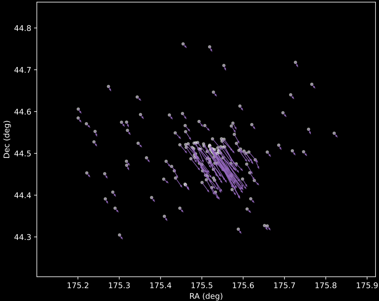
Gaia DR3 Cluster 8 Proper Motion Vectors (n=141)
