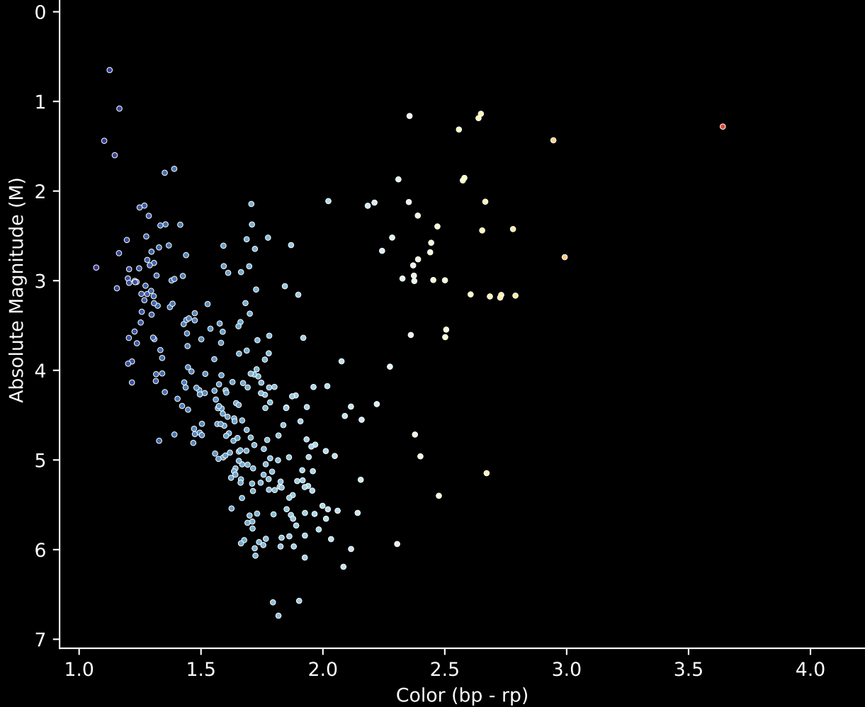
Gaia Cluster: [Berkeley_15] Stars (n= 311) Hertzsprung-Russel Diagram
