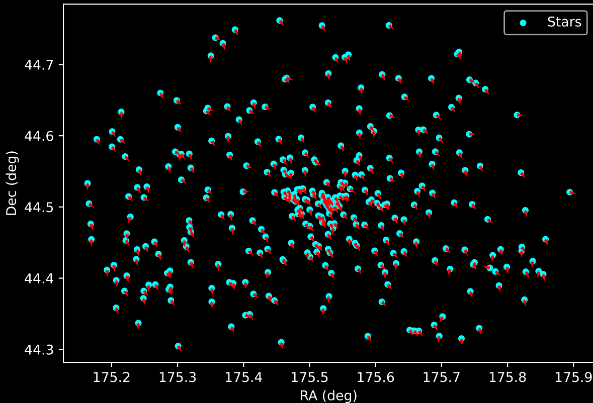
Gaia Cluster: [Berkeley_15] Proper Motion Vectors for Gaia Star Field (n= 311)
