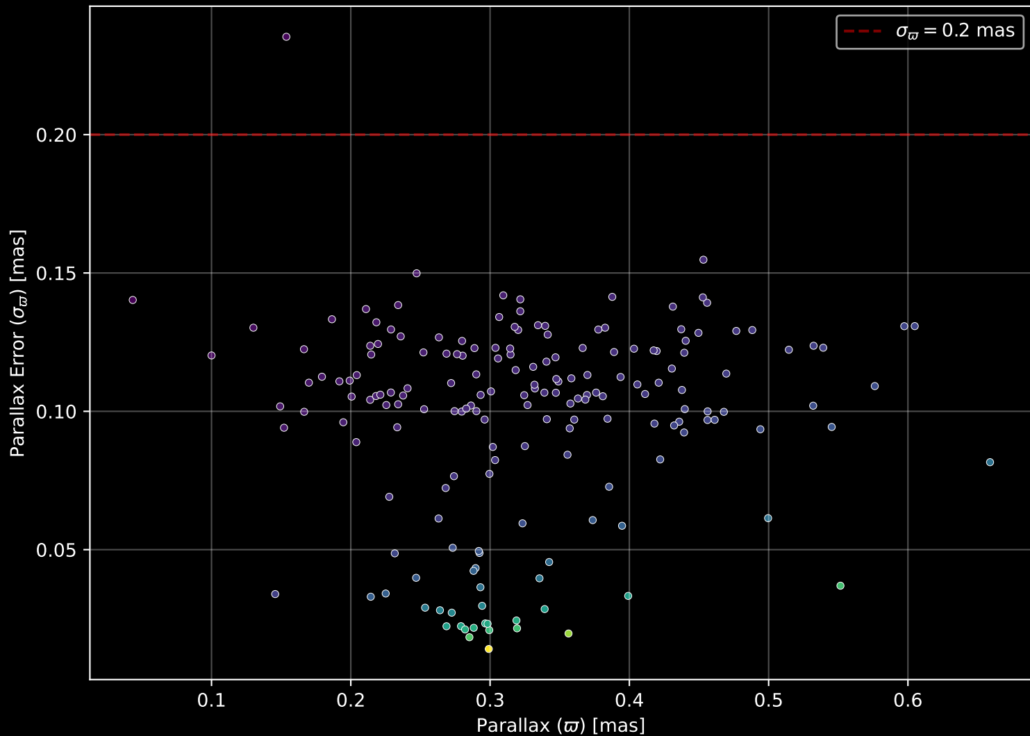
Gaia Cluster: [Berkeley_17] Parallax Quality (n= 181)
