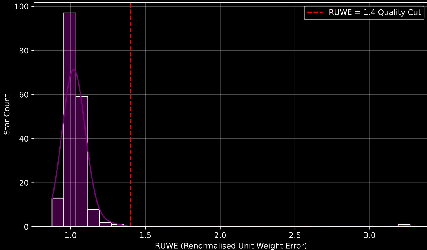
Gaia Cluster: [Berkeley_17] RUWE Distribution (n= 181)
