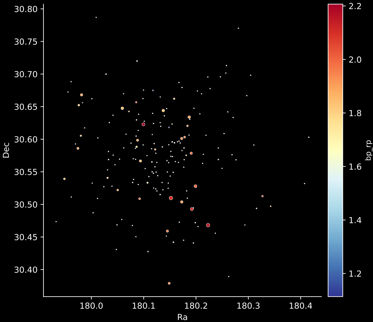
Gaia Cluster: [Berkeley_17] Stars: 181
