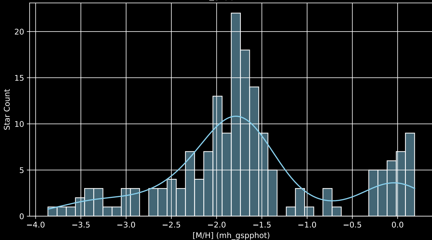
Gaia Cluster: [Berkeley_17 [M/H] (mh_gspphot) (n= 181)
