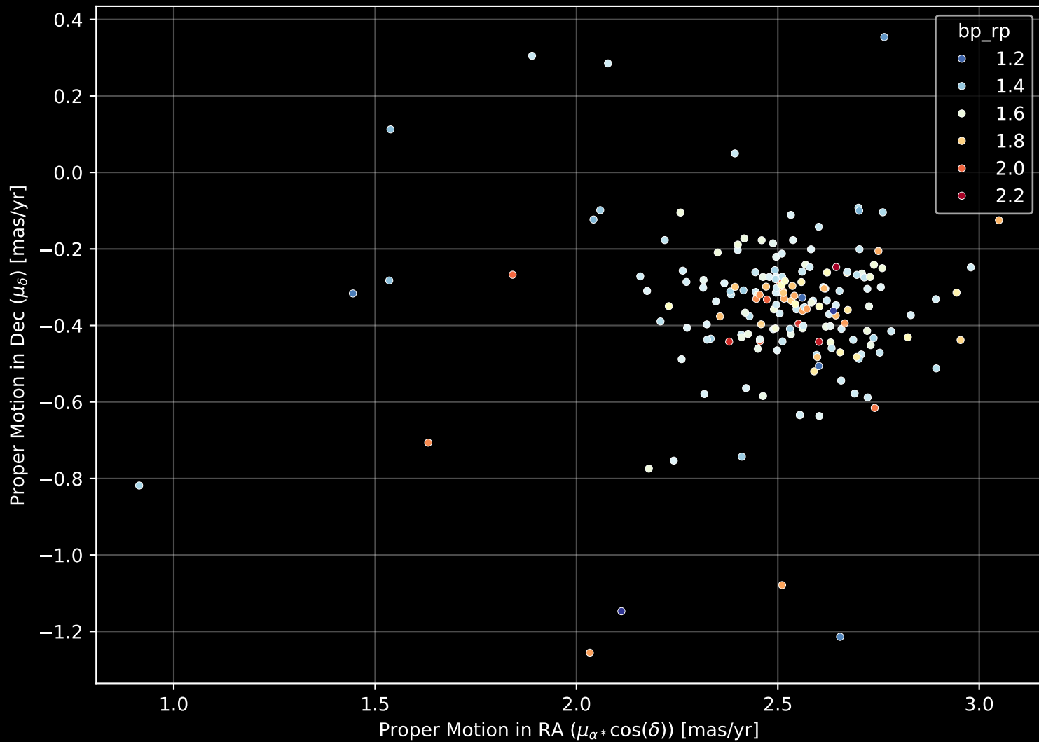
Gaia Cluster: [Berkeley_17] Proper Motion Diagram (n= 181)
