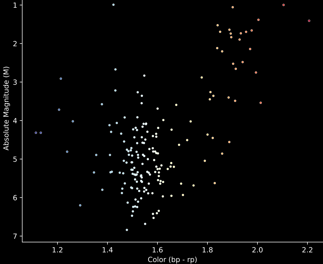
Gaia Cluster: [Berkeley_17] Stars (n= 181) Hertzsprung-Russel Diagram
