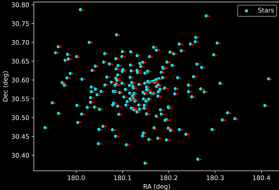
Gaia Cluster: [Berkeley_17] Proper Motion Vectors for Gaia Star Field (n= 181)
