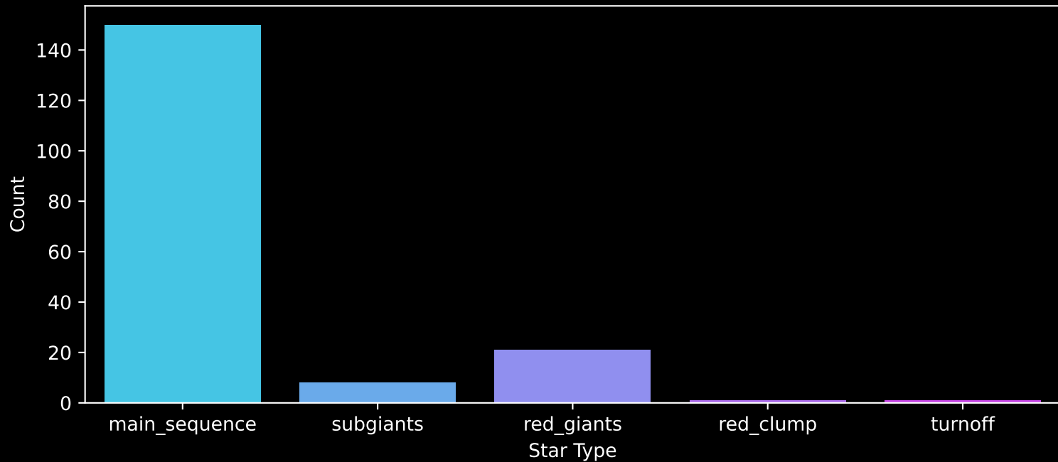
Gaia Cluster: [Berkeley_17] Count plot of Star Type
