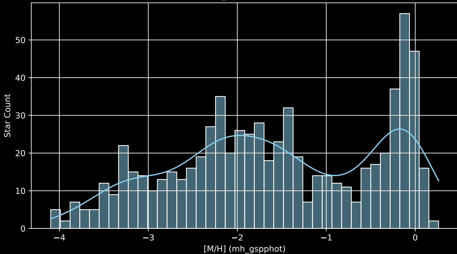
Gaia Cluster: [Berkeley_18 [M/H] (mh_gspphot) (n= 712)
