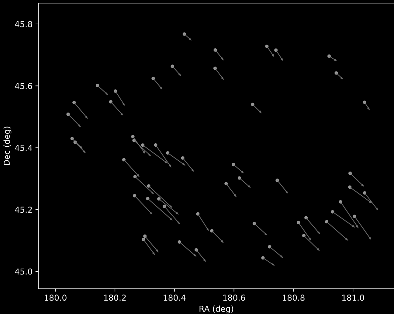
Gaia DR3 Cluster 14 Proper Motion Vectors (n=54)
