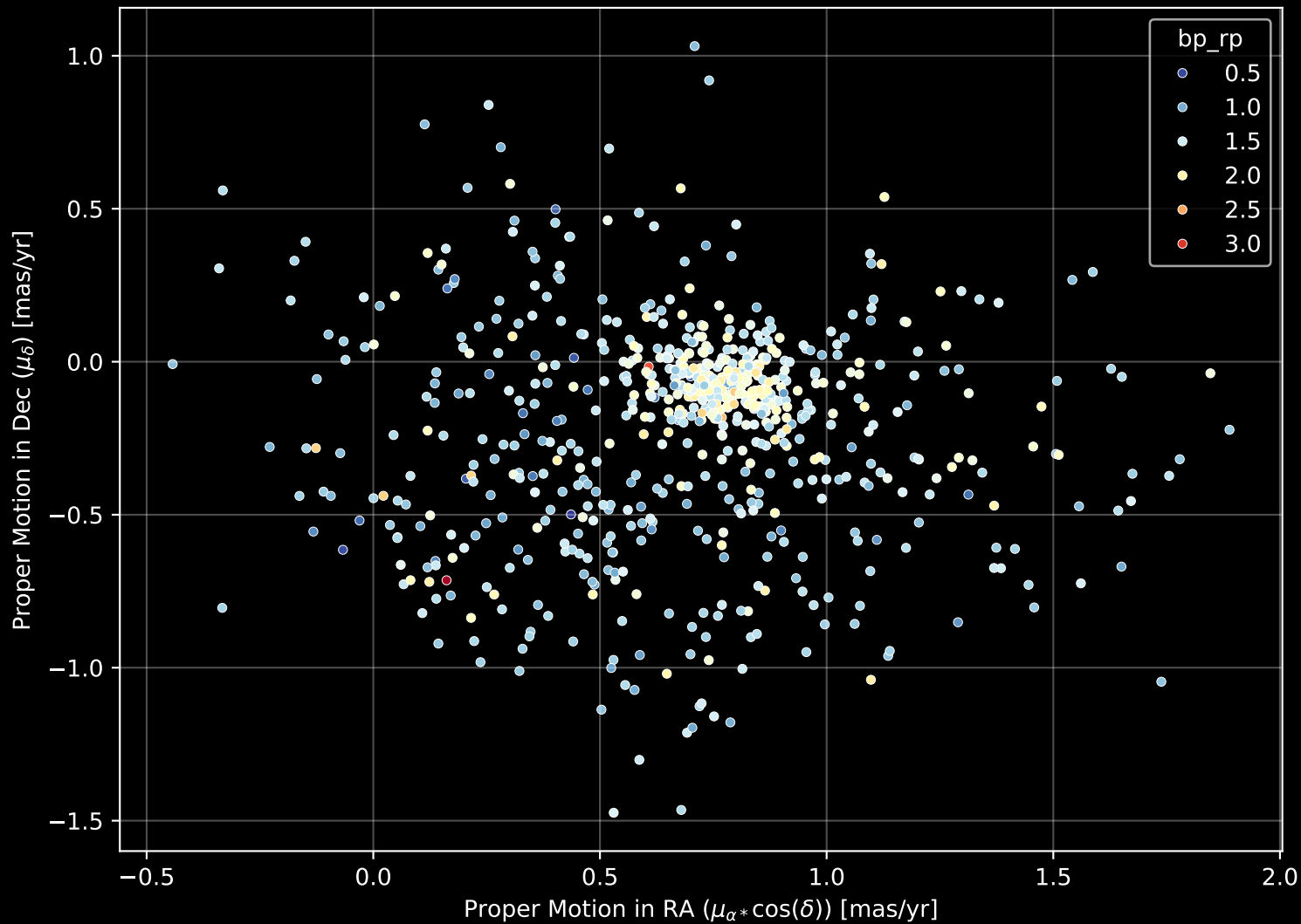
Gaia Cluster: [Berkeley_18] Proper Motion Diagram (n= 712)
