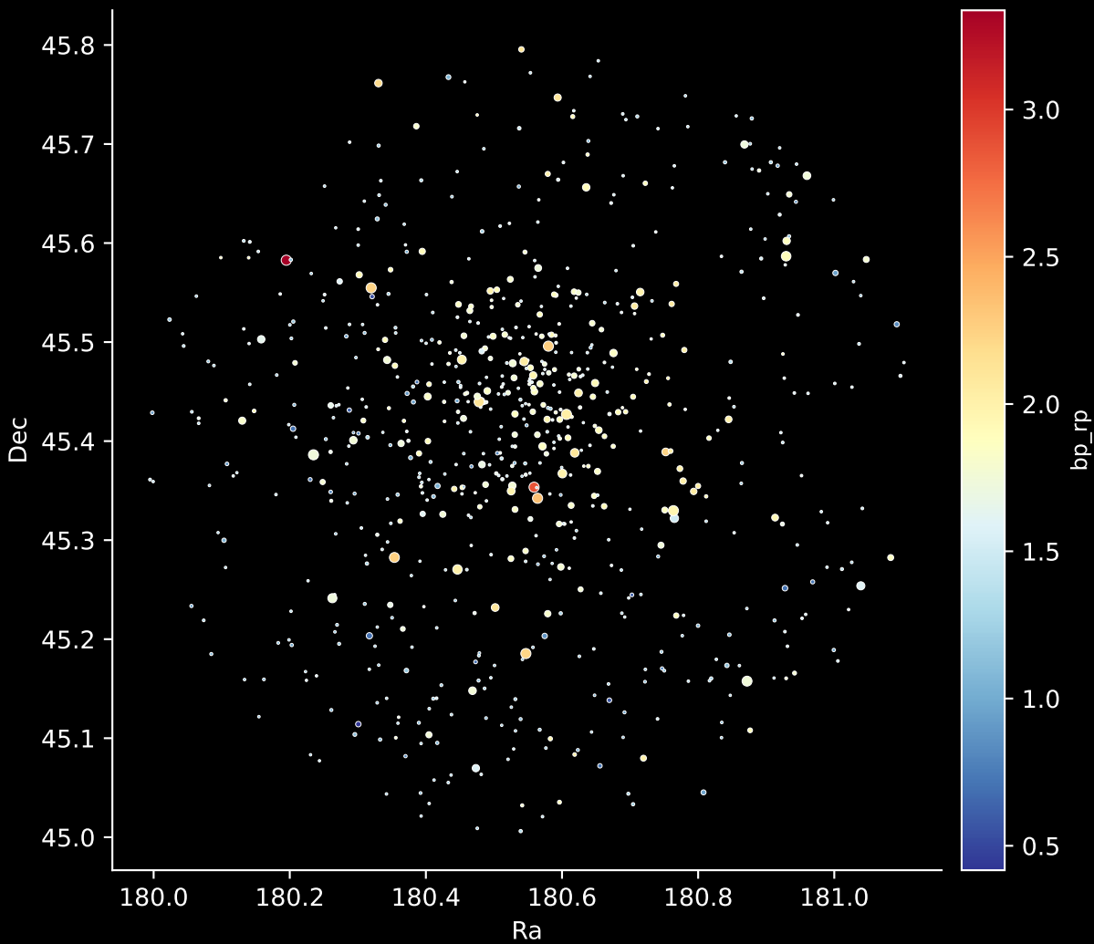
Gaia Cluster: [Berkeley_18] Stars: 712
