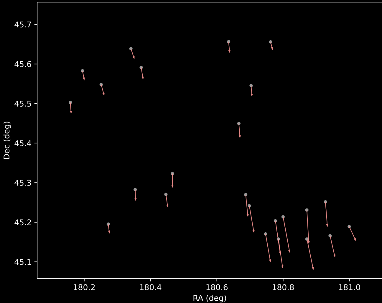
Gaia DR3 Cluster 7 Proper Motion Vectors (n=24)
