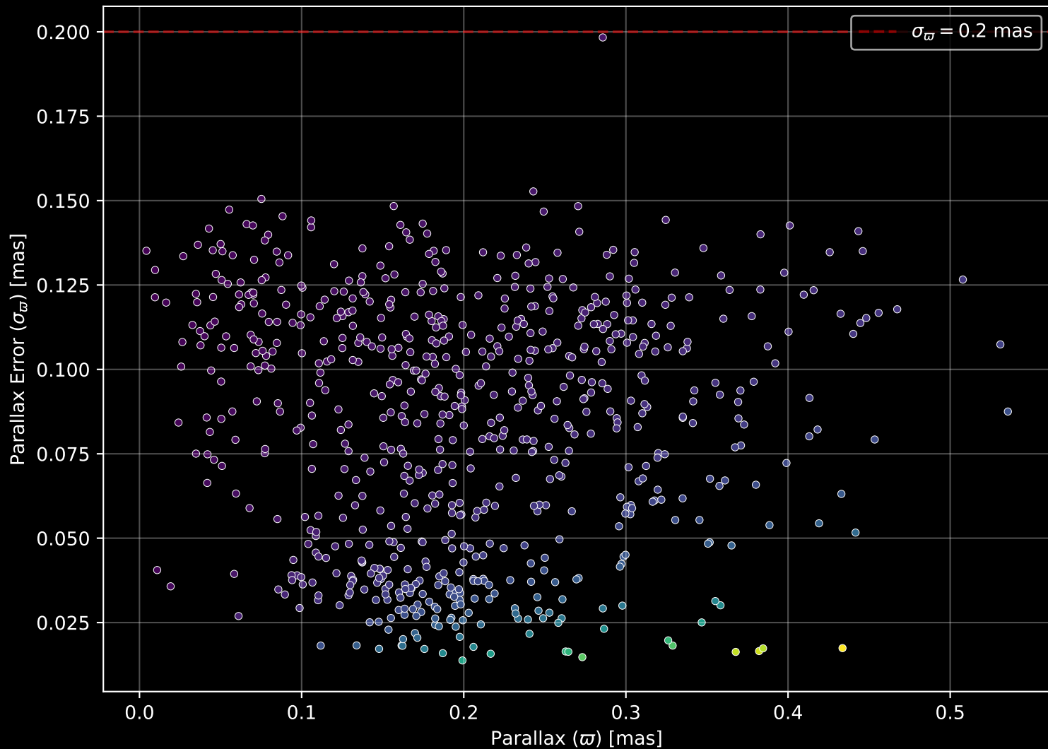
Gaia Cluster: [Berkeley_18] Parallax Quality (n= 712)
