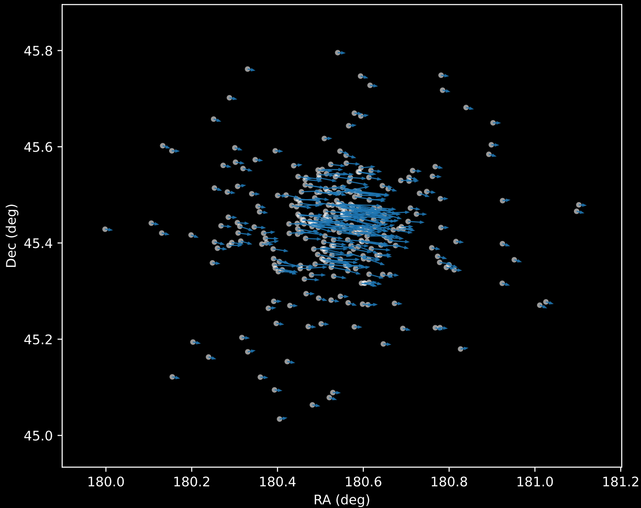
Gaia DR3 Cluster 20 Proper Motion Vectors (n=303)
