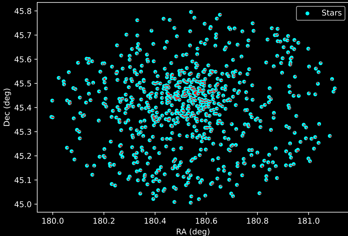
Gaia Cluster: [Berkeley_18] Proper Motion Vectors for Gaia Star Field (n= 712)
