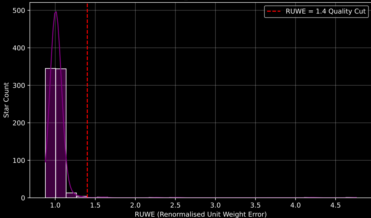
Gaia Cluster: [Berkeley_18] RUWE Distribution (n= 712)
