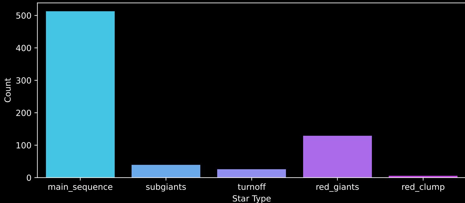
Gaia Cluster: [Berkeley_18] Count plot of Star Type
