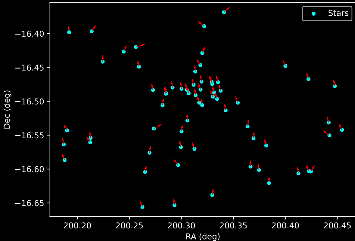
Gaia Cluster: [Berkeley_25] Proper Motion Vectors for Gaia Star Field (n= 65)
