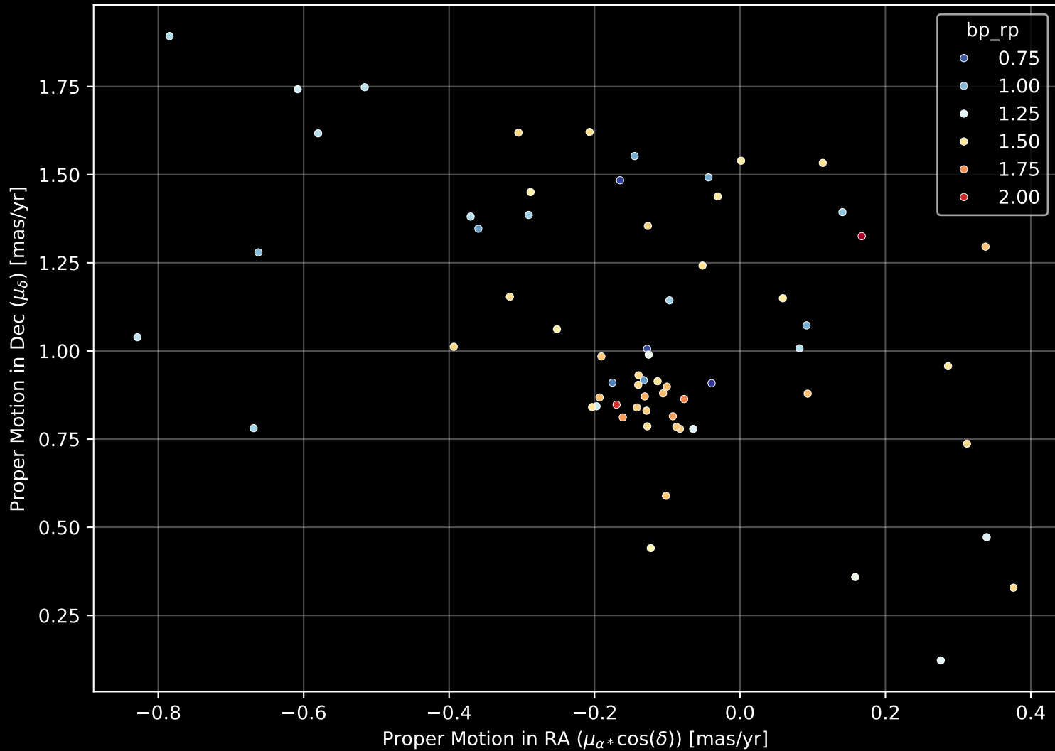
Gaia Cluster: [Berkeley_25] Proper Motion Diagram (n= 65)
