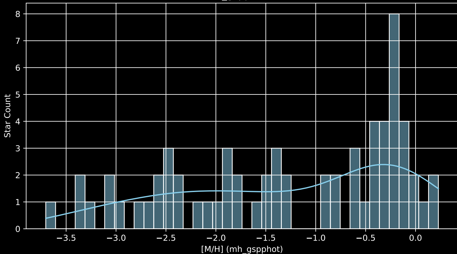
Gaia Cluster: [Berkeley_25 [M/H] (mh_gspphot) (n= 65)
