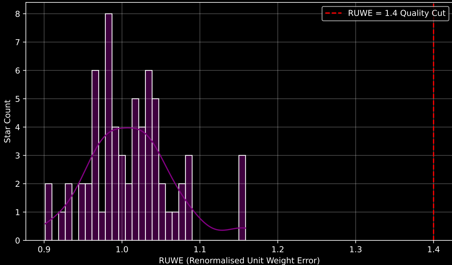
Gaia Cluster: [Berkeley_25] RUWE Distribution (n= 65)
