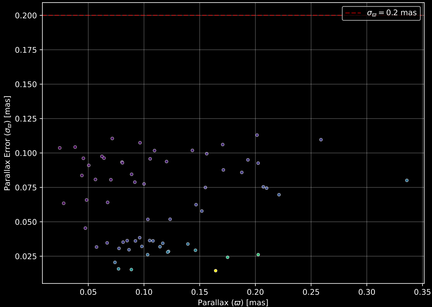
Gaia Cluster: [Berkeley_25] Parallax Quality (n= 65)
