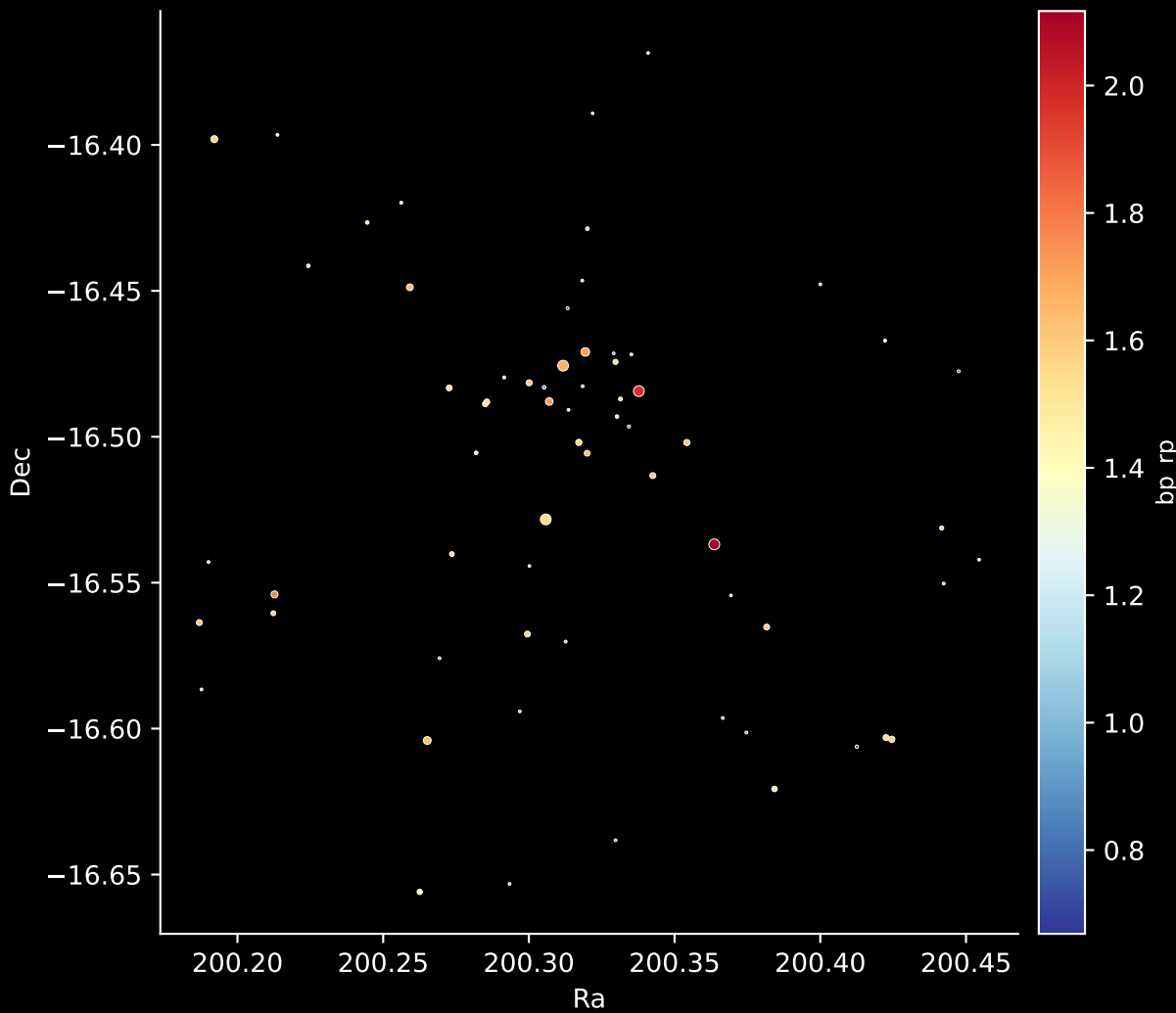
Gaia Cluster: [Berkeley_25] Stars: 65
