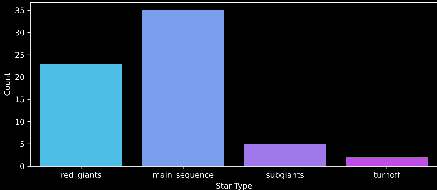
Gaia Cluster: [Berkeley_25] Count plot of Star Type
