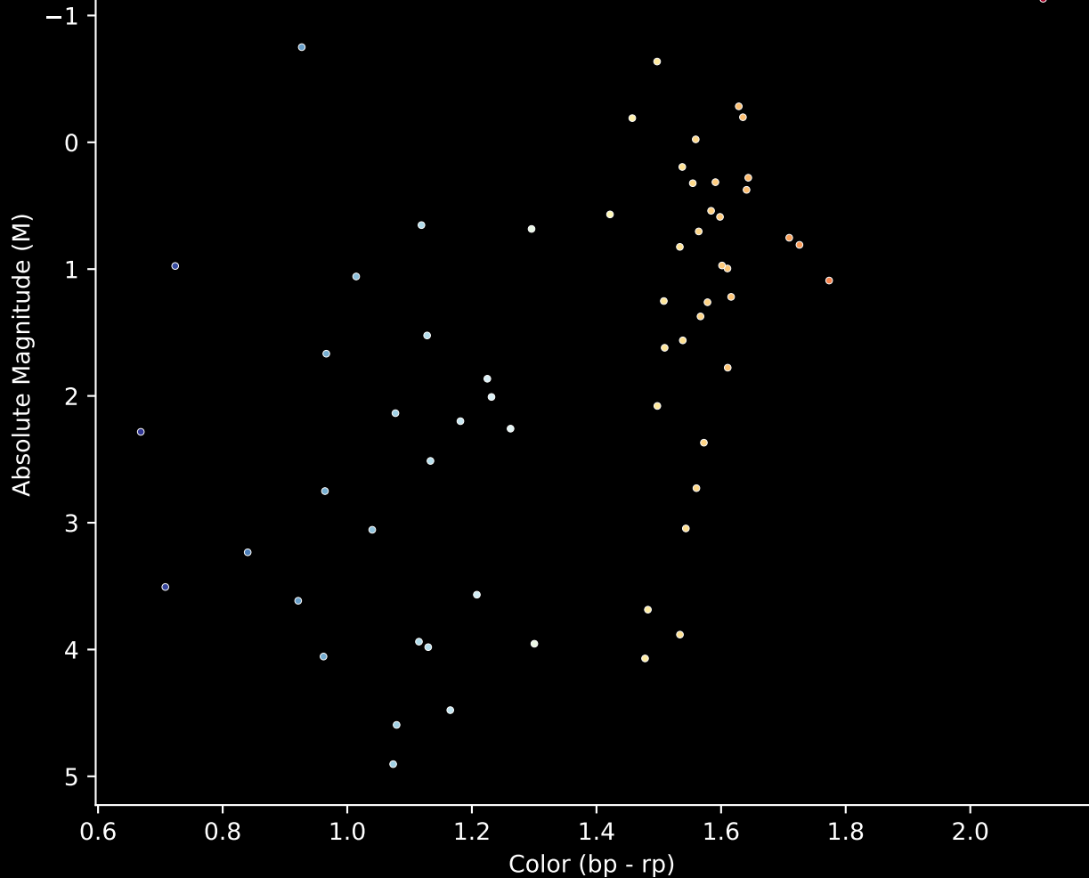
Gaia Cluster: [Berkeley_25] Stars (n= 65) Hertzsprung-Russell Diagram
