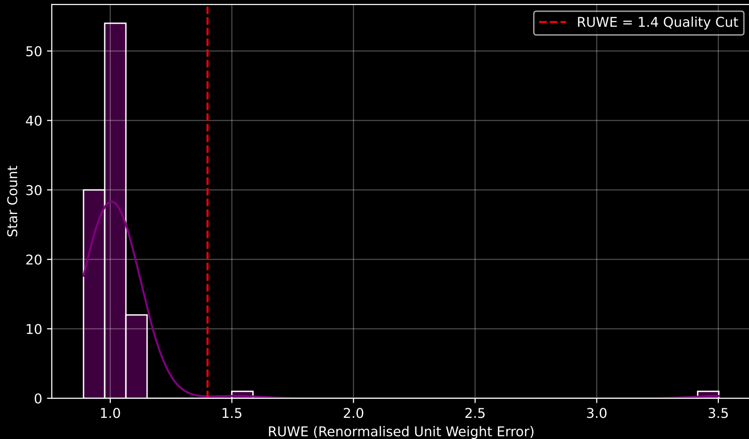
Gaia Cluster: [Berkeley_27] RUWE Distribution (n= 98)
