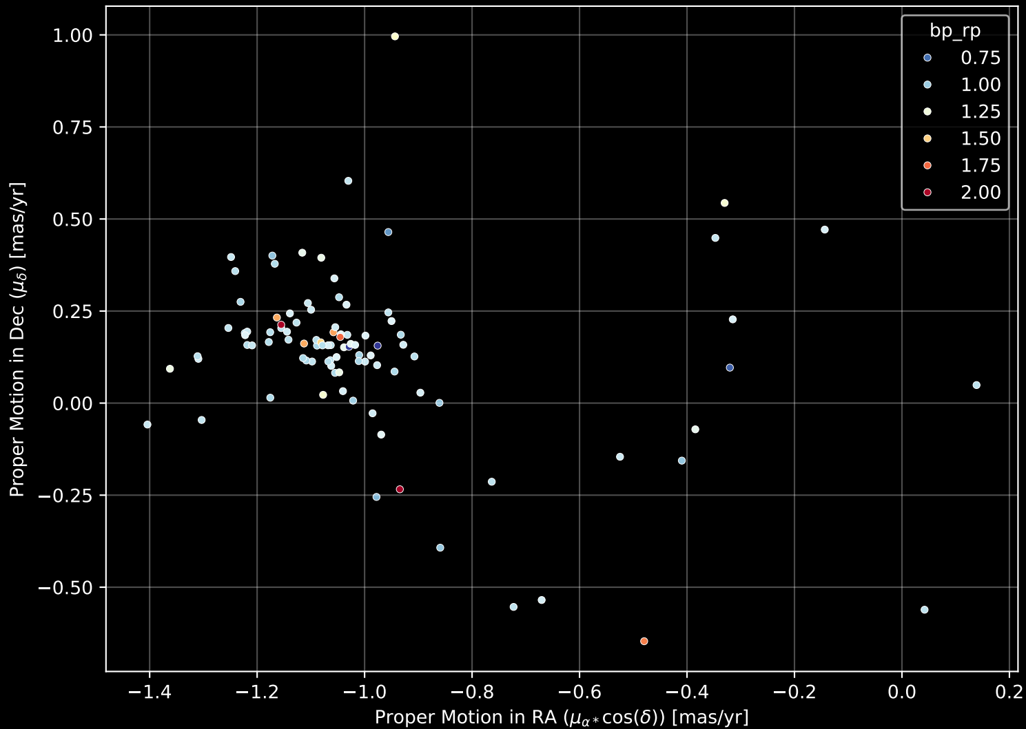
Gaia Cluster: [Berkeley_27] Proper Motion Diagram (n= 98)
