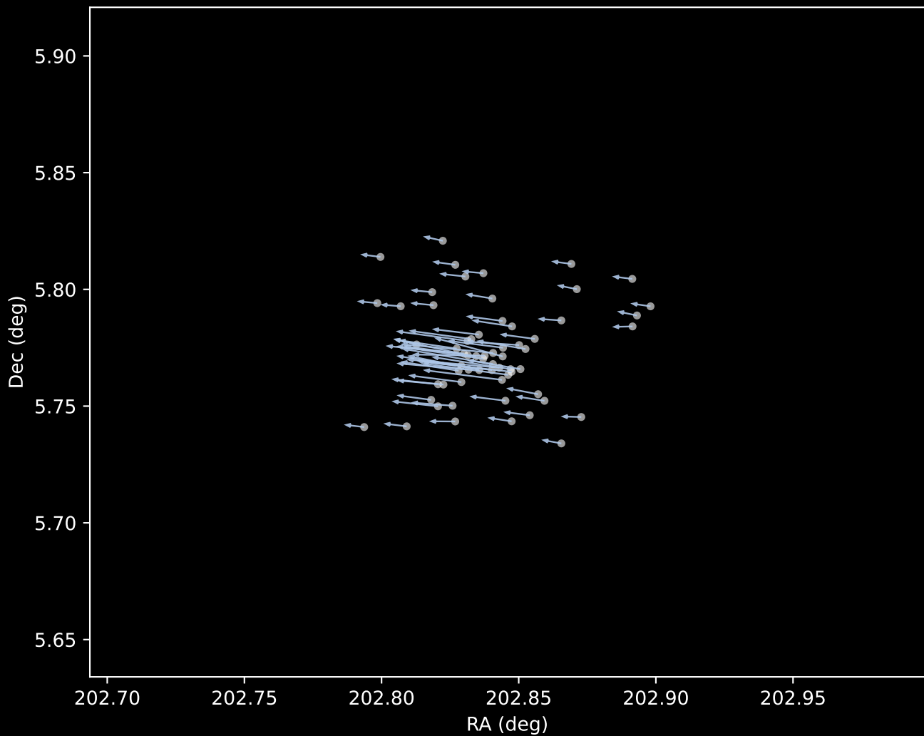
Gaia DR3 Cluster 1 Proper Motion Vectors (n=63)
