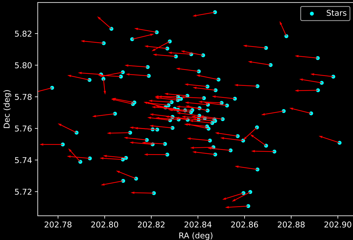
Gaia Cluster: [Berkeley_27] Proper Motion Vectors for Gaia Star Field (n= 98)
