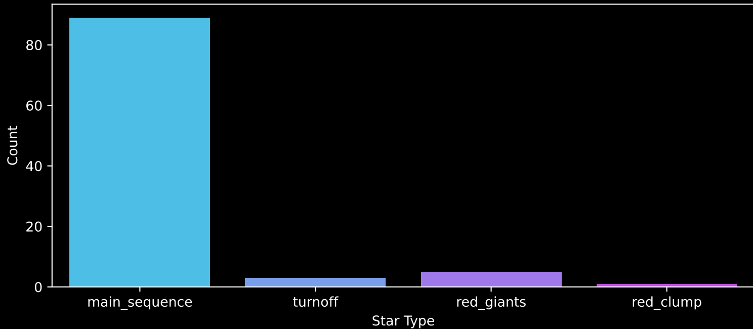
Gaia Cluster: [Berkeley_27] Count plot of Star Type
