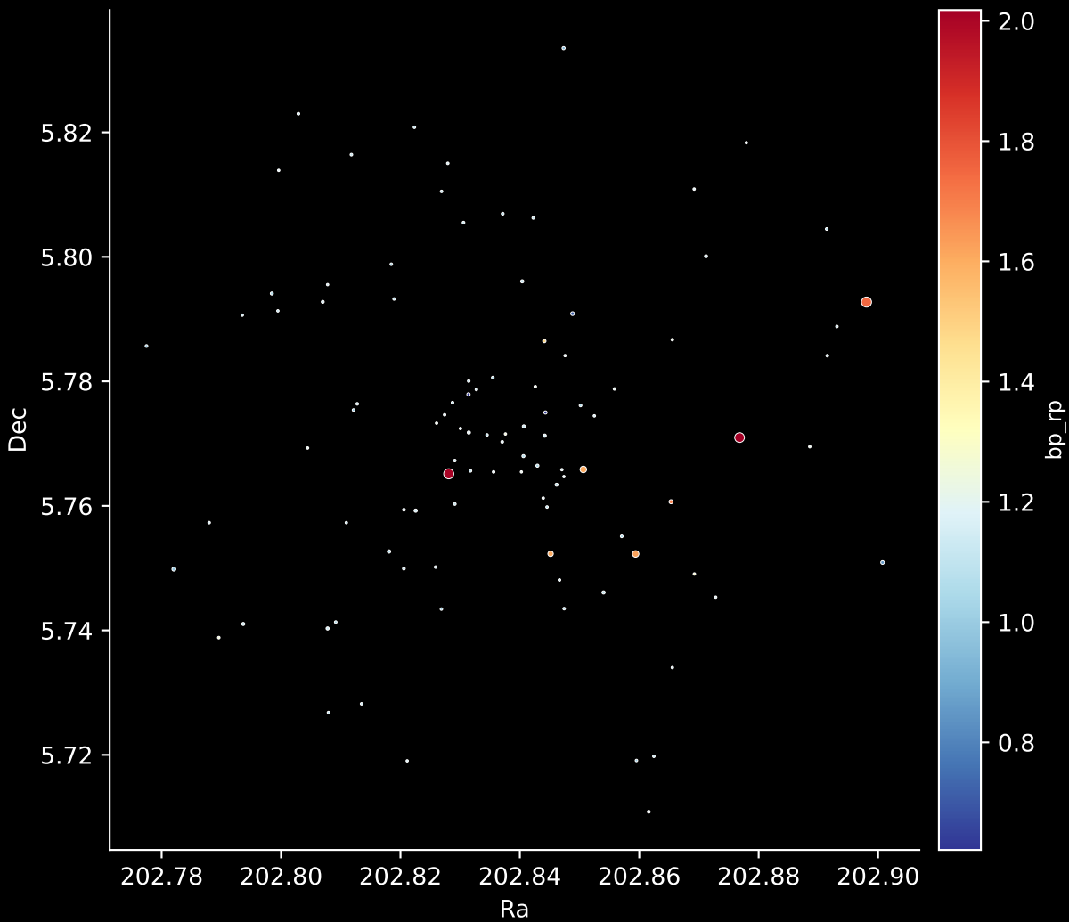
Gaia Cluster: [Berkeley_27] Stars: 98
