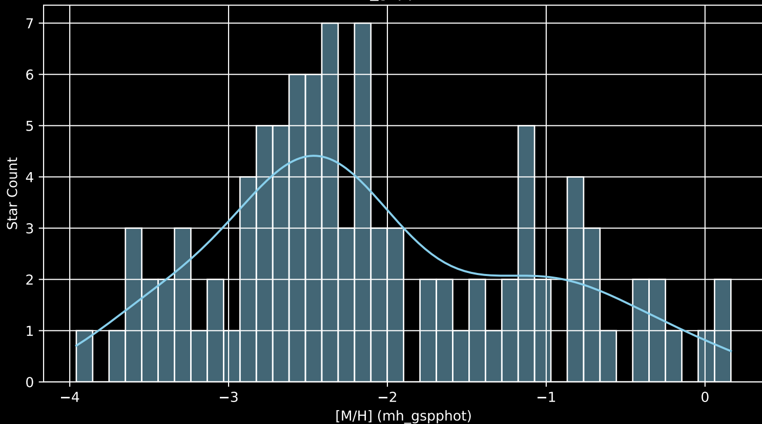
Gaia Cluster: [Berkeley_27 [M/H] (mh_gspphot) (n= 98)
