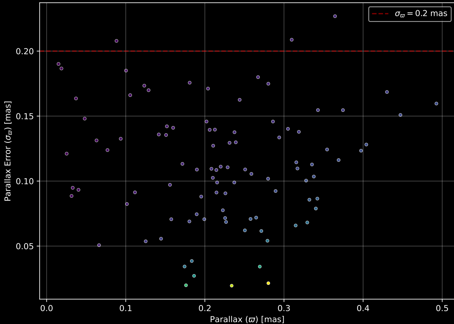
Gaia Cluster: [Berkeley_27] Parallax Quality (n= 98)
