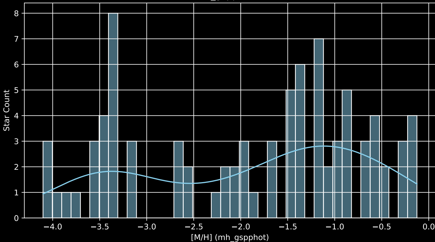
Gaia Cluster: [Berkeley_28 [M/H] (mh_gspphot) (n= 85)
