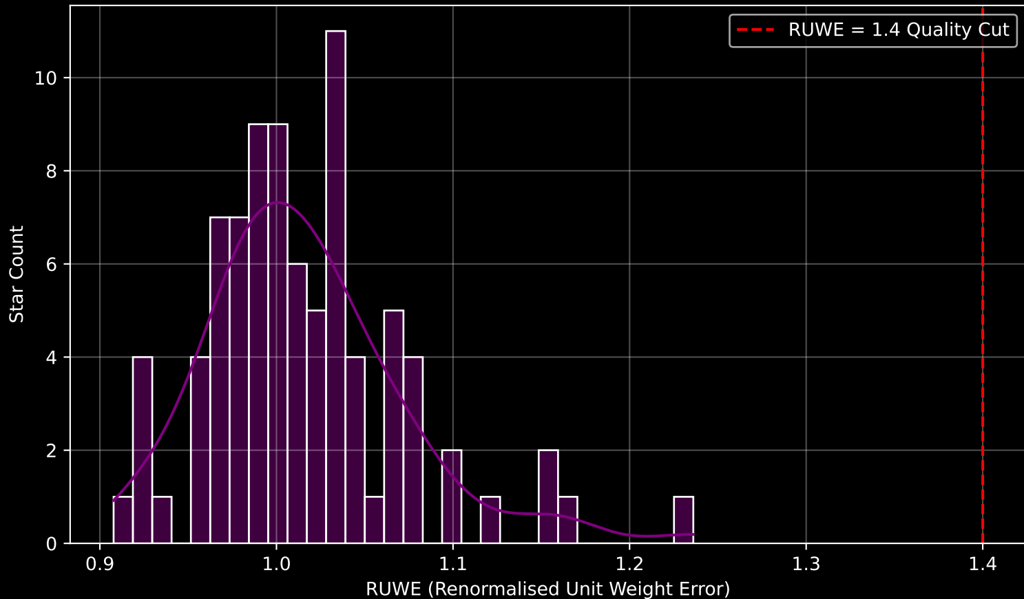
Gaia Cluster: [Berkeley_28] RUWE Distribution (n= 85)
