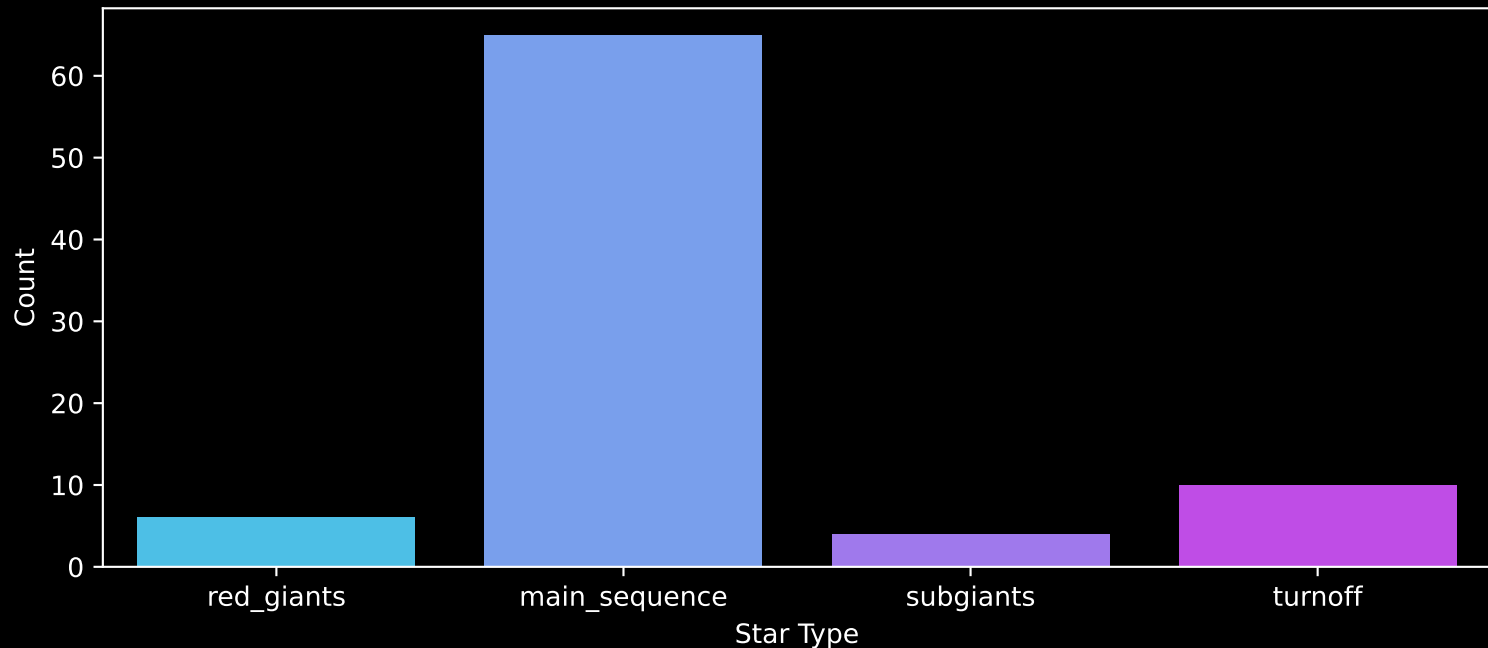
Gaia Cluster: [Berkeley_28] Count plot of Star Type
