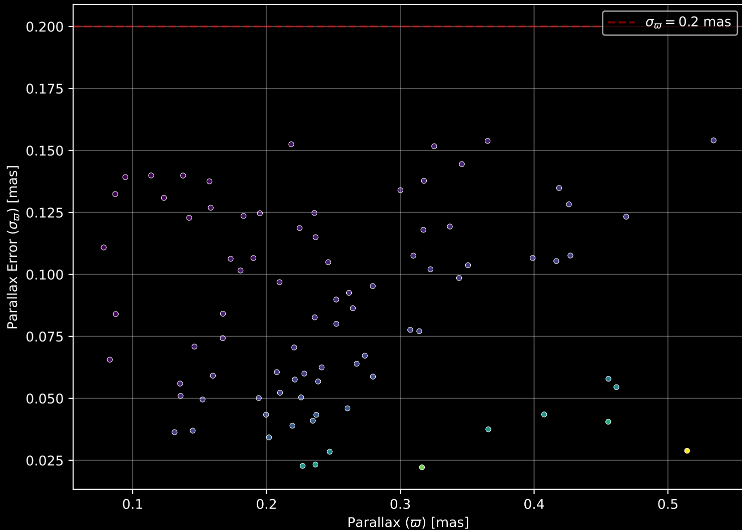
Gaia Cluster: [Berkeley_28] Parallax Quality (n= 85)
