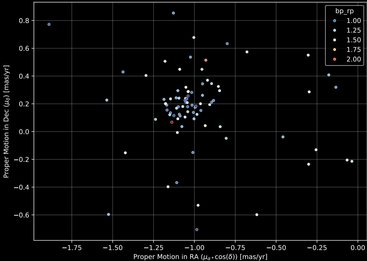
Gaia Cluster: [Berkeley_28] Proper Motion Diagram (n= 85)
