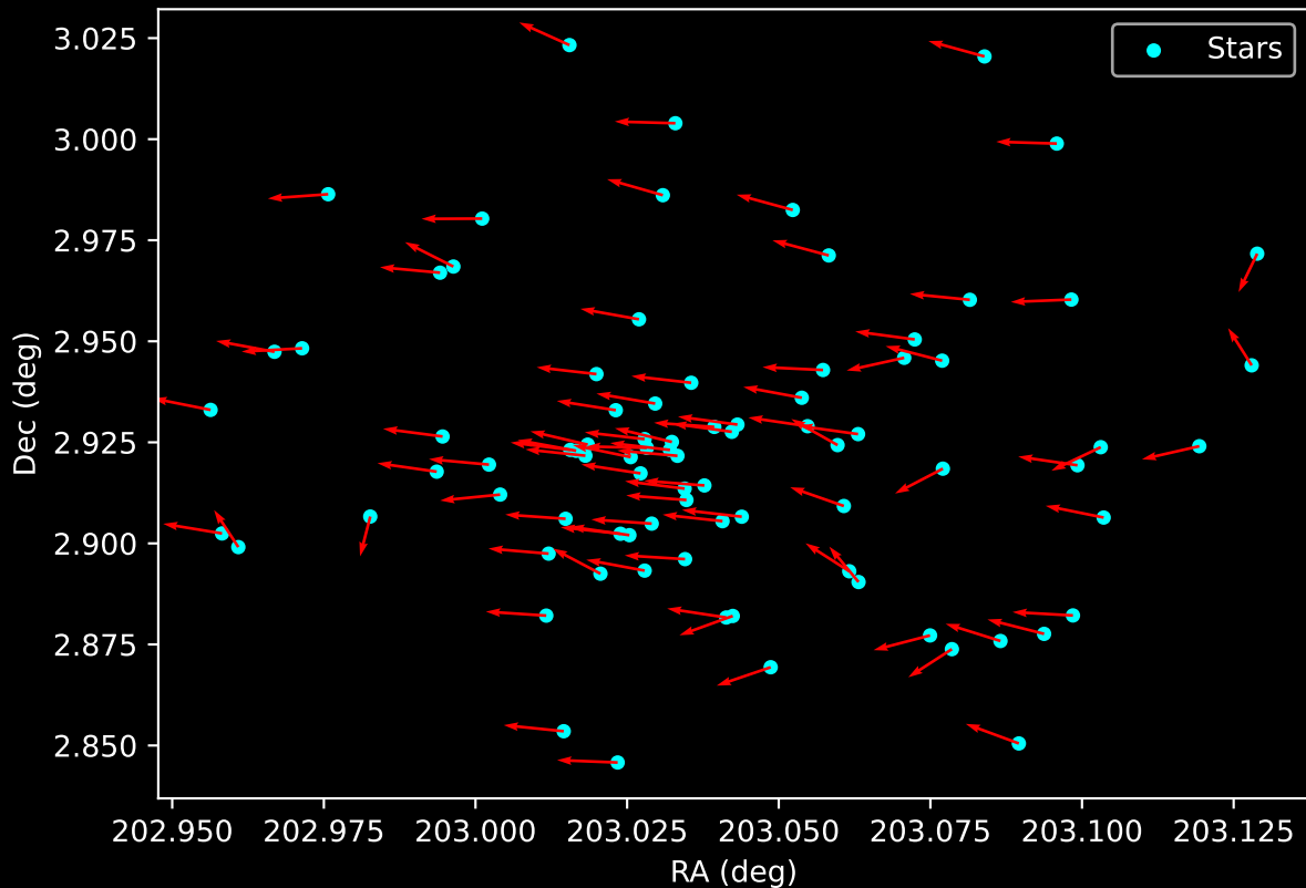
Gaia Cluster: [Berkeley_28] Proper Motion Vectors for Gaia Star Field (n= 85)
