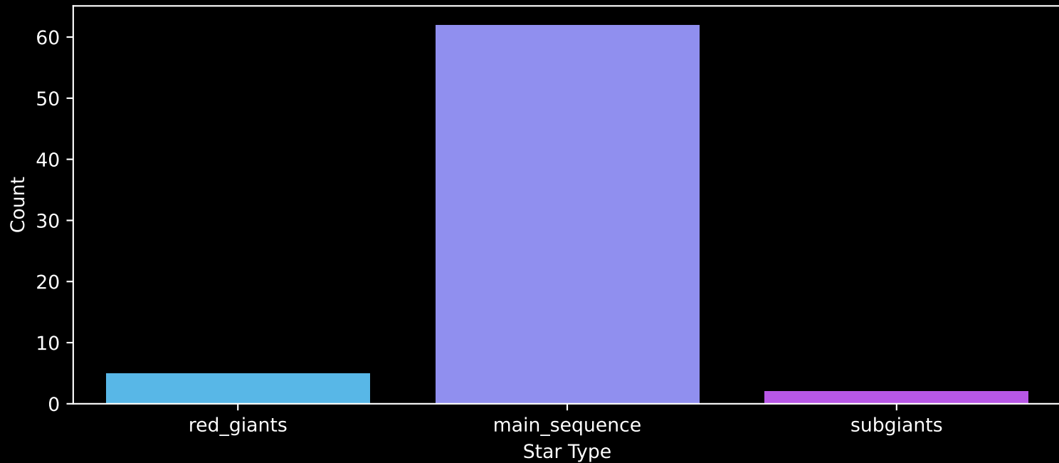
Gaia Cluster: [Berkeley_29] Count plot of Star Type
