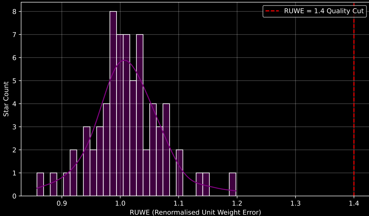
Gaia Cluster: [Berkeley_29] RUWE Distribution (n= 69)
