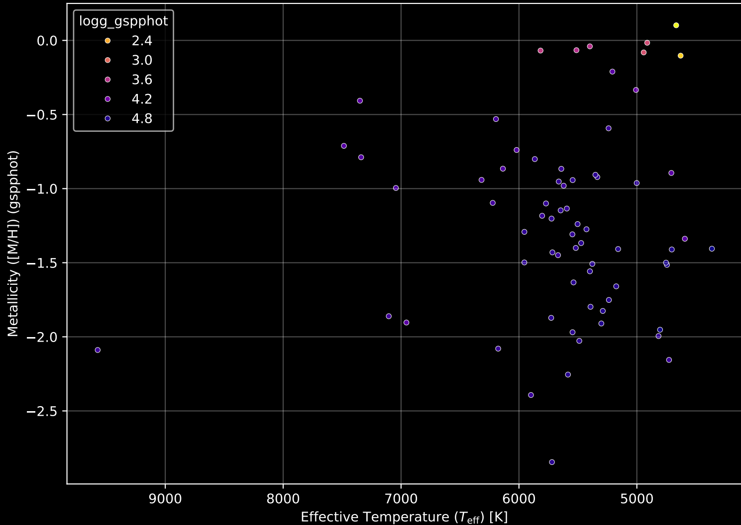
Gaia Cluster: [Berkeley_29] Stellar Population Parameters (n= 69)
