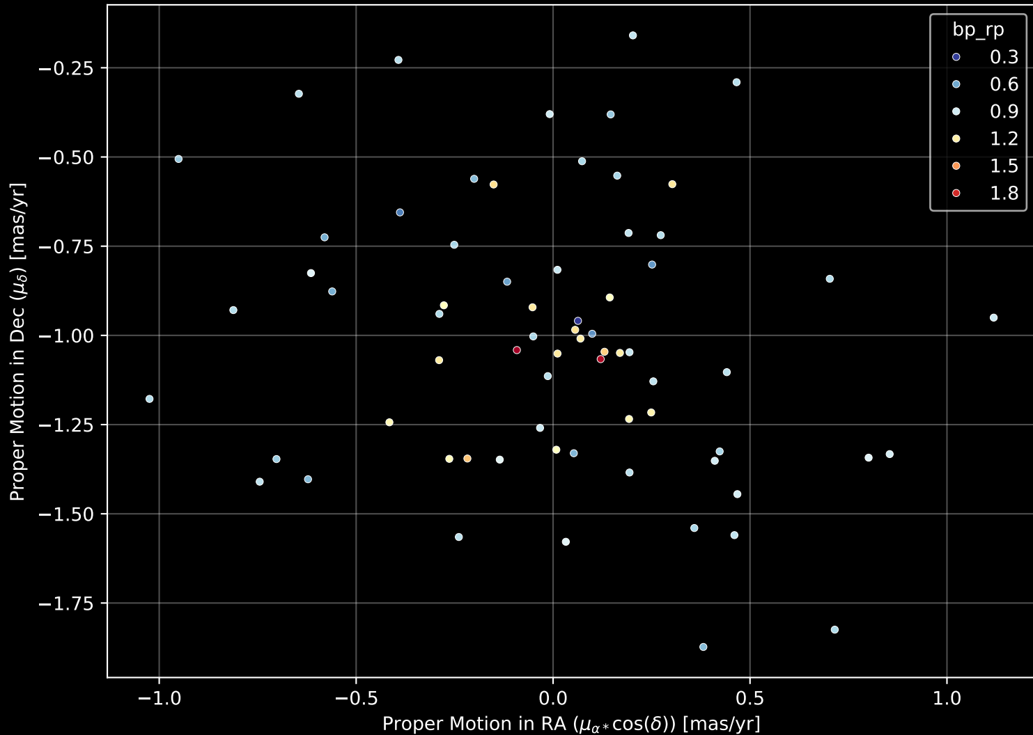
Gaia Cluster: [Berkeley_29] Proper Motion Diagram (n= 69)
