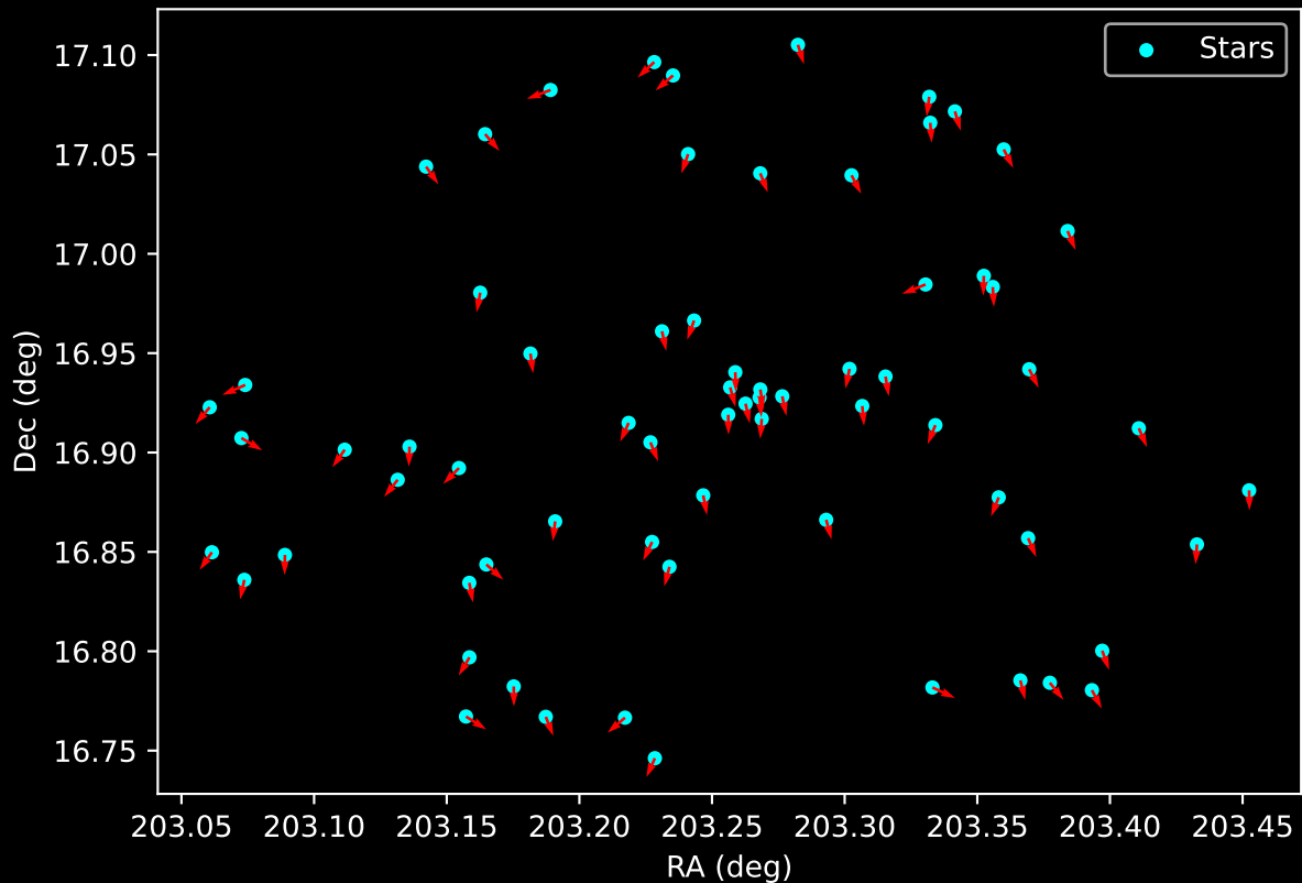
Gaia Cluster: [Berkeley_29] Proper Motion Vectors for Gaia Star Field (n= 69)
