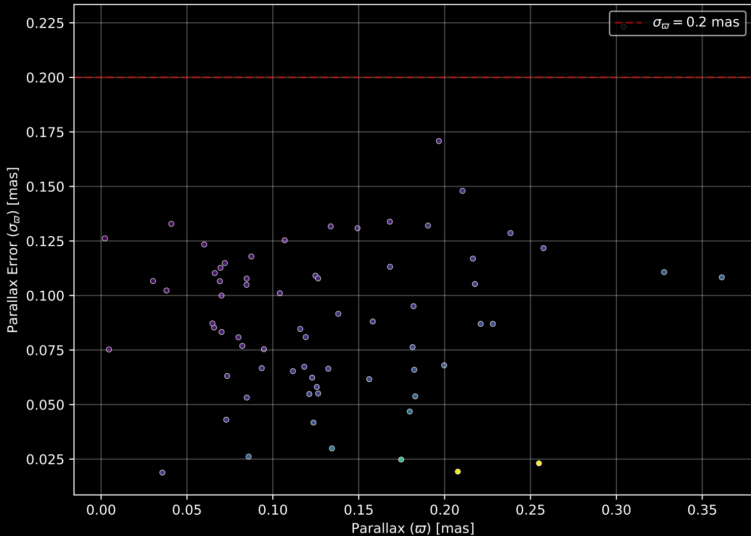
Gaia Cluster: [Berkeley_29] Parallax Quality (n= 69)
