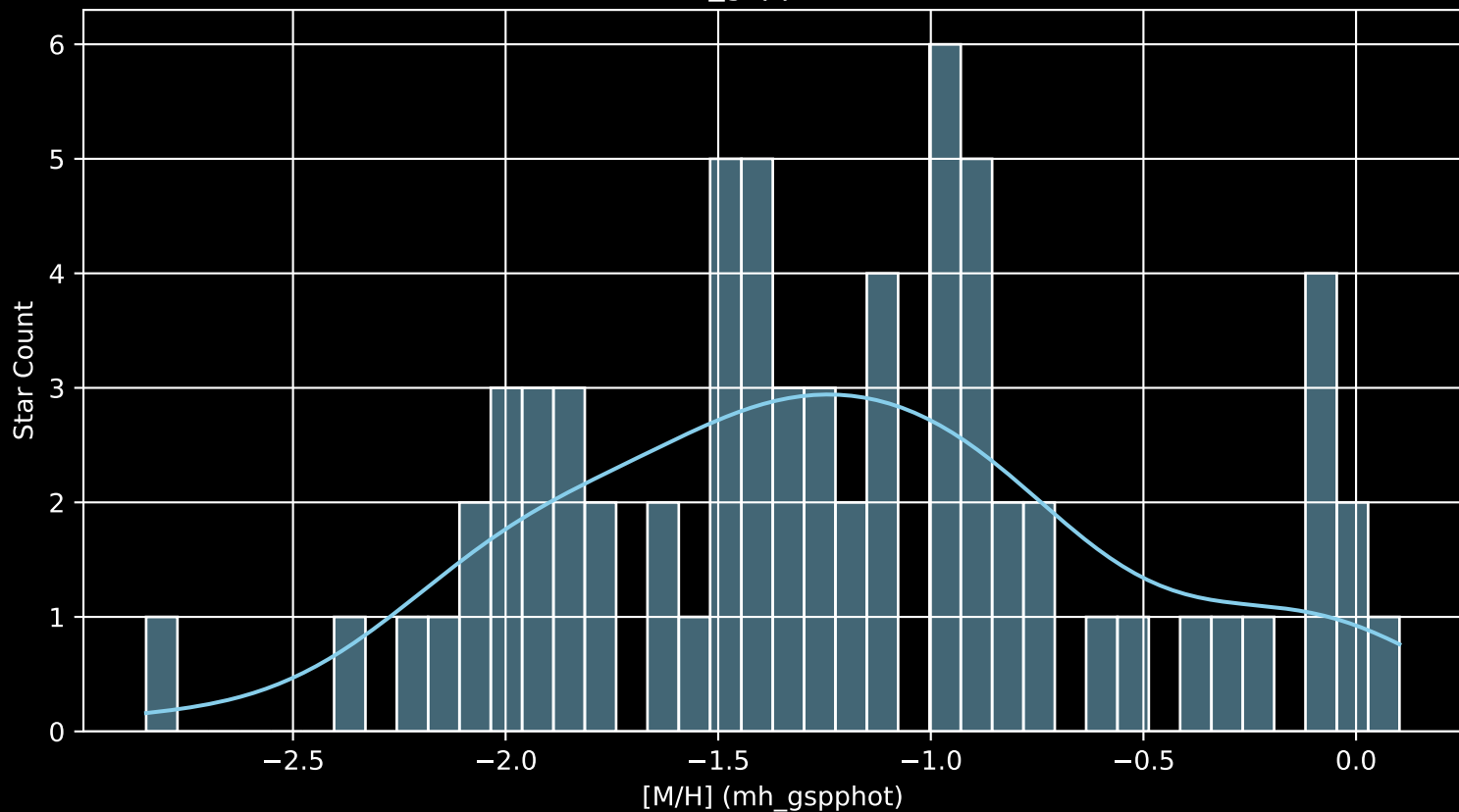
Gaia Cluster: [Berkeley_29 [M/H] (mh_gspphot) (n= 69)
