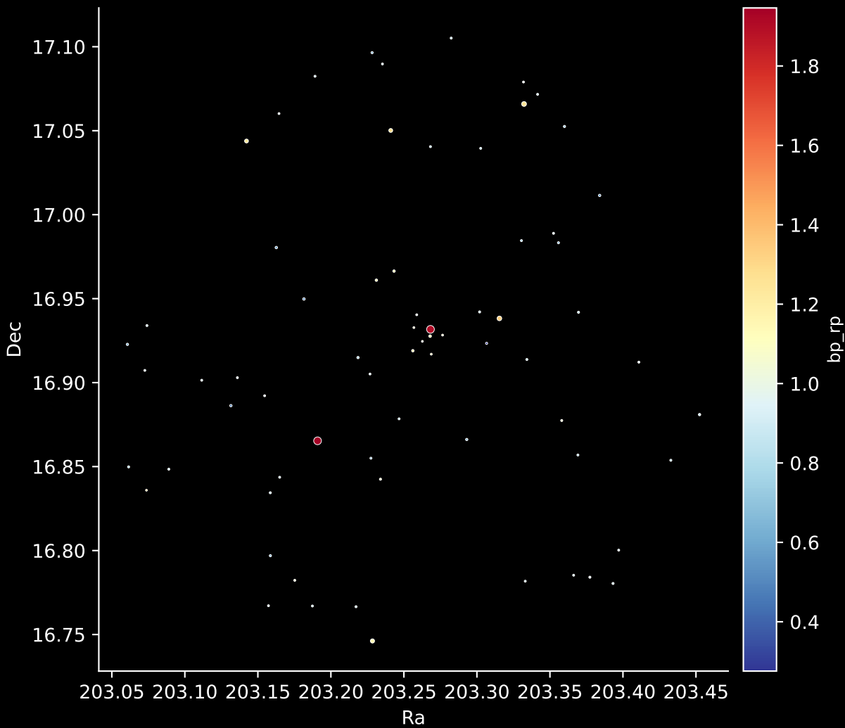
Gaia Cluster: [Berkeley_29] Stars: 69
