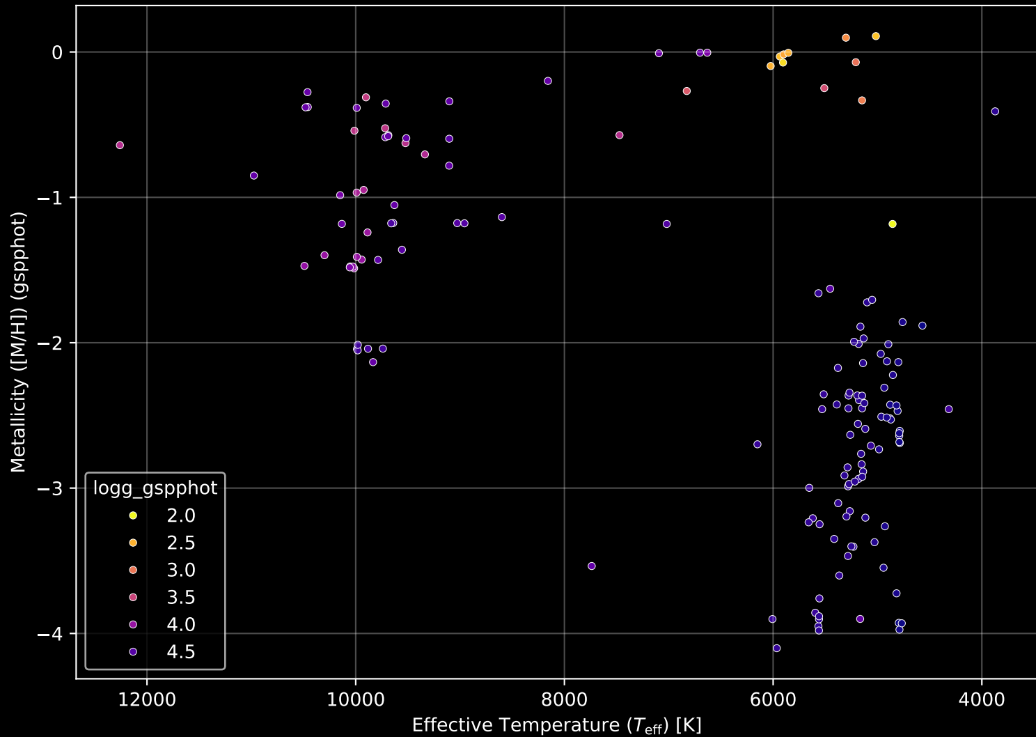
Gaia Cluster: [Berkeley_33] Stellar Population Parameters (n= 153)
