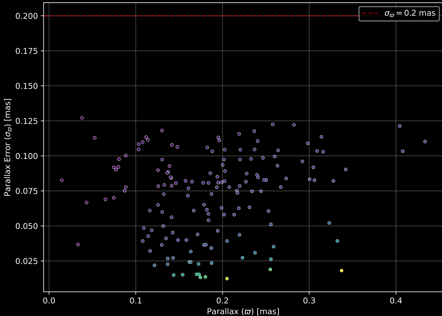
Gaia Cluster: [Berkeley_33] Parallax Quality (n= 153)
