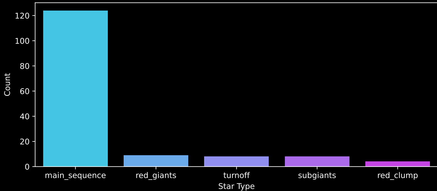
Gaia Cluster: [Berkeley_33] Count plot of Star Type
