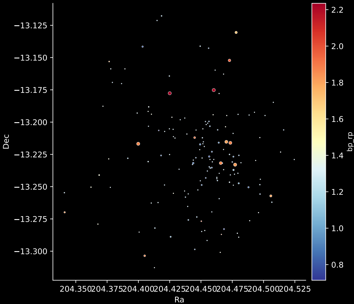
Gaia Cluster: [Berkeley_33] Stars: 153
