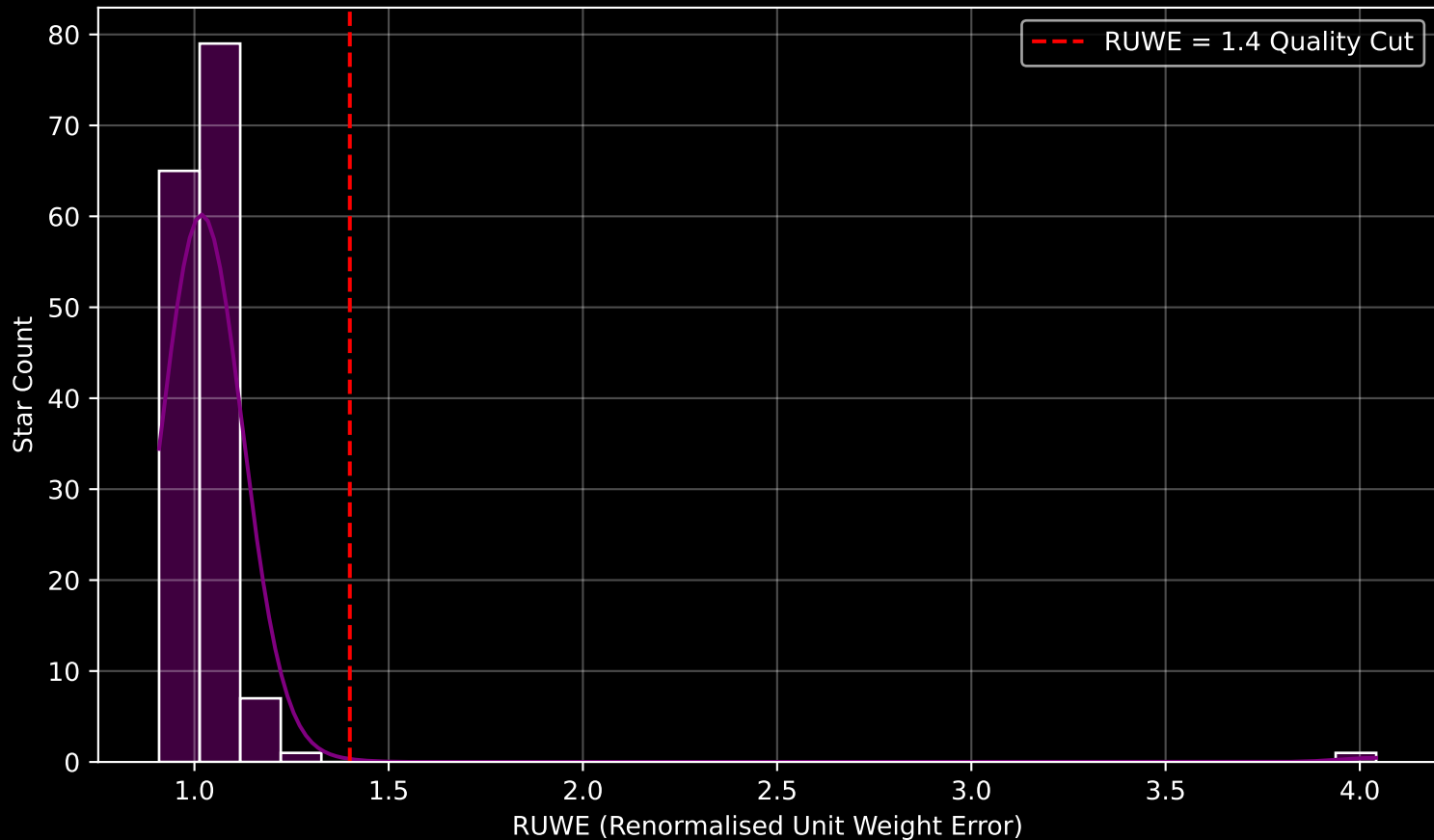
Gaia Cluster: [Berkeley_33] RUWE Distribution (n= 153)
