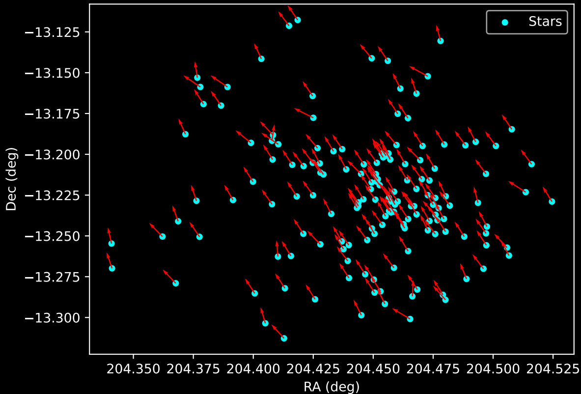
Gaia Cluster: [Berkeley_33] Proper Motion Vectors for Gaia Star Field (n= 153)
