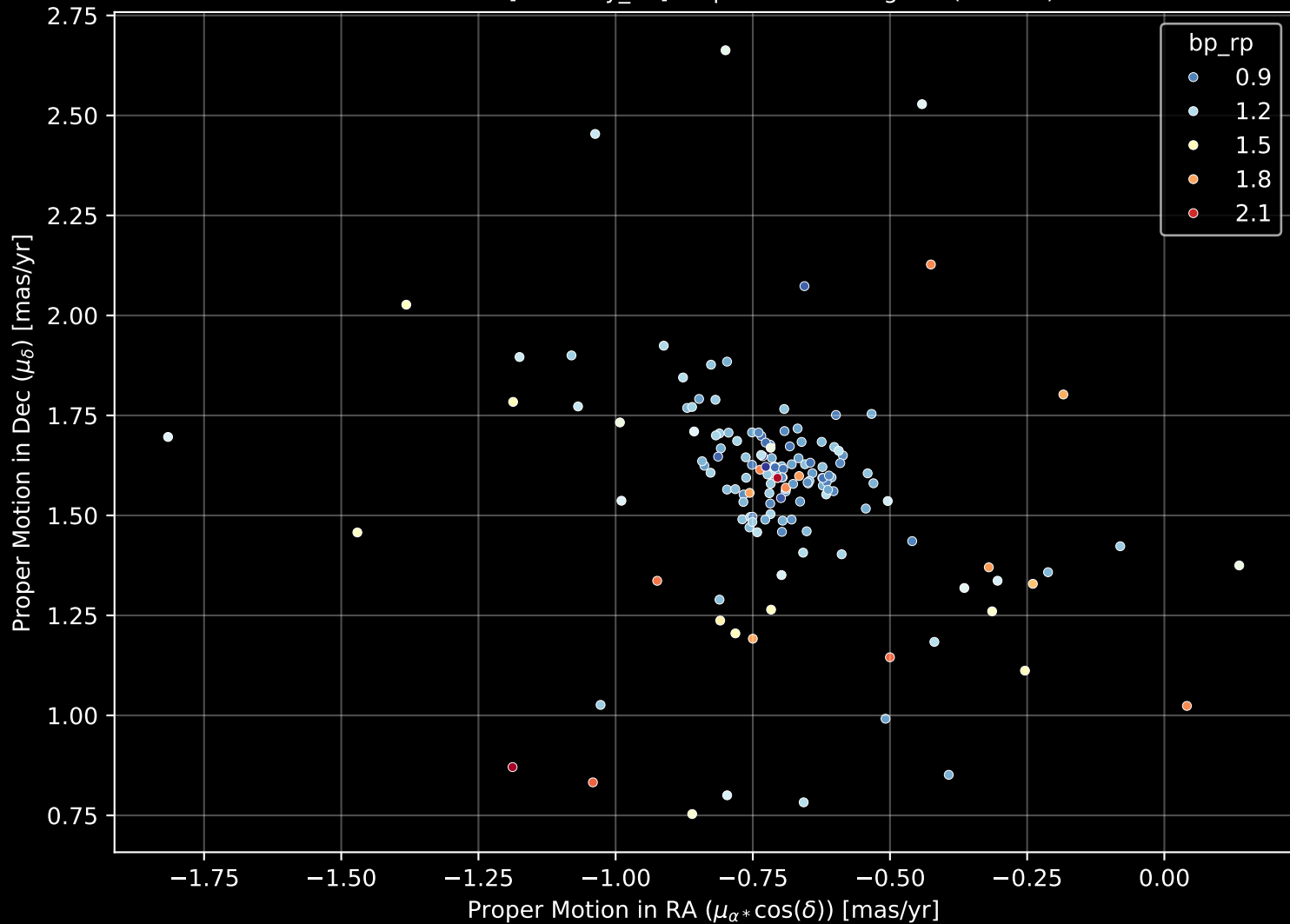
Gaia Cluster: [Berkeley_33] Proper Motion Diagram (n= 153)
