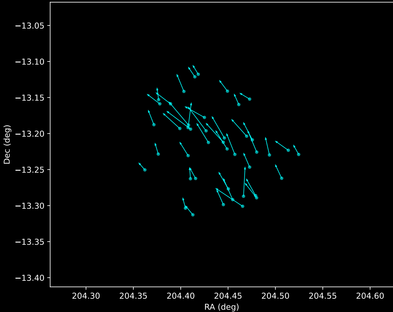
Gaia DR3 Noise Stream Proper Motion Vectors (n=43)
