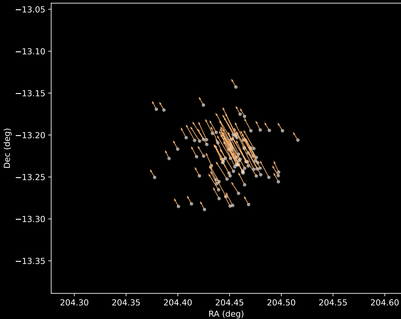
Gaia DR3 Cluster 3 Proper Motion Vectors (n=92)
