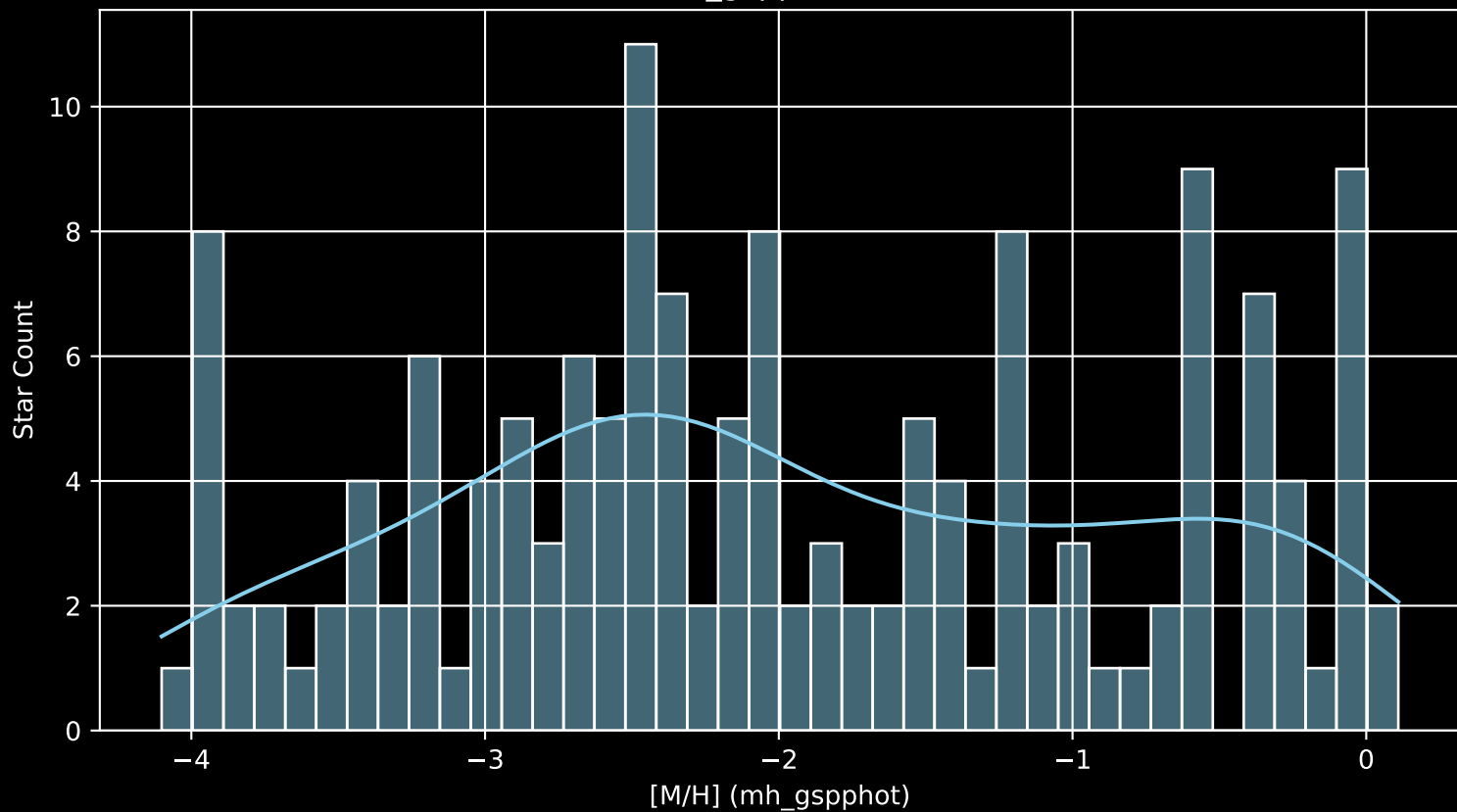
Gaia Cluster: [Berkeley_33 [M/H] (mh_gspphot) (n= 153)
