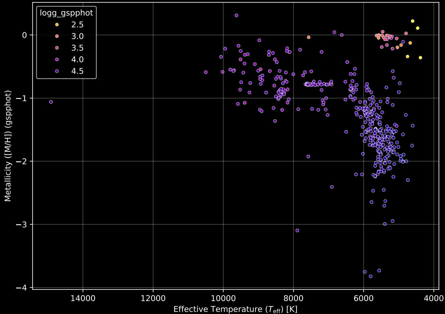
Gaia Cluster: [Berkeley_35] Stellar Population Parameters (n= 410)
