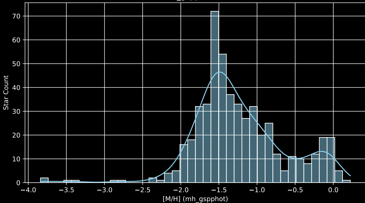
Gaia Cluster: [Berkeley_39 [M/H] (mh_gspphot) (n= 519)
