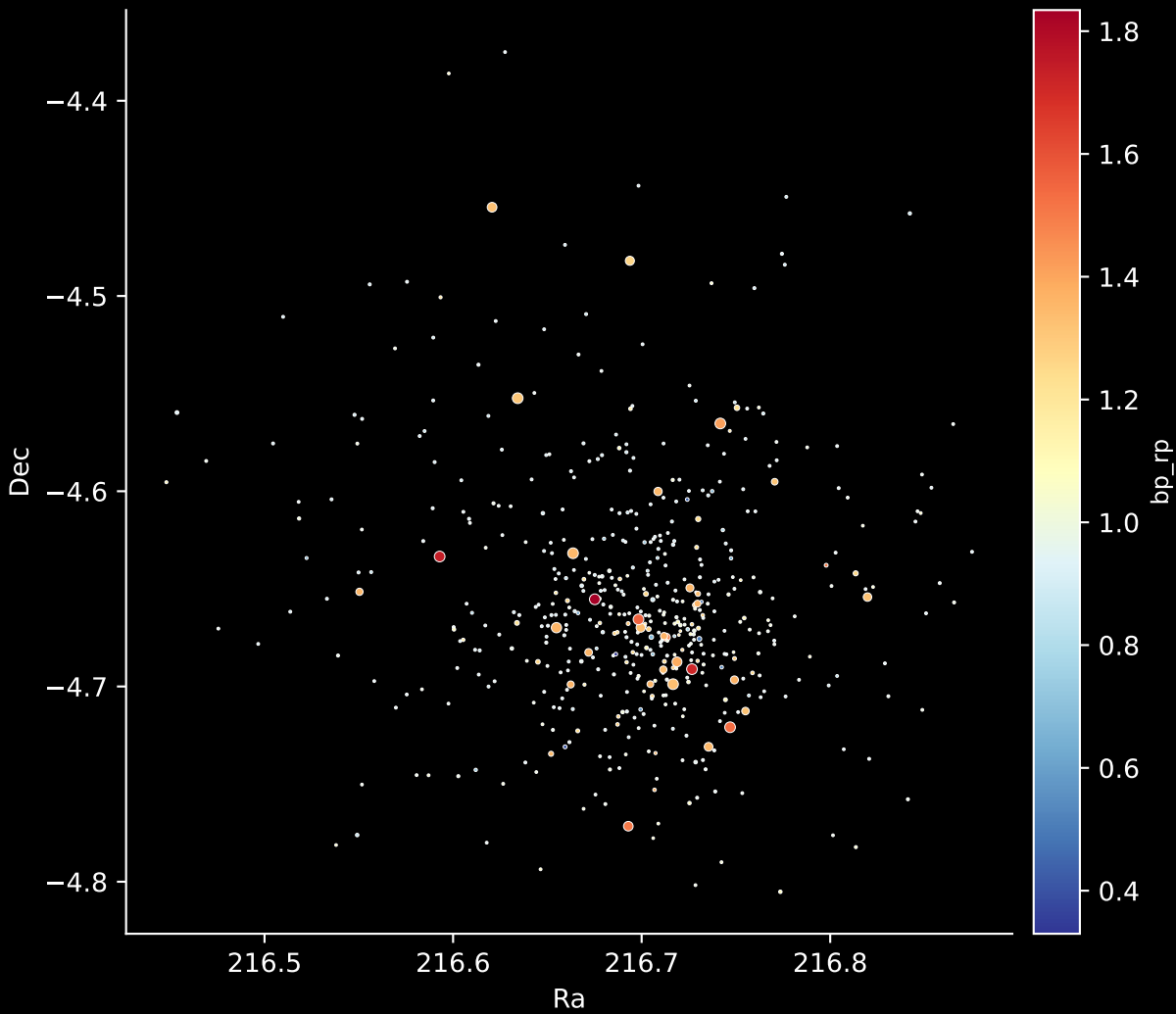
Gaia Cluster: [Berkeley_39] Stars: 519
