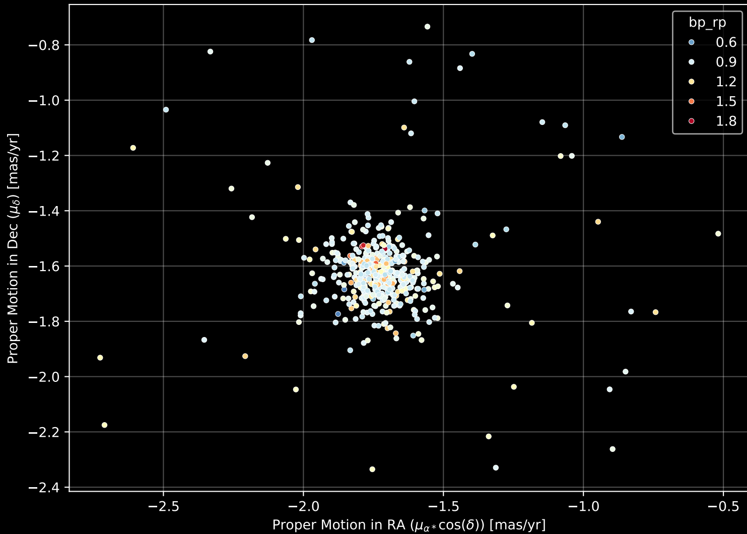
Gaia Cluster: [Berkeley_39] Proper Motion Diagram (n= 519)
