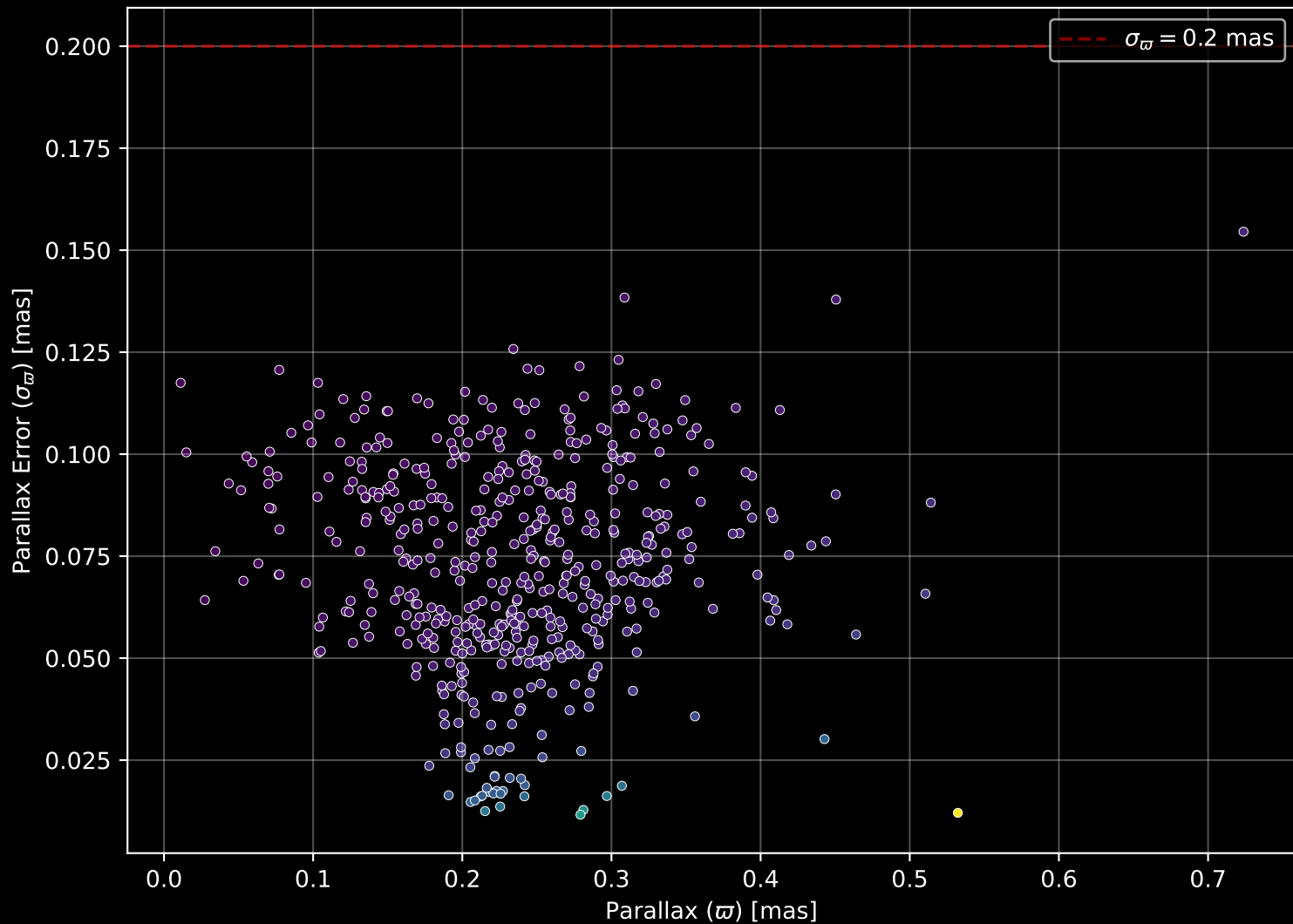
Gaia Cluster: [Berkeley_39] Parallax Quality (n= 519)
