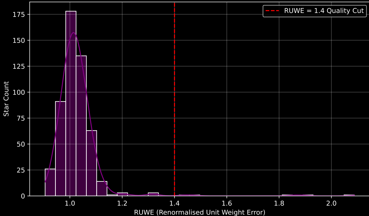
Gaia Cluster: [Berkeley_39] RUWE Distribution (n= 519)
