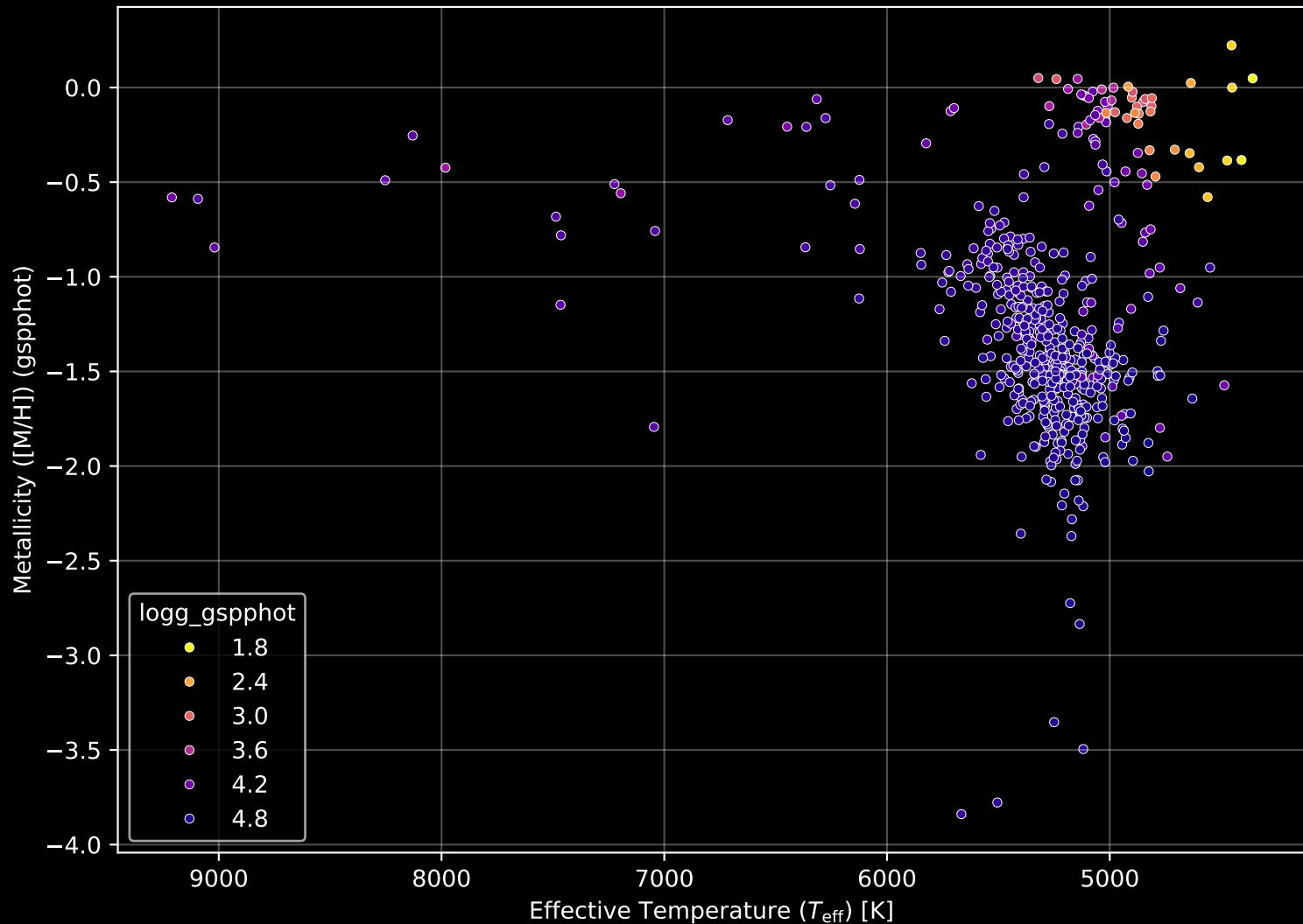
Gaia Cluster: [Berkeley_39] Stellar Population Parameters (n= 519)
