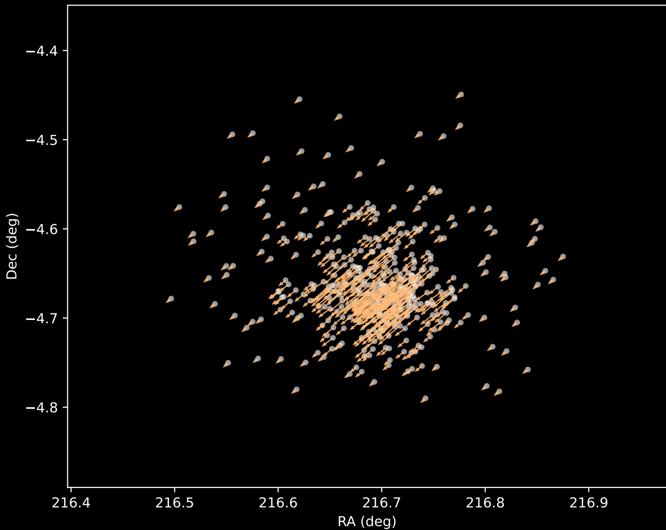
Gaia DR3 Cluster 3 Proper Motion Vectors (n=412)
