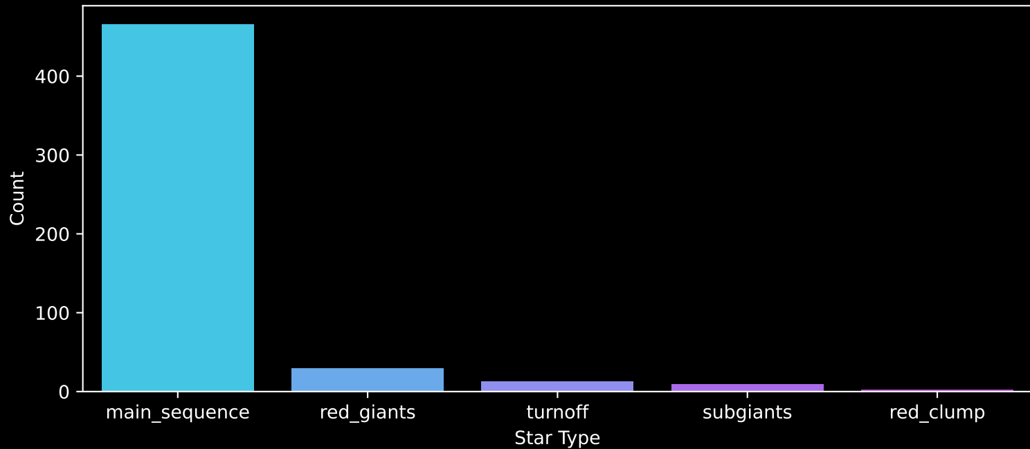
Gaia Cluster: [Berkeley_39] Count plot of Star Type
