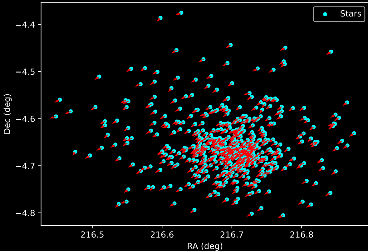
Gaia Cluster: [Berkeley_39] Proper Motion Vectors for Gaia Star Field (n= 519)
