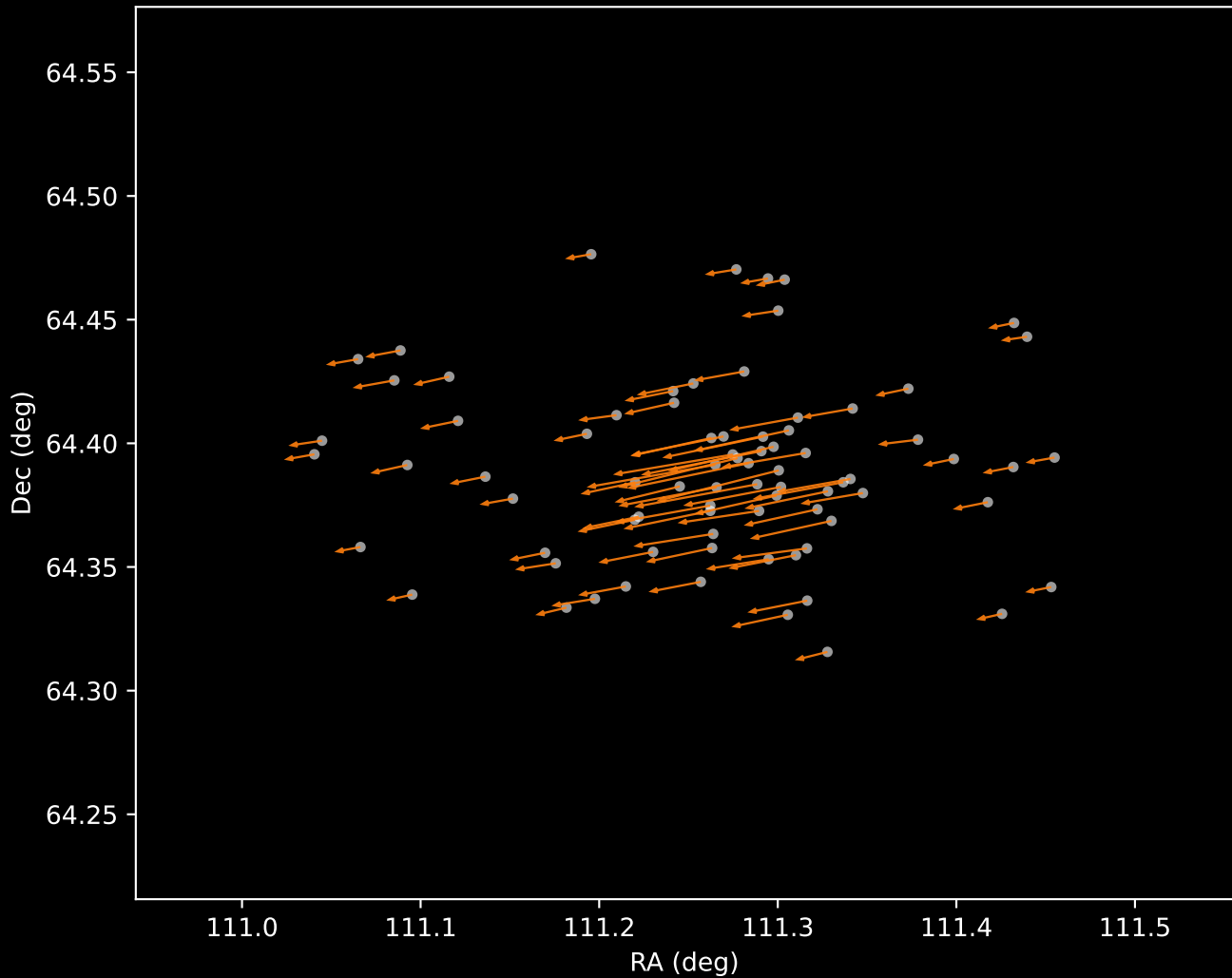
Gaia DR3 Cluster 2 Proper Motion Vectors (n=79)
