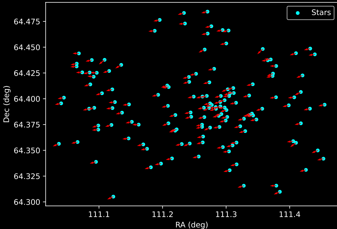
Gaia Cluster: [Berkeley_4] Proper Motion Vectors for Gaia Star Field (n= 139)
