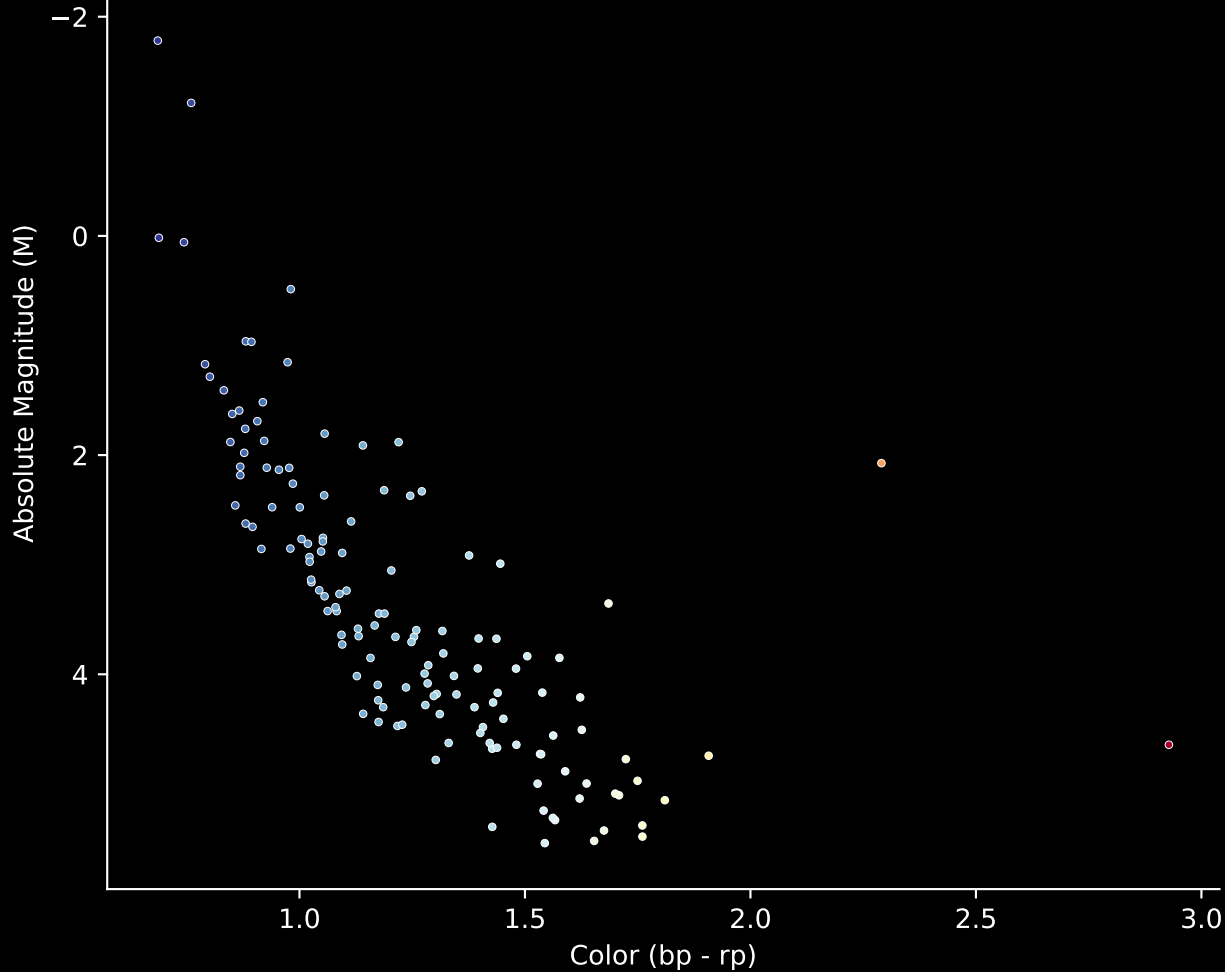
Gaia Cluster: [Berkeley_4] Stars (n= 139) Hertzsprung-Russel Diagram
