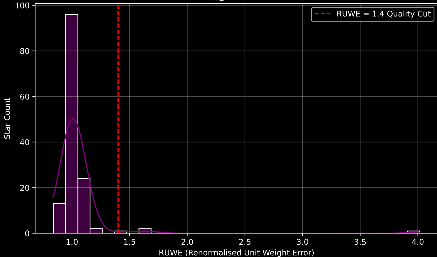
Gaia Cluster: [Berkeley_4] RUWE Distribution (n= 139)
