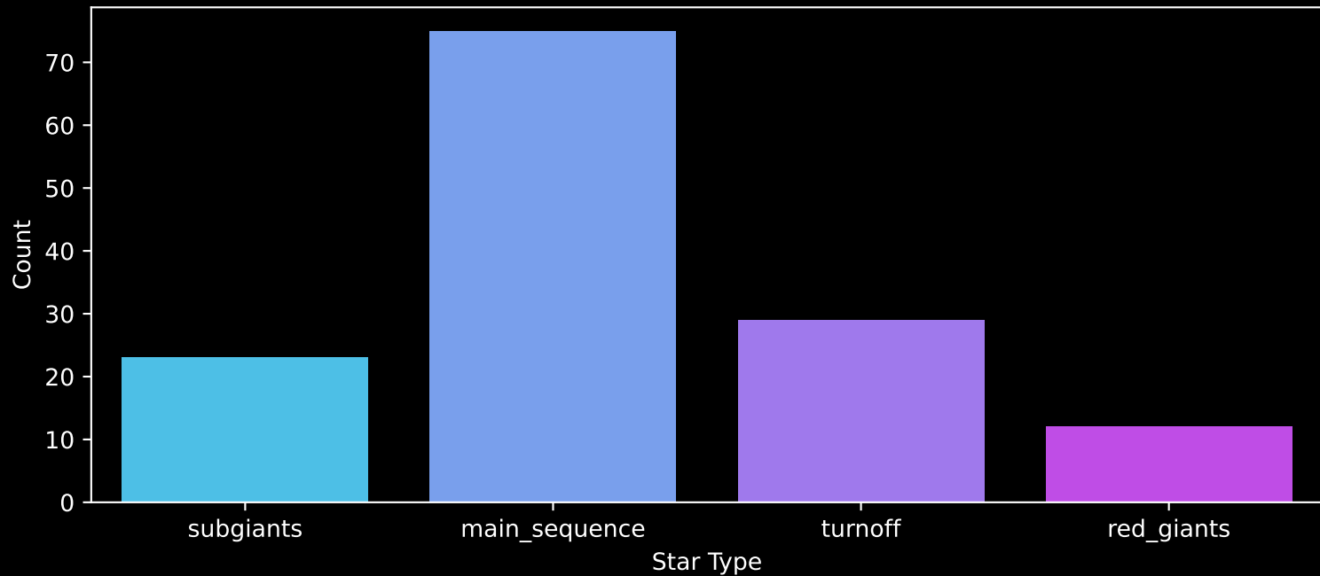
Gaia Cluster: [Berkeley_4] Count plot of Star Type
