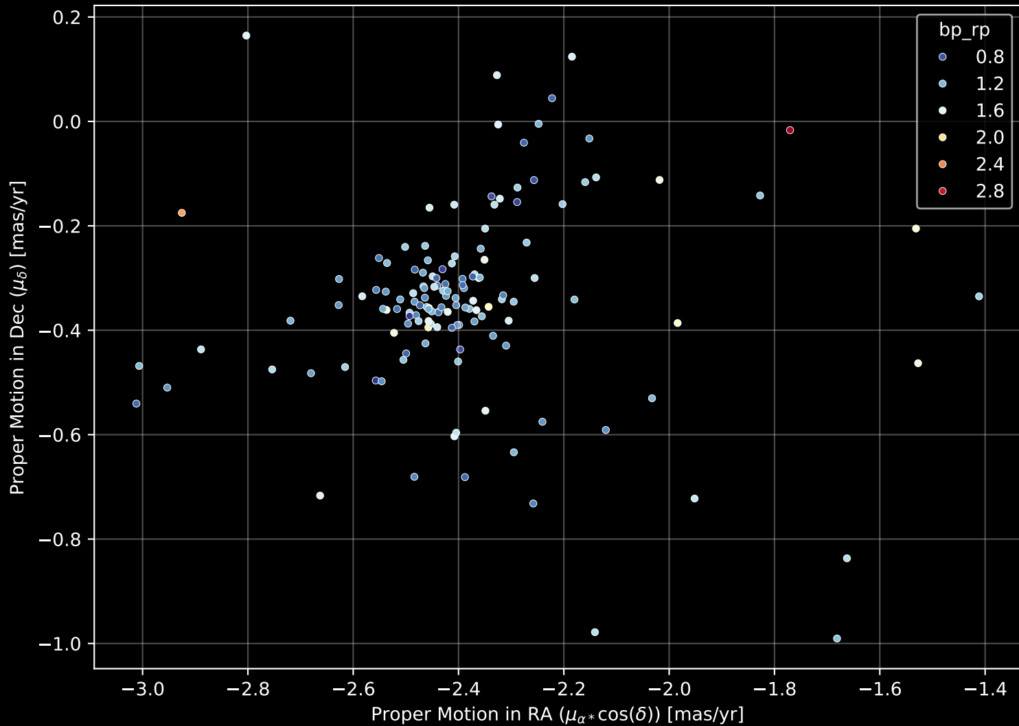
Gaia Cluster: [Berkeley_4] Proper Motion Diagram (n= 139)
