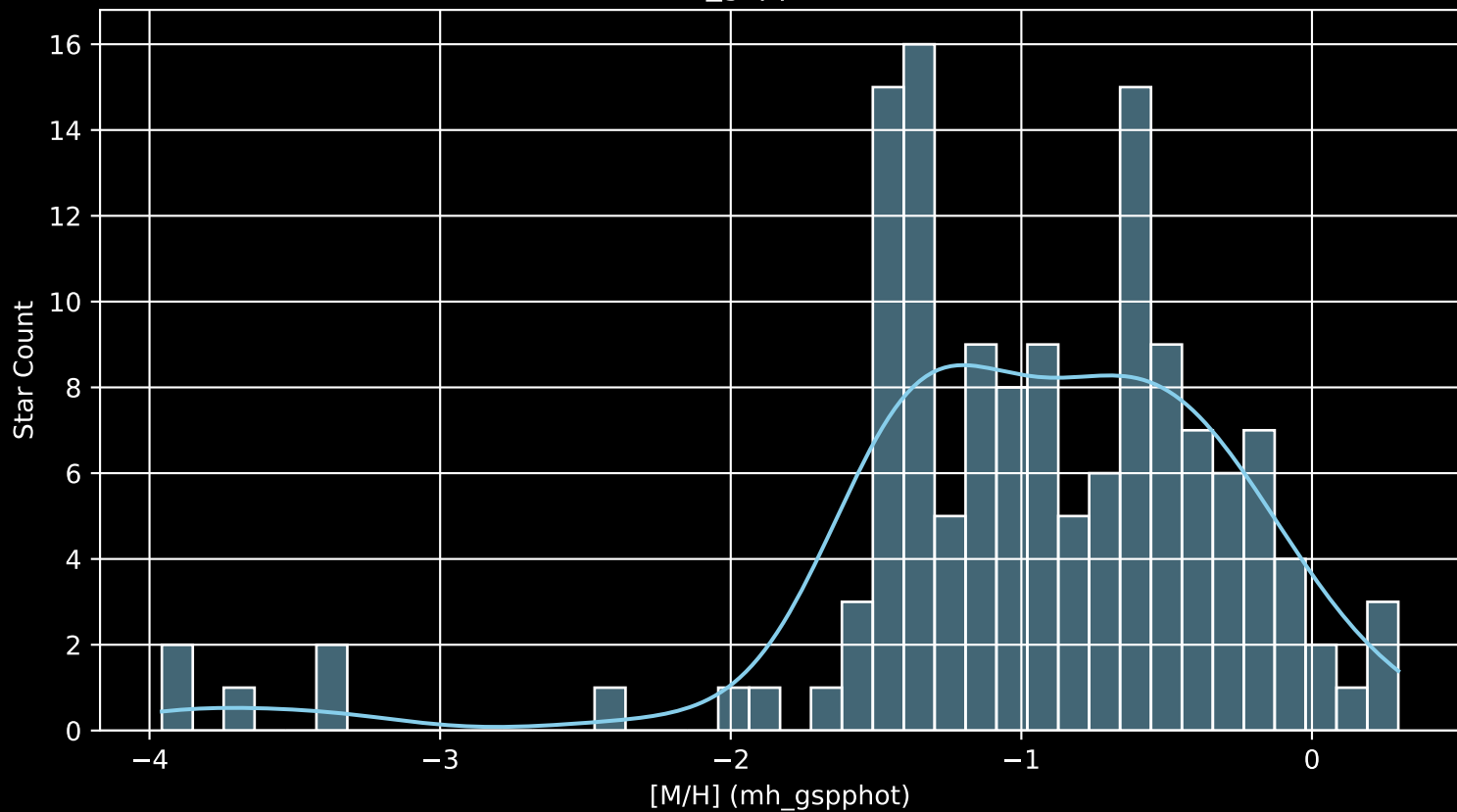
Gaia Cluster: [Berkeley_4 [M/H] (mh_gspphot) (n= 139)
