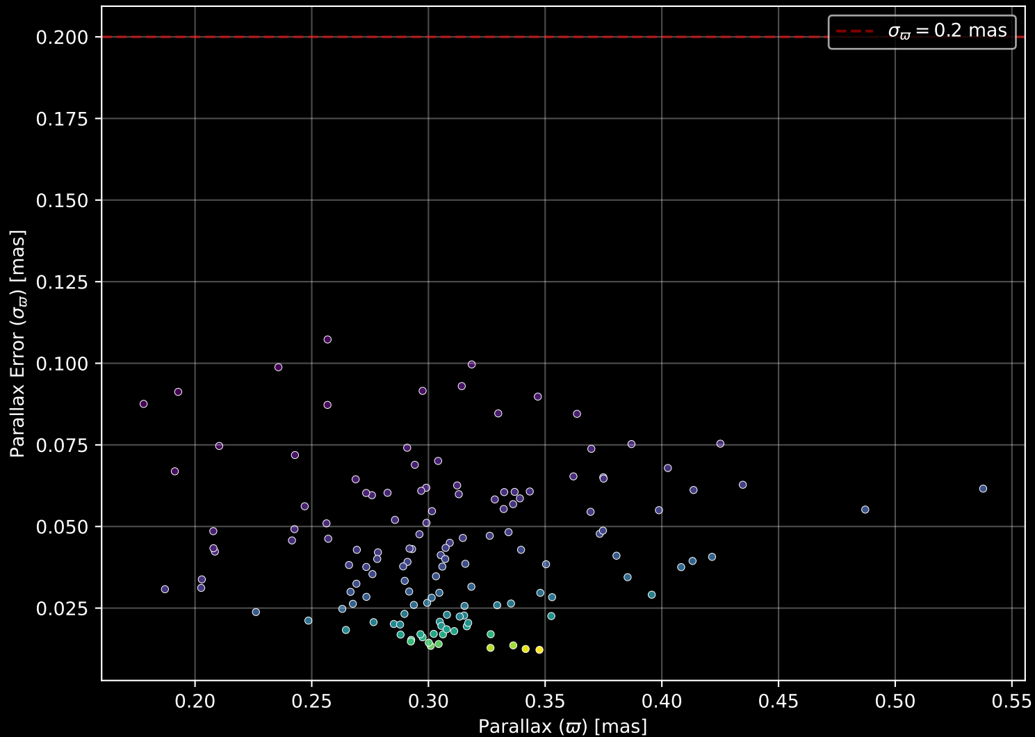
Gaia Cluster: [Berkeley_4] Parallax Quality (n= 139)
