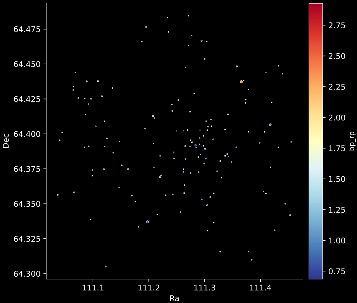
Gaia Cluster: [Berkeley_4] Stars: 139
