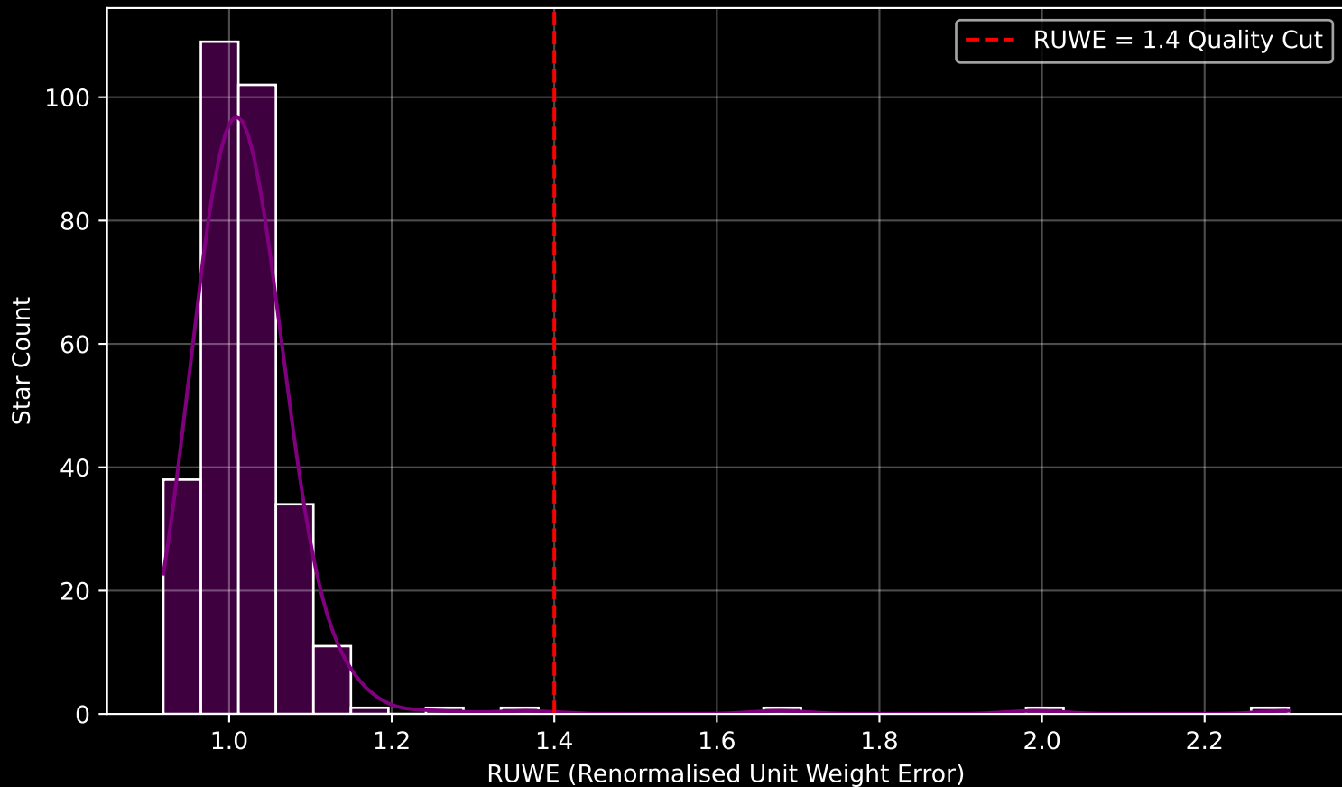
Gaia Cluster: [Berkeley_44] RUWE Distribution (n= 300)
