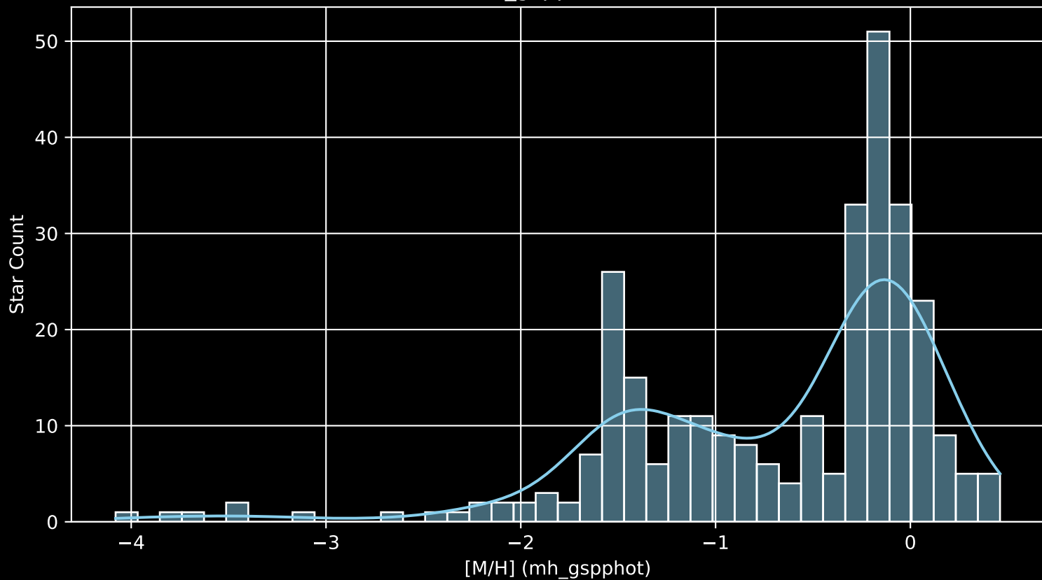
Gaia Cluster: [Berkeley_44 [M/H] (mh_gspphot) (n= 298)
