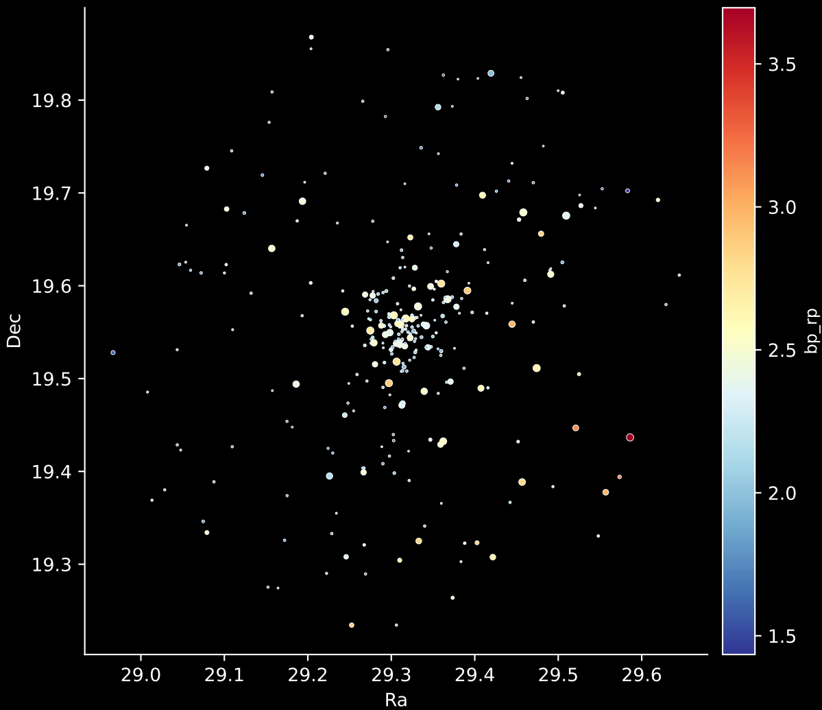
Gaia Cluster: [Berkeley_44] Stars: 300
