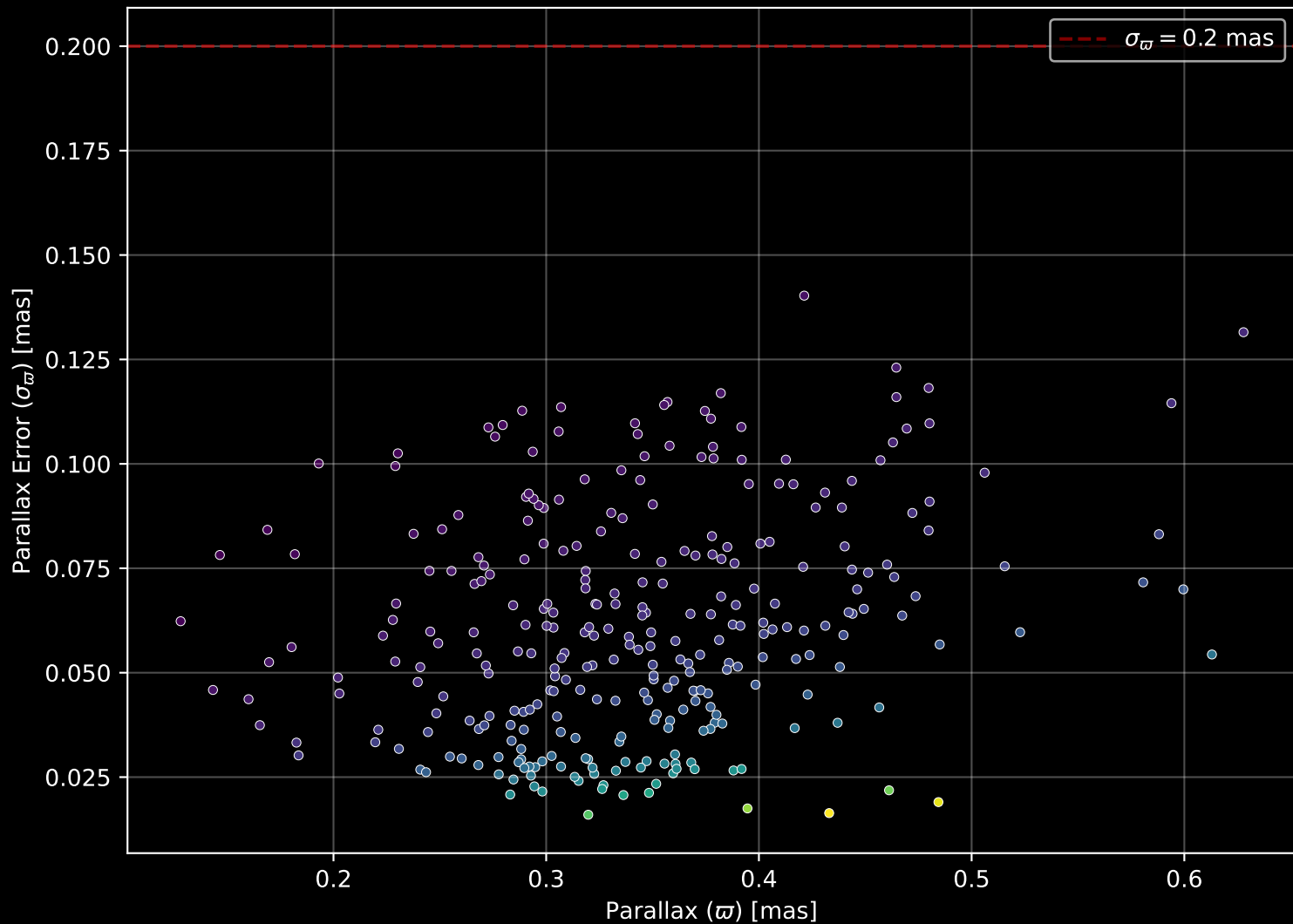
Gaia Cluster: [Berkeley_44] Parallax Quality (n= 300)
