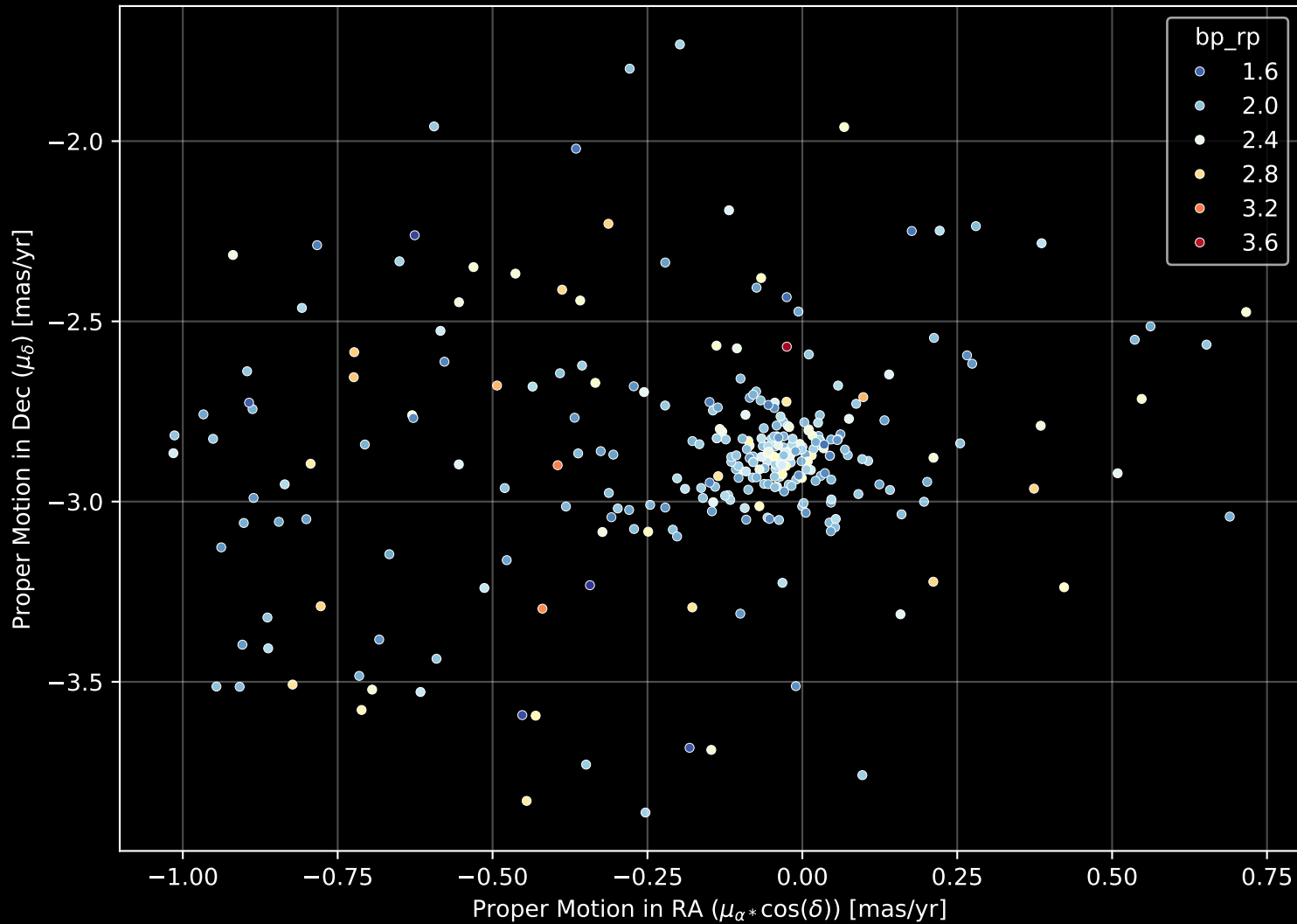
Gaia Cluster: [Berkeley_44] Proper Motion Diagram (n= 300)
