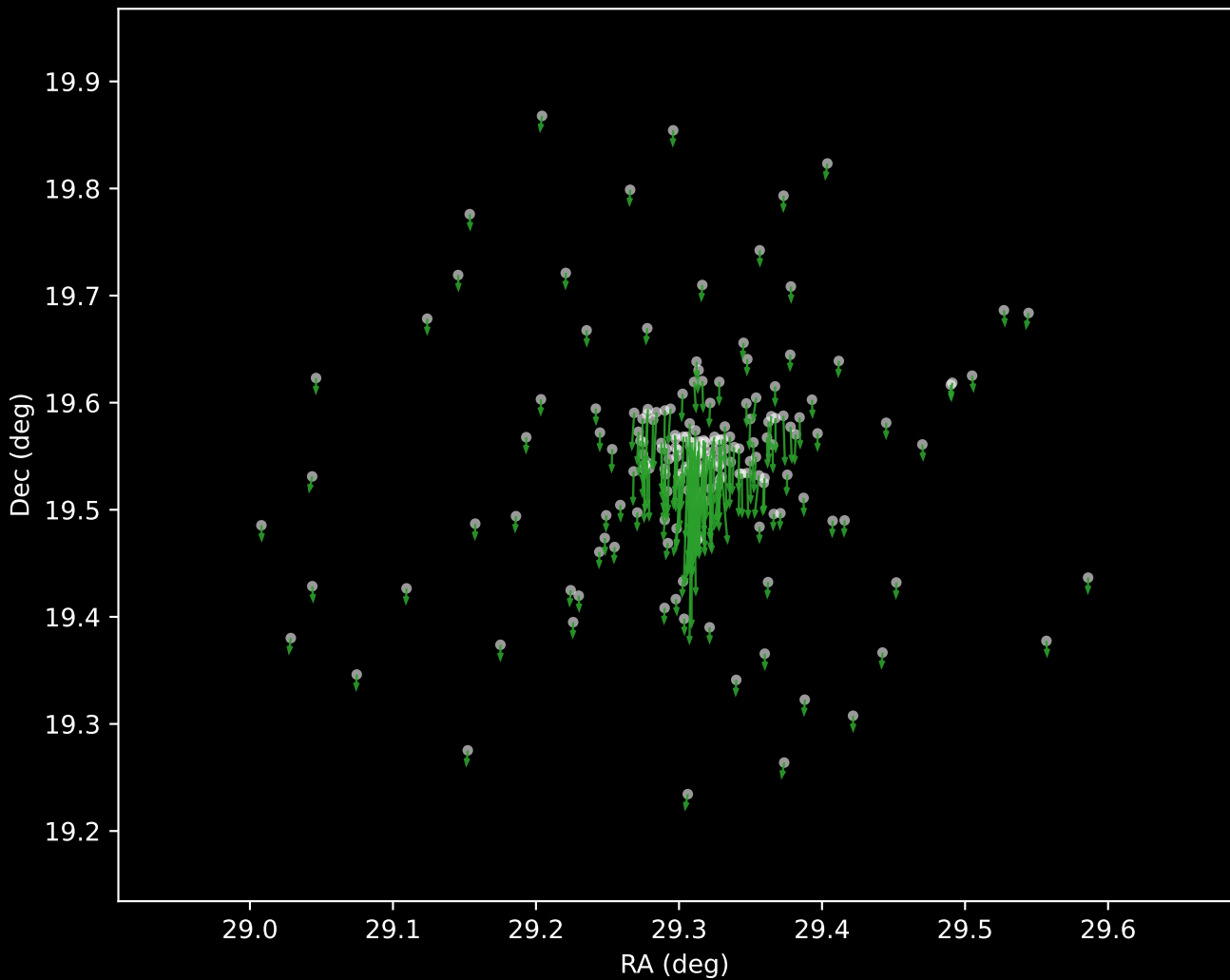
Gaia DR3 Cluster 4 Proper Motion Vectors (n=199)
