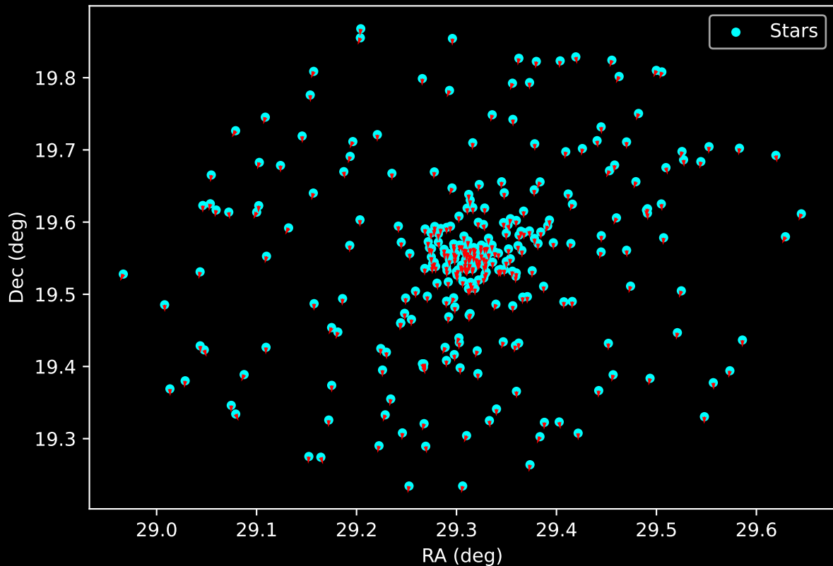
Gaia Cluster: [Berkeley_44] Proper Motion Vectors for Gaia Star Field (n= 300)
