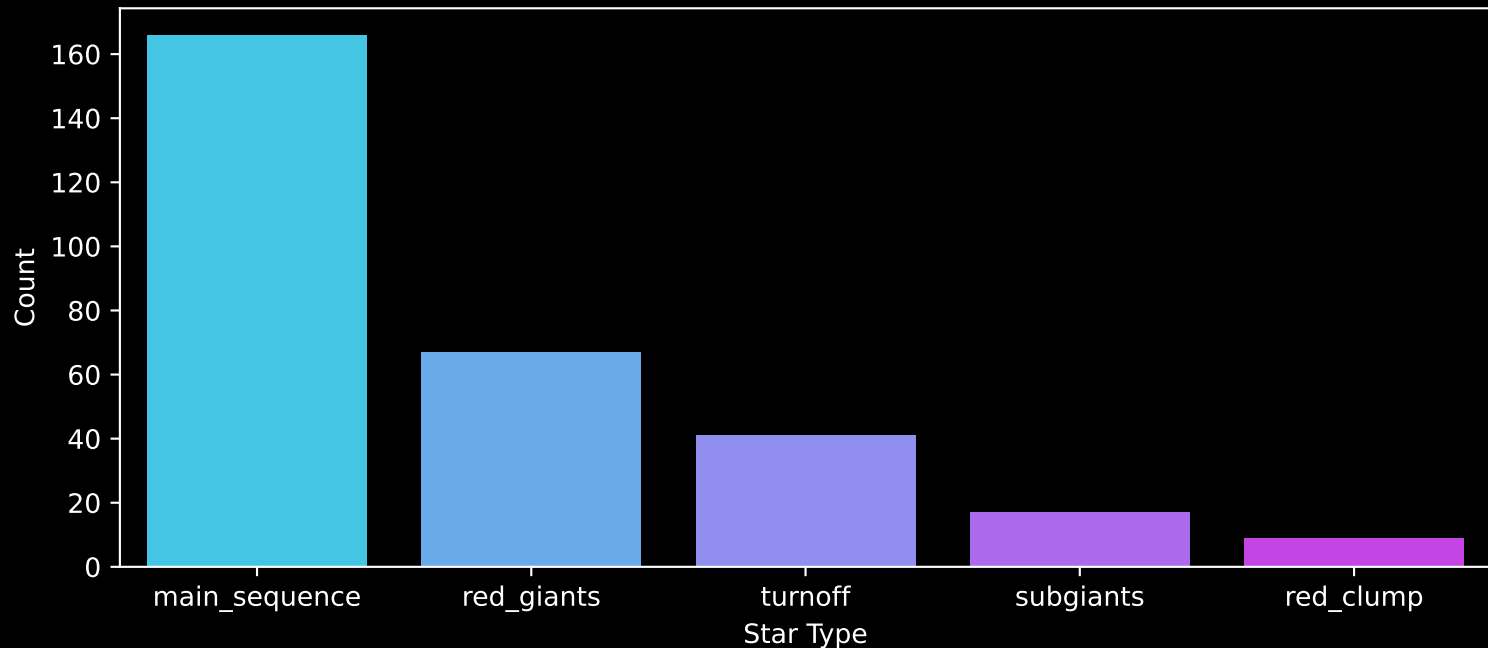
Gaia Cluster: [Berkeley_44] Count plot of Star Type
