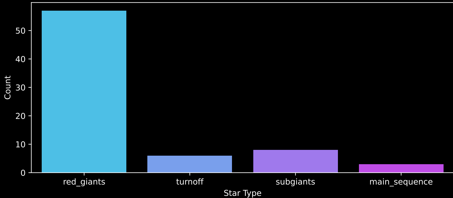
Gaia Cluster: [Berkeley_52] Count plot of Star Type
