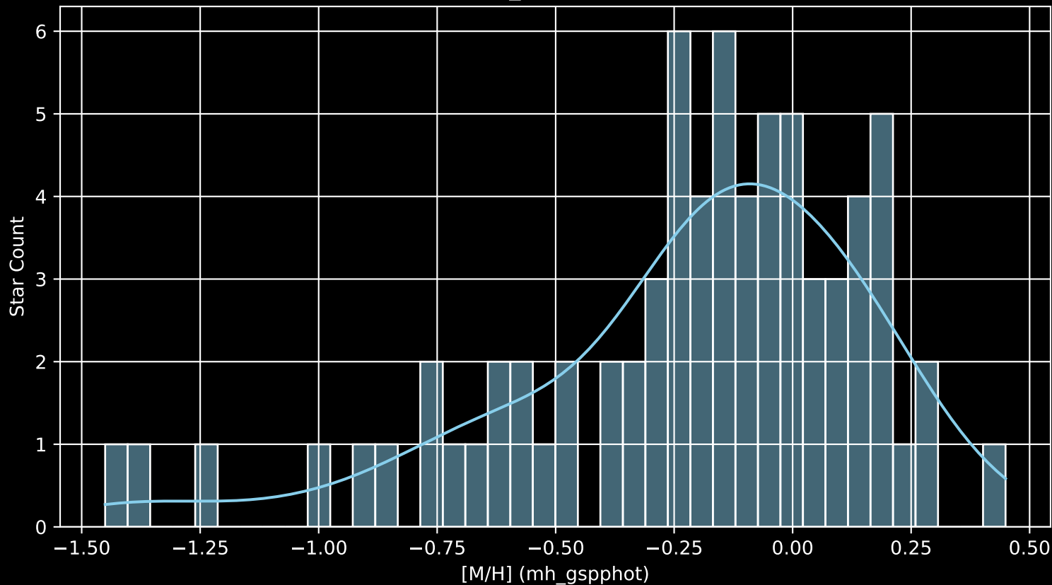
Gaia Cluster: [Berkeley_52 [M/H] (mh_gspphot) (n= 73)
