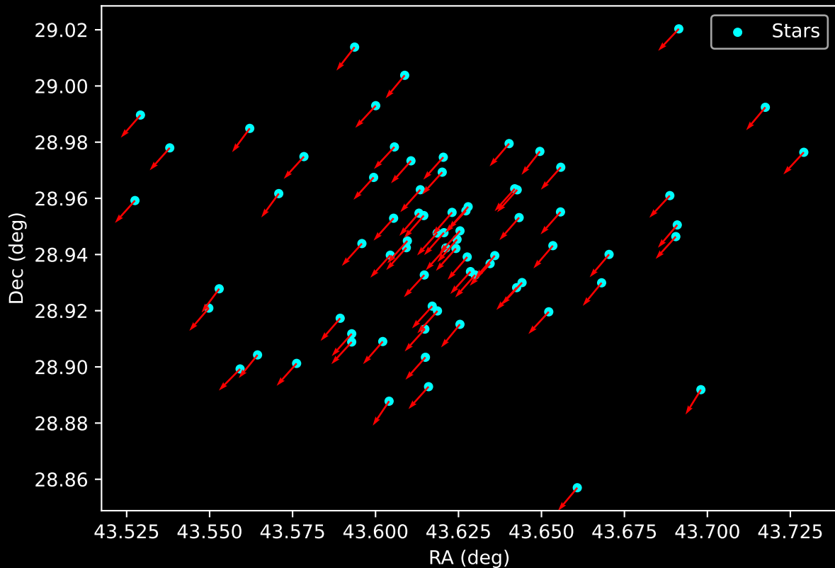
Gaia Cluster: [Berkeley_52] Proper Motion Vectors for Gaia Star Field (n= 74)
