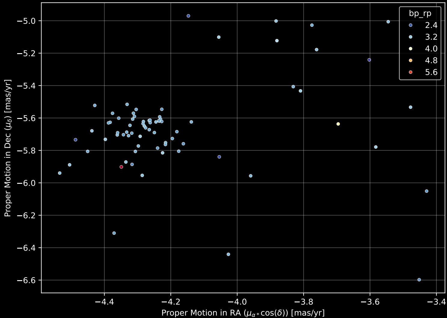
Gaia Cluster: [Berkeley_52] Proper Motion Diagram (n= 74)
