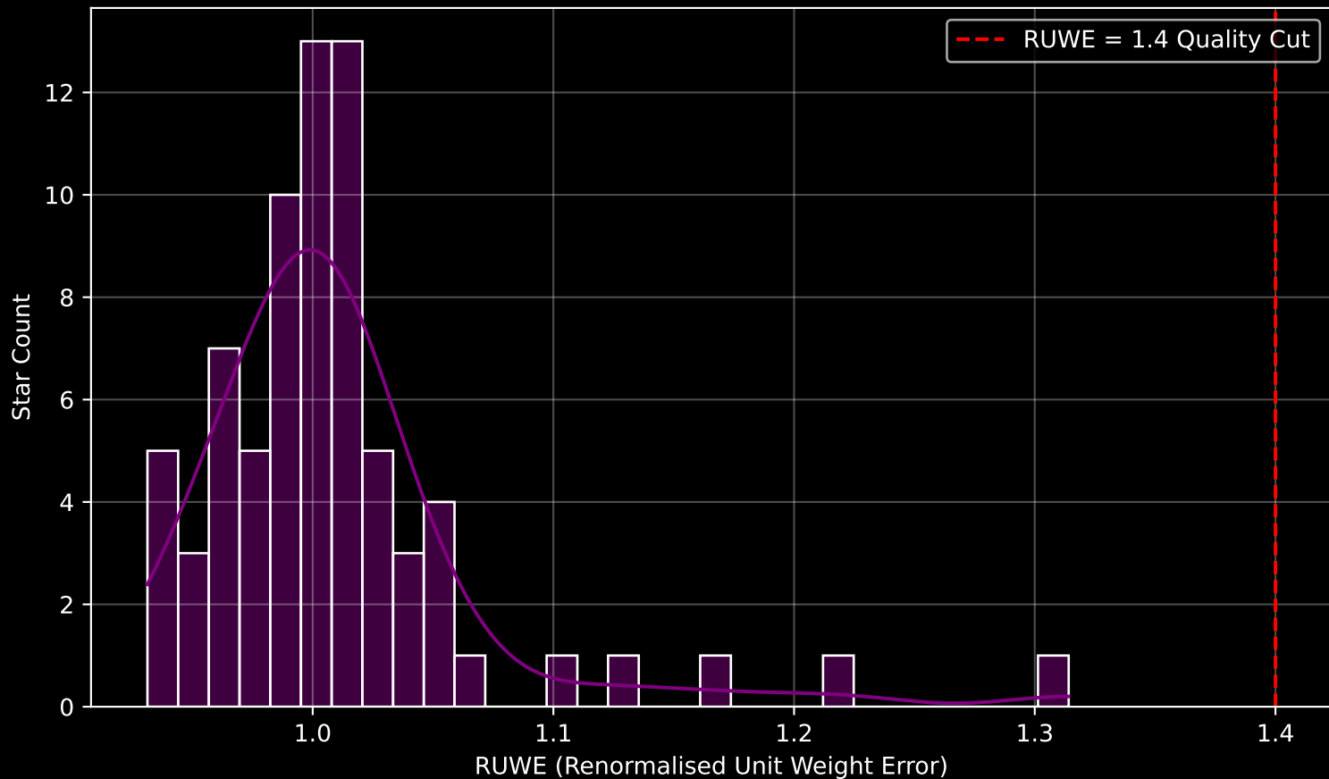
Gaia Cluster: [Berkeley_52] RUWE Distribution (n= 74)
