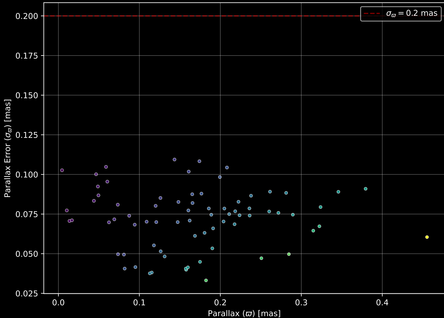
Gaia Cluster: [Berkeley_52] Parallax Quality (n= 74)
