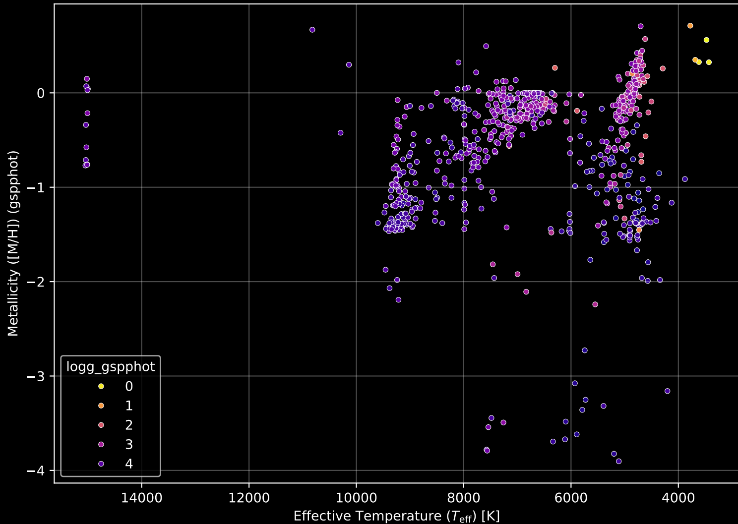
Gaia Cluster: [Berkeley_53] Stellar Population Parameters (n= 724)
