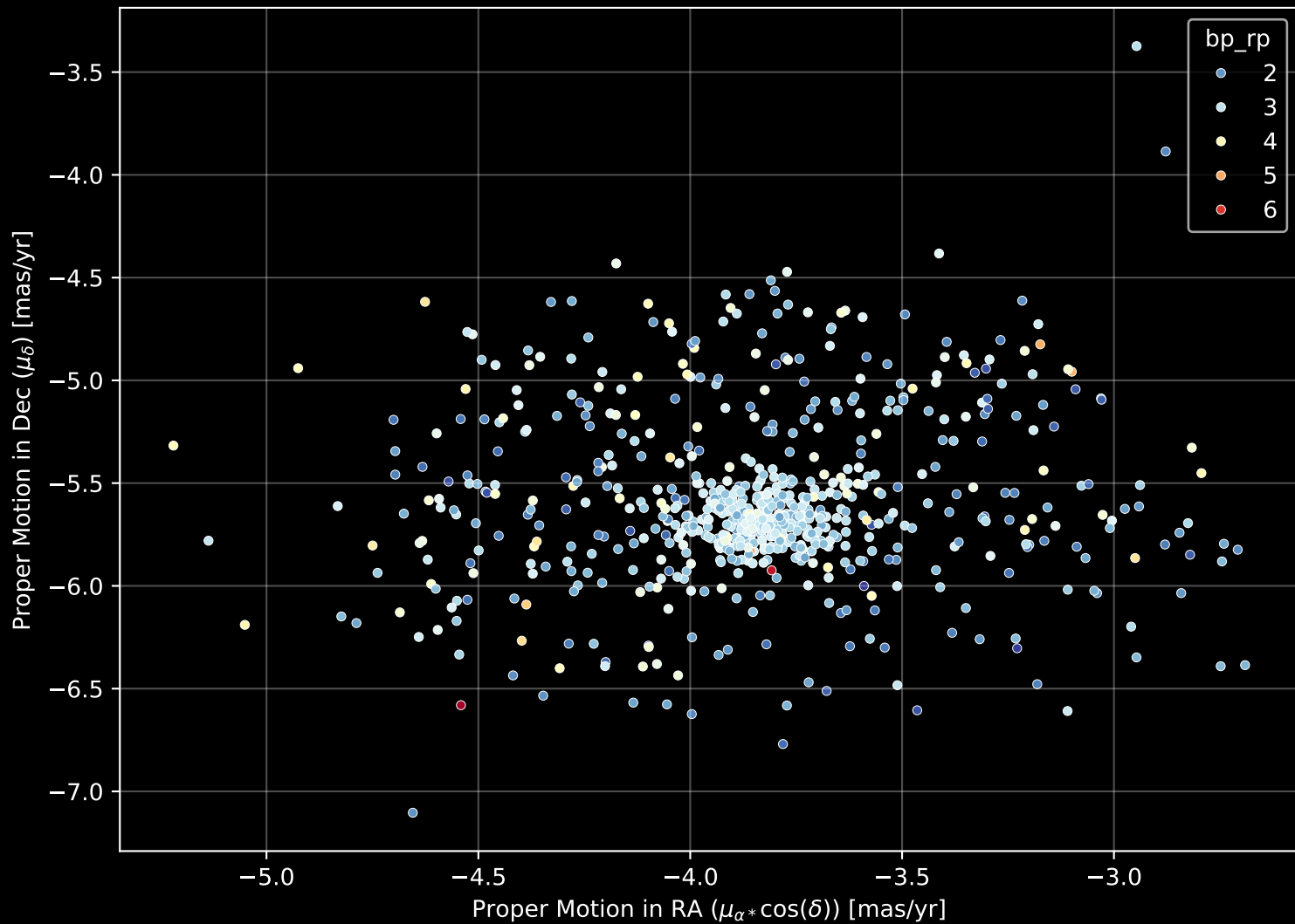
Gaia Cluster: [Berkeley_53] Proper Motion Diagram (n= 724)
