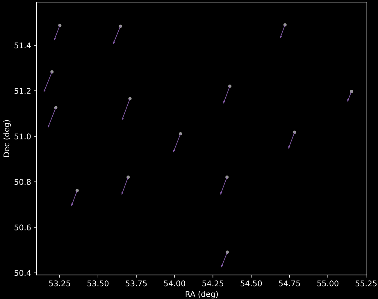
Gaia DR3 Cluster 8 Proper Motion Vectors (n=14)
