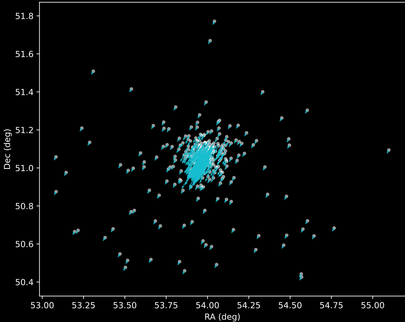
Gaia DR3 Cluster 18 Proper Motion Vectors (n=356)
