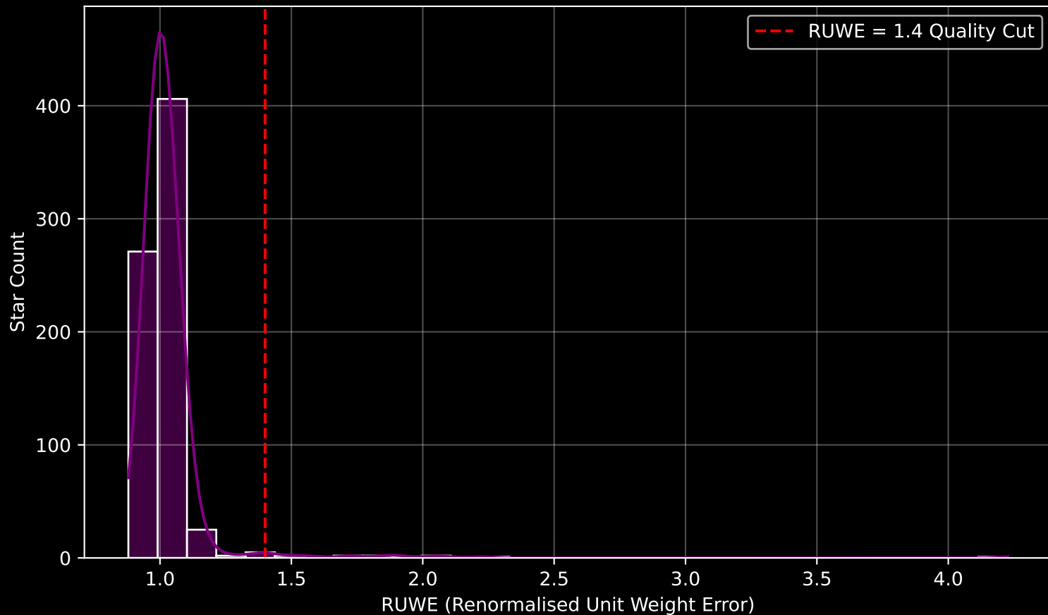
Gaia Cluster: [Berkeley_53] RUWE Distribution (n= 721)
