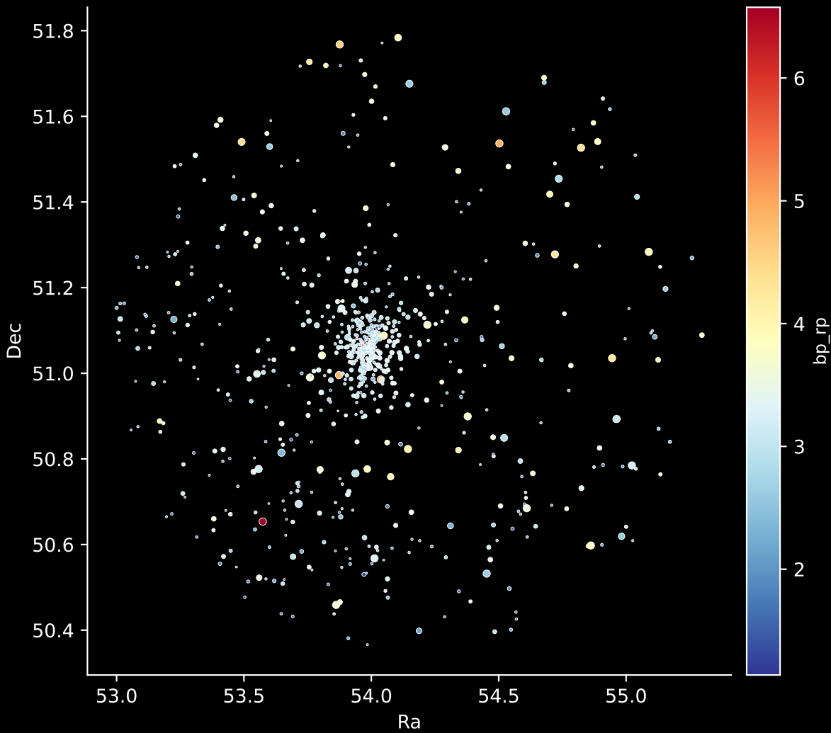
Gaia Cluster: [Berkeley_53] Stars: 724
