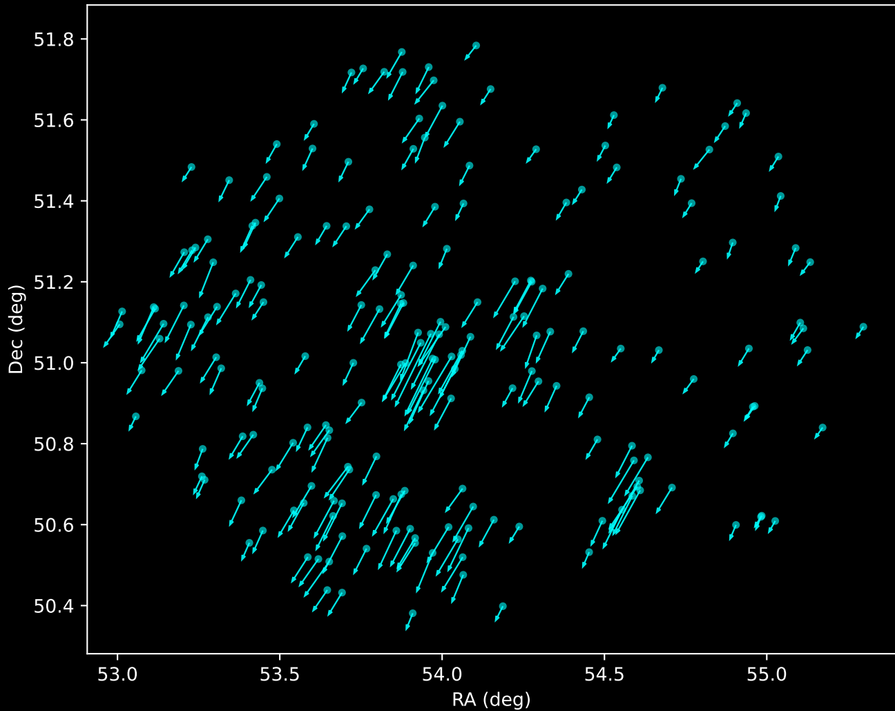
Gaia DR3 Noise Stream Proper Motion Vectors (n=200)
