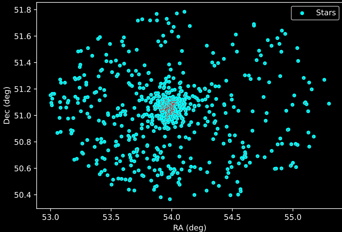
Gaia Cluster: [Berkeley_53] Proper Motion Vectors for Gaia Star Field (n= 724)
