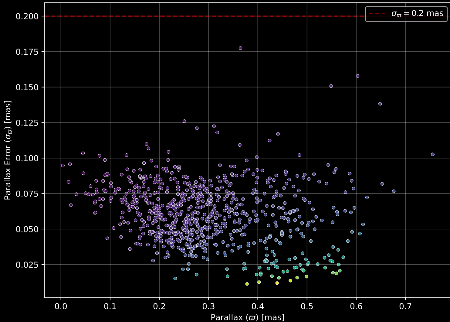
Gaia Cluster: [Berkeley_53] Parallax Quality (n= 724)
