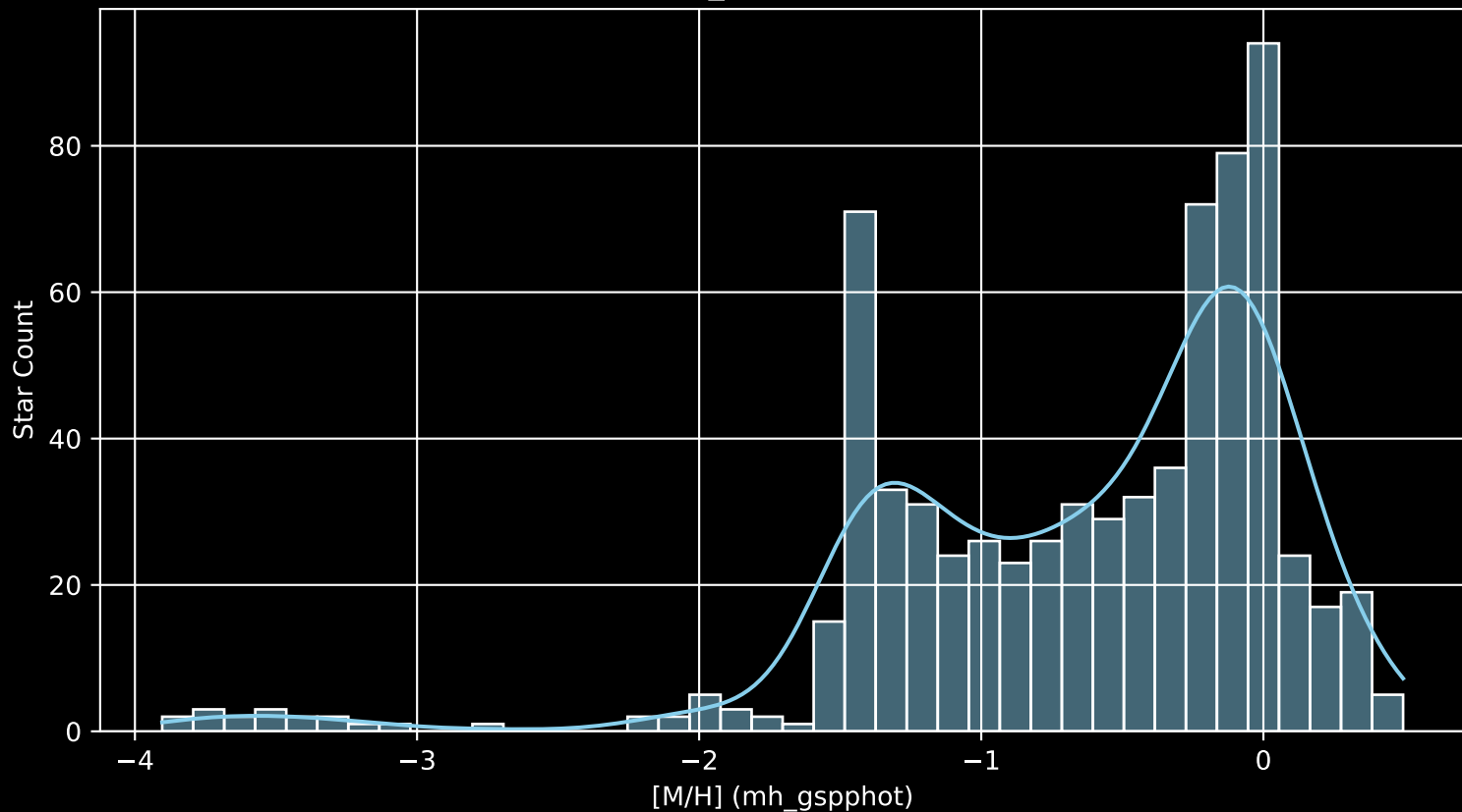
Gaia Cluster: [Berkeley_53 [M/H] (mh_gspphot) (n= 719)
