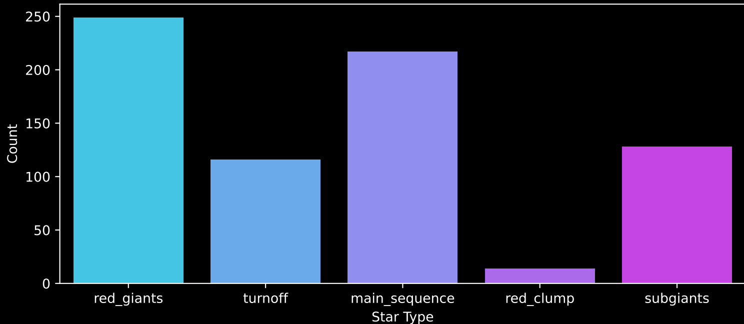
Gaia Cluster: [Berkeley_53] Count plot of Star Type
