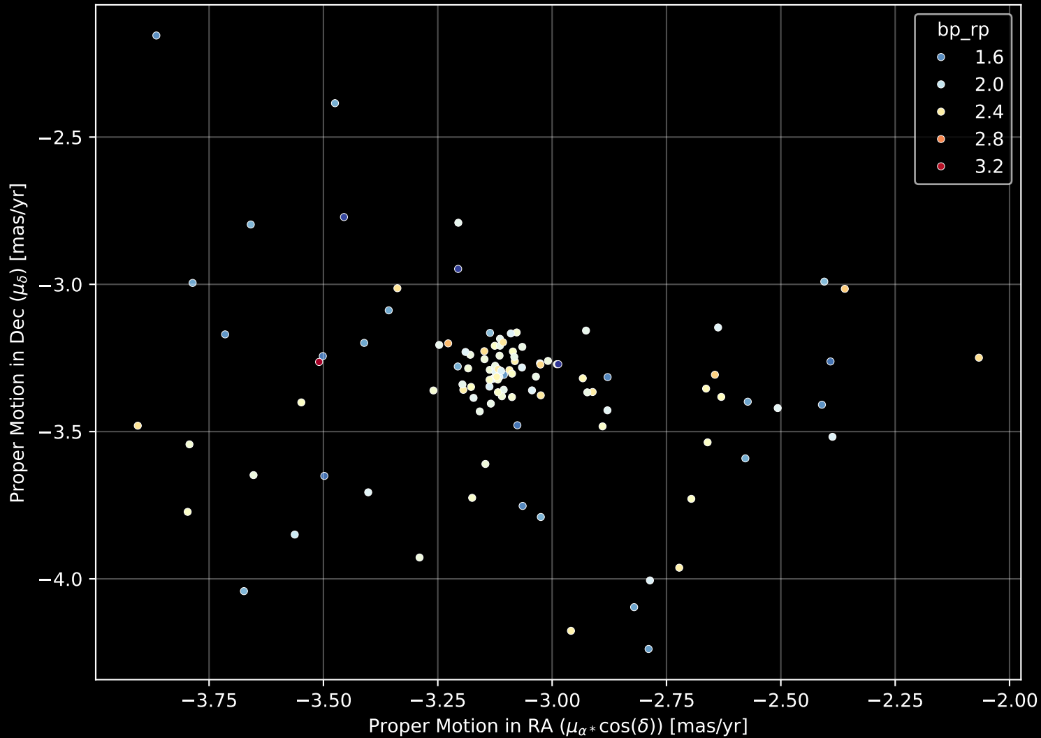
Gaia Cluster: [Berkeley_54] Proper Motion Diagram (n= 114)
