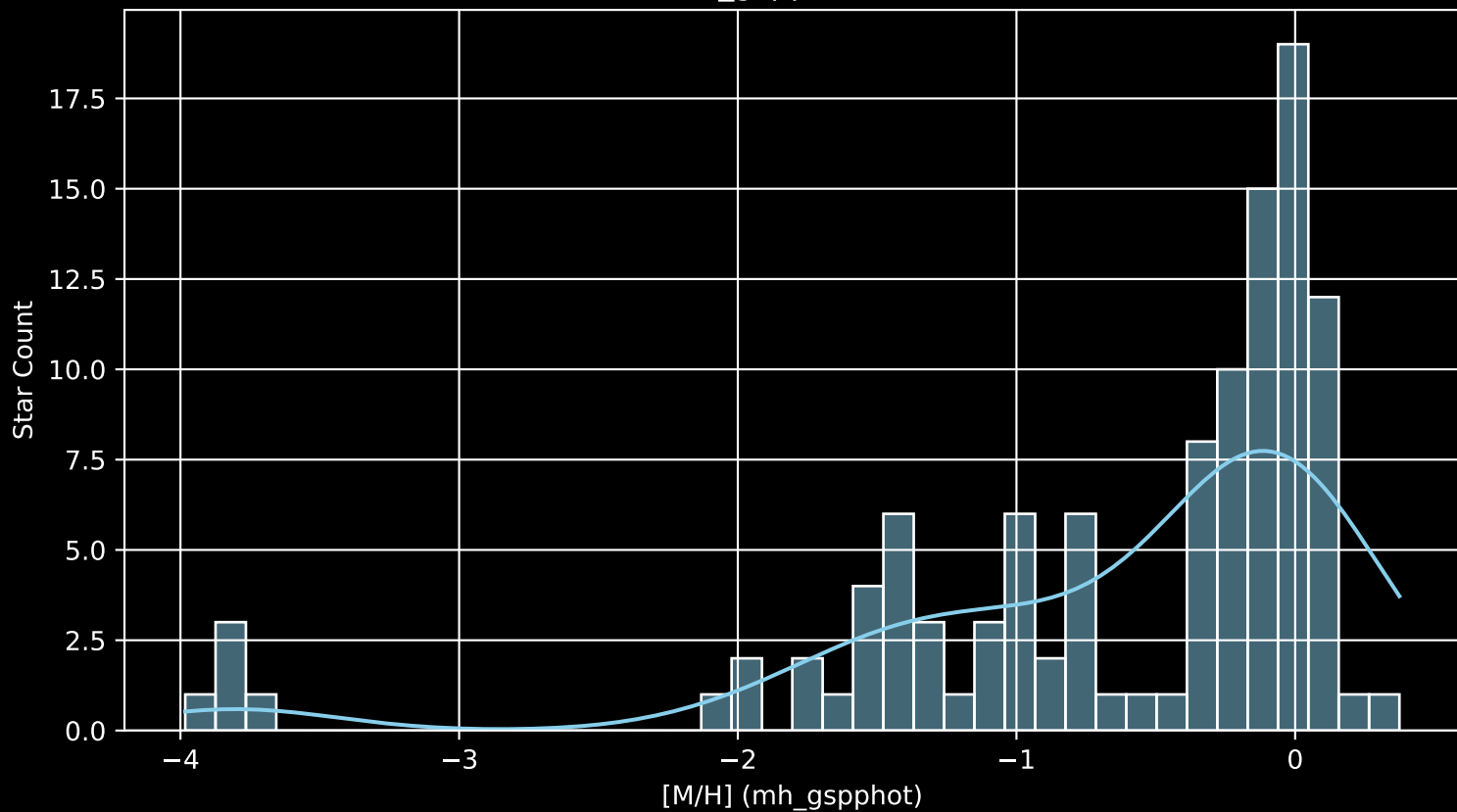
Gaia Cluster: [Berkeley_54 [M/H] (mh_gspphot) (n= 111)
