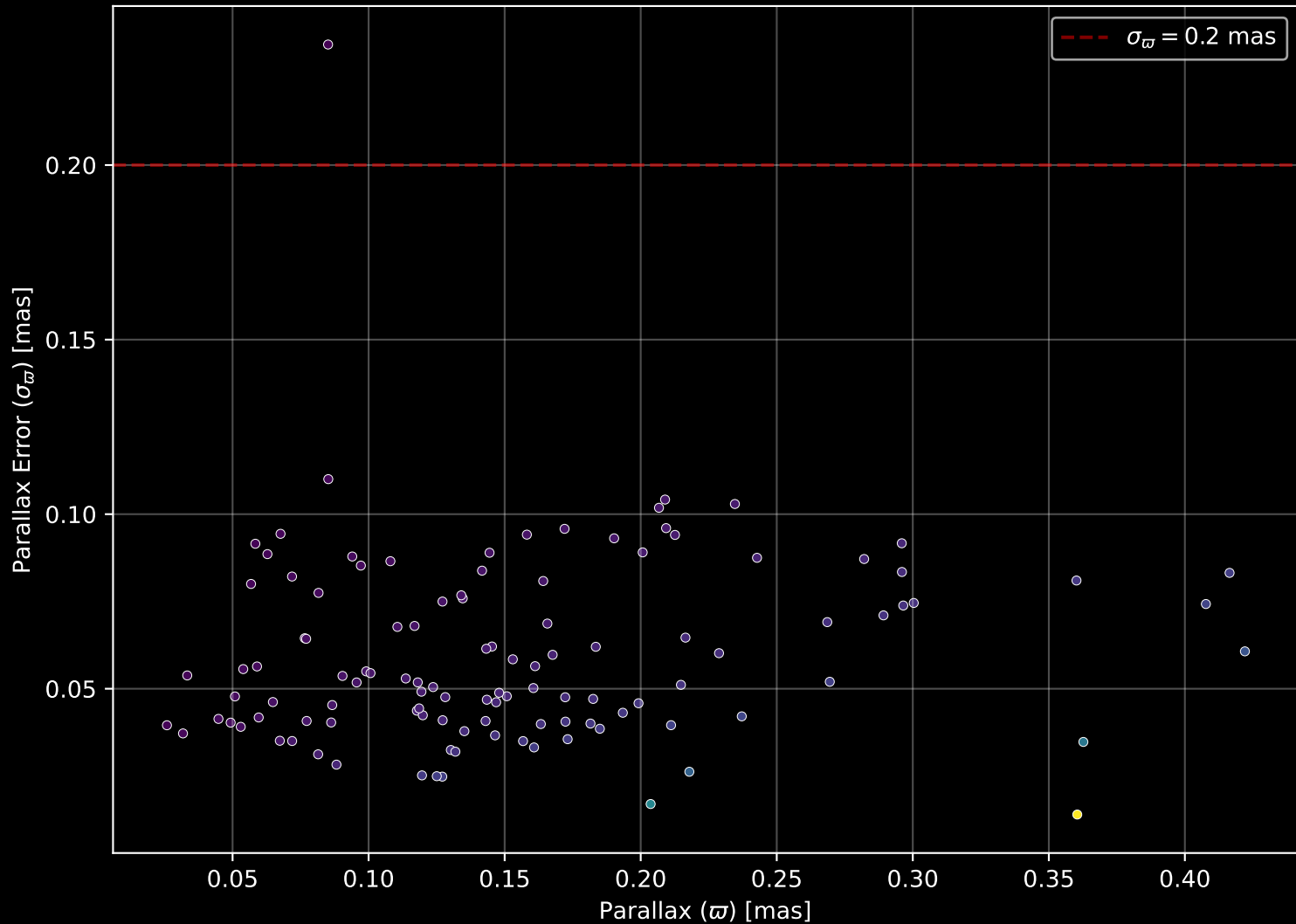
Gaia Cluster: [Berkeley_54] Parallax Quality (n= 114)
