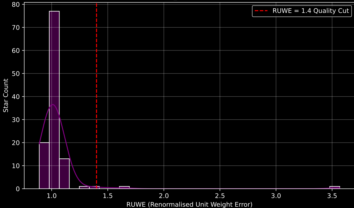
Gaia Cluster: [Berkeley_54] RUWE Distribution (n= 114)
