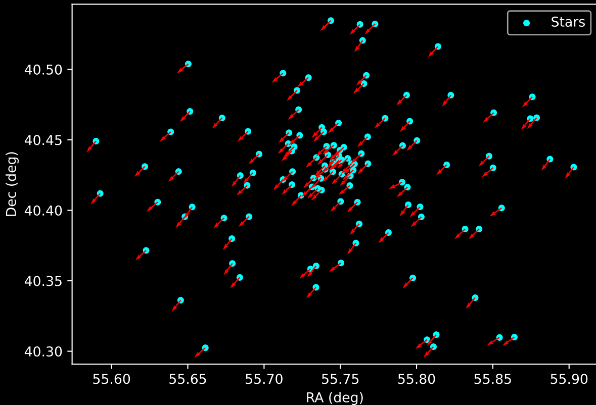
Gaia Cluster: [Berkeley_54] Proper Motion Vectors for Gaia Star Field (n= 114)
