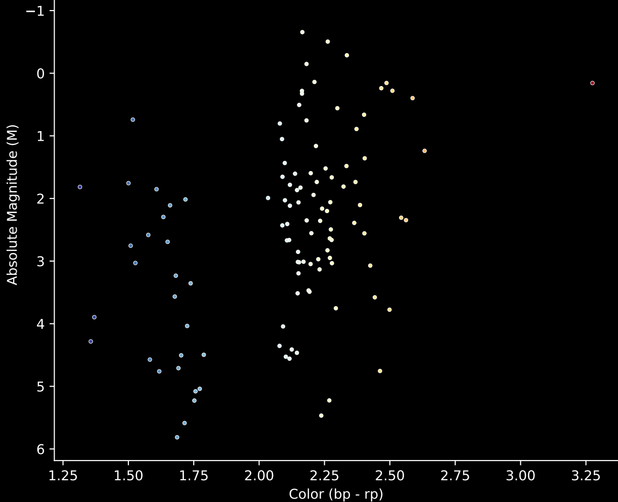
Gaia Cluster: [Berkeley_54] Stars (n= 114) Hertzsprung-Russel Diagram
