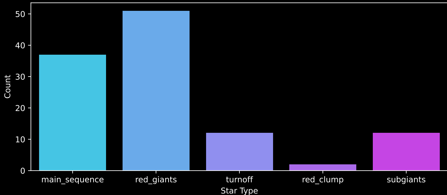
Gaia Cluster: [Berkeley_54] Count plot of Star Type
