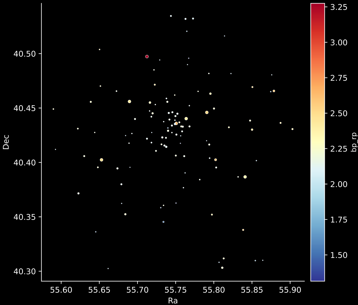
Gaia Cluster: [Berkeley_54] Stars: 114
