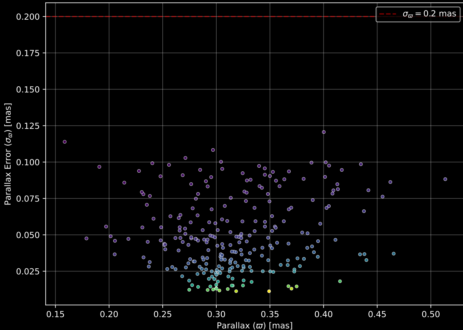
Gaia Cluster: [Berkeley_58] Parallax Quality (n= 258)
