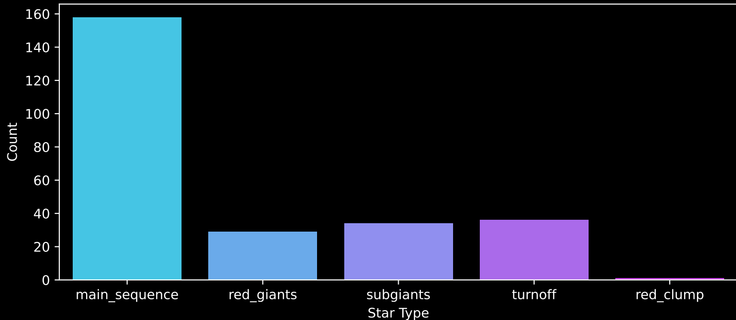
Gaia Cluster: [Berkeley_58] Count plot of Star Type
