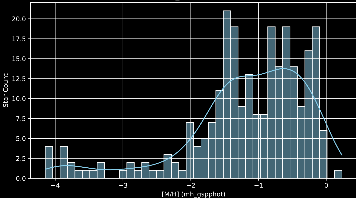
Gaia Cluster: [Berkeley_58 [M/H] (mh_gspphot) (n= 258)
