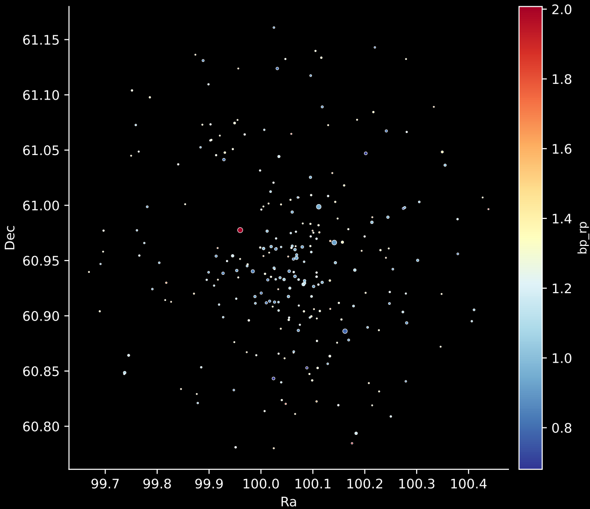
Gaia Cluster: [Berkeley_58] Stars: 258
