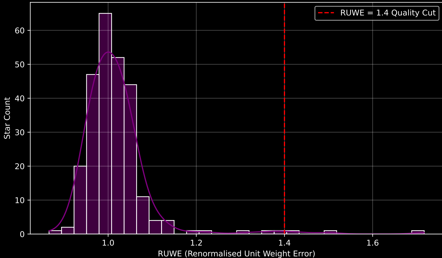
Gaia Cluster: [Berkeley_58] RUWE Distribution (n= 258)
