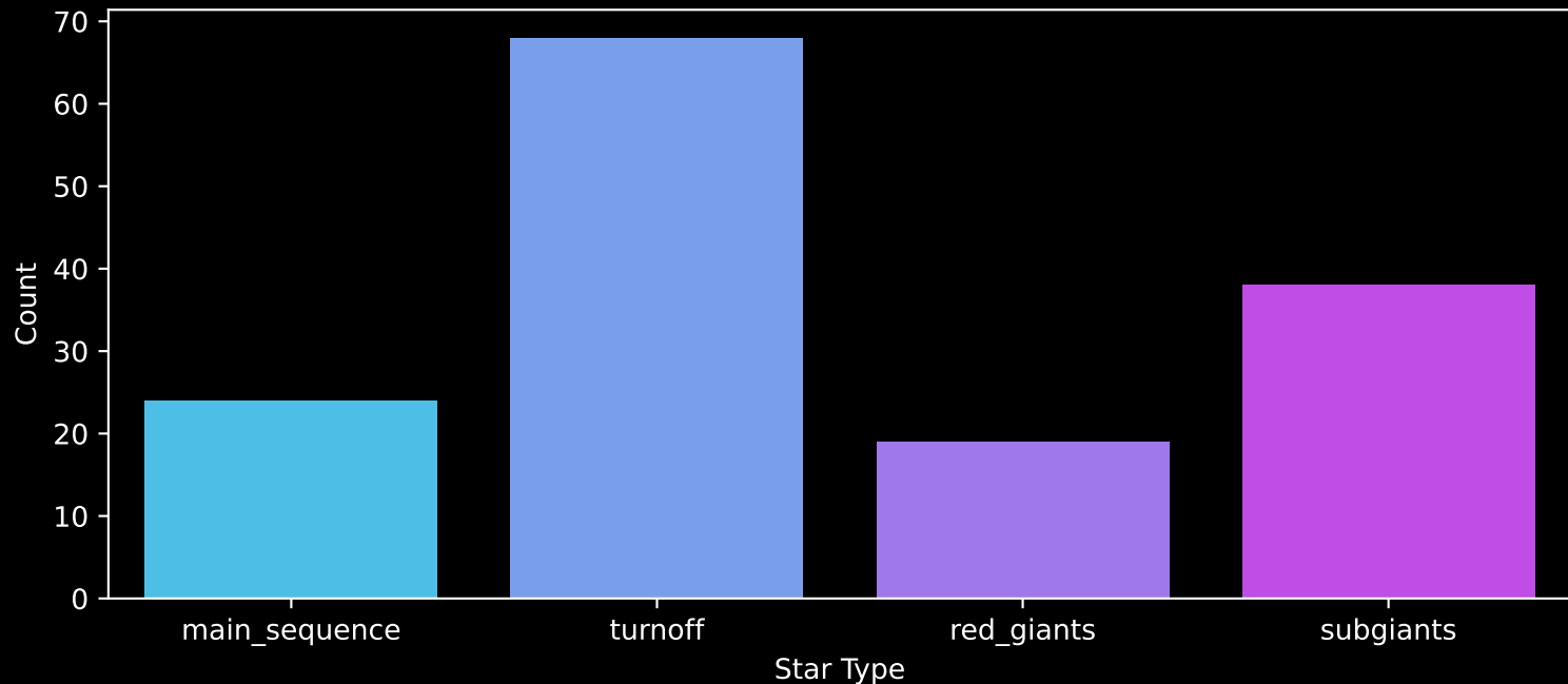
Gaia Cluster: [Berkeley_59] Count plot of Star Type
