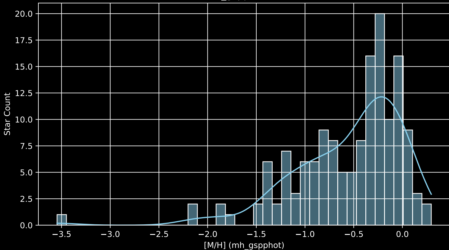
Gaia Cluster: [Berkeley_59 [M/H] (mh_gspphot) (n= 149)
