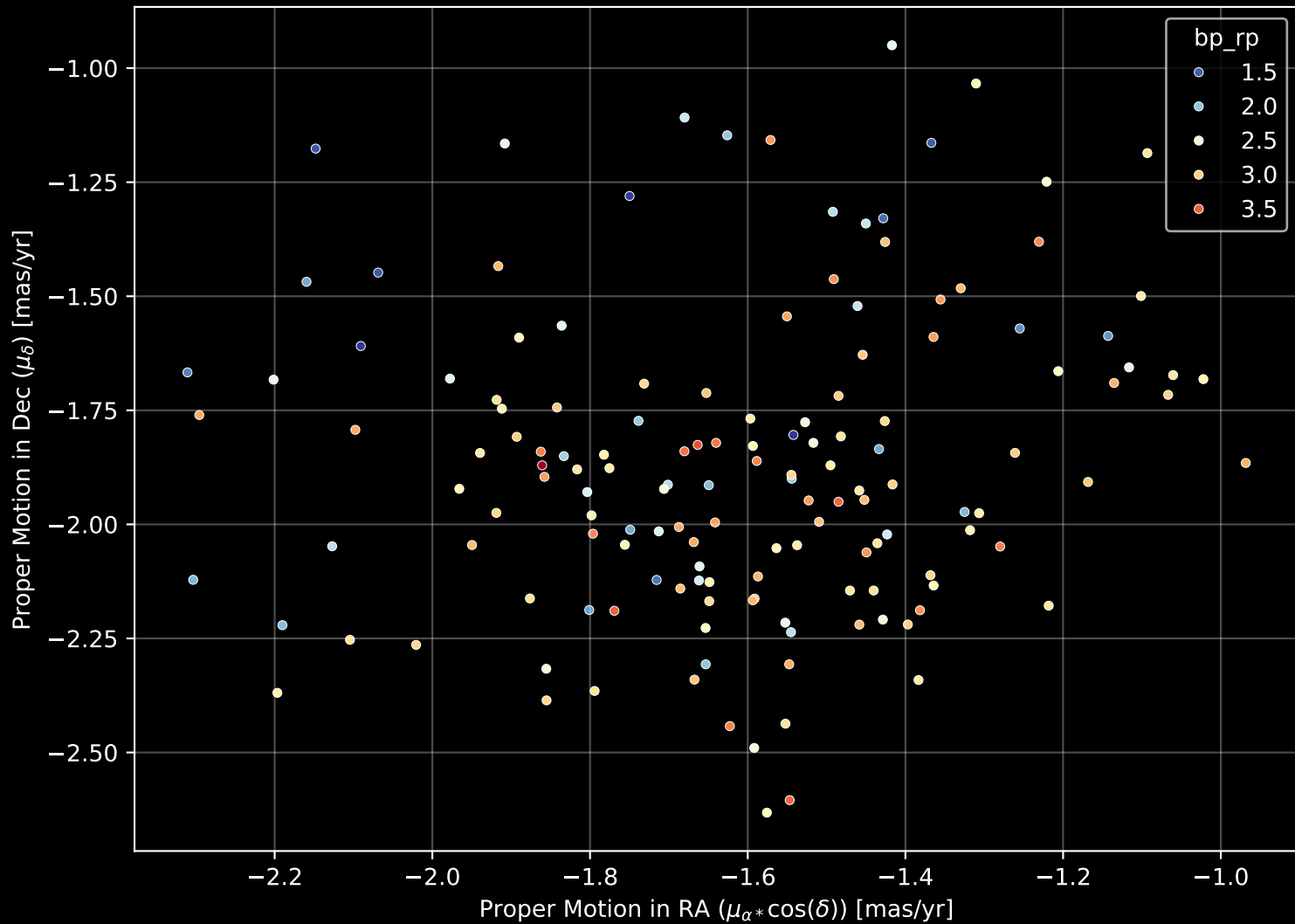
Gaia Cluster: [Berkeley_59] Proper Motion Diagram (n= 149)
