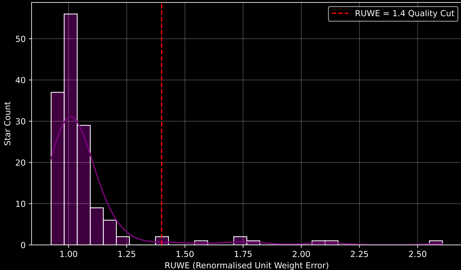
Gaia Cluster: [Berkeley_59] RUWE Distribution (n= 148)
