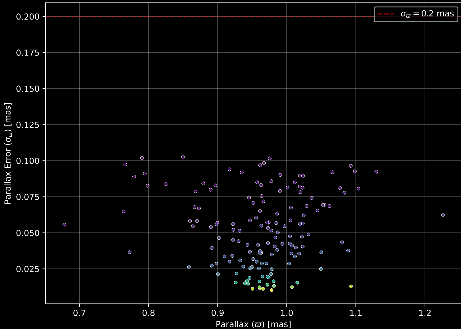
Gaia Cluster: [Berkeley_59] Parallax Quality (n= 149)
