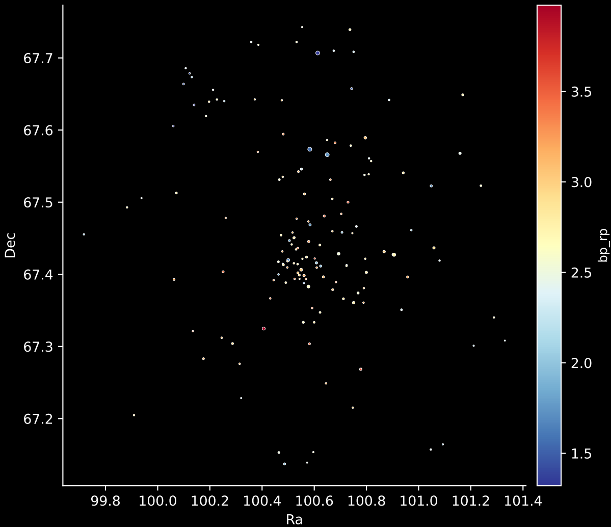
Gaia Cluster: [Berkeley_59] Stars: 149
