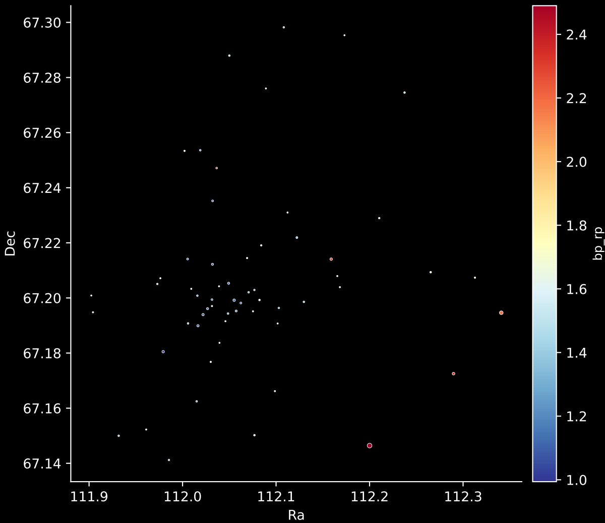
Gaia Cluster: [Berkeley_61] Stars: 59
