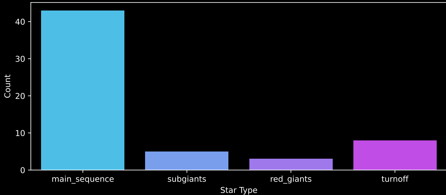
Gaia Cluster: [Berkeley_61] Count plot of Star Type
