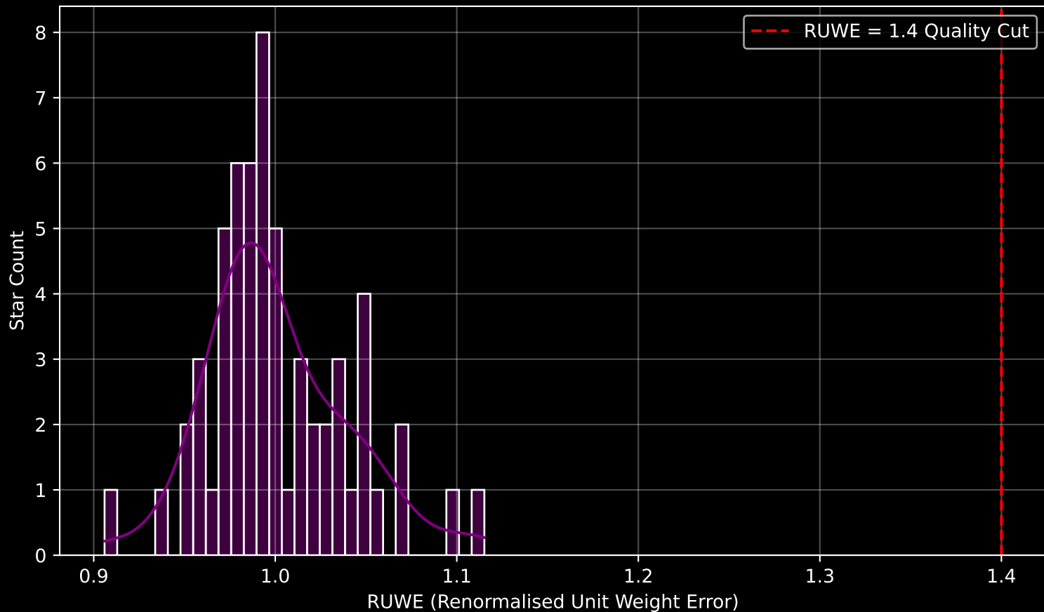
Gaia Cluster: [Berkeley_61] RUWE Distribution (n= 59)
