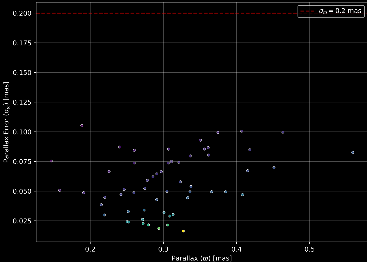
Gaia Cluster: [Berkeley_61] Parallax Quality (n= 59)
