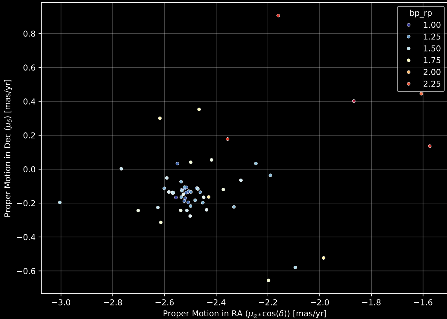
Gaia Cluster: [Berkeley_61] Proper Motion Diagram (n= 59)
