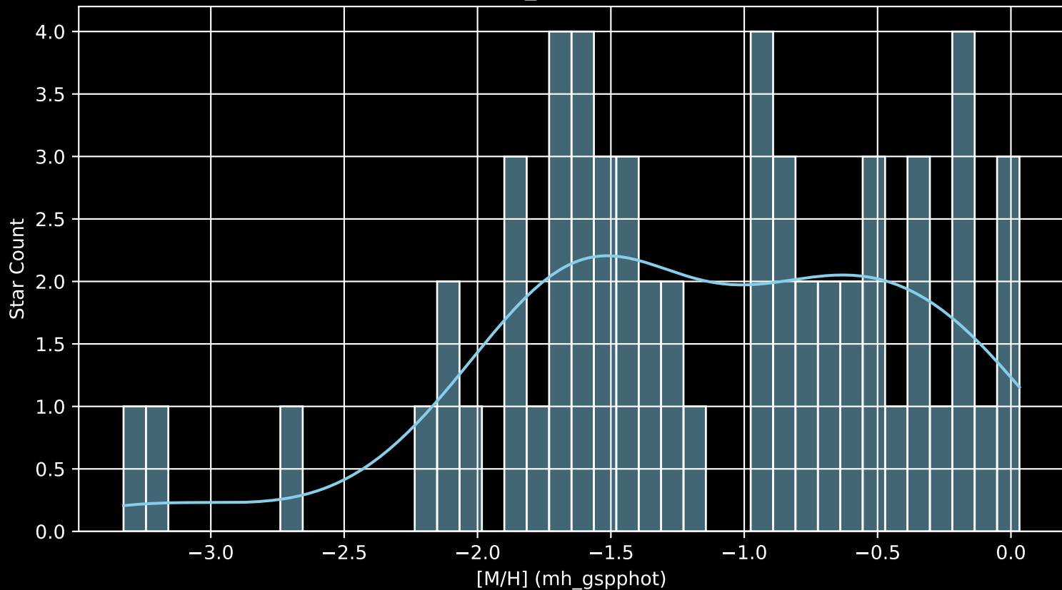
Gaia Cluster: [Berkeley_61 [M/H] (mh_gspphot) (n= 59)
