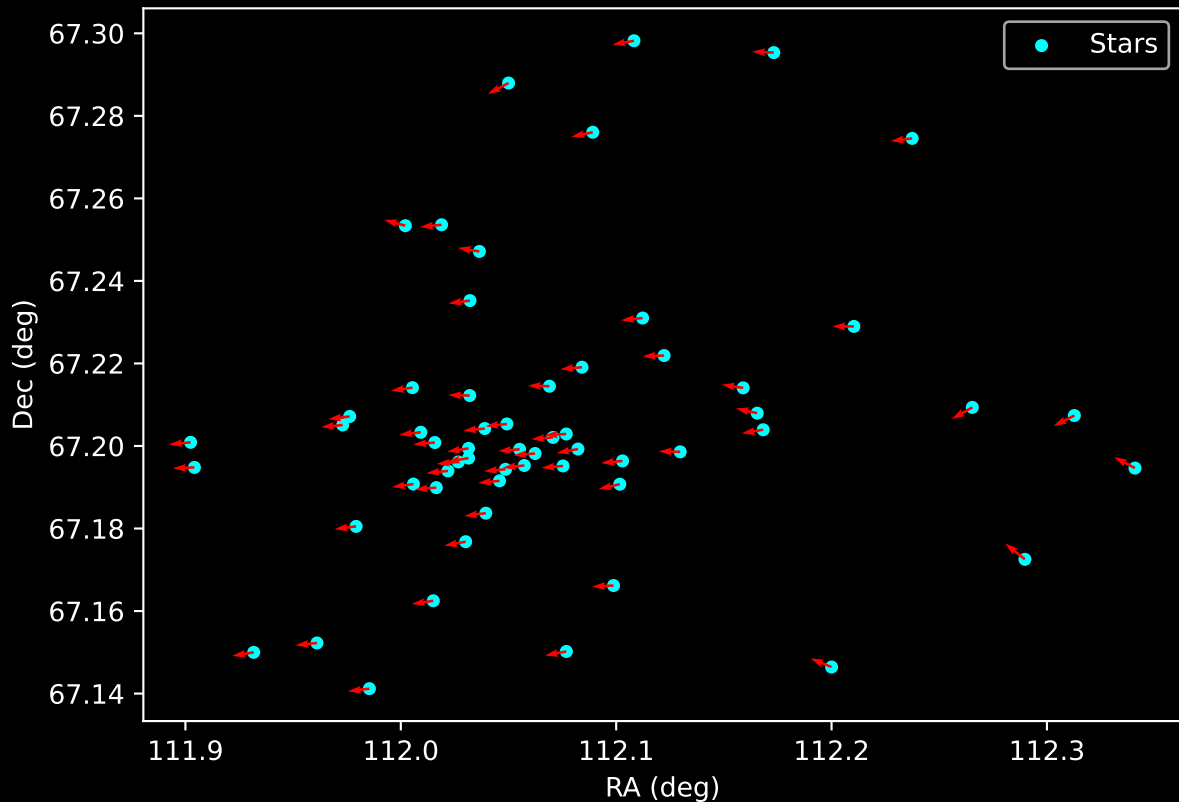
Gaia Cluster: [Berkeley_61] Proper Motion Vectors for Gaia Star Field (n= 59)
