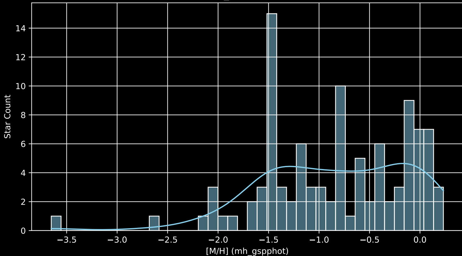
Gaia Cluster: [Berkeley_63 [M/H] (mh_gspphot) (n= 102)
