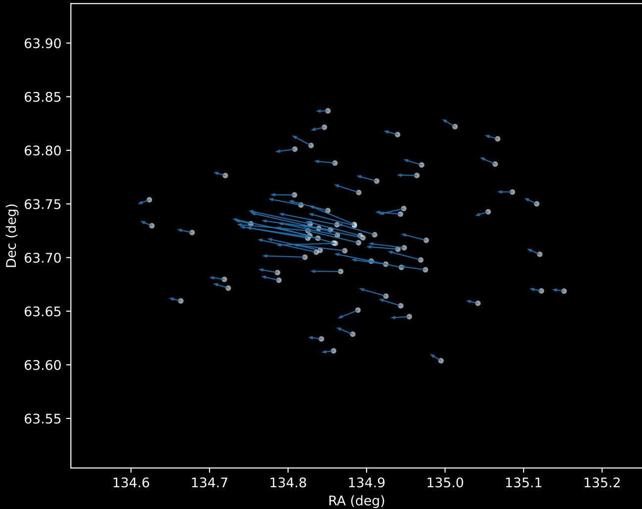
Gaia DR3 Cluster 0 Proper Motion Vectors (n=73)
