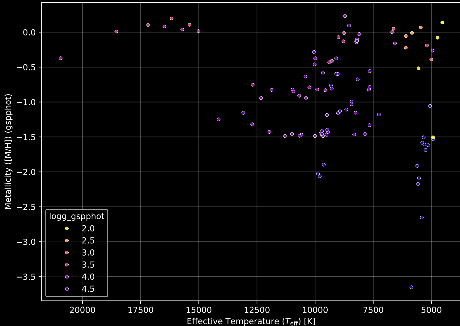
Gaia Cluster: [Berkeley_63] Stellar Population Parameters (n= 102)
