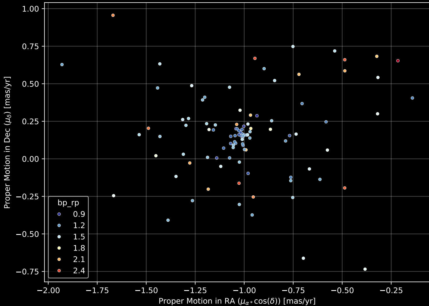
Gaia Cluster: [Berkeley_63] Proper Motion Diagram (n= 102)
