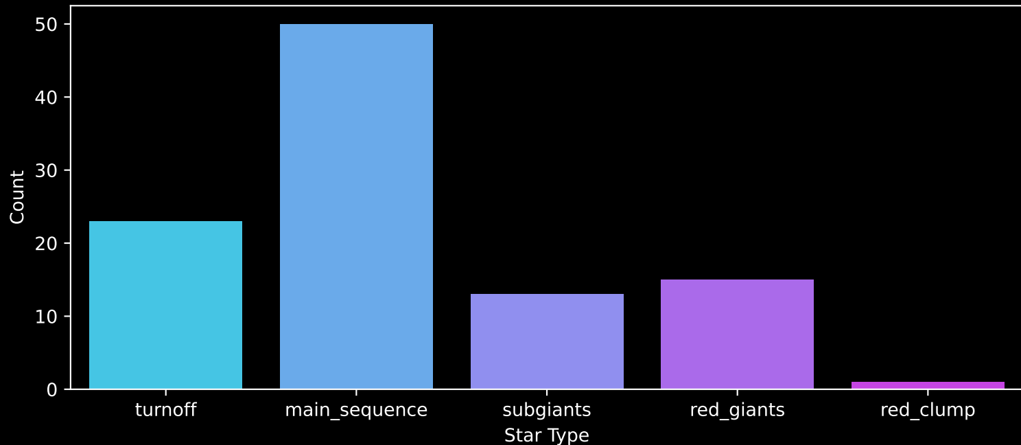
Gaia Cluster: [Berkeley_63] Count plot of Star Type
