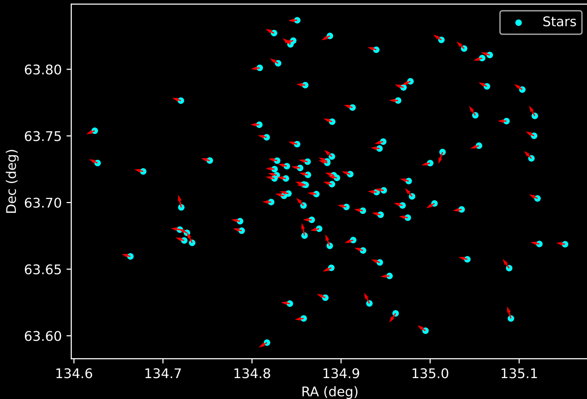
Gaia Cluster: [Berkeley_63] Proper Motion Vectors for Gaia Star Field (n= 102)
