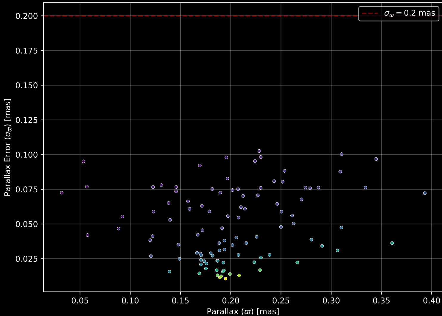
Gaia Cluster: [Berkeley_63] Parallax Quality (n= 102)
