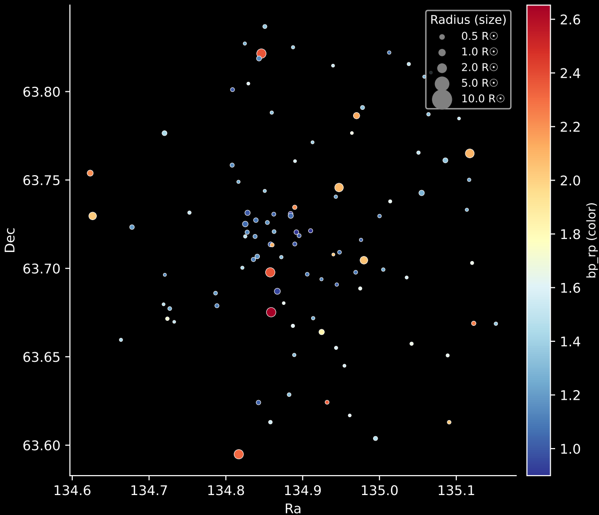
Gaia Cluster: [Berkeley_63] Stars: 102
