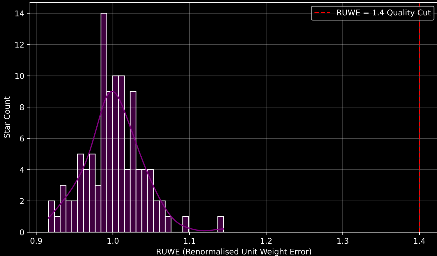
Gaia Cluster: [Berkeley_63] RUWE Distribution (n= 102)
