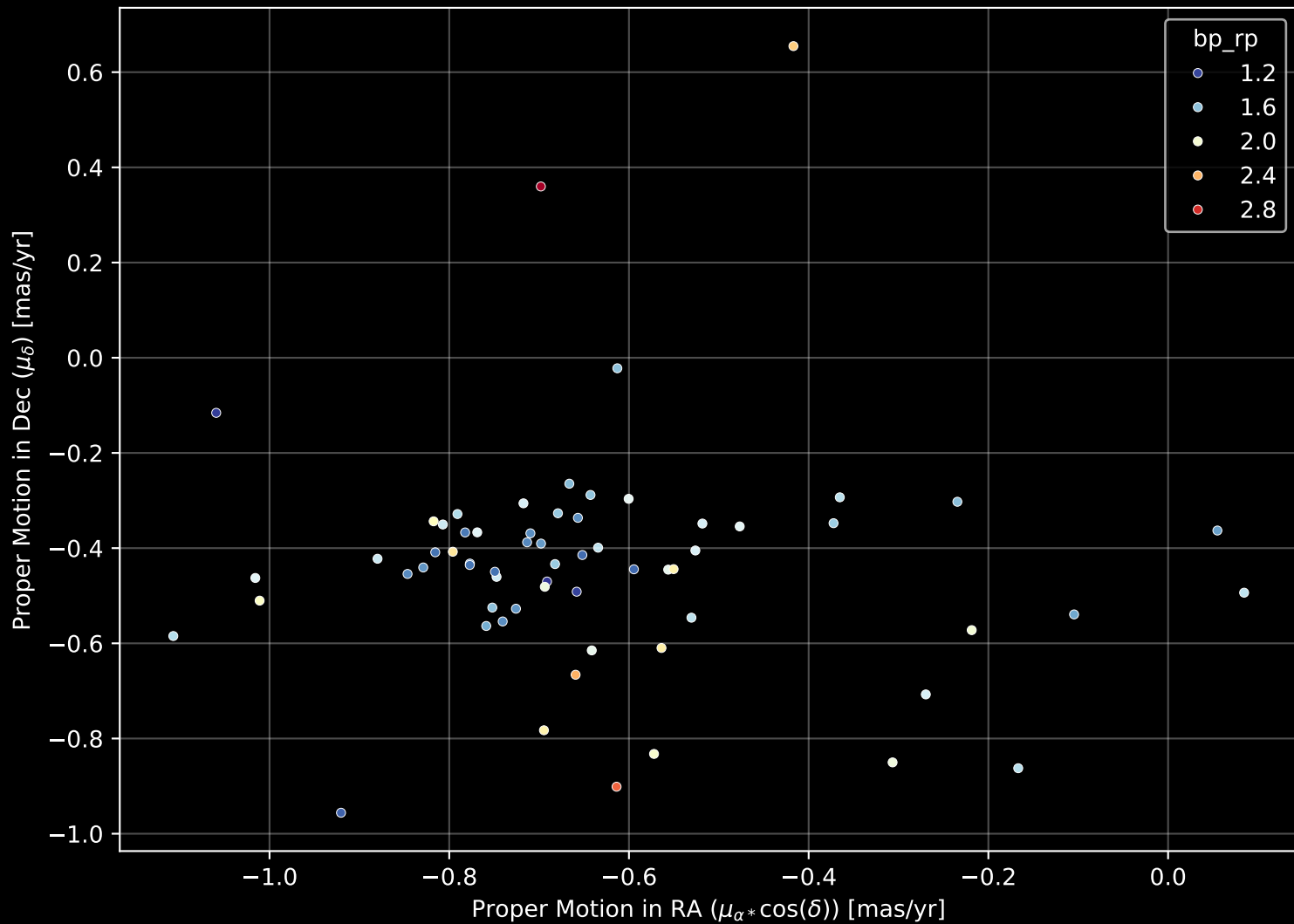
Gaia Cluster: [Berkeley_65] Proper Motion Diagram (n= 64)
