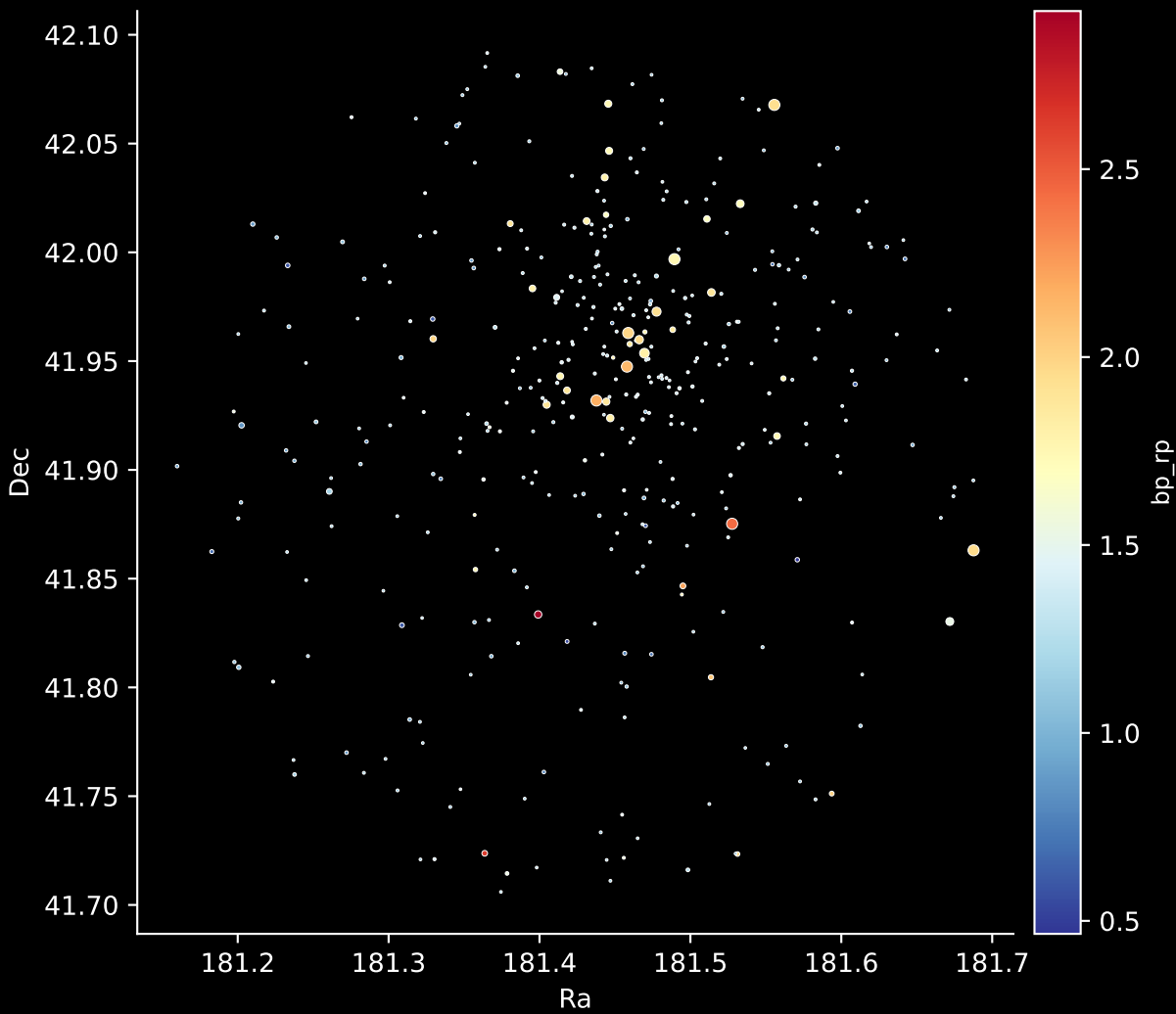
Gaia Cluster: [Berkeley_70] Stars: 399
