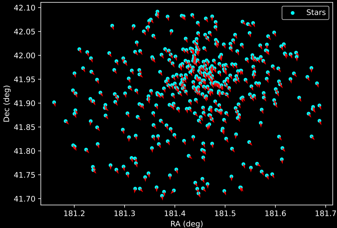
Gaia Cluster: [Berkeley_70] Proper Motion Vectors for Gaia Star Field (n= 399)
