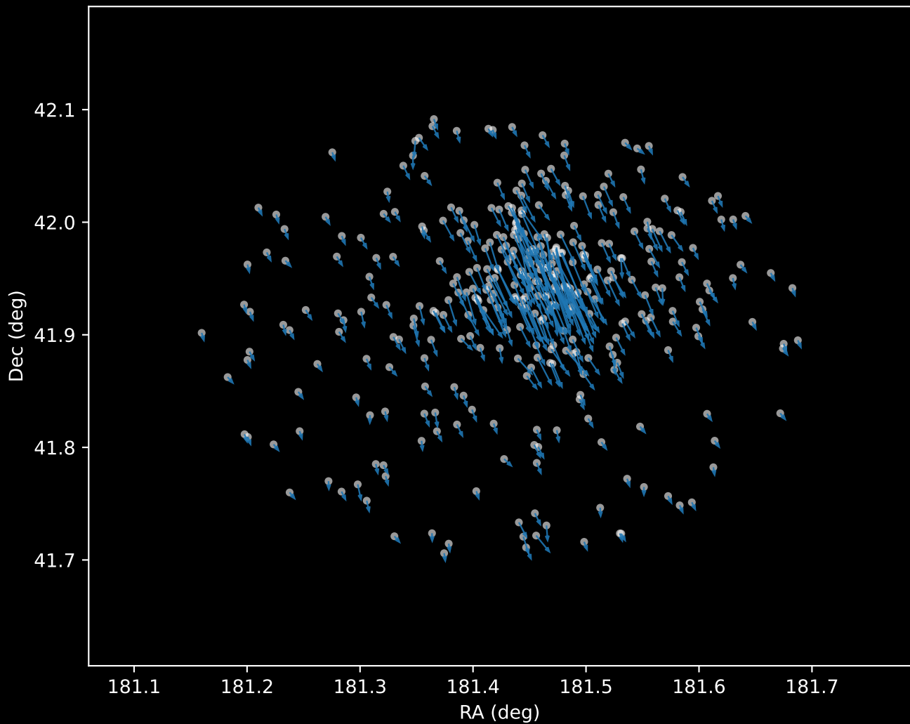
Gaia DR3 Cluster 0 Proper Motion Vectors (n=354)
