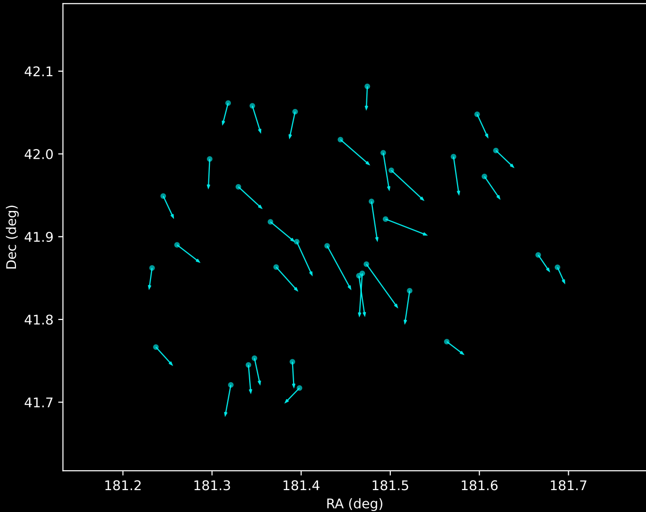
Gaia DR3 Noise Stream Proper Motion Vectors (n=35)
