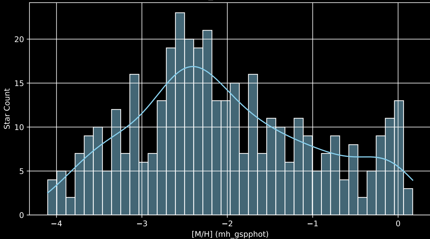
Gaia Cluster: [Berkeley_70 [M/H] (mh_gspphot) (n= 399)
