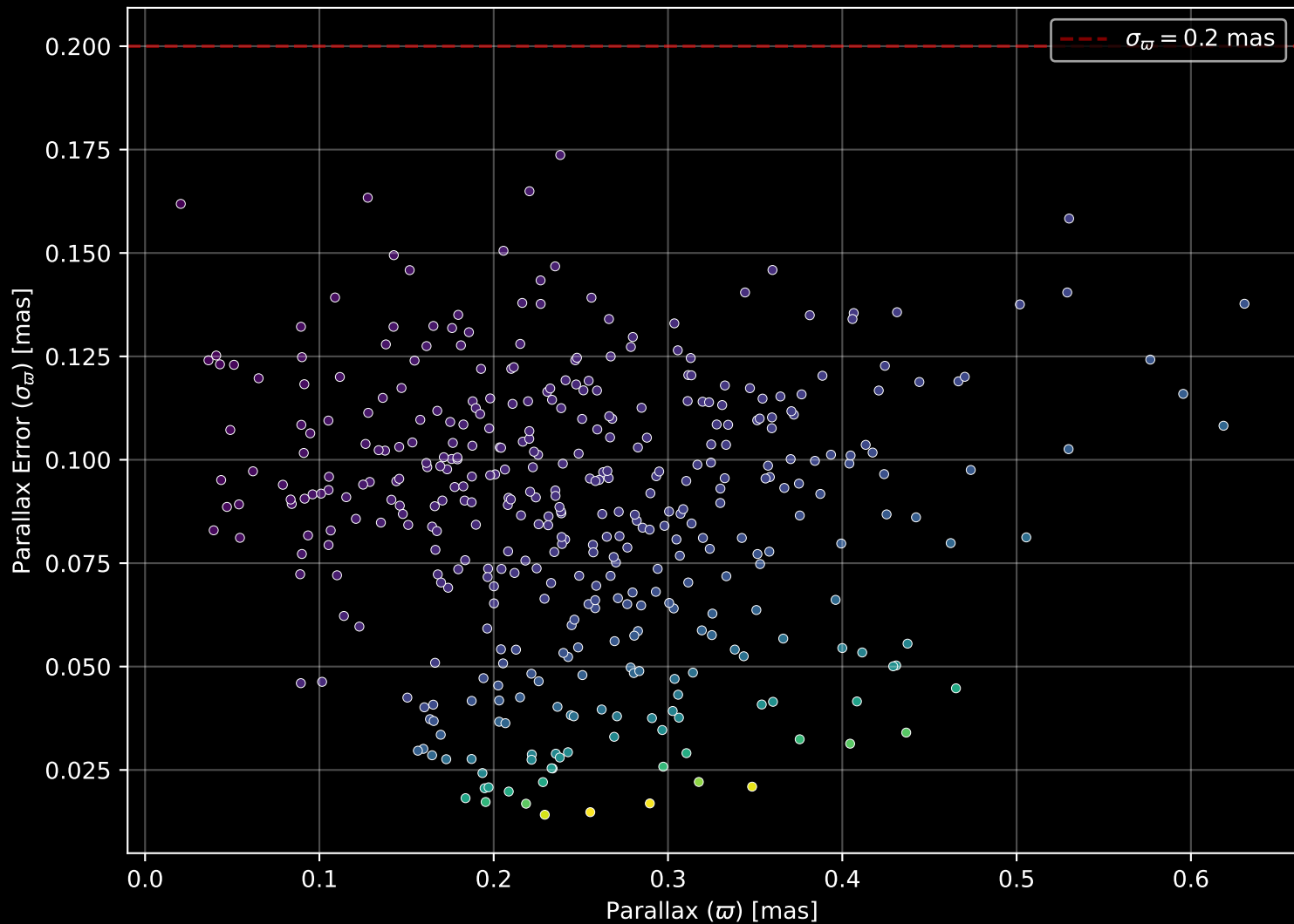
Gaia Cluster: [Berkeley_70] Parallax Quality (n= 399)
