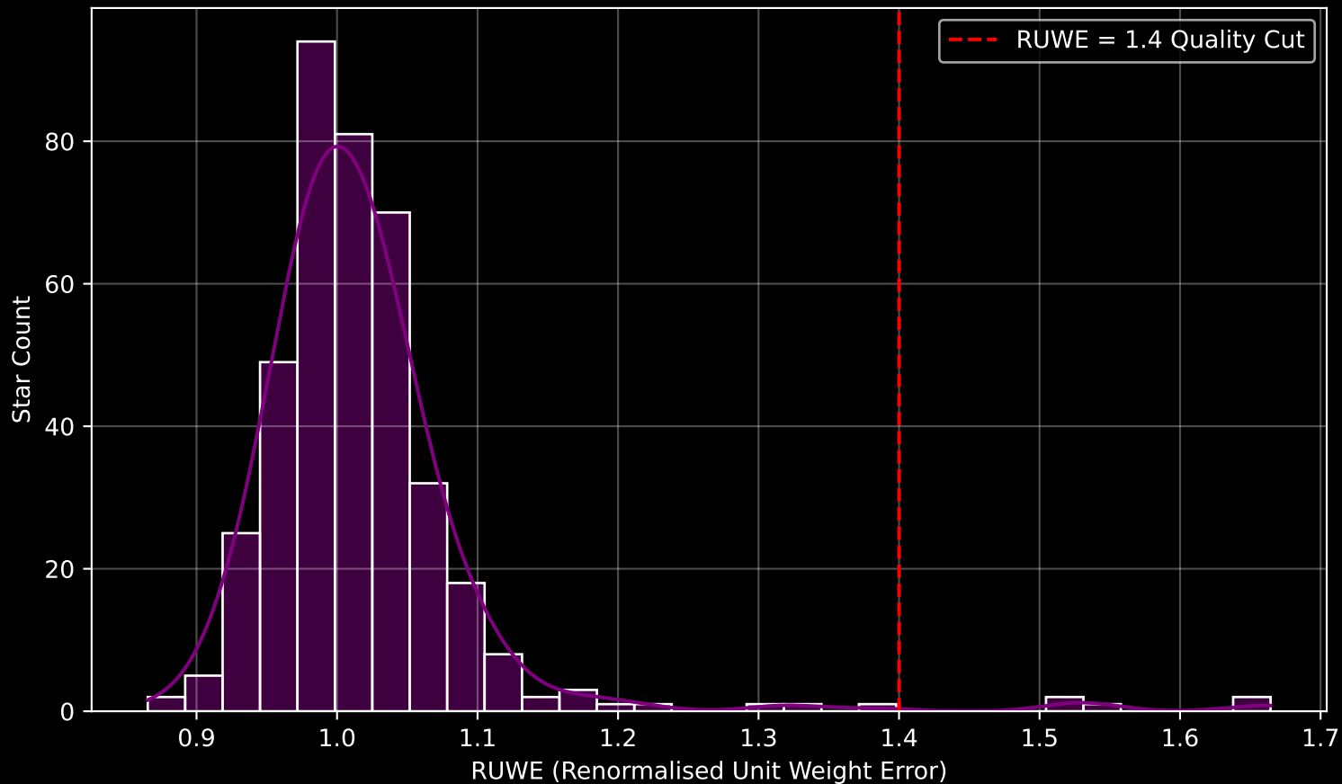
Gaia Cluster: [Berkeley_70] RUWE Distribution (n= 399)
