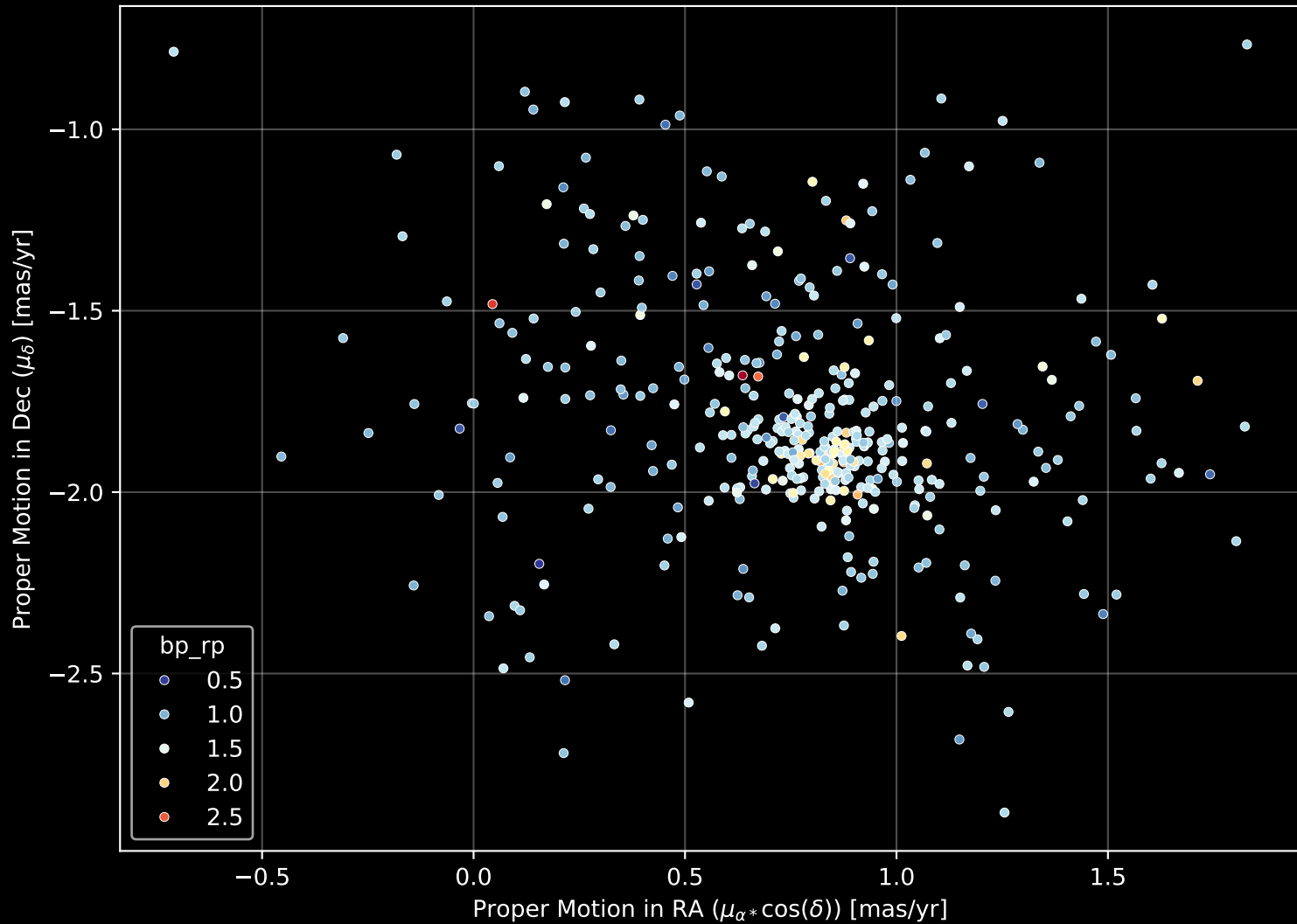
Gaia Cluster: [Berkeley_70] Proper Motion Diagram (n= 399)
