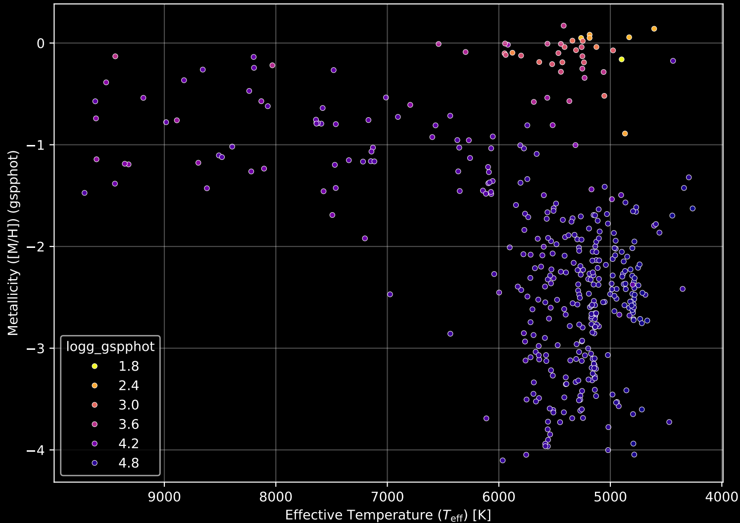
Gaia Cluster: [Berkeley_70] Stellar Population Parameters (n= 399)
