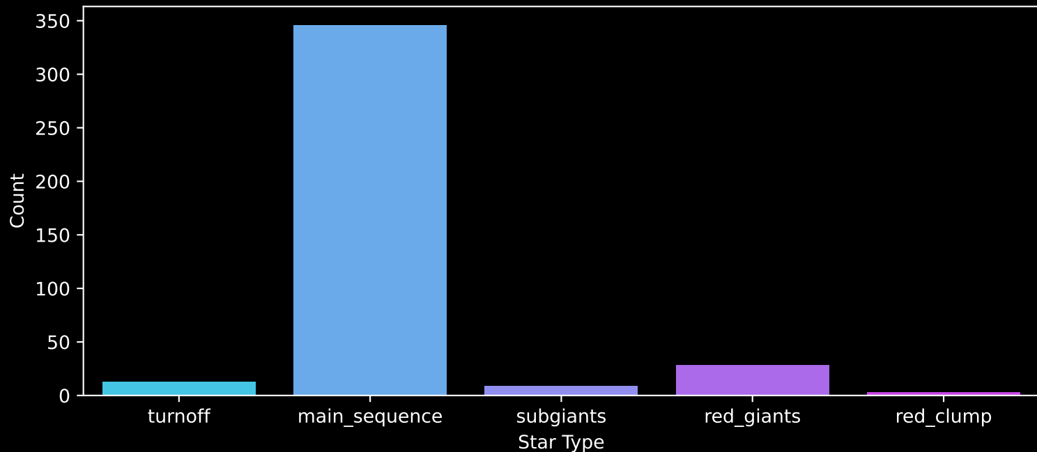
Gaia Cluster: [Berkeley_70] Count plot of Star Type
