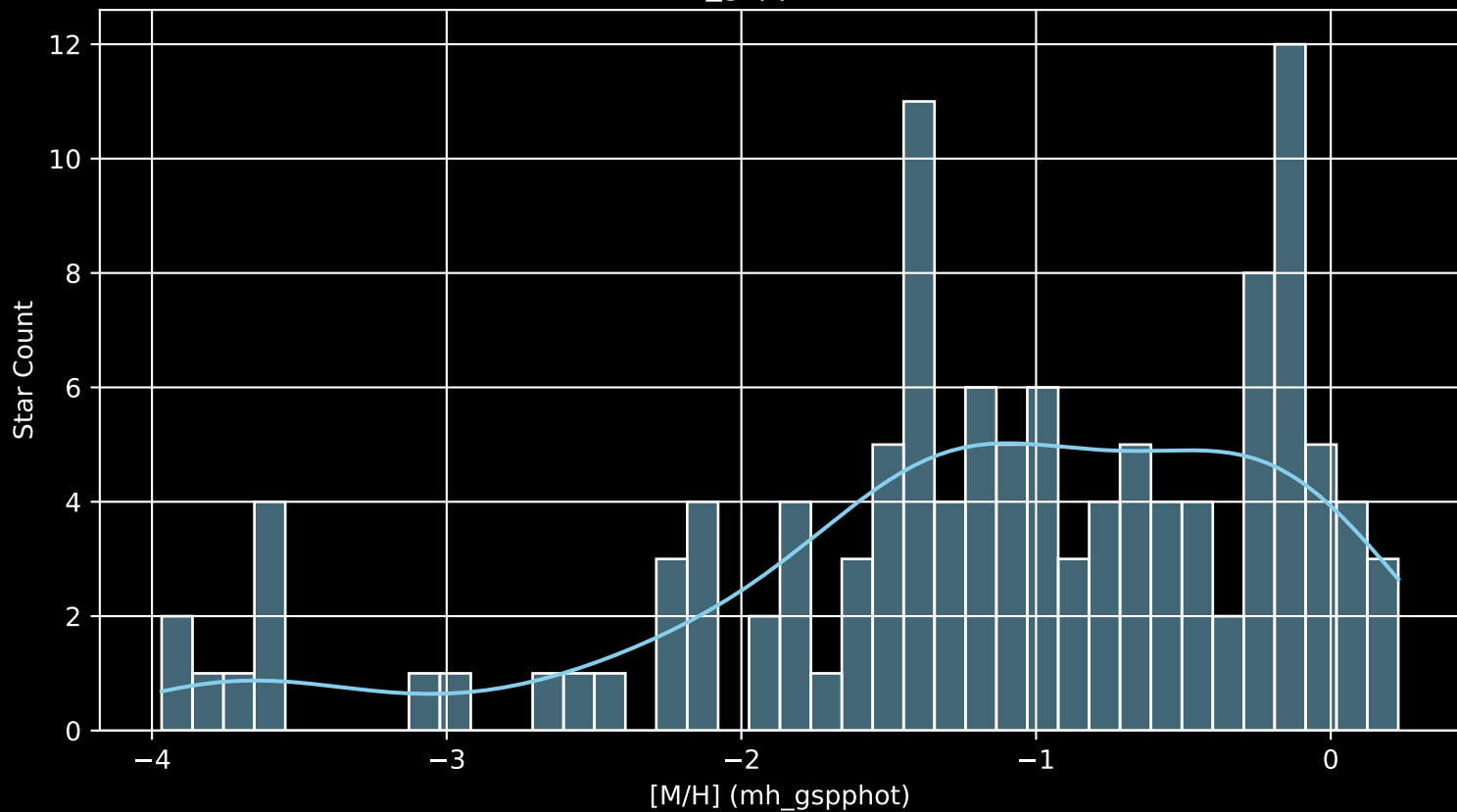
Gaia Cluster: [Berkeley_71 [M/H] (mh_gspphot) (n= 121)
