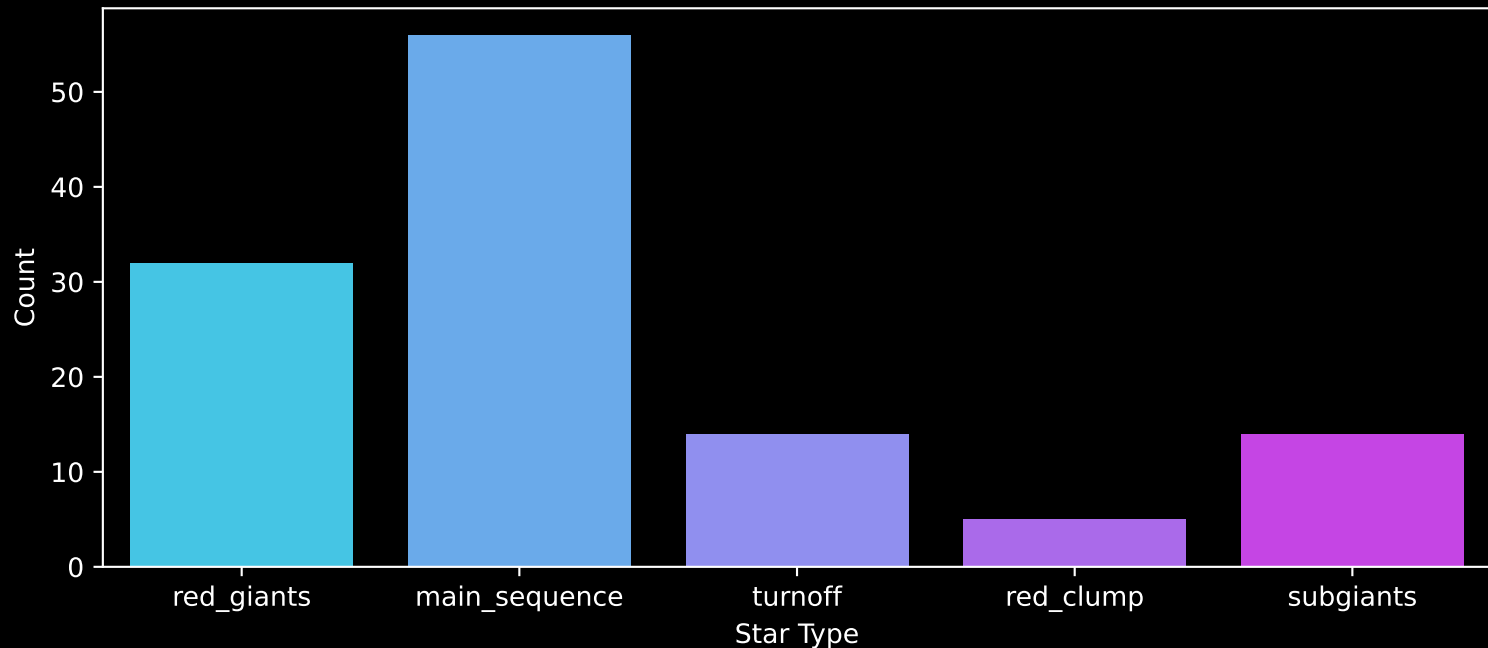
Gaia Cluster: [Berkeley_71] Count plot of Star Type
