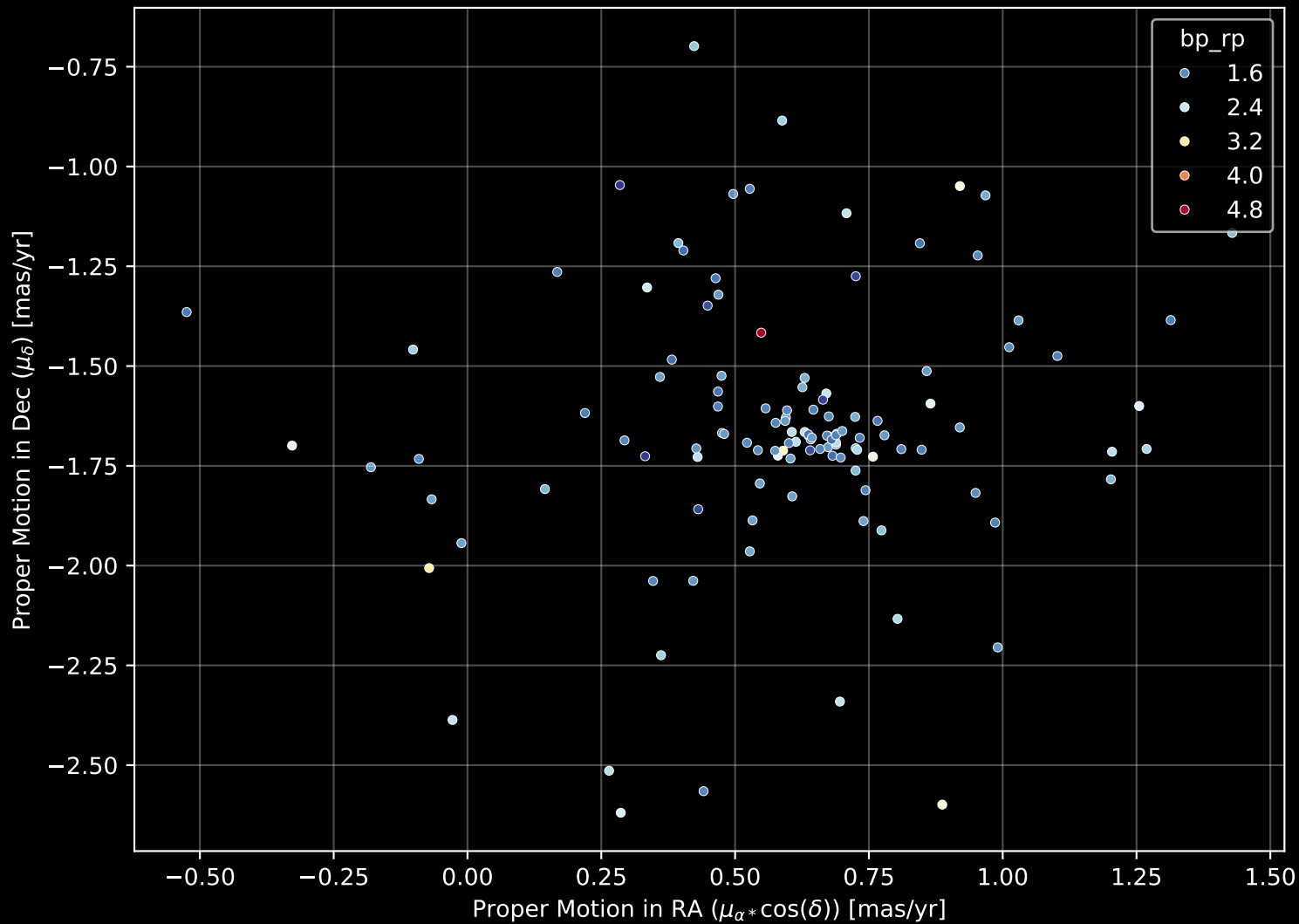
Gaia Cluster: [Berkeley_71] Proper Motion Diagram (n= 121)
