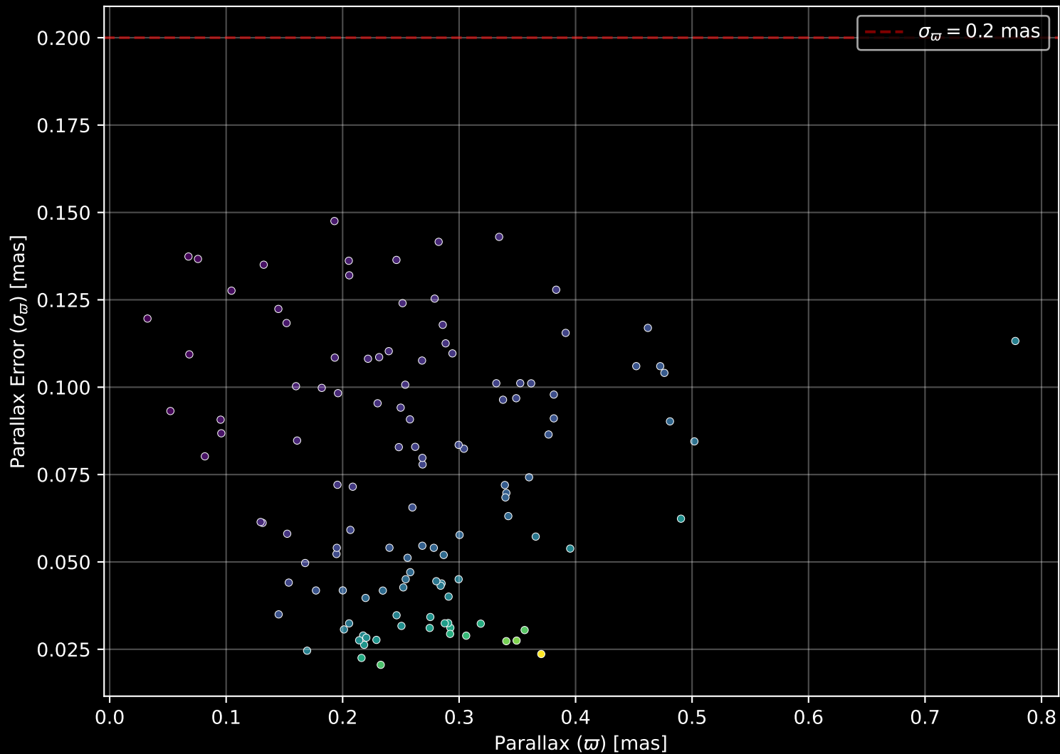
Gaia Cluster: [Berkeley_71] Parallax Quality (n= 121)
