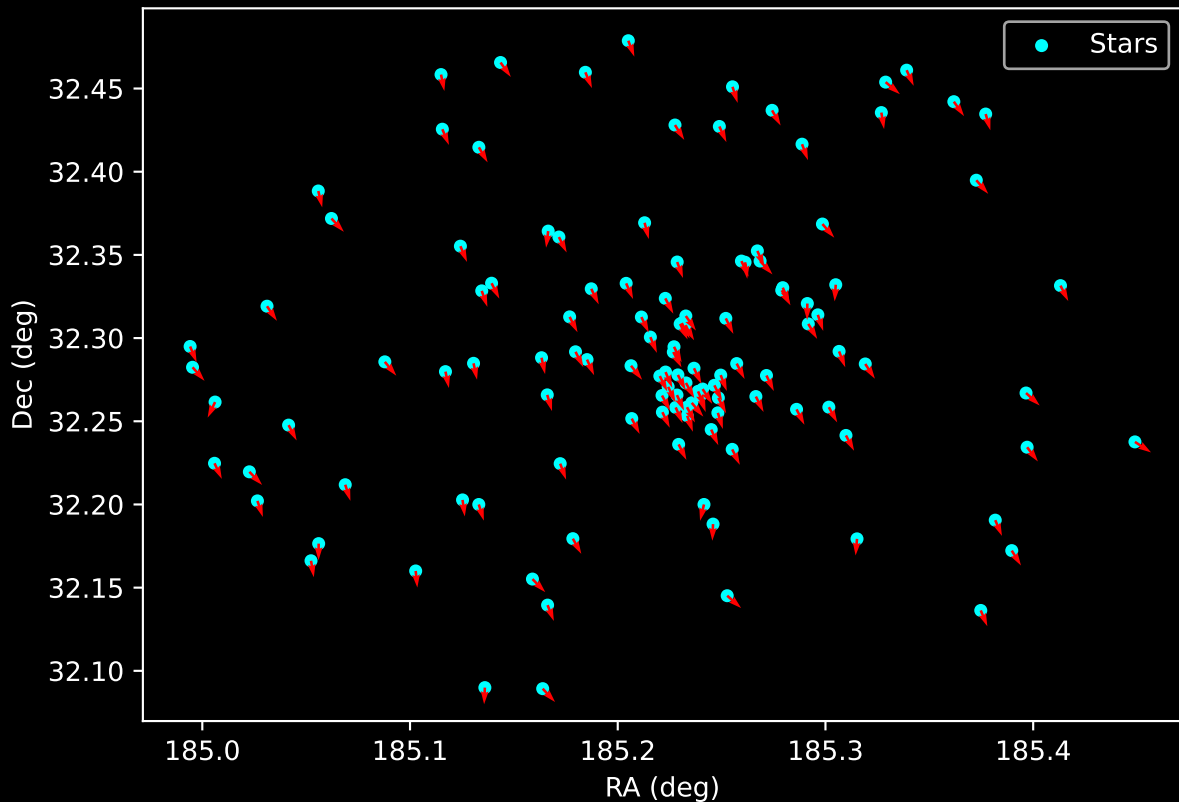
Gaia Cluster: [Berkeley_71] Proper Motion Vectors for Gaia Star Field (n= 121)
