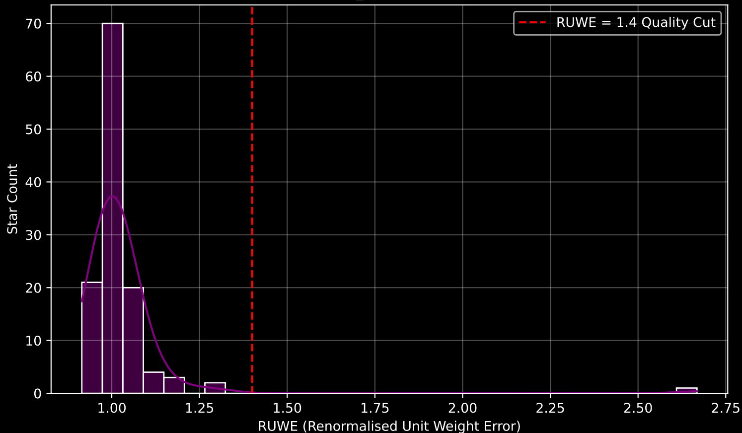
Gaia Cluster: [Berkeley_71] RUWE Distribution (n= 121)
