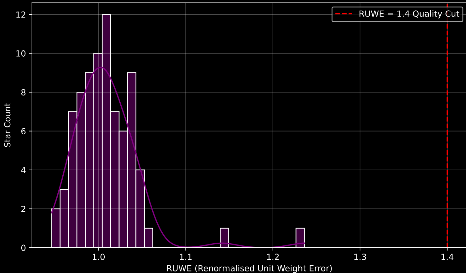
Gaia Cluster: [Berkeley_75] RUWE Distribution (n= 80)
