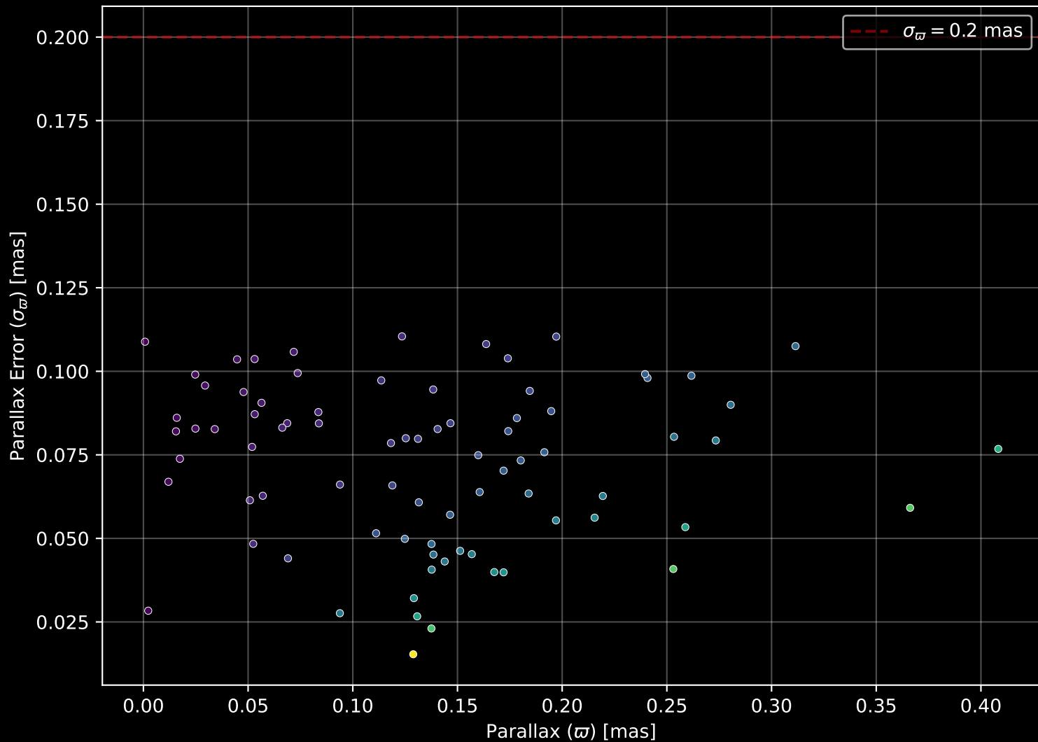
Gaia Cluster: [Berkeley_75] Parallax Quality (n= 80)
