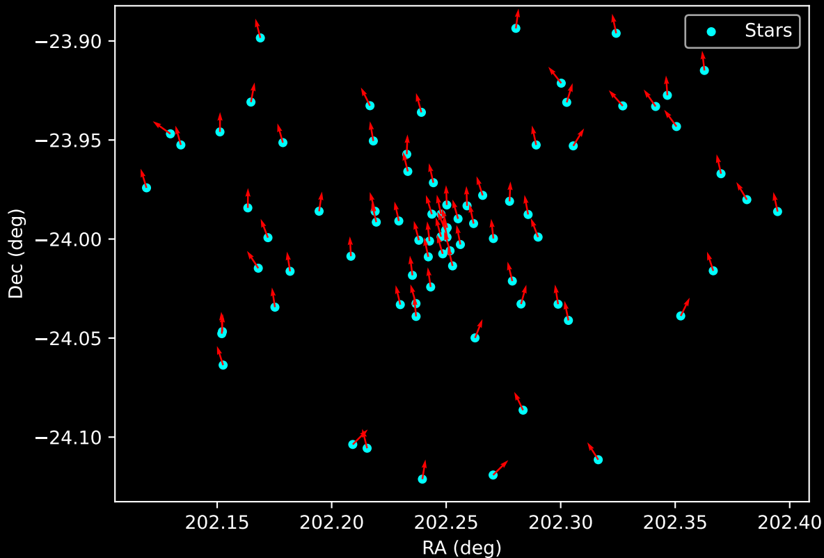
Gaia Cluster: [Berkeley_75] Proper Motion Vectors for Gaia Star Field (n= 80)
