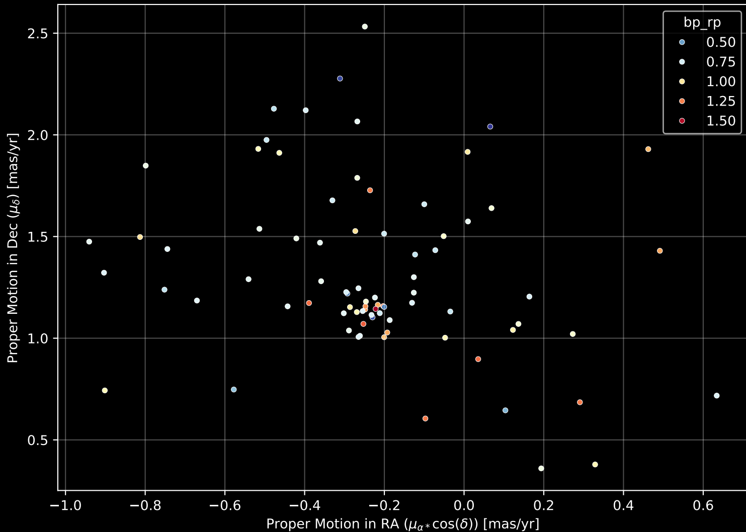
Gaia Cluster: [Berkeley_75] Proper Motion Diagram (n= 80)
