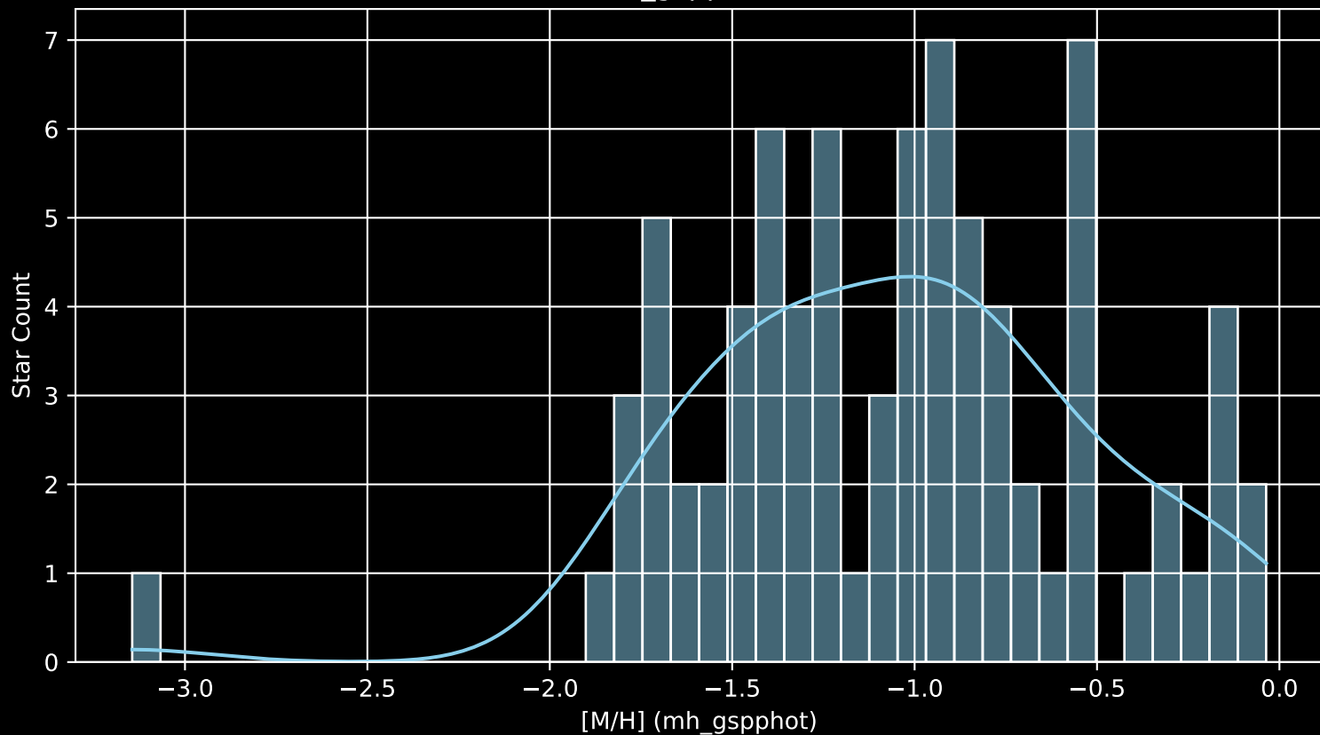
Gaia Cluster: [Berkeley_75 [M/H] (mh_gspphot) (n= 80)
