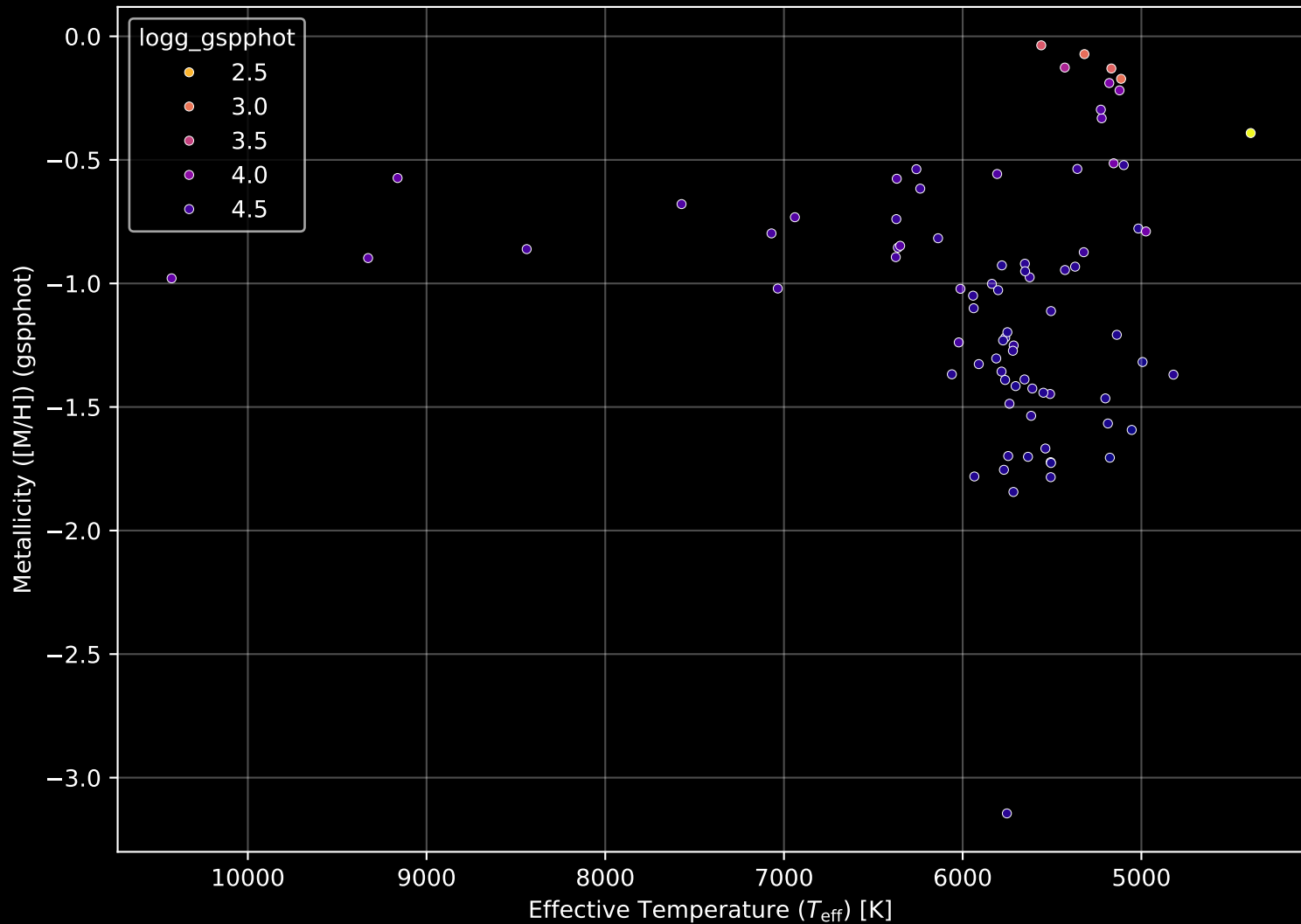
Gaia Cluster: [Berkeley_75] Stellar Population Parameters (n= 80)
