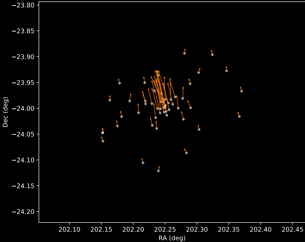
Gaia DR3 Cluster 2 Proper Motion Vectors (n=52)
