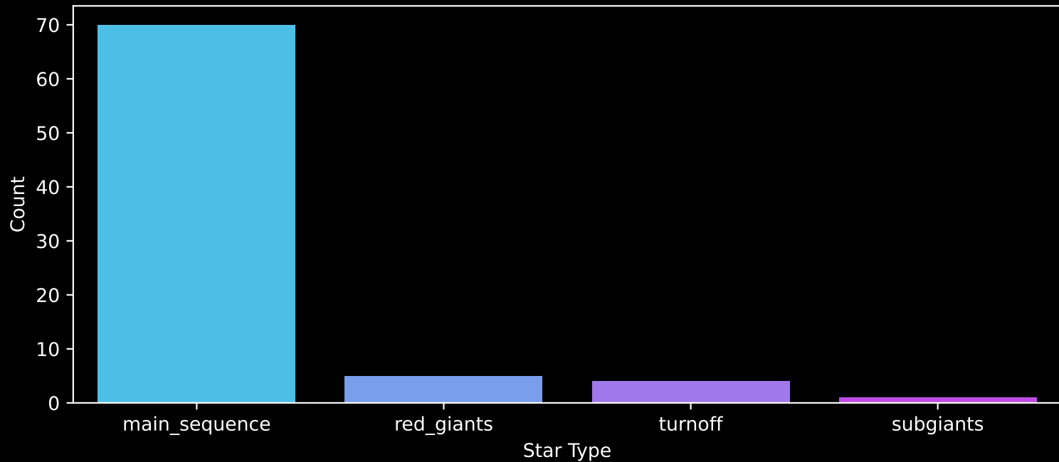
Gaia Cluster: [Berkeley_75] Count plot of Star Type
