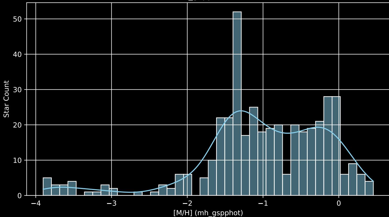
Gaia Cluster: [Berkeley_79 [M/H] (mh_gspphot) (n= 416)
