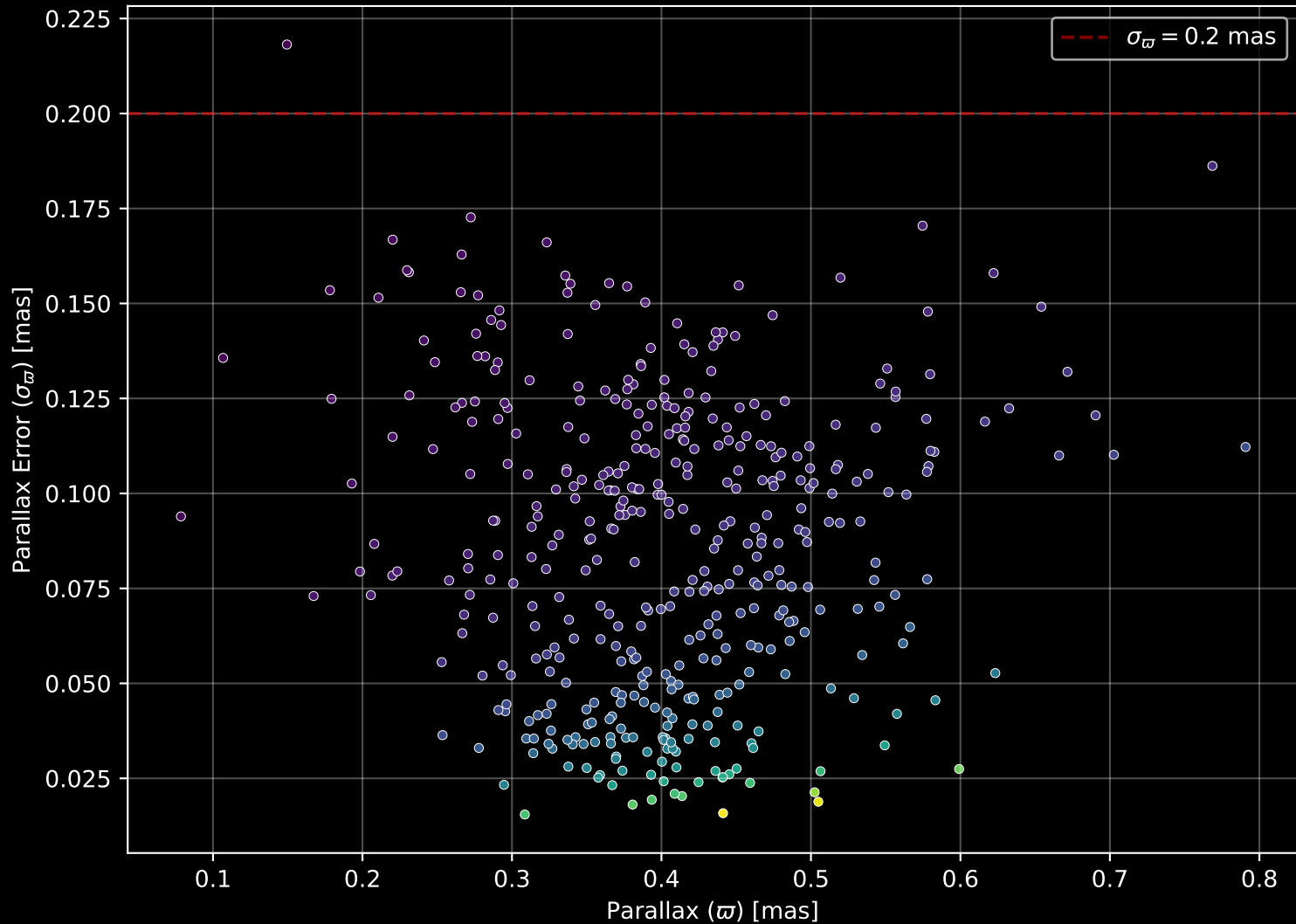
Gaia Cluster: [Berkeley_79] Parallax Quality (n= 419)
