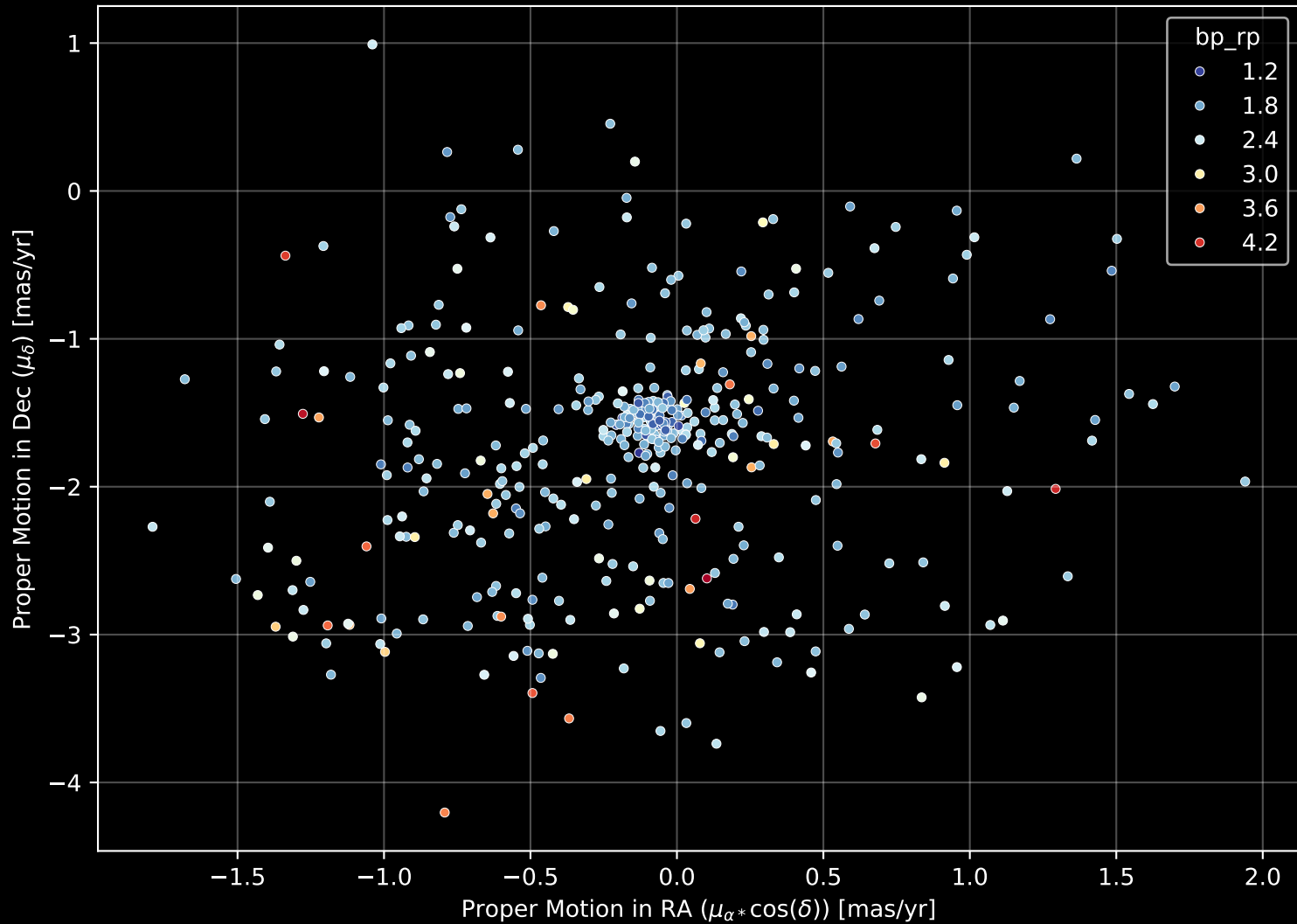
Gaia Cluster: [Berkeley_79] Proper Motion Diagram (n= 419)
