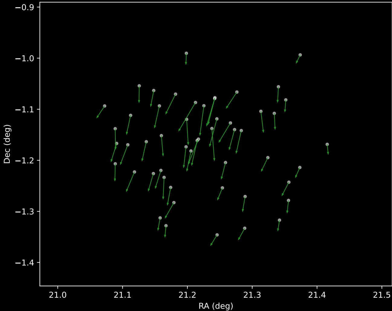
Gaia DR3 Cluster 4 Proper Motion Vectors (n=52)
