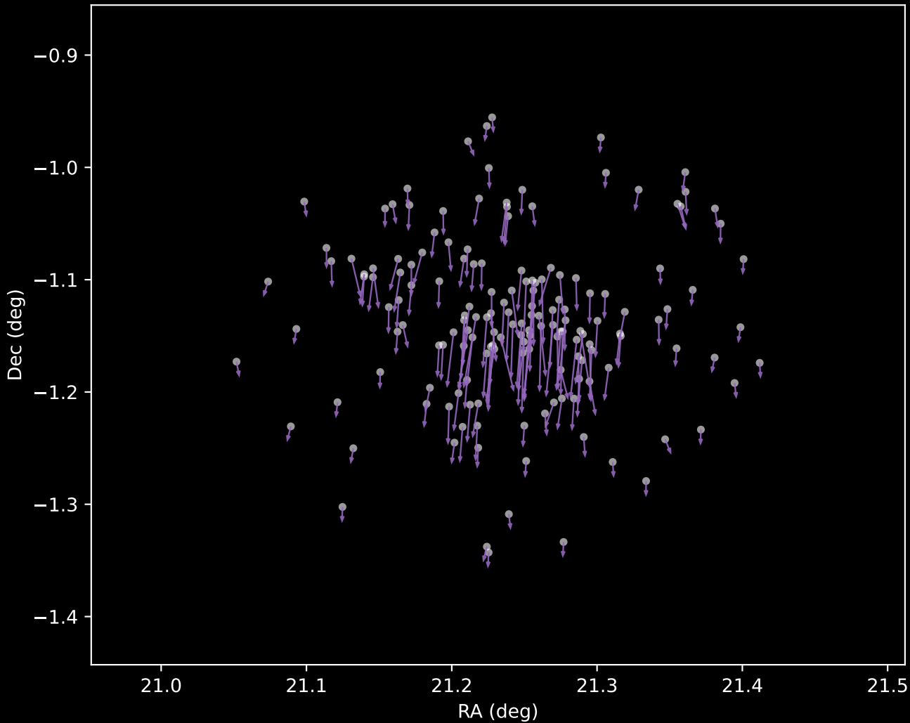
Gaia DR3 Cluster 8 Proper Motion Vectors (n=160)
