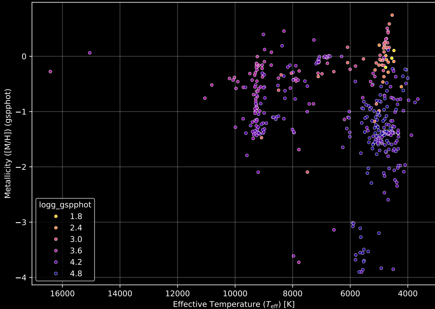
Gaia Cluster: [Berkeley_79] Stellar Population Parameters (n= 419)
