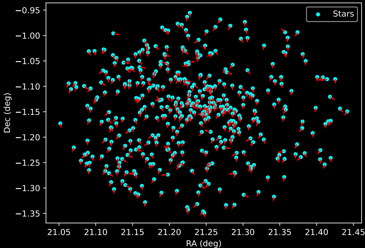
Gaia Cluster: [Berkeley_79] Proper Motion Vectors for Gaia Star Field (n= 419)
