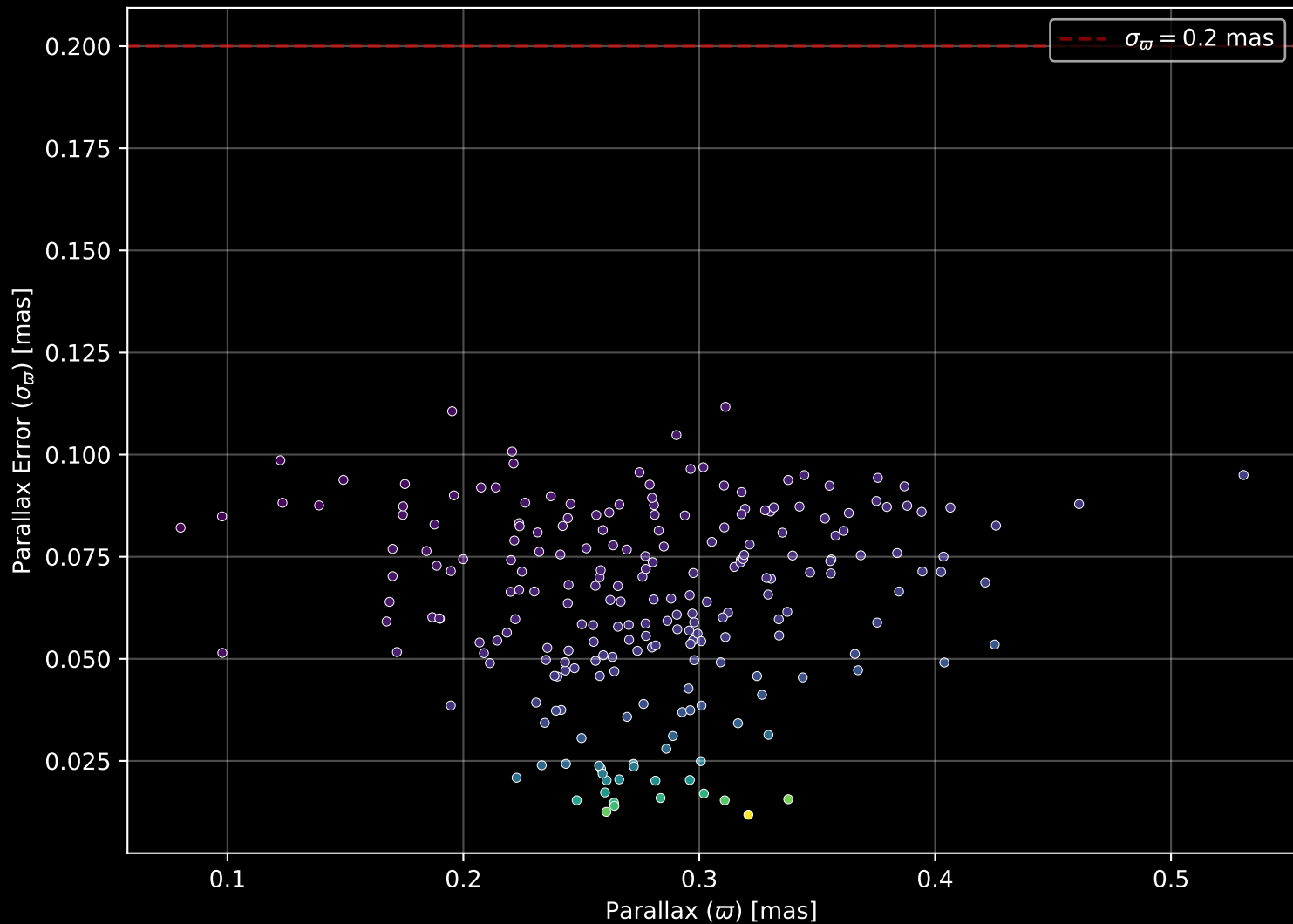
Gaia Cluster: [Berkeley_8] Parallax Quality (n= 225)
