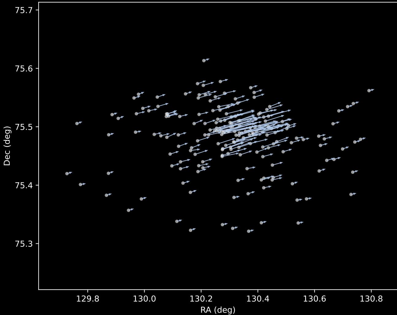
Gaia DR3 Cluster 1 Proper Motion Vectors (n=188)
