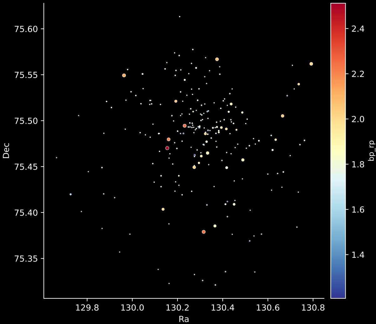
Gaia Cluster: [Berkeley_8] Stars: 225
