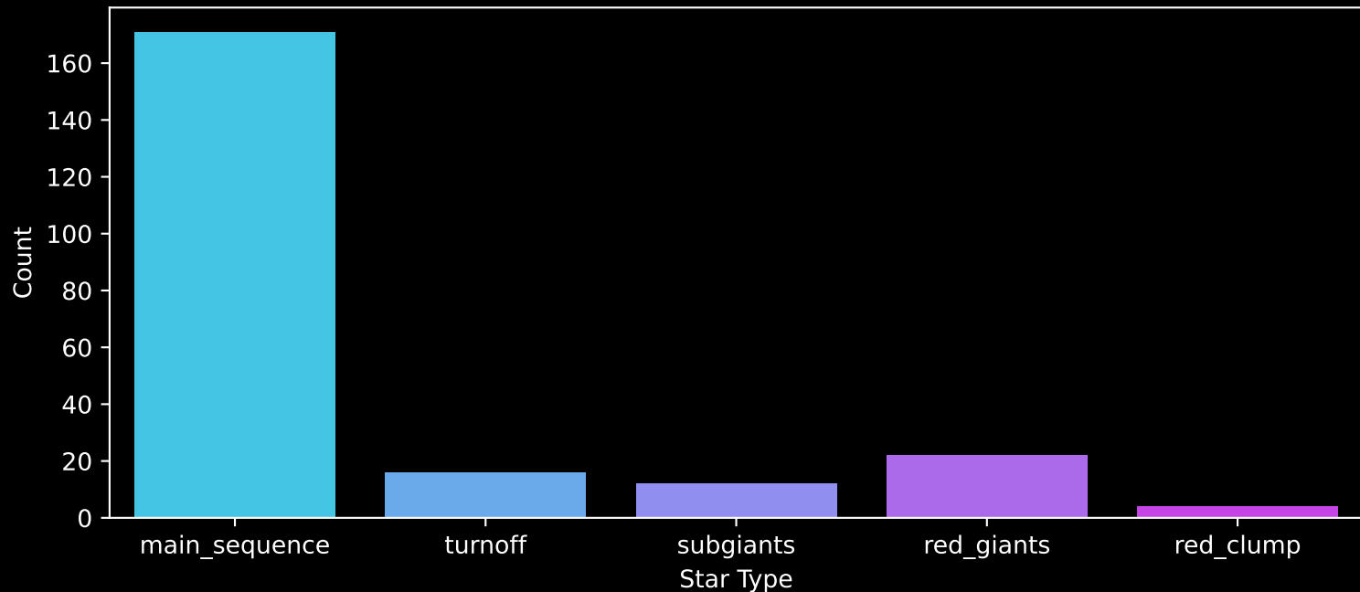
Gaia Cluster: [Berkeley_8] Count plot of Star Type
