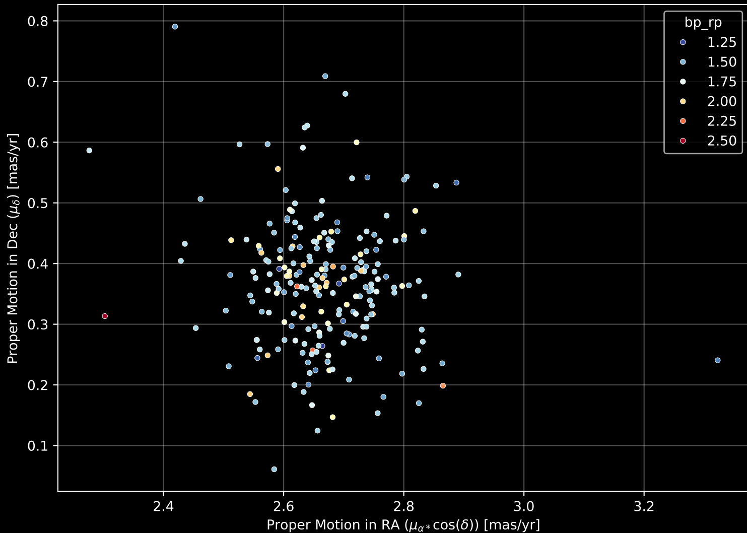
Gaia Cluster: [Berkeley_8] Proper Motion Diagram (n= 225)
