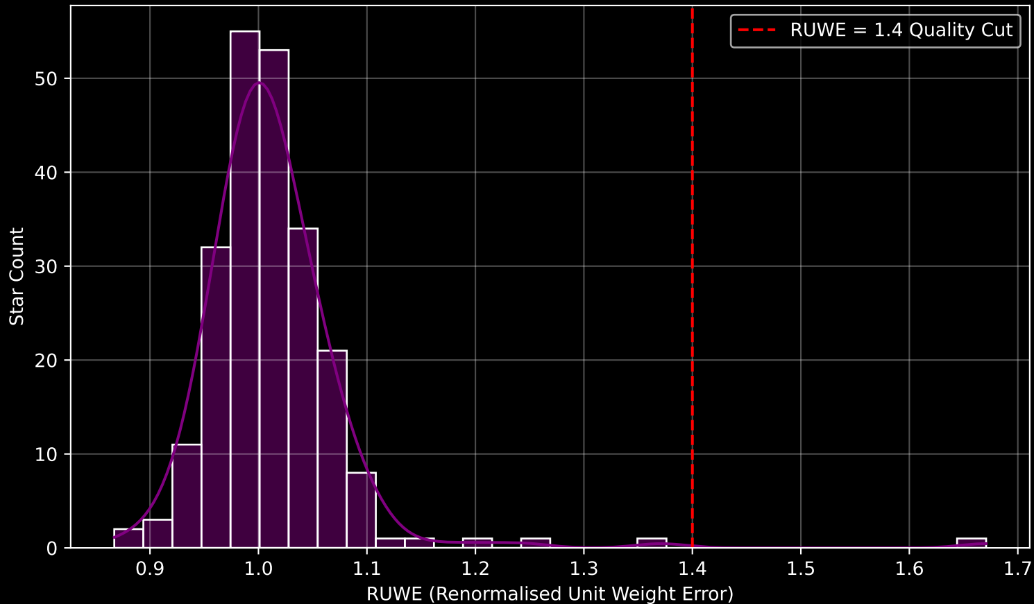
Gaia Cluster: [Berkeley_8] RUWE Distribution (n= 225)
