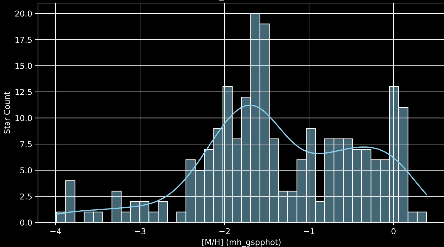
Gaia Cluster: [Berkeley_8 [M/H] (mh_gspphot) (n= 225)
