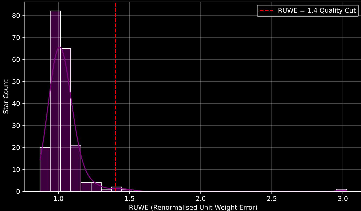
Gaia Cluster: [Berkeley_80] RUWE Distribution (n= 201)
