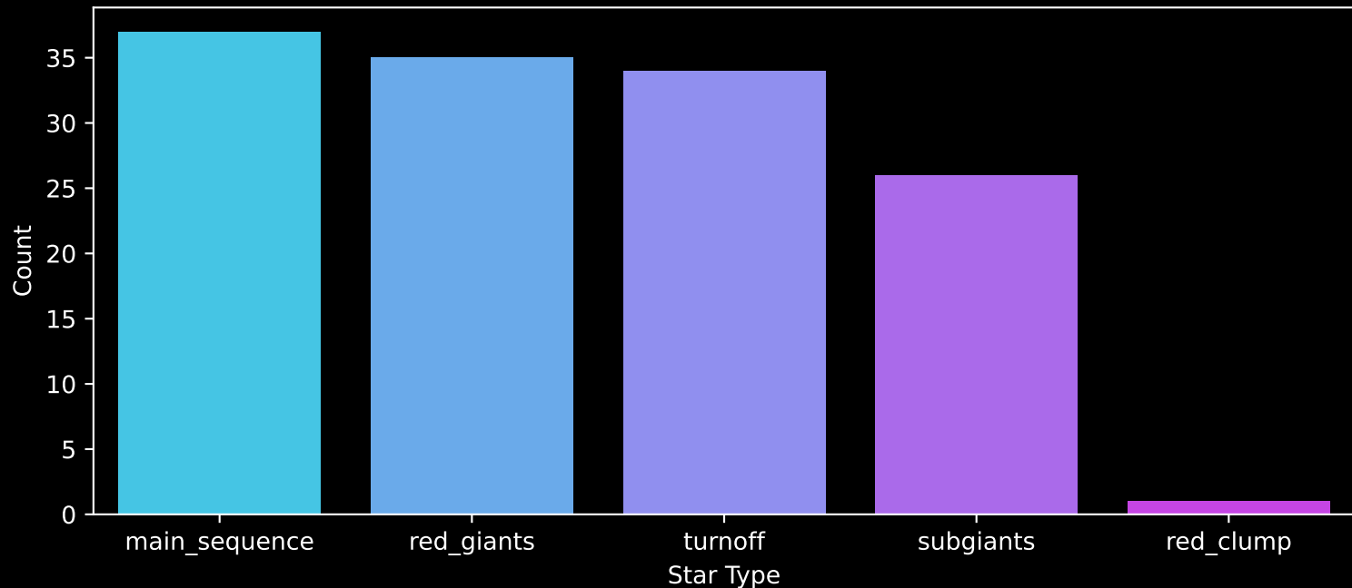
Gaia Cluster: [Berkeley_87] Count plot of Star Type
