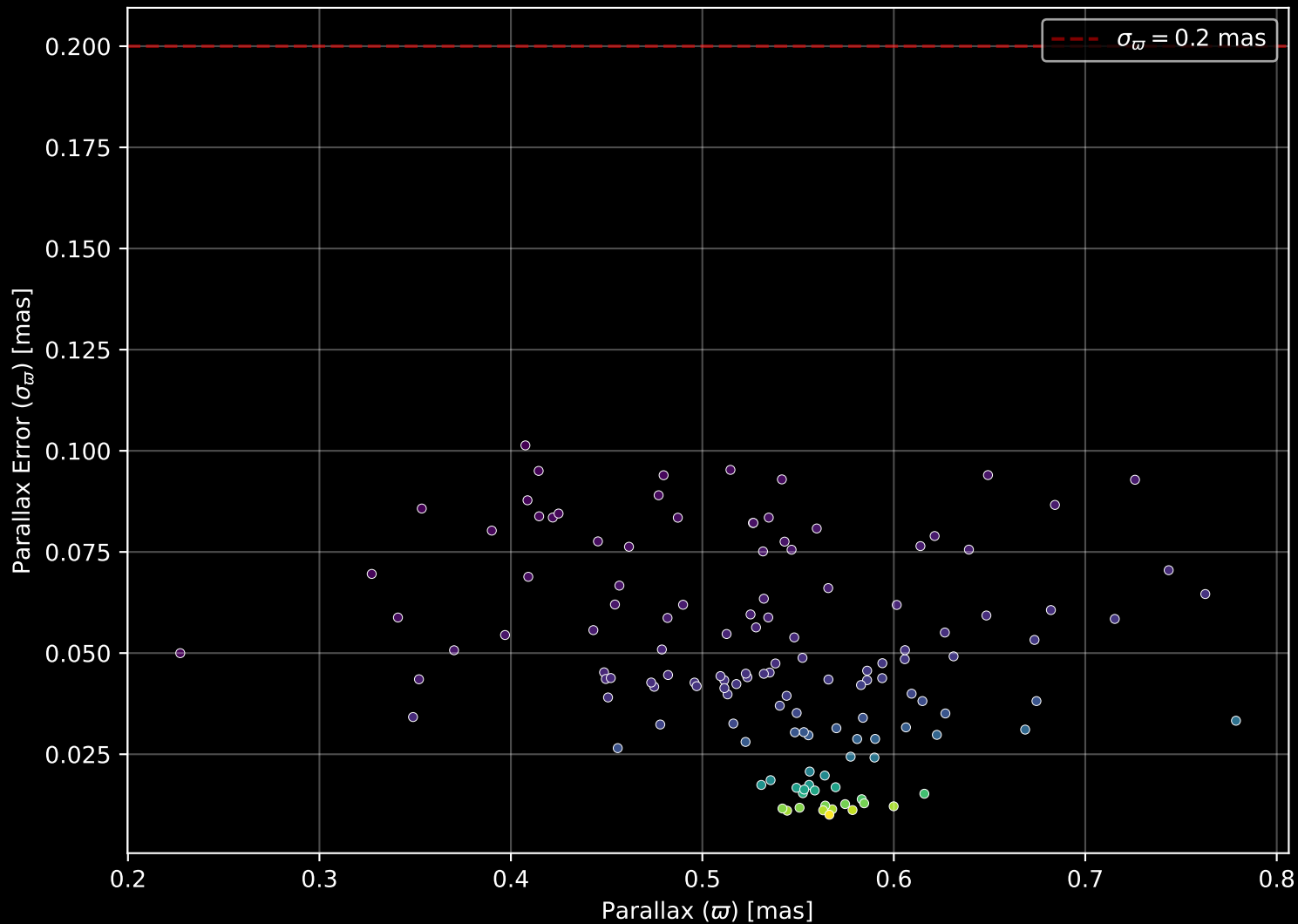
Gaia Cluster: [Berkeley_87] Parallax Quality (n= 133)
