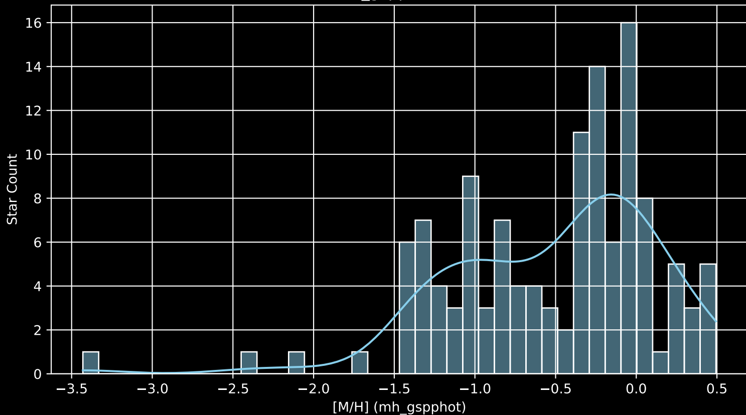
Gaia Cluster: [Berkeley_87 [M/H] (mh_gspphot) (n= 125)
