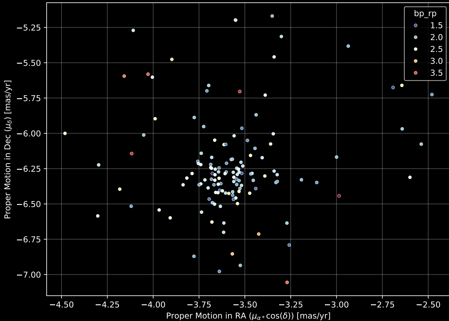
Gaia Cluster: [Berkeley_87] Proper Motion Diagram (n= 133)
