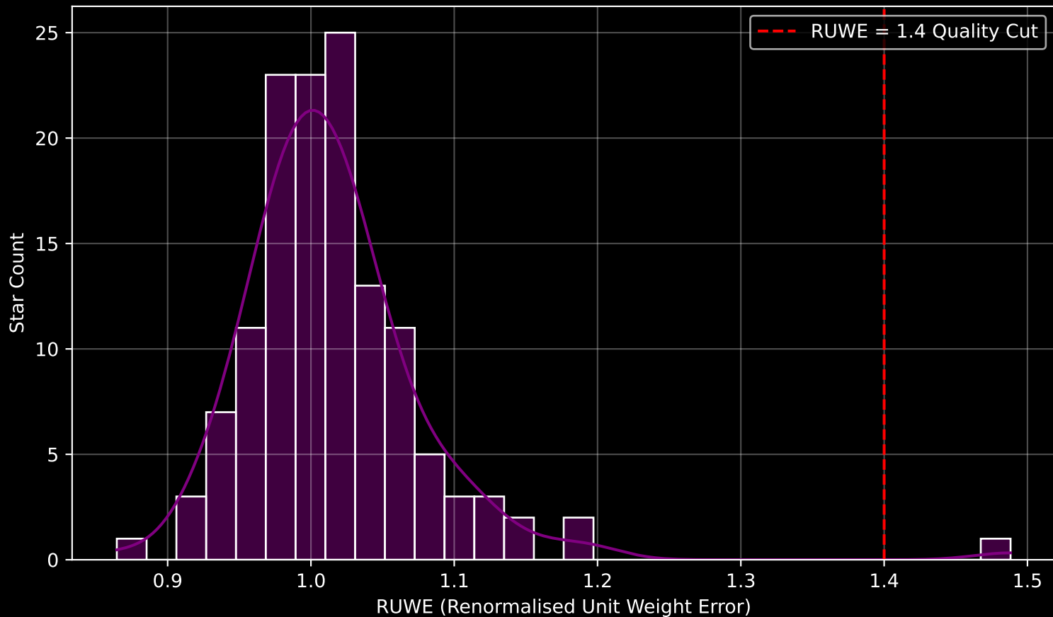
Gaia Cluster: [Berkeley_87] RUWE Distribution (n= 133)
