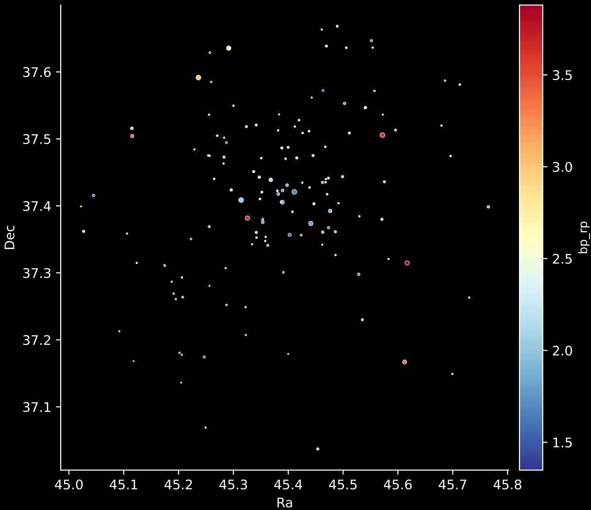
Gaia Cluster: [Berkeley_87] Stars: 133
