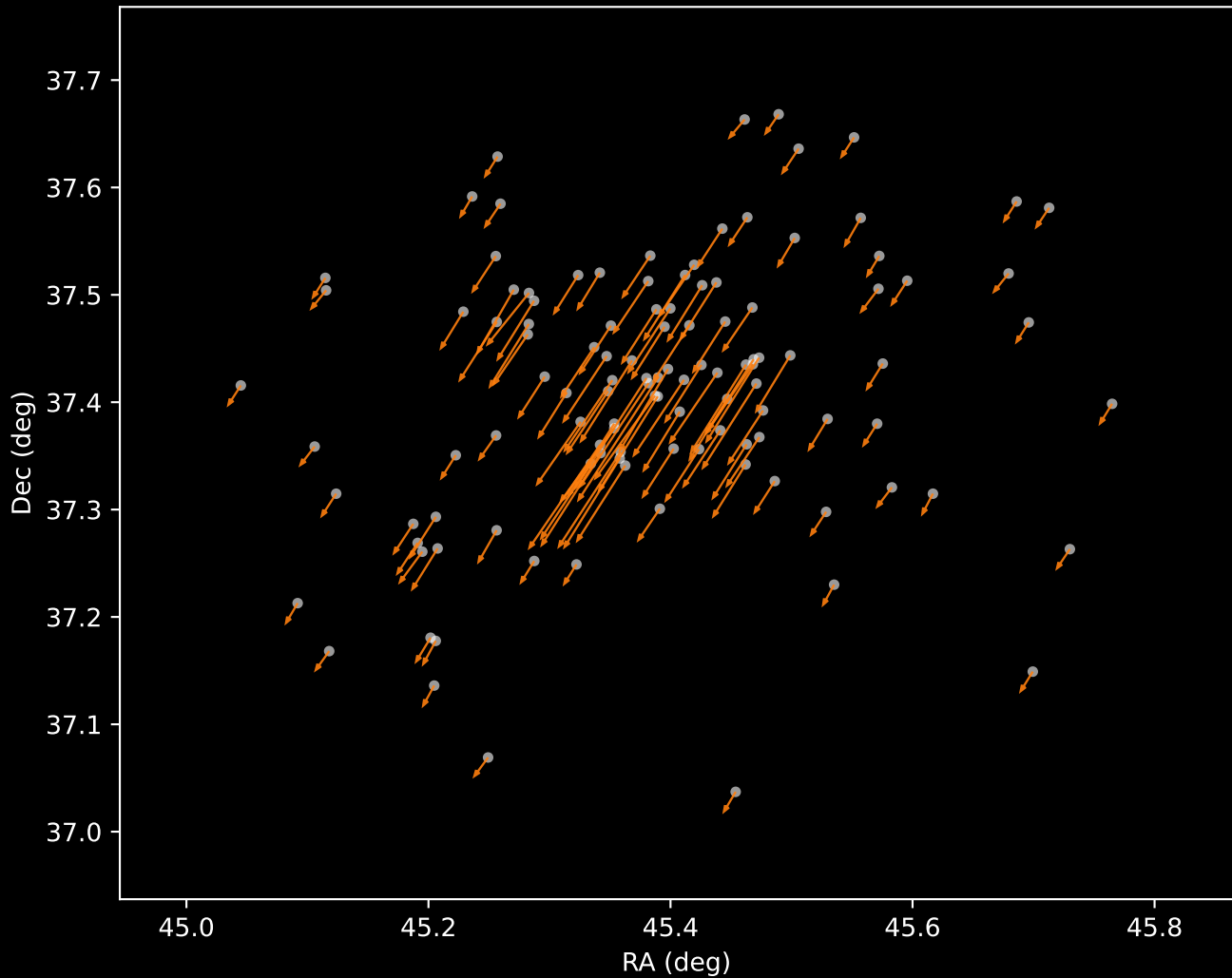
Gaia DR3 Cluster 2 Proper Motion Vectors (n=115)
