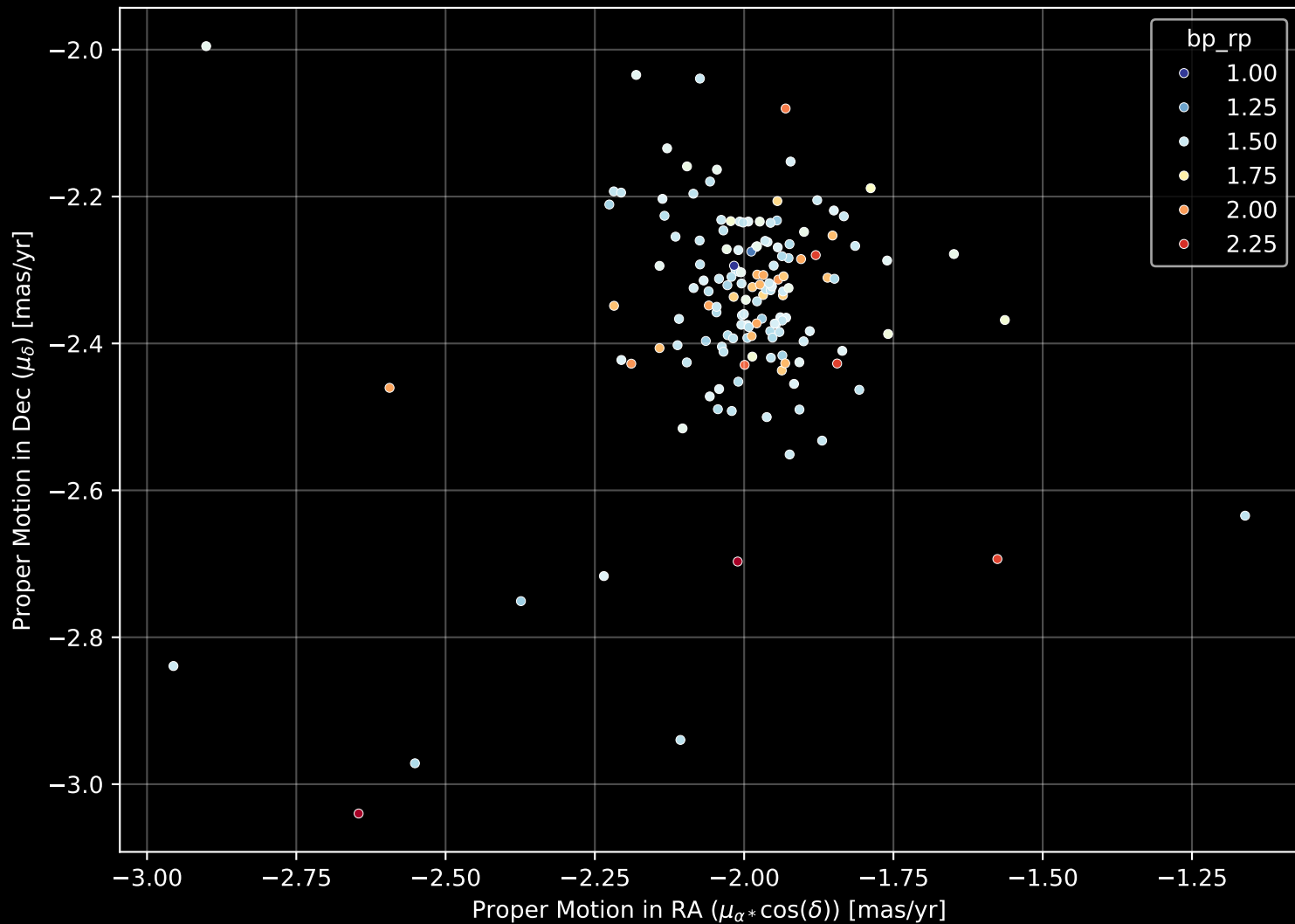
Gaia Cluster: [Berkeley_89] Proper Motion Diagram (n= 149)
