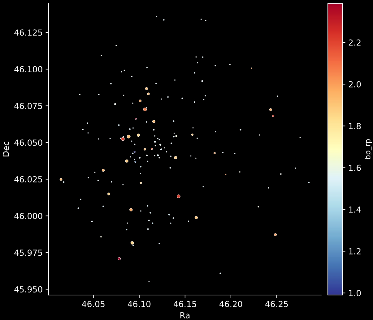
Gaia Cluster: [Berkeley_89] Stars: 149
