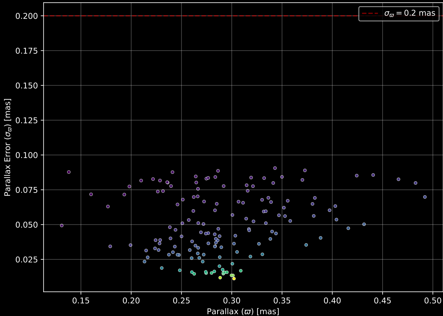
Gaia Cluster: [Berkeley_89] Parallax Quality (n= 149)
