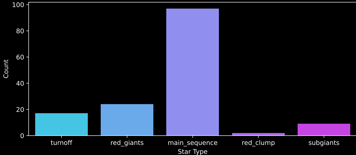
Gaia Cluster: [Berkeley_89] Count plot of Star Type
