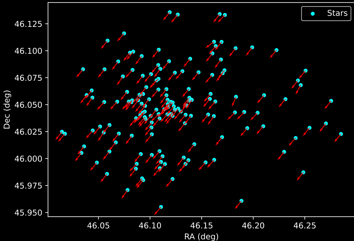
Gaia Cluster: [Berkeley_89] Proper Motion Vectors for Gaia Star Field (n= 149)
