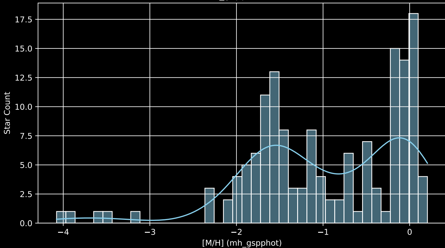
Gaia Cluster: [Berkeley_89 [M/H] (mh_gspphot) (n= 148)
