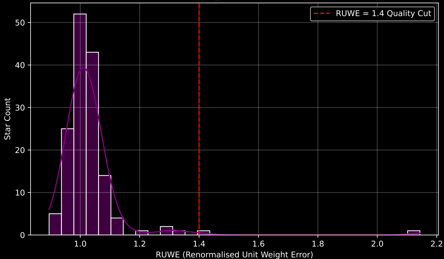
Gaia Cluster: [Berkeley_89] RUWE Distribution (n= 149)
