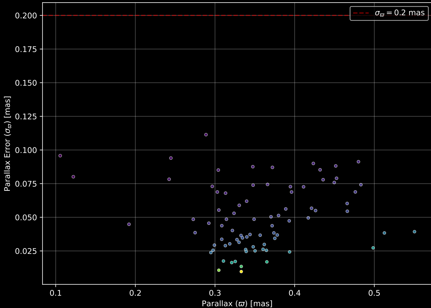
Gaia Cluster: [Berkeley_90] Parallax Quality (n= 81)
