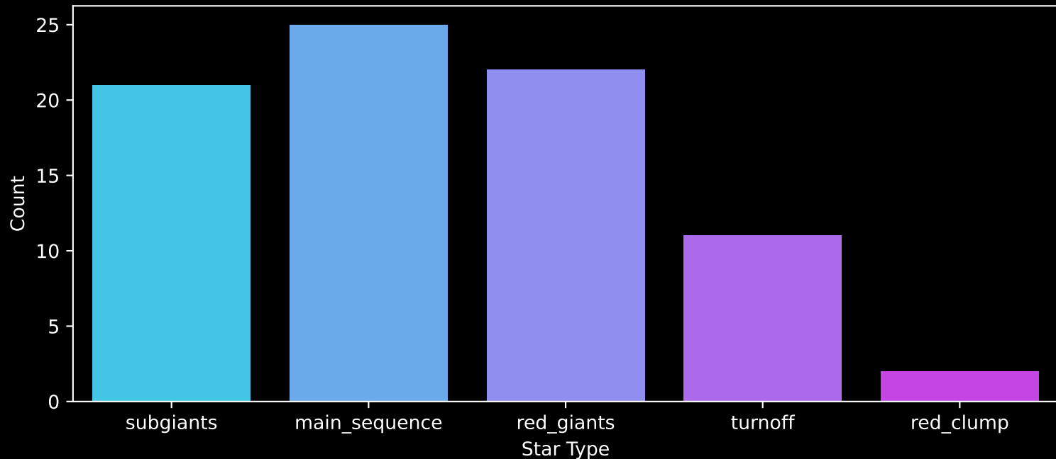
Gaia Cluster: [Berkeley_90] Count plot of Star Type
