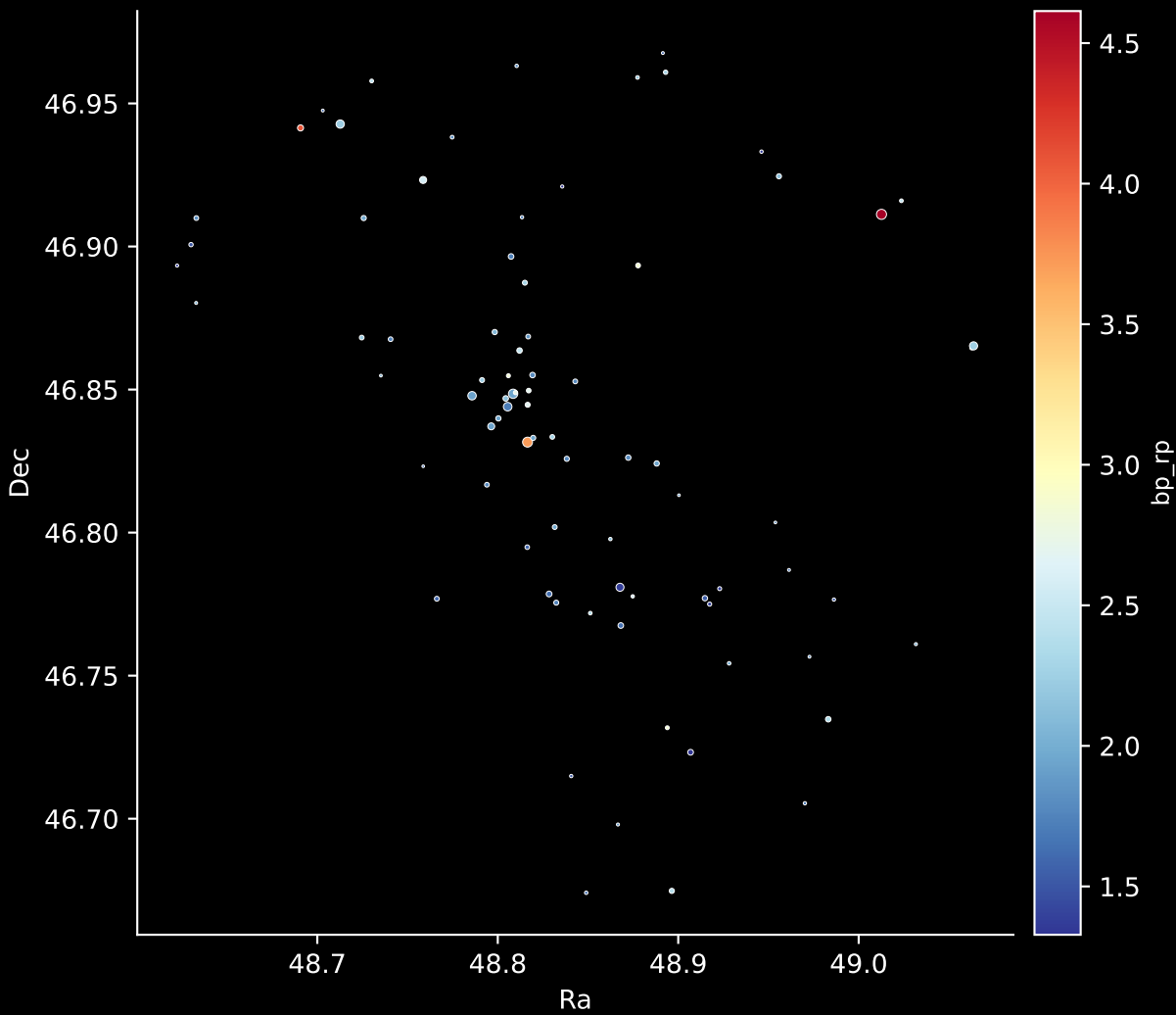
Gaia Cluster: [Berkeley_90] Stars: 81
