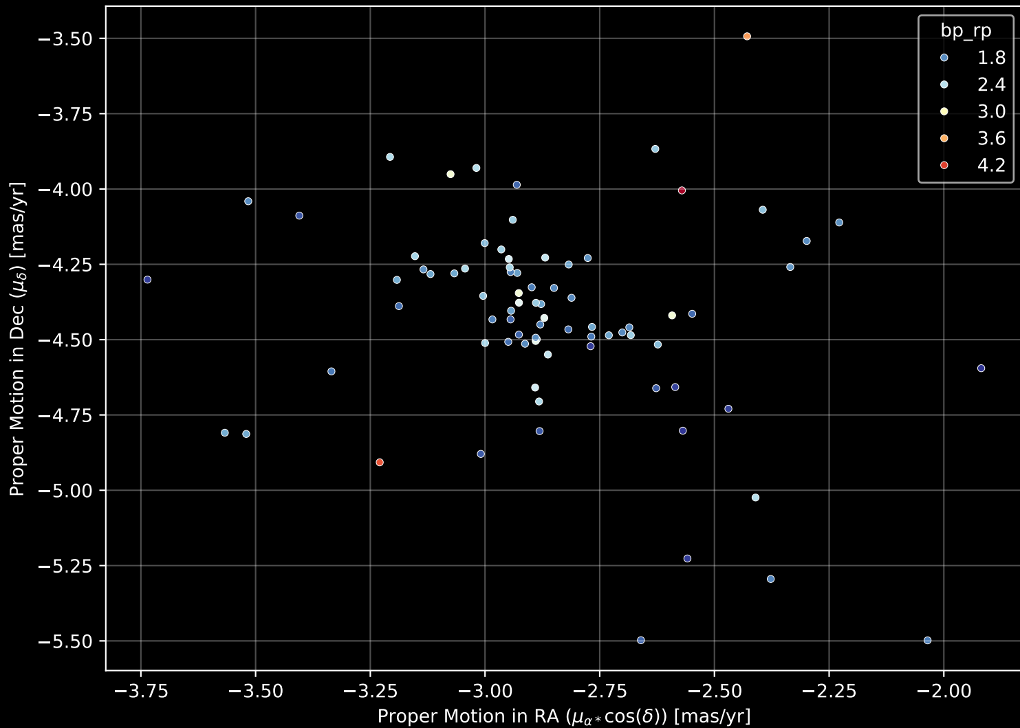
Gaia Cluster: [Berkeley_90] Proper Motion Diagram (n= 81)
