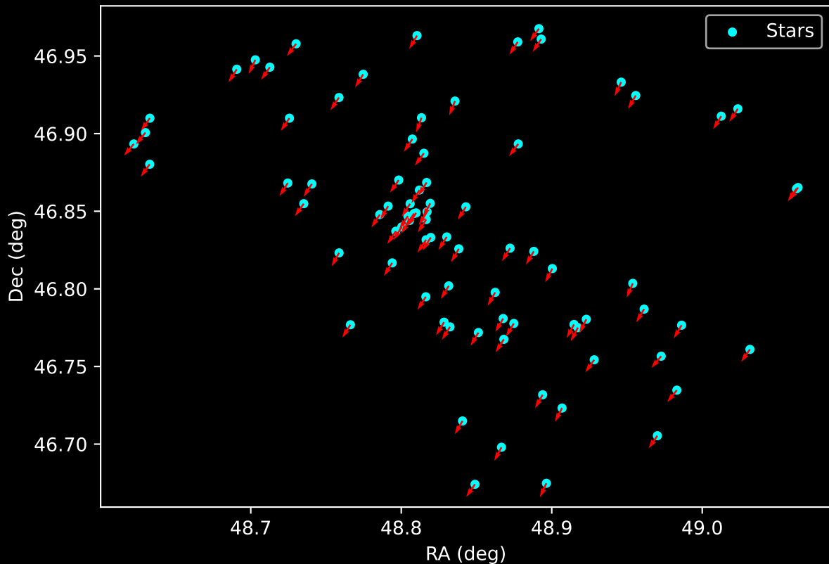
Gaia Cluster: [Berkeley_90] Proper Motion Vectors for Gaia Star Field (n= 81)
