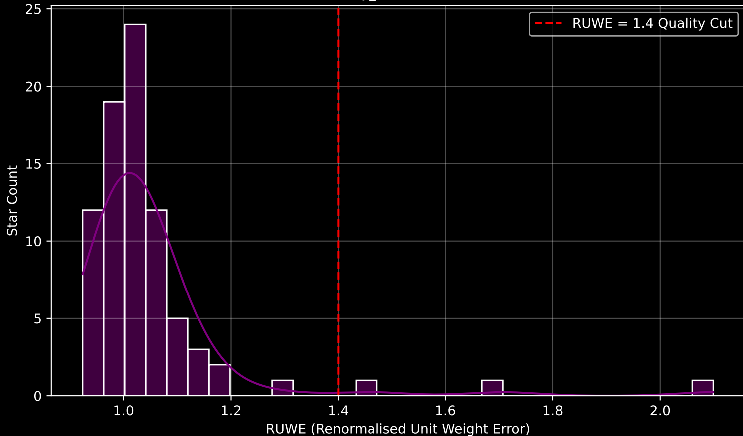
Gaia Cluster: [Berkeley_90] RUWE Distribution (n= 81)
