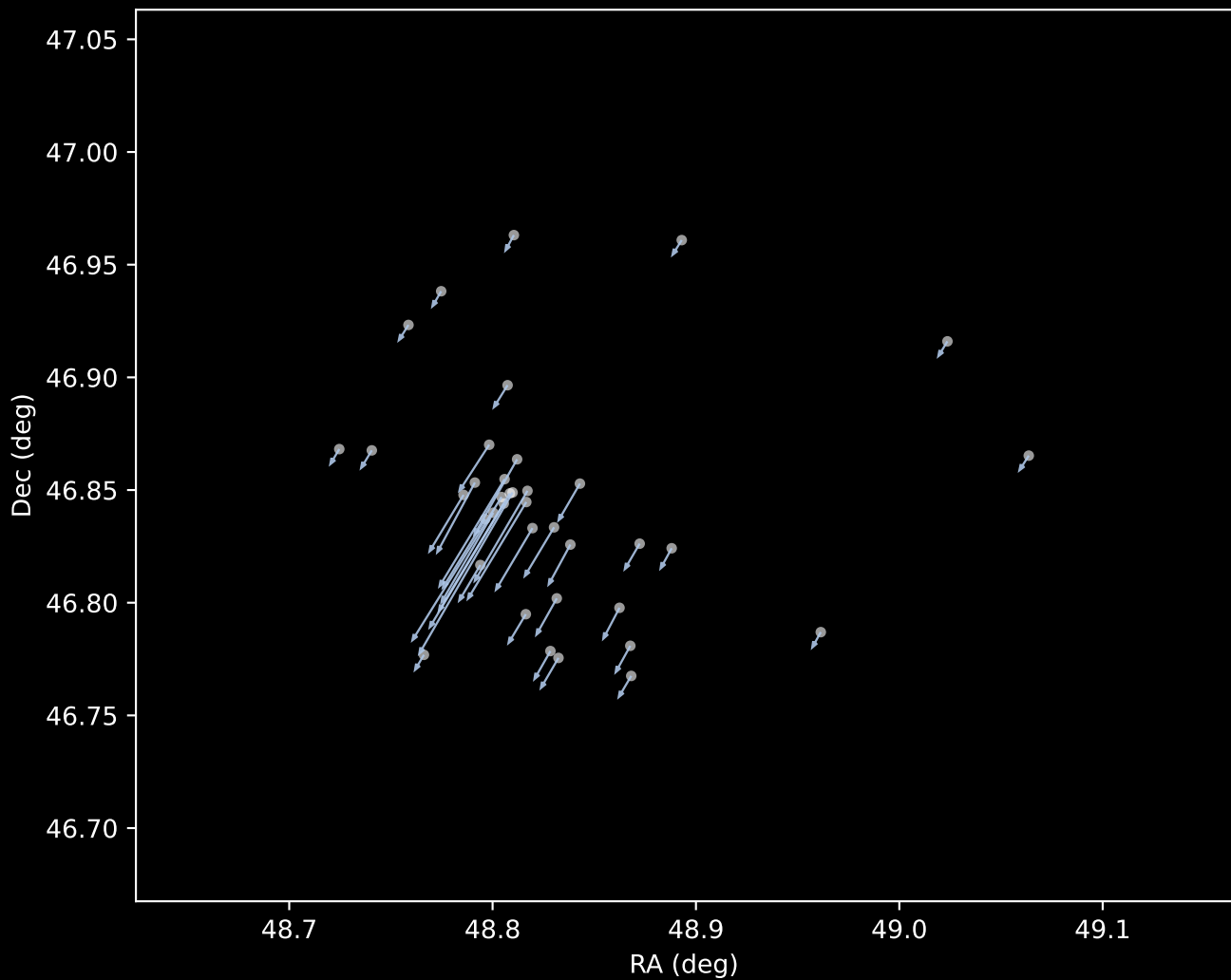
Gaia DR3 Cluster 1 Proper Motion Vectors (n=38)
