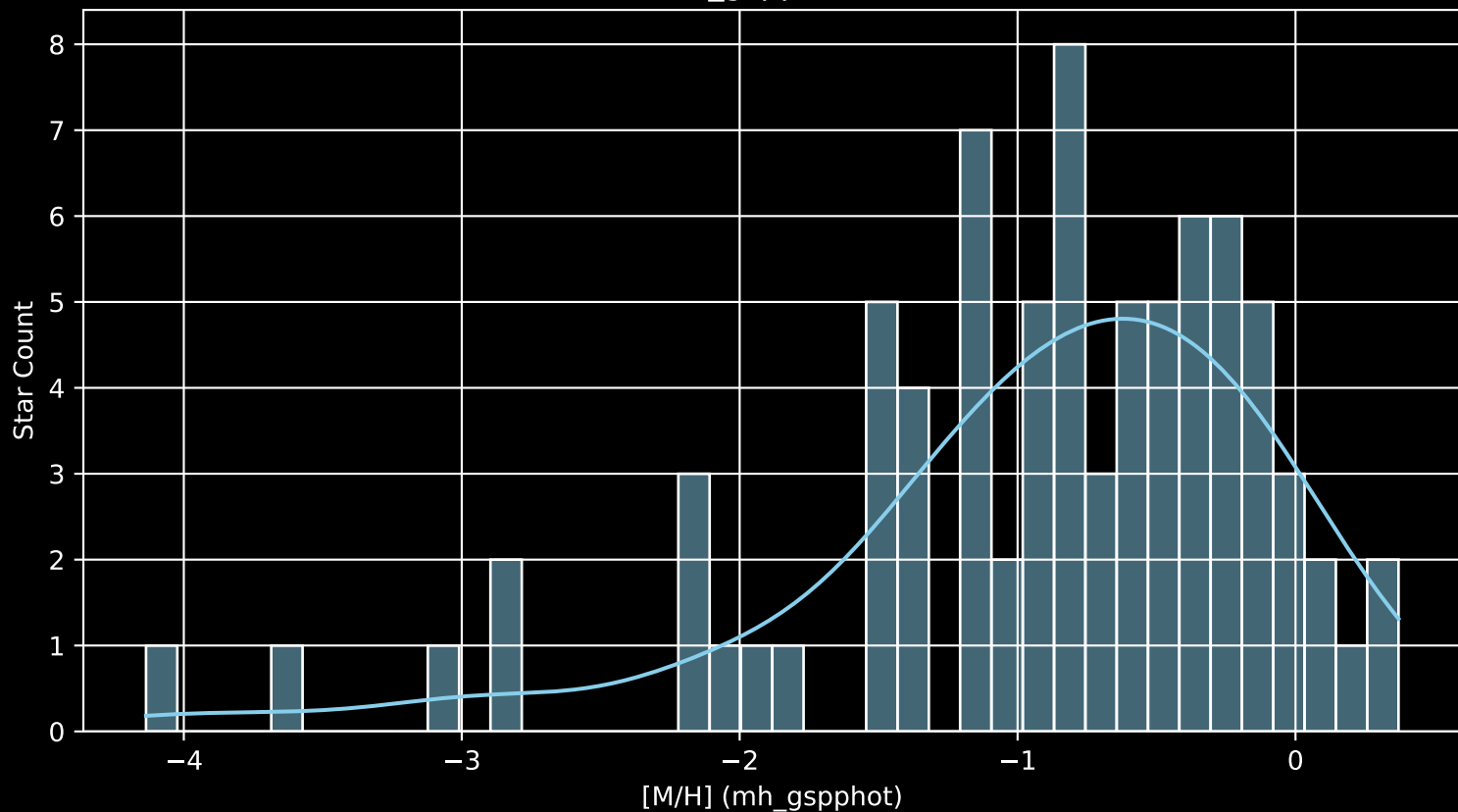
Gaia Cluster: [Berkeley_90 [M/H] (mh_gspphot) (n= 80)
