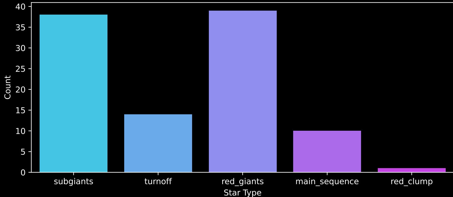
Gaia Cluster: [Berkeley_95] Count plot of Star Type
