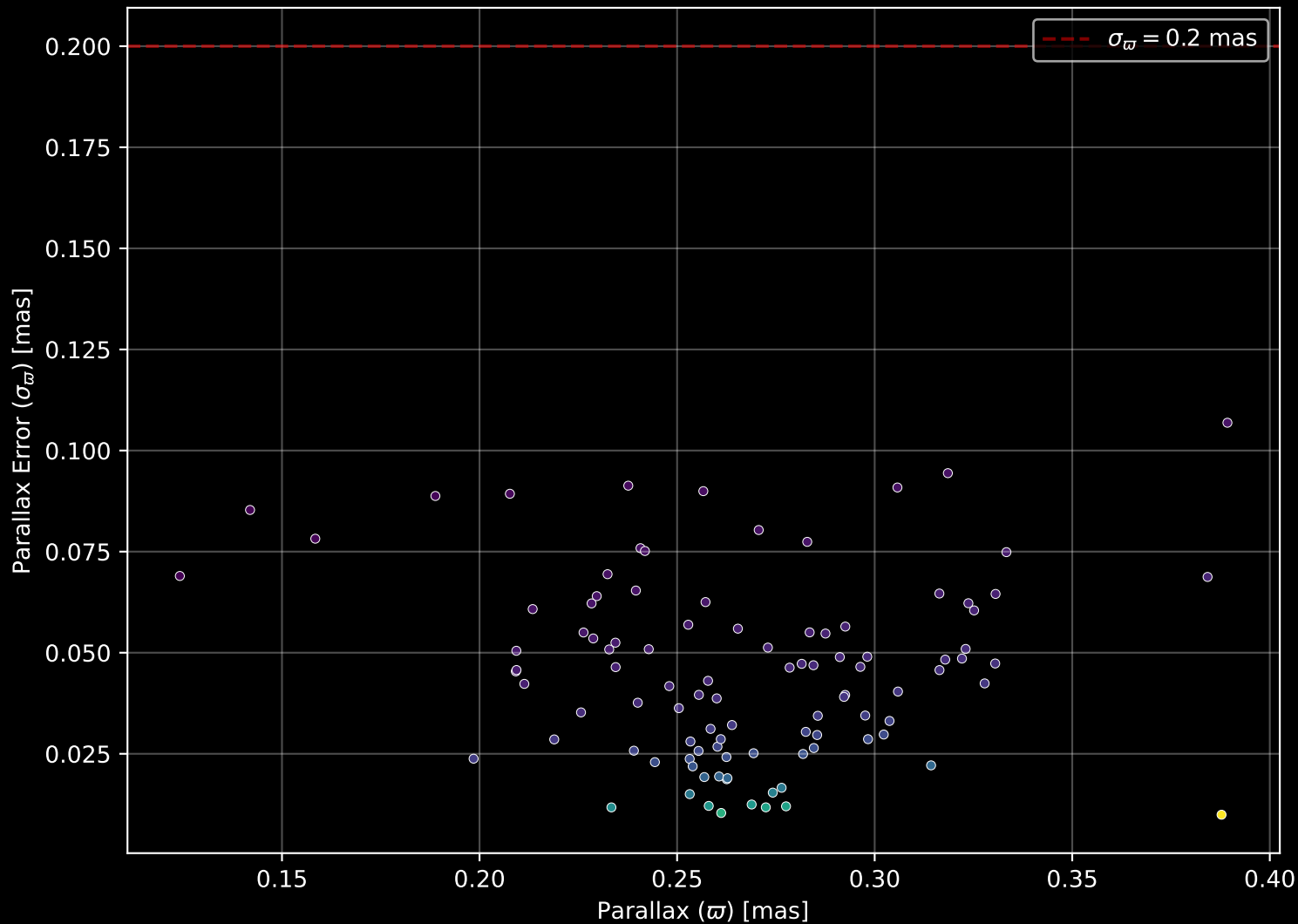
Gaia Cluster: [Berkeley_95] Parallax Quality (n= 102)
