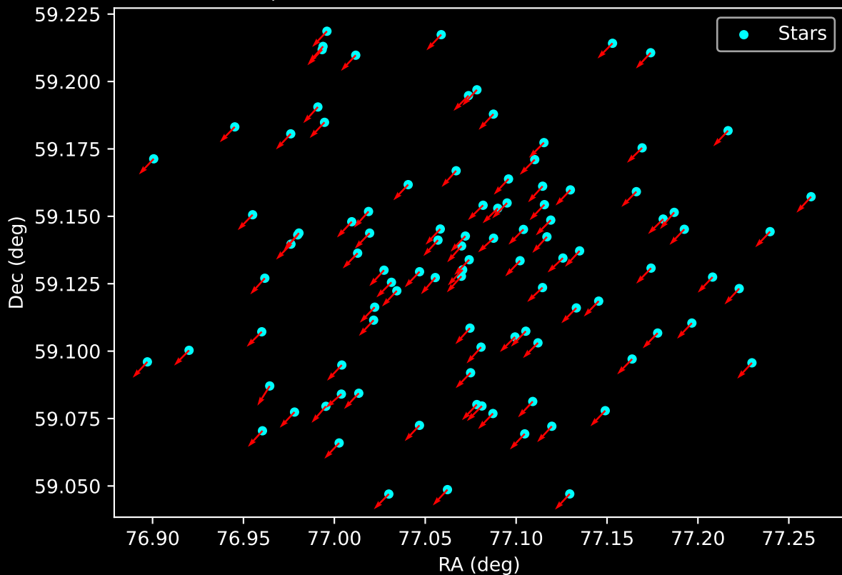
Gaia Cluster: [Berkeley_95] Proper Motion Vectors for Gaia Star Field (n= 102)
