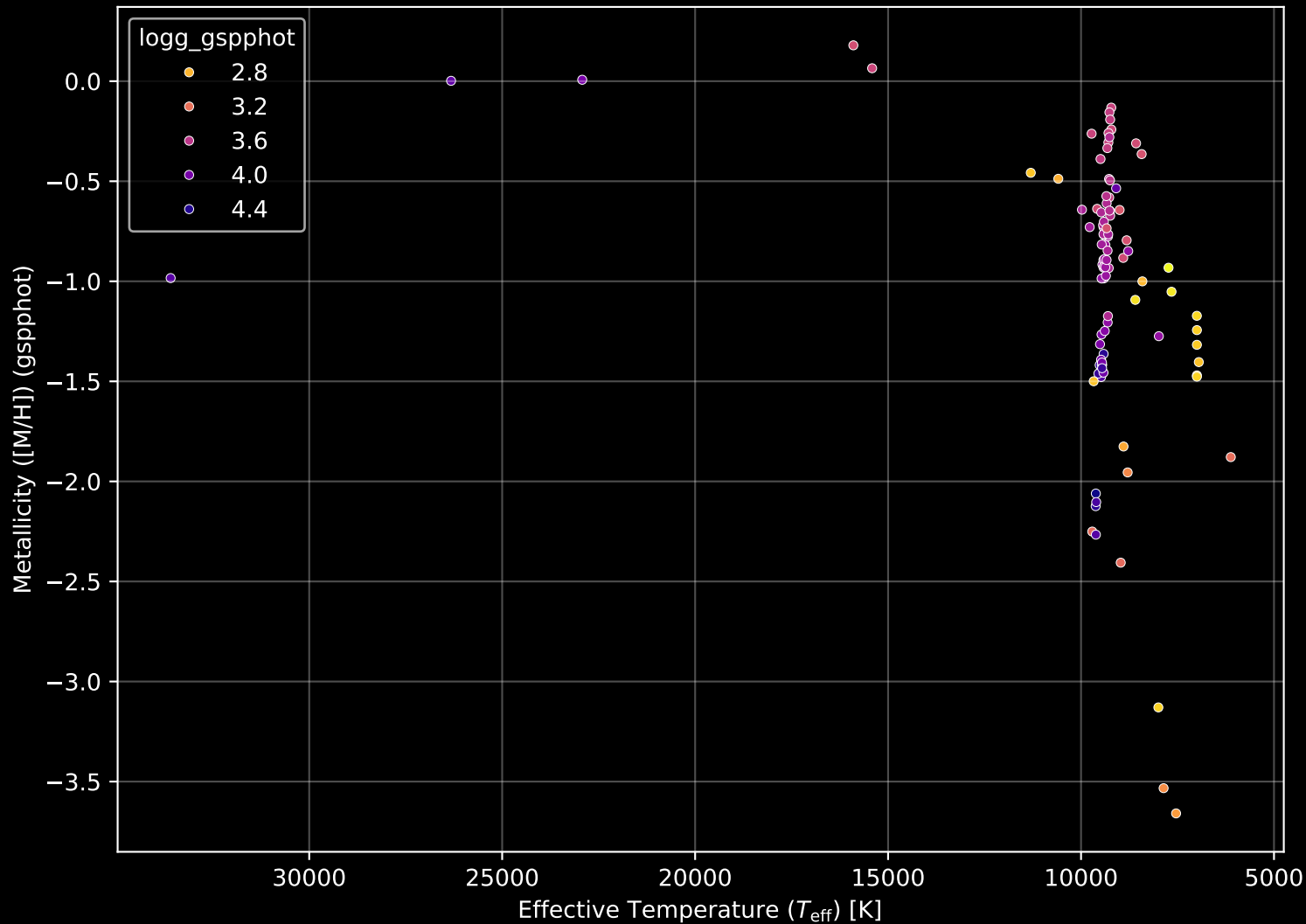
Gaia Cluster: [Berkeley_95] Stellar Population Parameters (n= 102)
