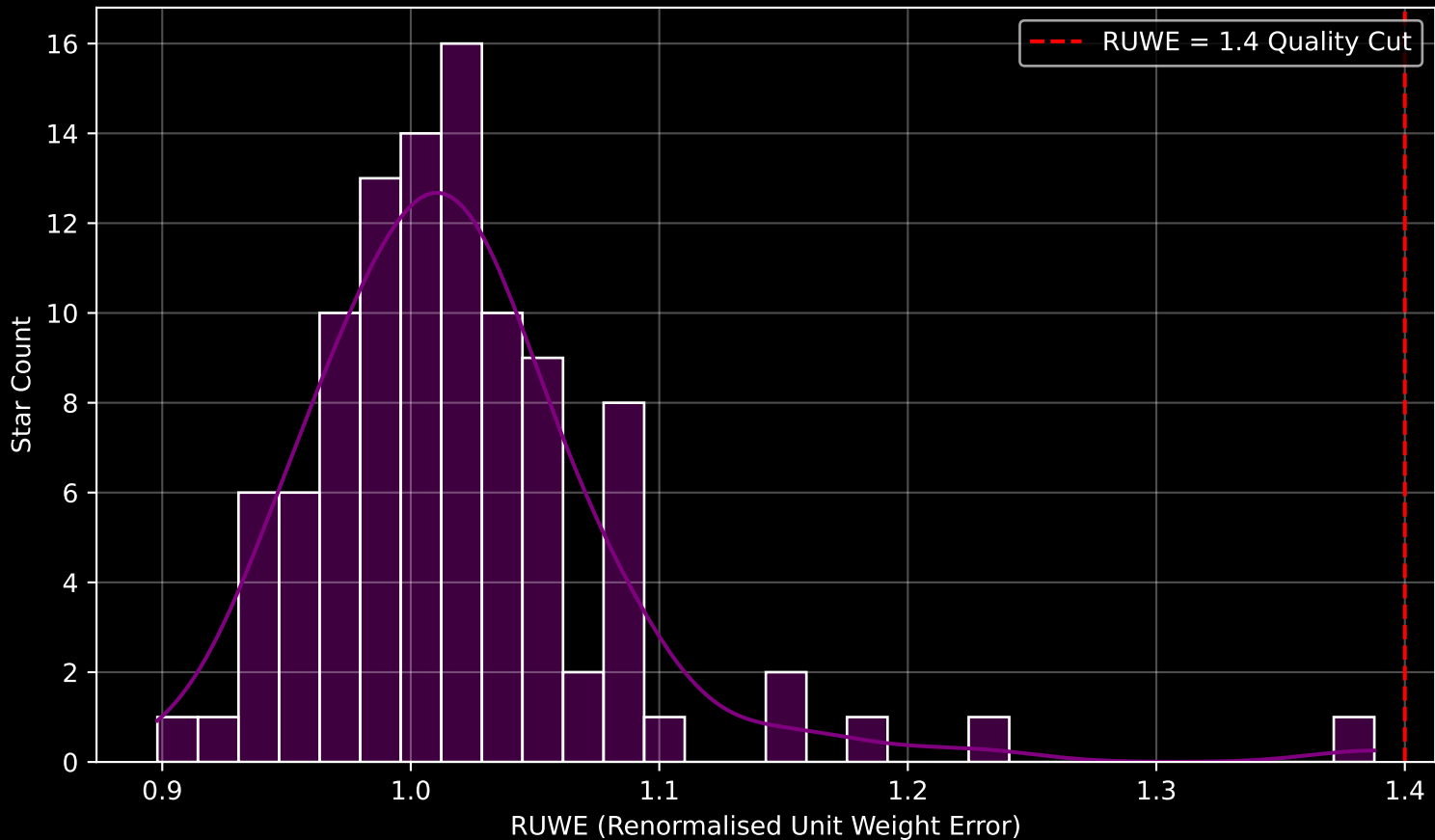
Gaia Cluster: [Berkeley_95] RUWE Distribution (n= 102)
