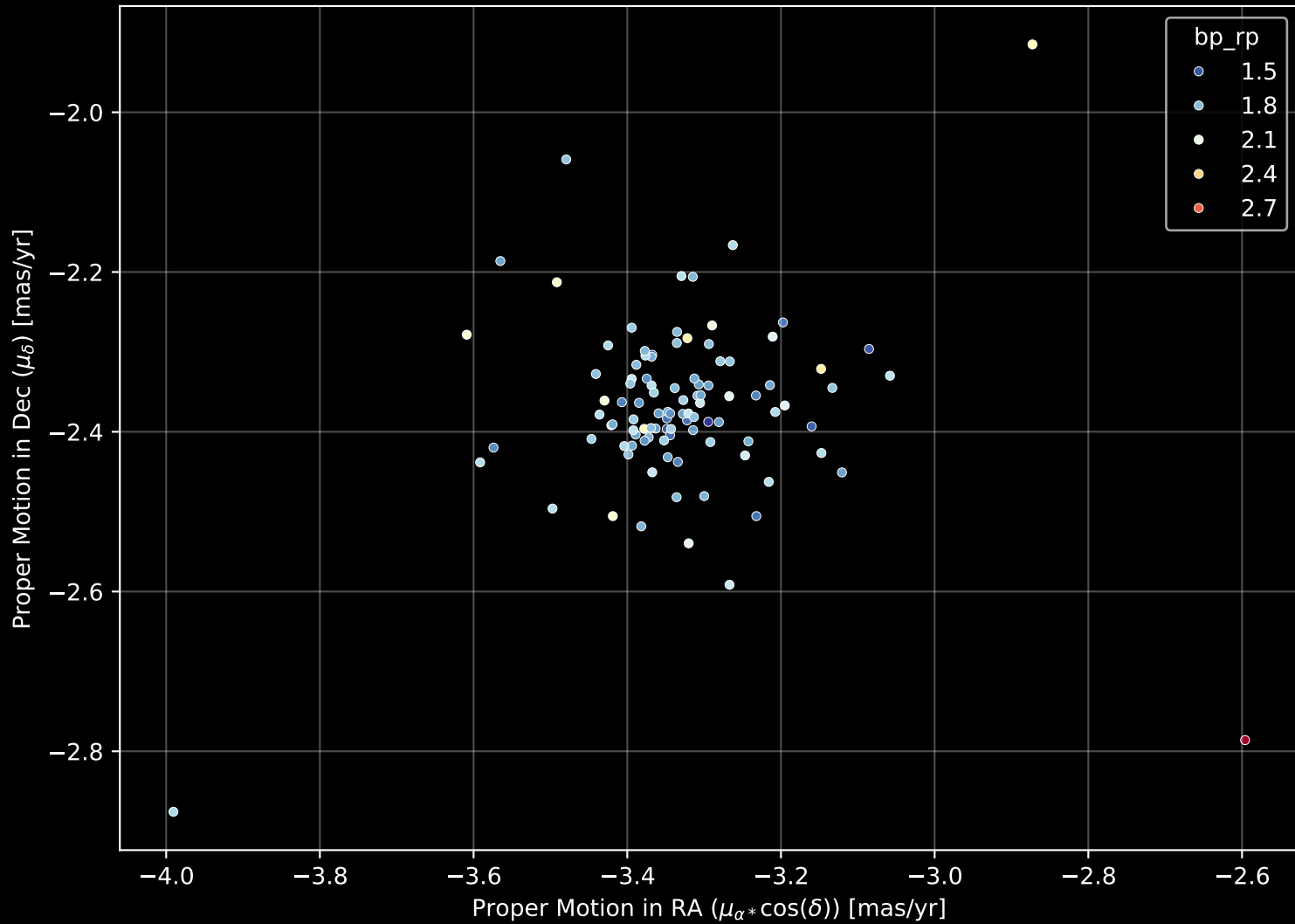
Gaia Cluster: [Berkeley_95] Proper Motion Diagram (n= 102)
