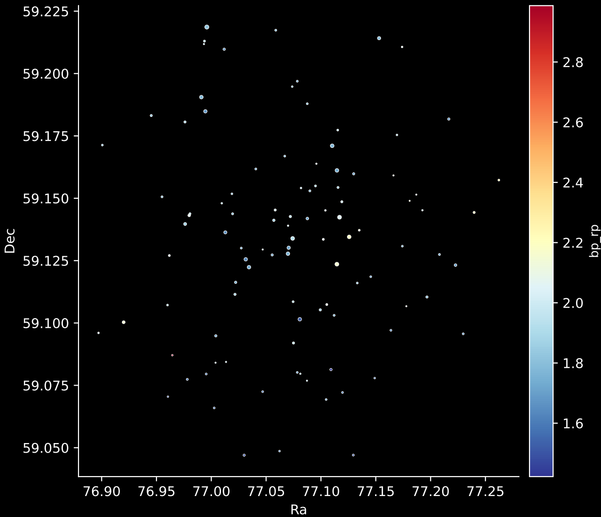
Gaia Cluster: [Berkeley_95] Stars: 102
