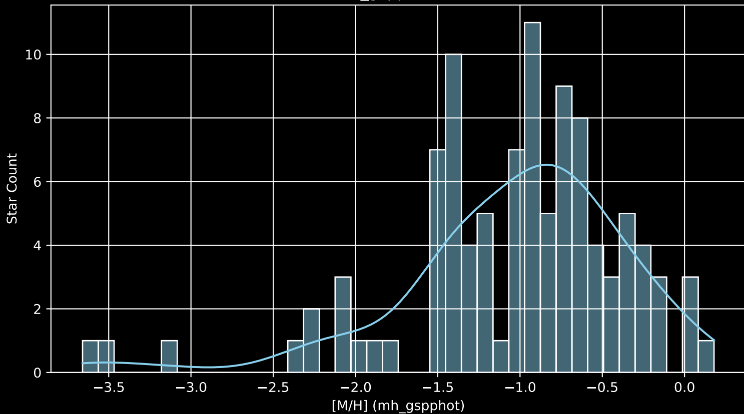
Gaia Cluster: [Berkeley_95 [M/H] (mh_gspphot) (n= 102)
