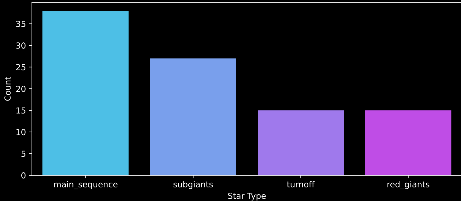
Gaia Cluster: [Berkeley_97] Count plot of Star Type
