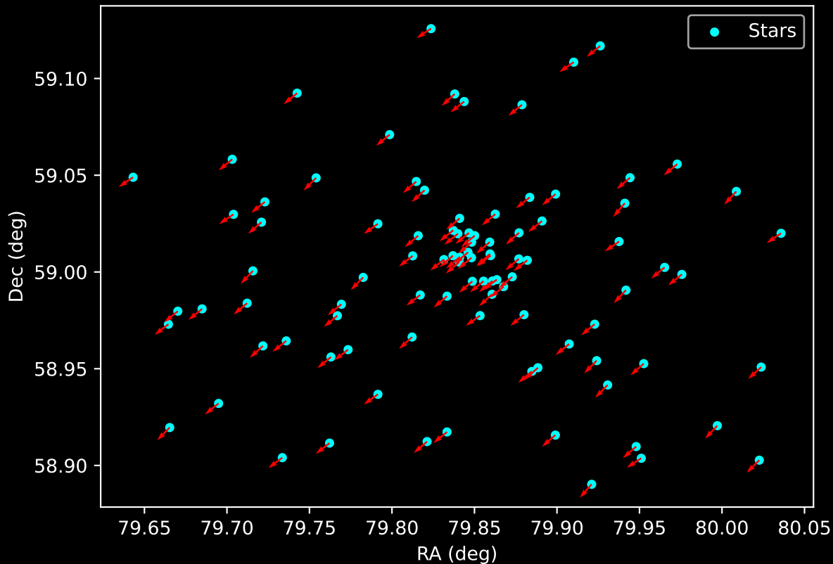
Gaia Cluster: [Berkeley_97] Proper Motion Vectors for Gaia Star Field (n= 95)
