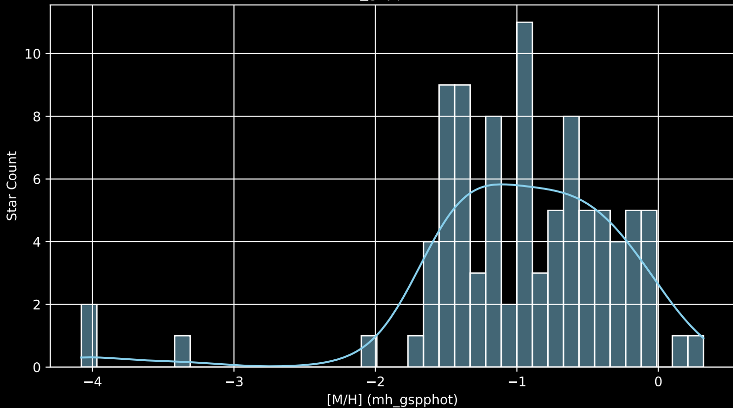
Gaia Cluster: [Berkeley_97 [M/H] (mh_gspphot) (n= 93)
