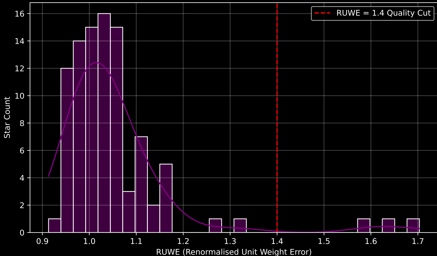
Gaia Cluster: [Berkeley_97] RUWE Distribution (n= 95)
