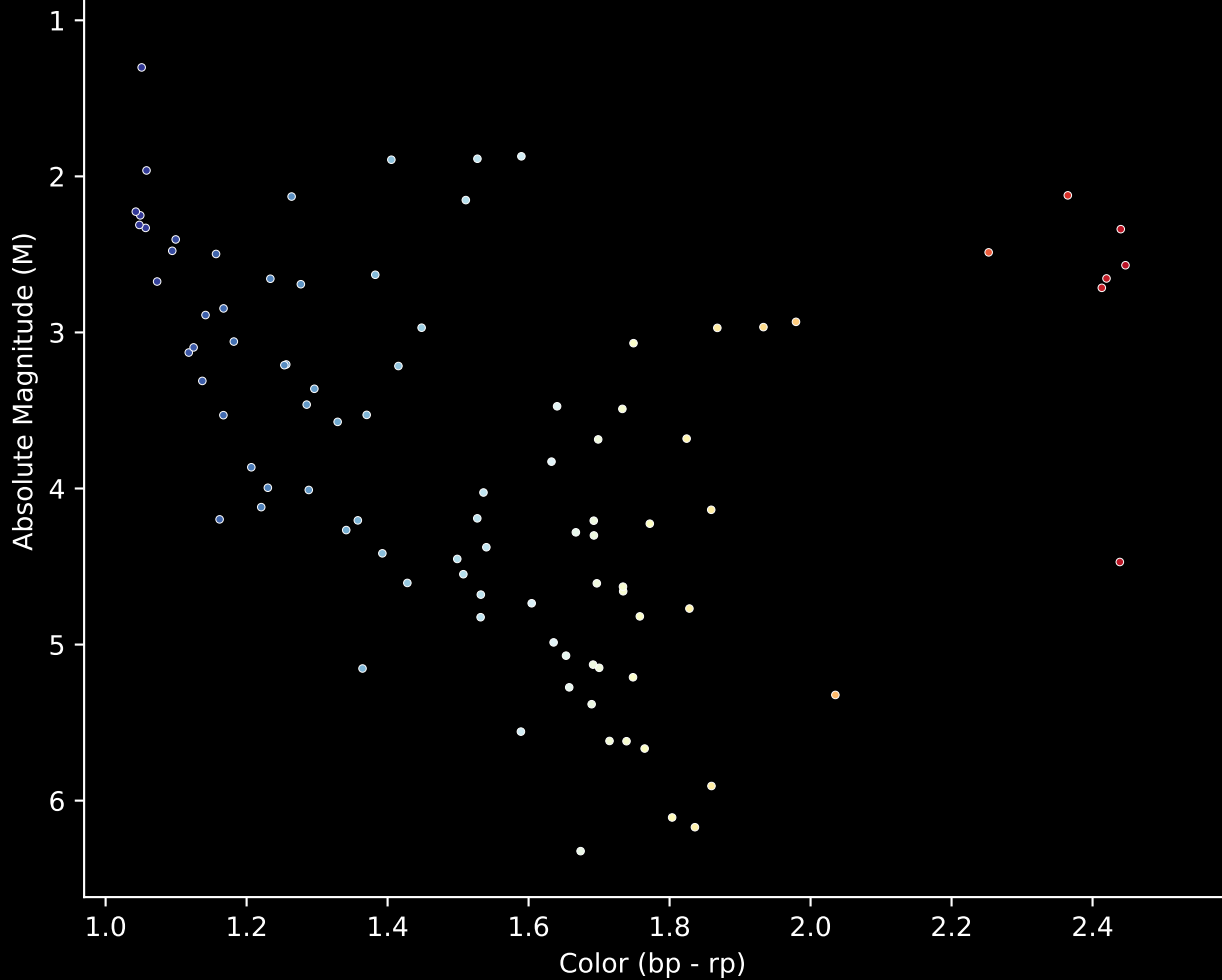
Gaia Cluster: [Berkeley_97] Stars (n= 95) Hertzprung-Russel Diagram
