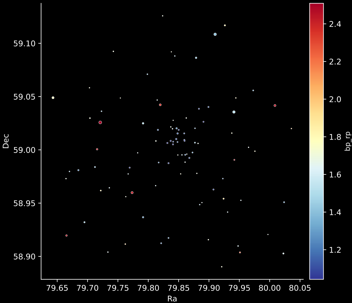
Gaia Cluster: [Berkeley_97] Stars: 95
