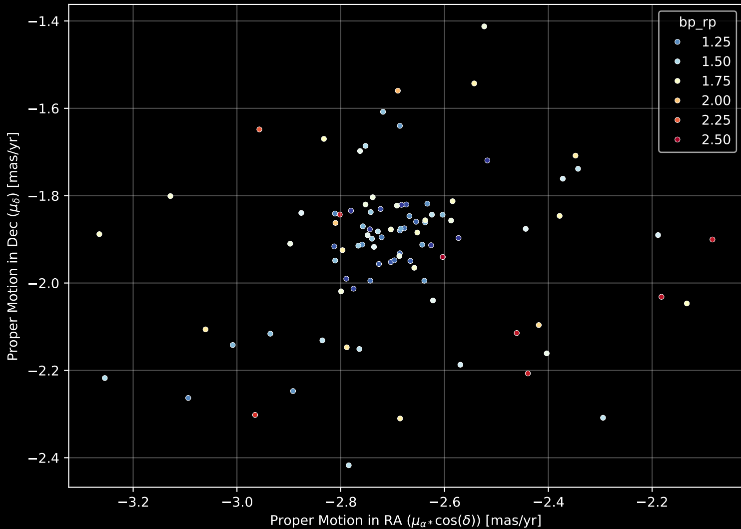
Gaia Cluster: [Berkeley_97] Proper Motion Diagram (n= 95)
