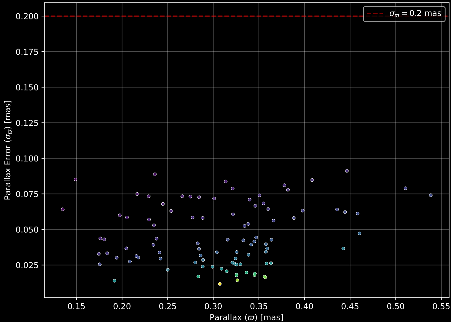
Gaia Cluster: [Berkeley_97] Parallax Quality (n= 95)
