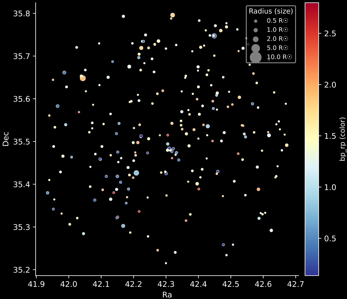
Gaia Cluster: [Buirakan_2] Stars: 235
