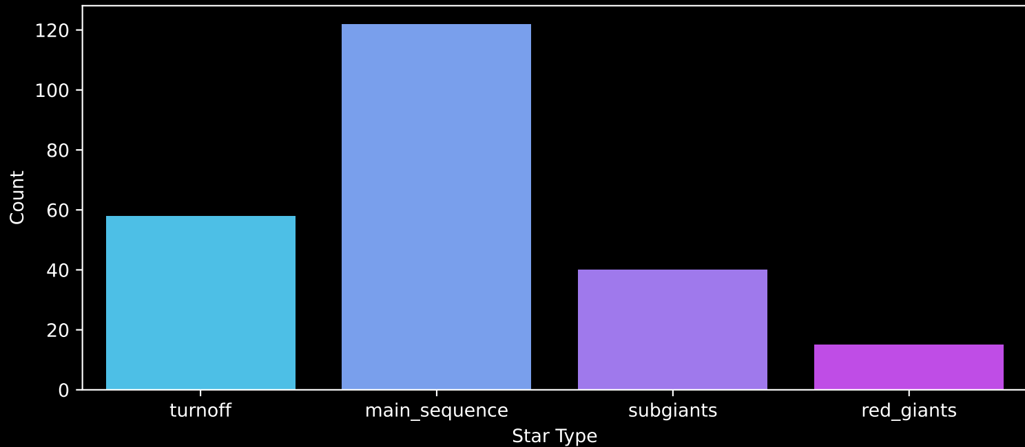
Gaia Cluster: [Biurakan_2] Count plot of Star Type
