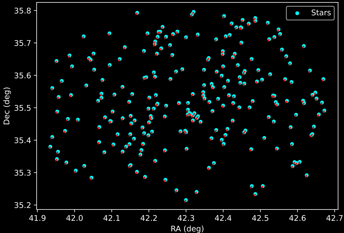
Gaia Cluster: [Biurakan_2] Proper Motion Vectors for Gaia Star Field (n= 235)
