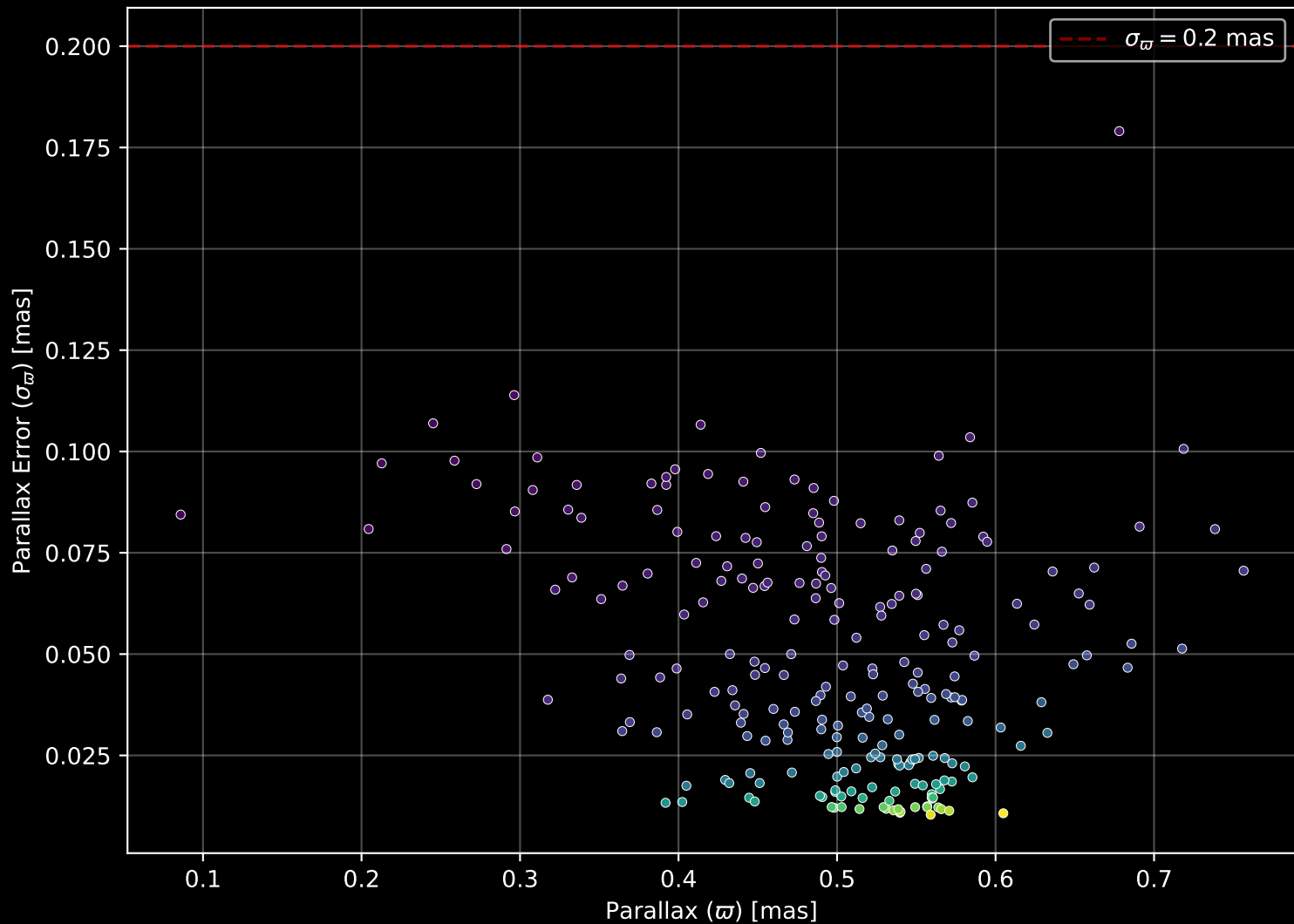
Gaia Cluster: [Biurakan_2] Parallax Quality (n= 235)
