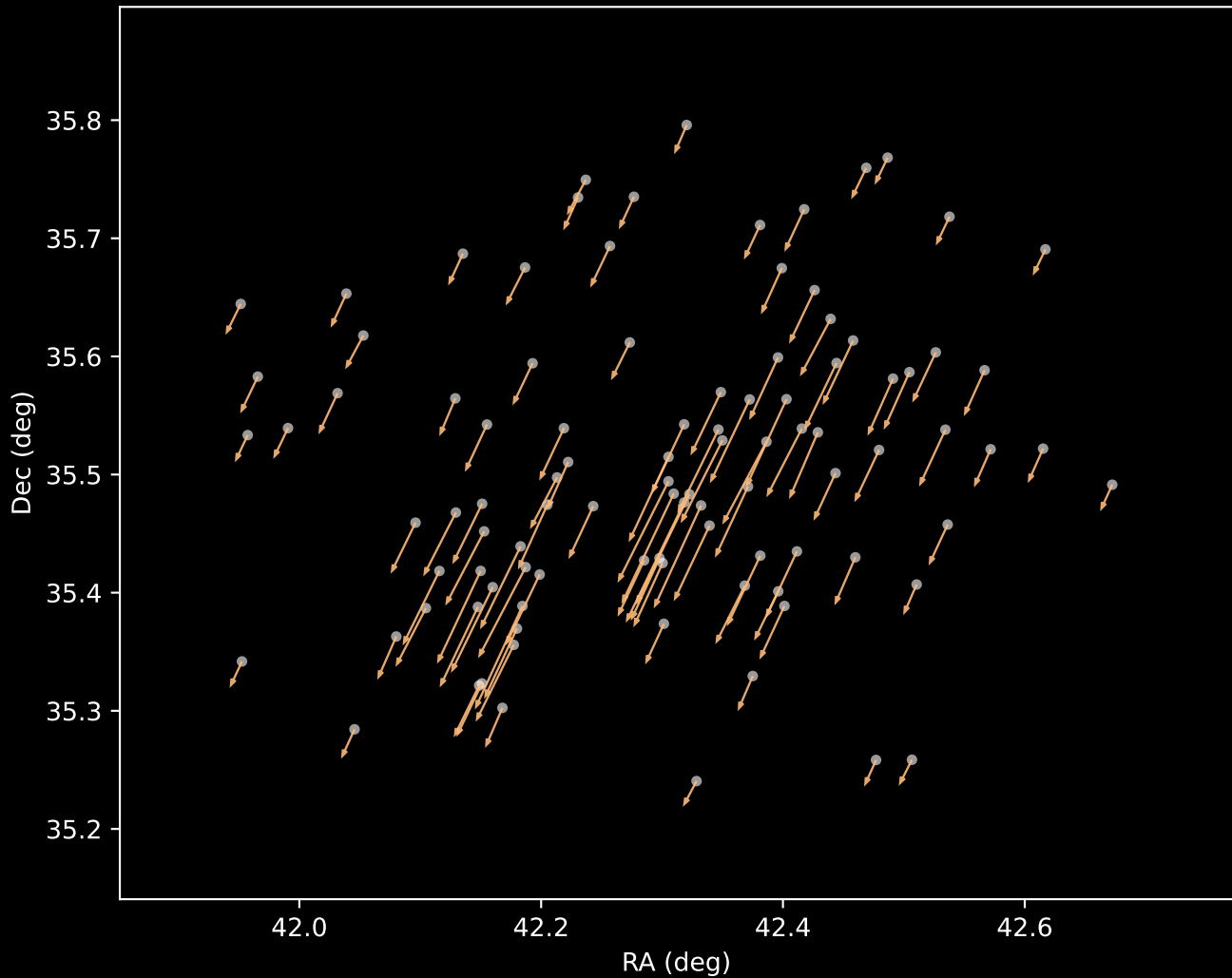
Gaia DR3 Cluster 3 Proper Motion Vectors (n=99)
