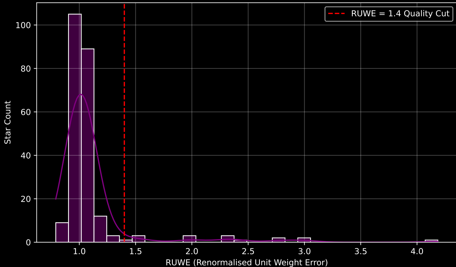
Gaia Cluster: [Biurakan_2] RUWE Distribution (n= 234)
