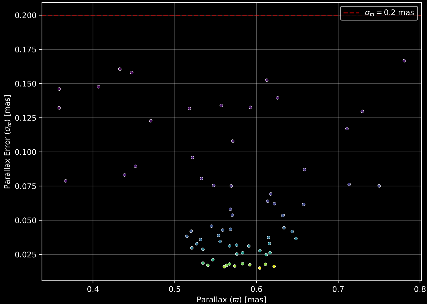
Gaia Cluster: [Bochum_13] Parallax Quality (n= 69)
