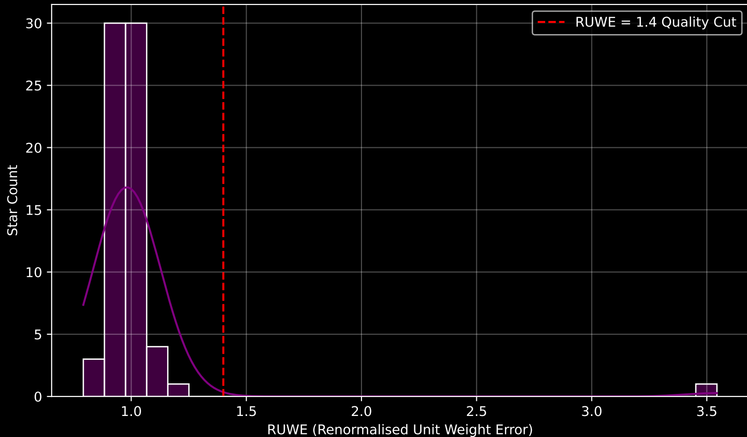
Gaia Cluster: [Bochum_13] RUWE Distribution (n= 69)
