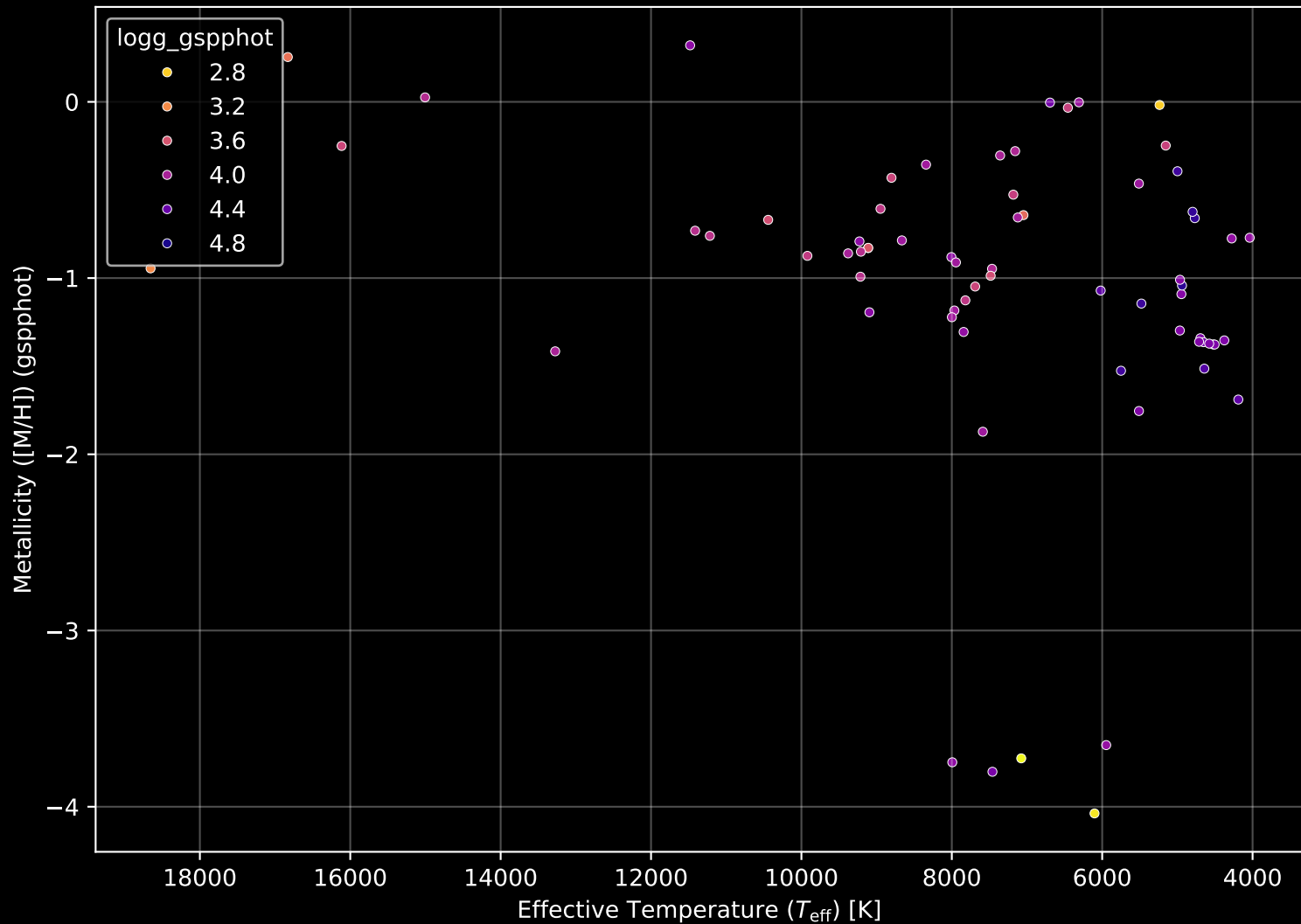
Gaia Cluster: [Bochum_13] Stellar Population Parameters (n= 69)
