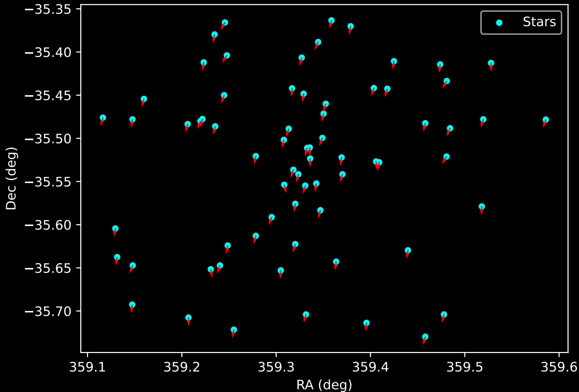
Gaia Cluster: [Bochum_13] Proper Motion Vectors for Gaia Star Field (n= 69)
