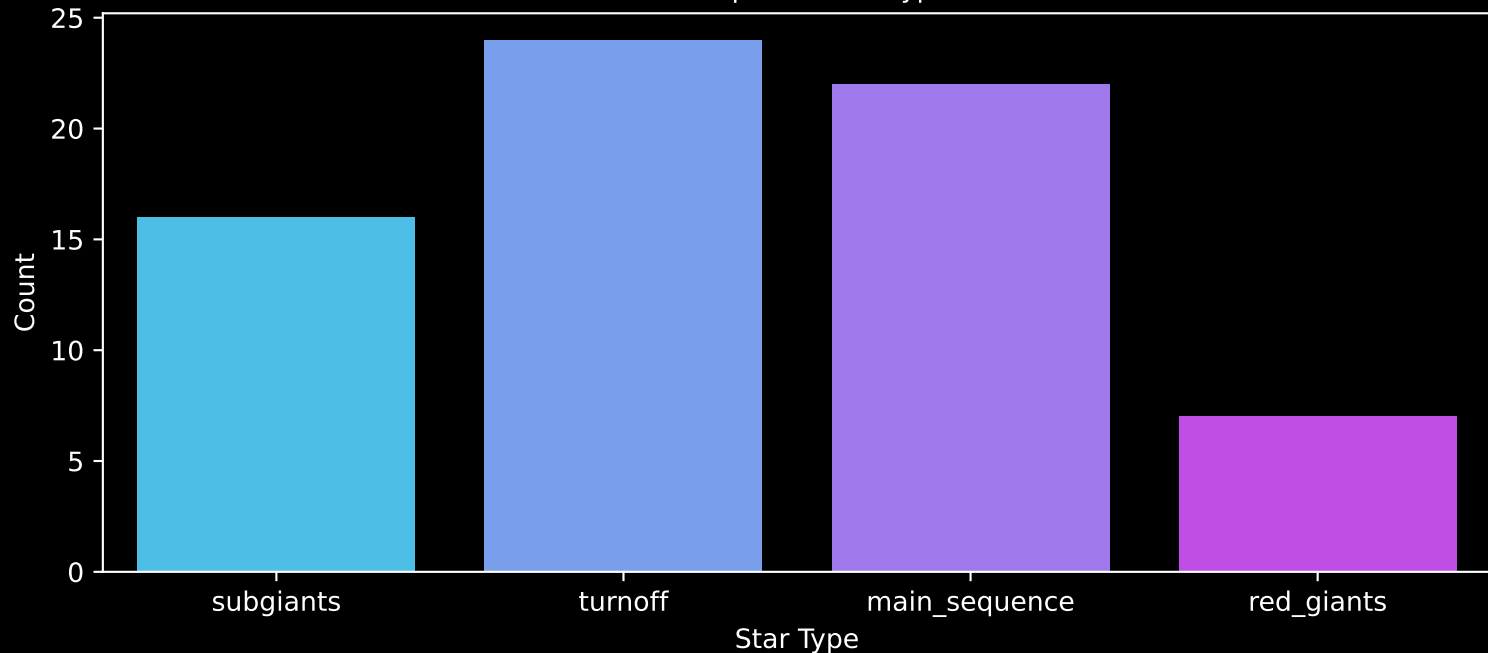
Gaia Cluster: [Bochum_13] Count plot of Star Type
