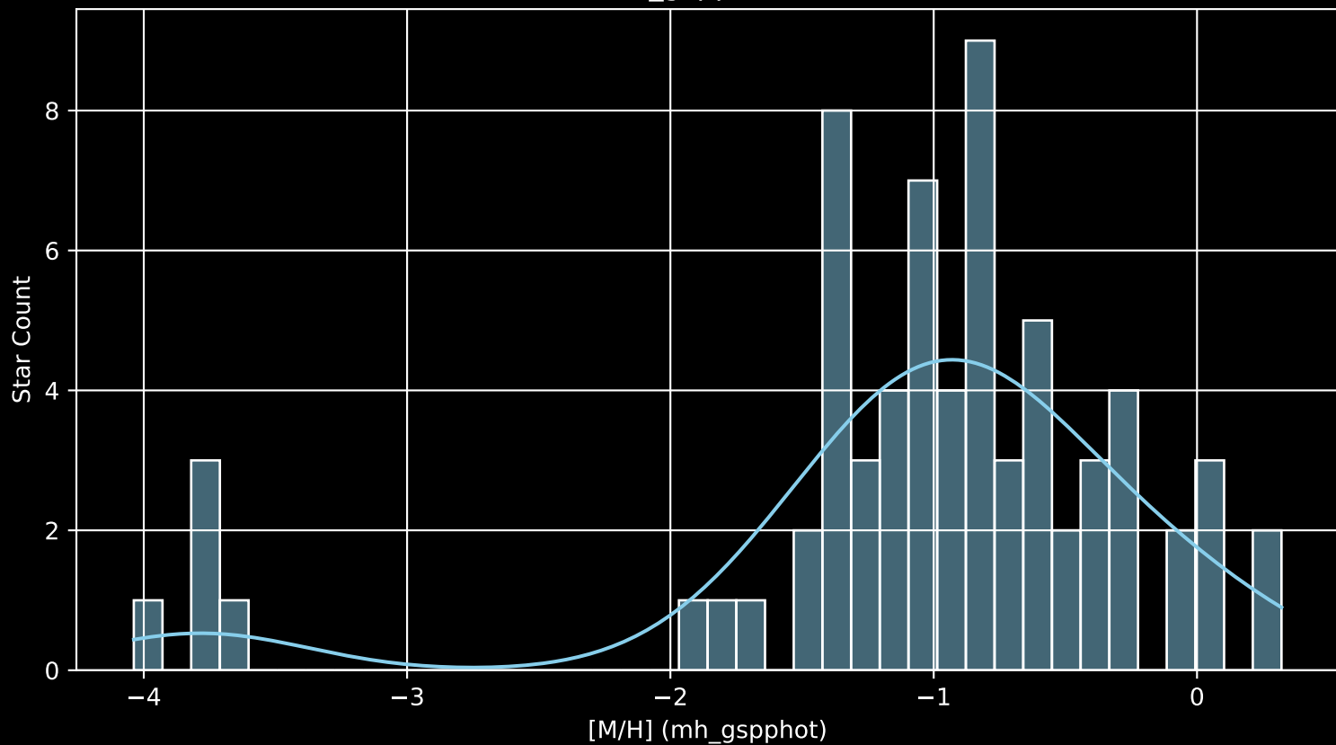
Gaia Cluster: [Bochum_13 [M/H] (mh_gspphot) (n= 69)
