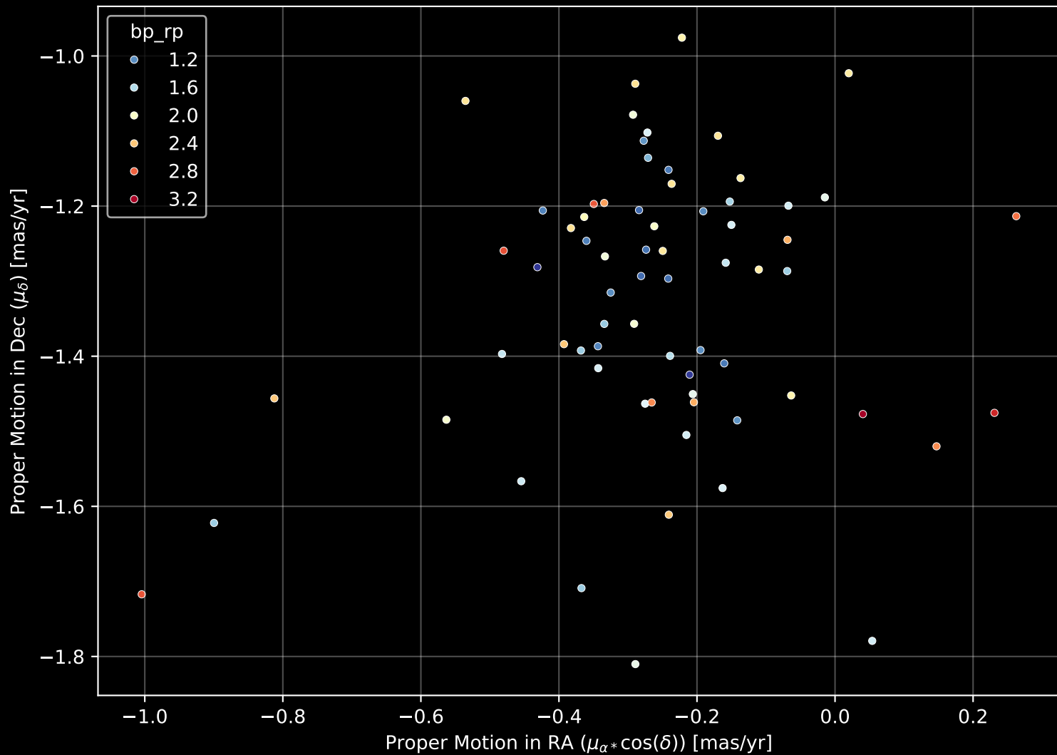
Gaia Cluster: [Bochum_13] Proper Motion Diagram (n= 69)
