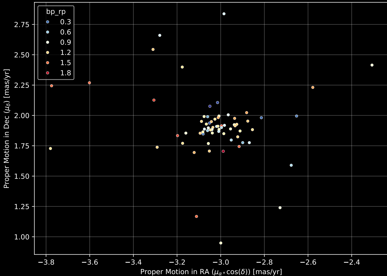
Gaia Cluster: [Bochum_4] Proper Motion Diagram (n= 68)
