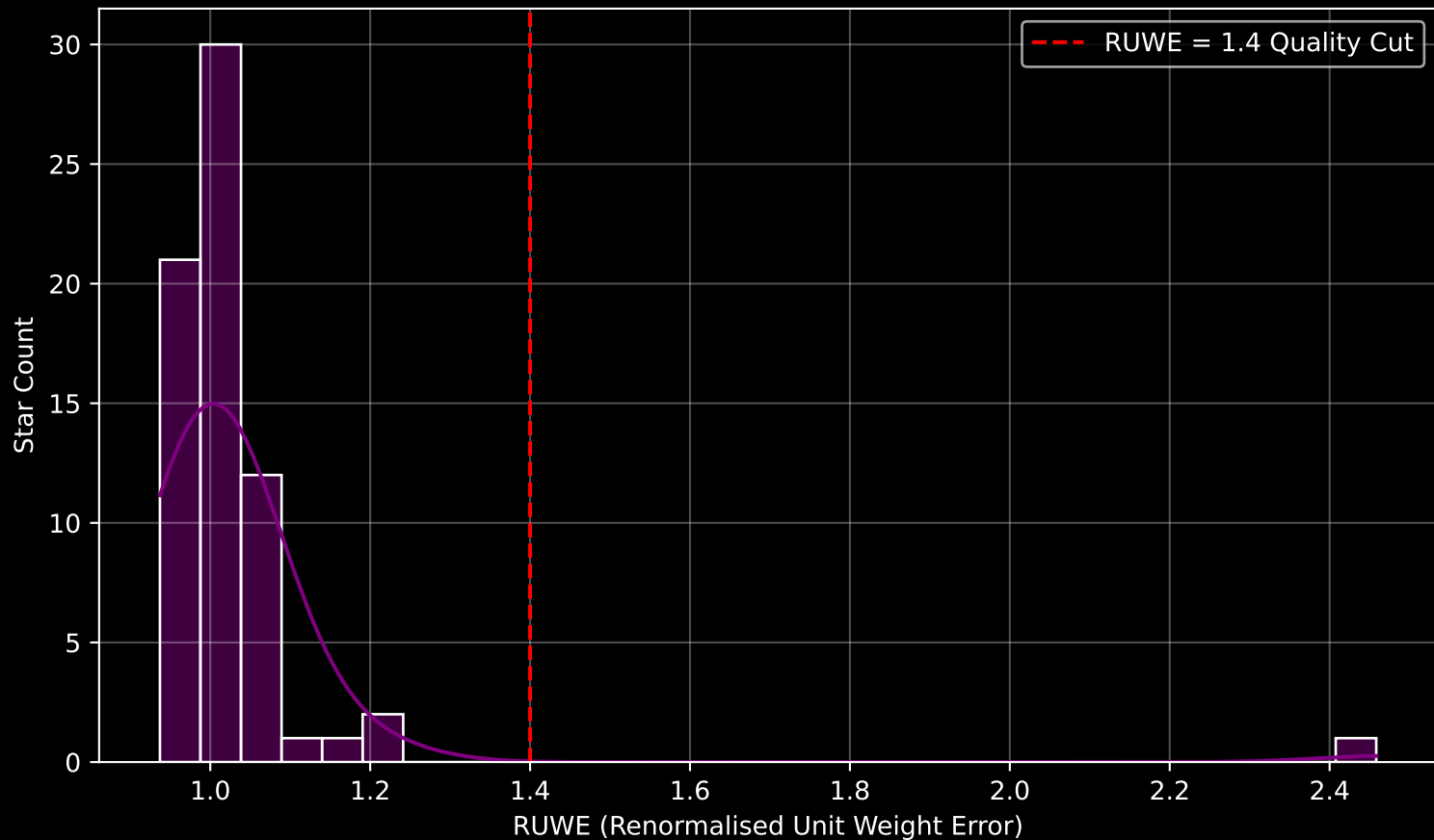
Gaia Cluster: [Bochum_4] RUWE Distribution (n= 68)
