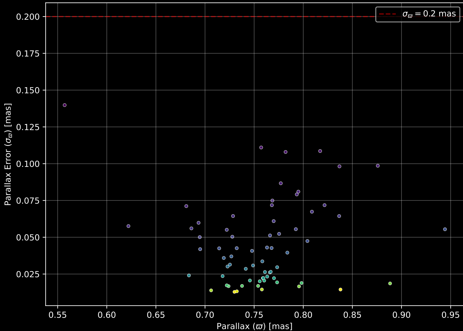
Gaia Cluster: [Bochum_4] Parallax Quality (n= 68)
