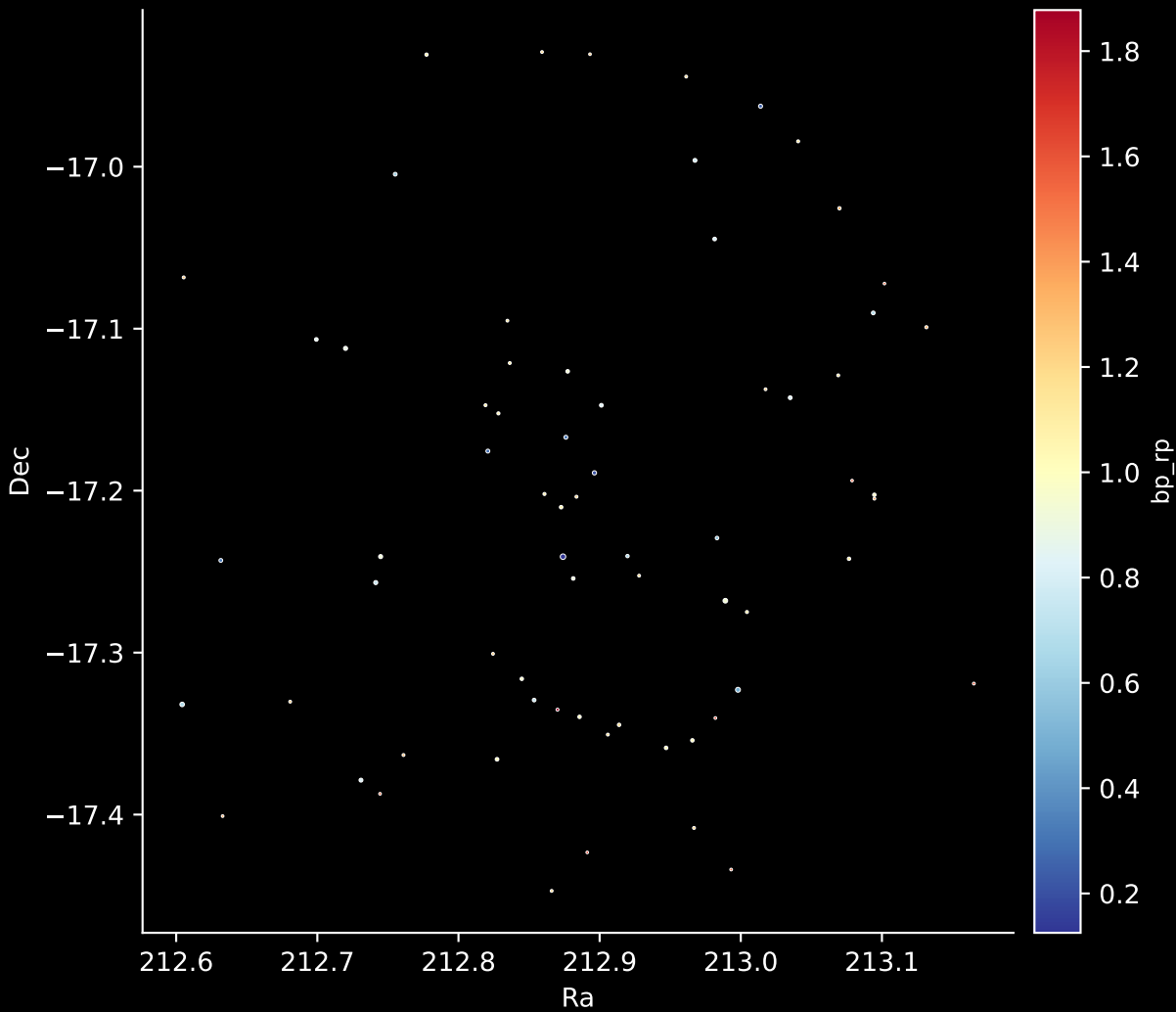
Gaia Cluster: [Bochum_4] Stars: 68
