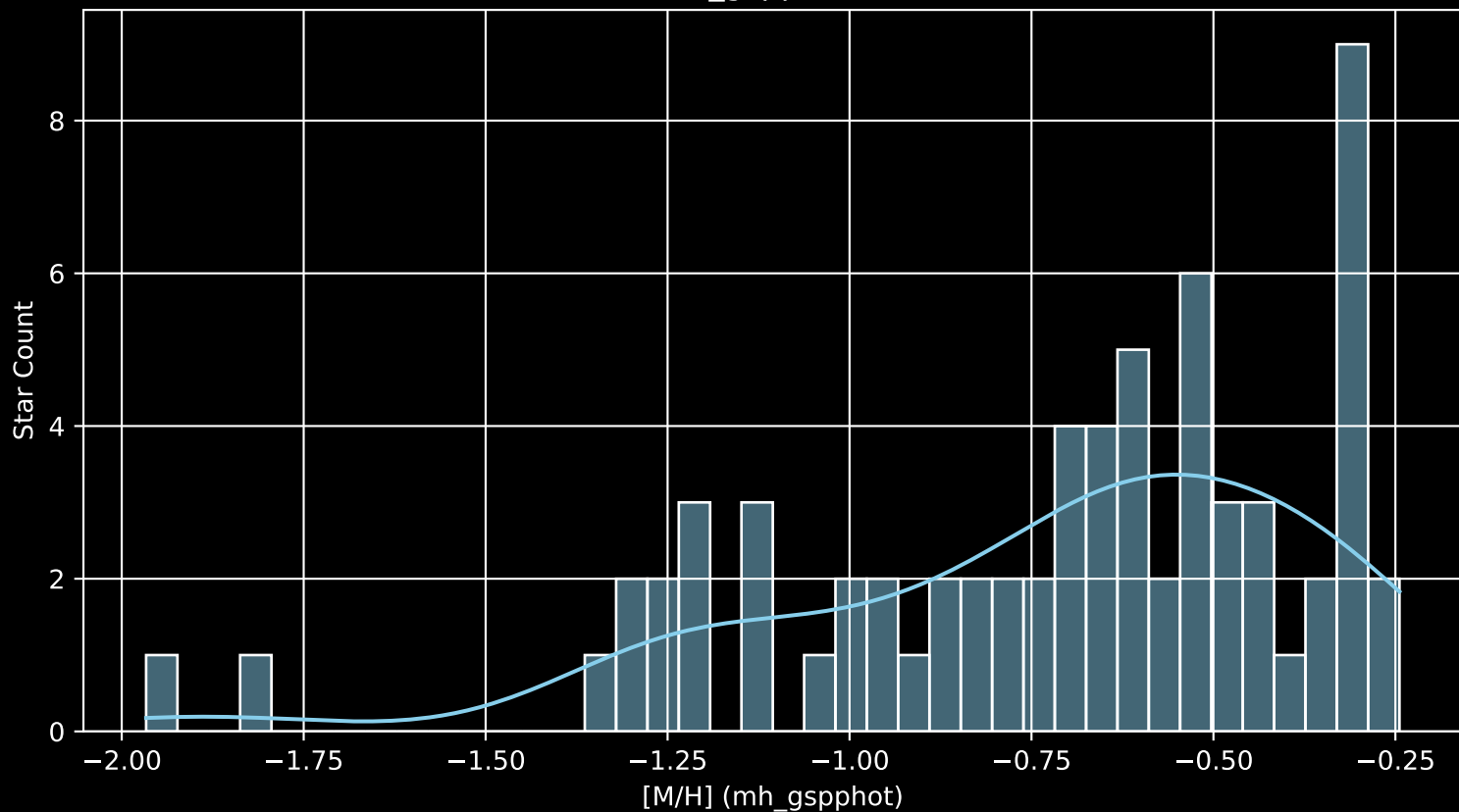
Gaia Cluster: [Bochum_4 [M/H] (mh_gspphot) (n= 68)
