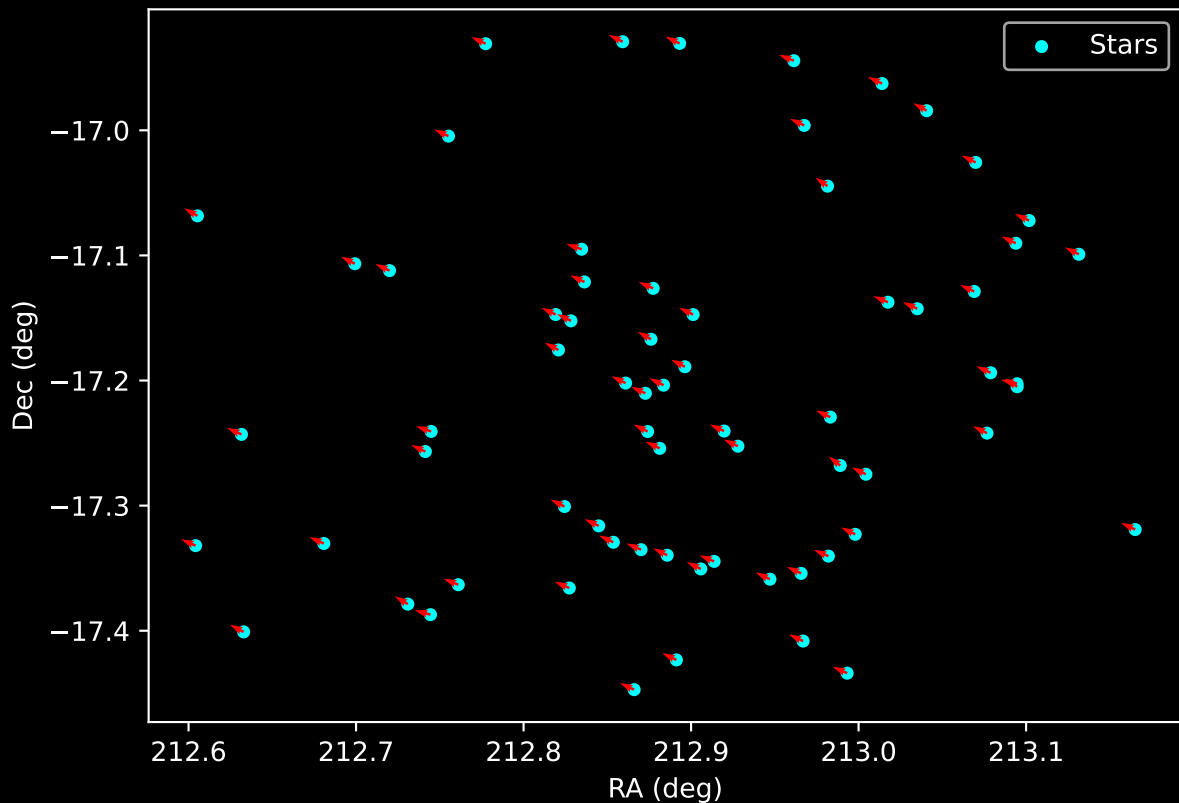
Gaia Cluster: [Bochum_4] Proper Motion Vectors for Gaia Star Field (n= 68)
