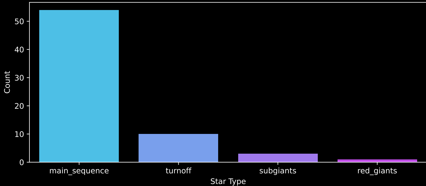
Gaia Cluster: [Bochum_4] Count plot of Star Type
