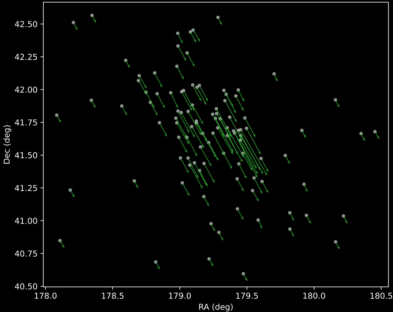
Gaia DR3 Cluster 4 Proper Motion Vectors (n=101)
