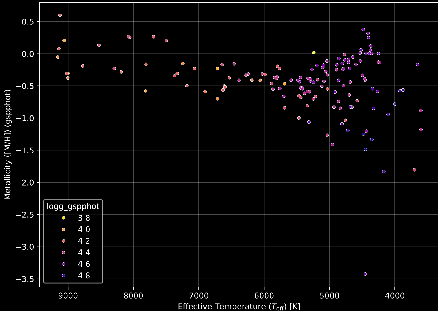
Gaia Cluster: [COIN-Gaia_12] Stellar Population Parameters (n= 150)
