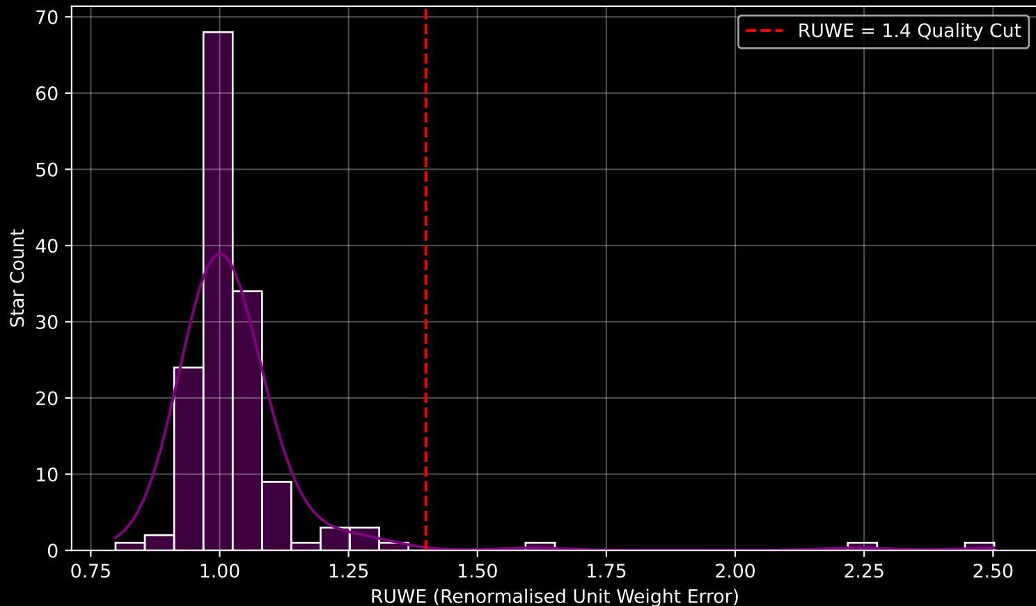
Gaia Cluster: [COIN-Gaia_12] RUWE Distribution (n= 149)
