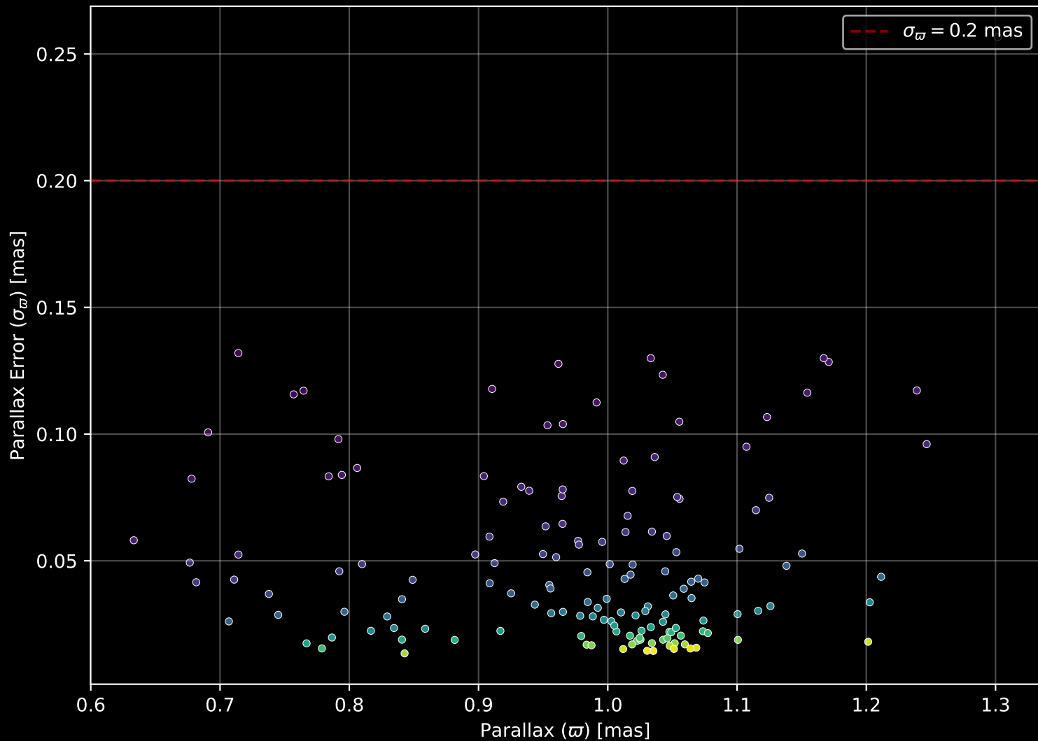
Gaia Cluster: [COIN-Gaia_12] Parallax Quality (n= 150)
