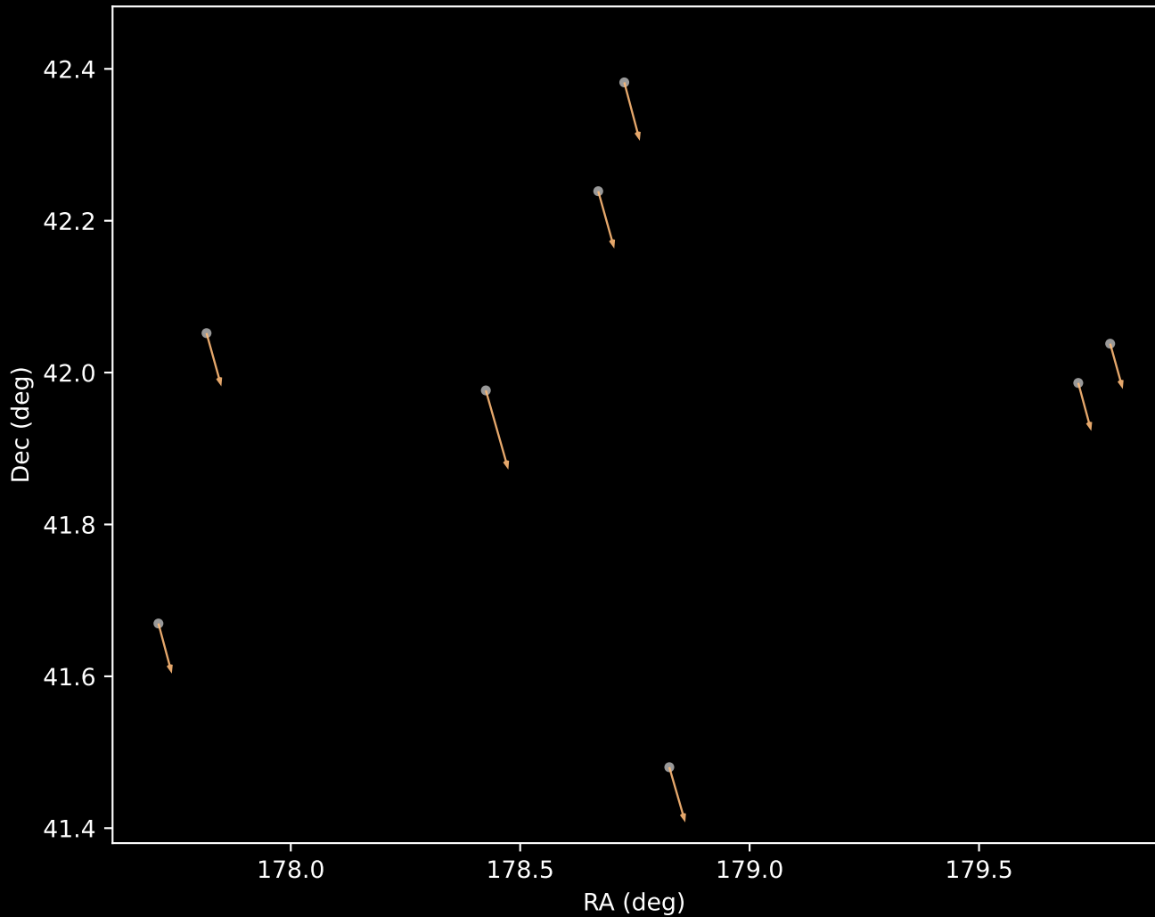
Gaia DR3 Cluster 3 Proper Motion Vectors (n=8)
