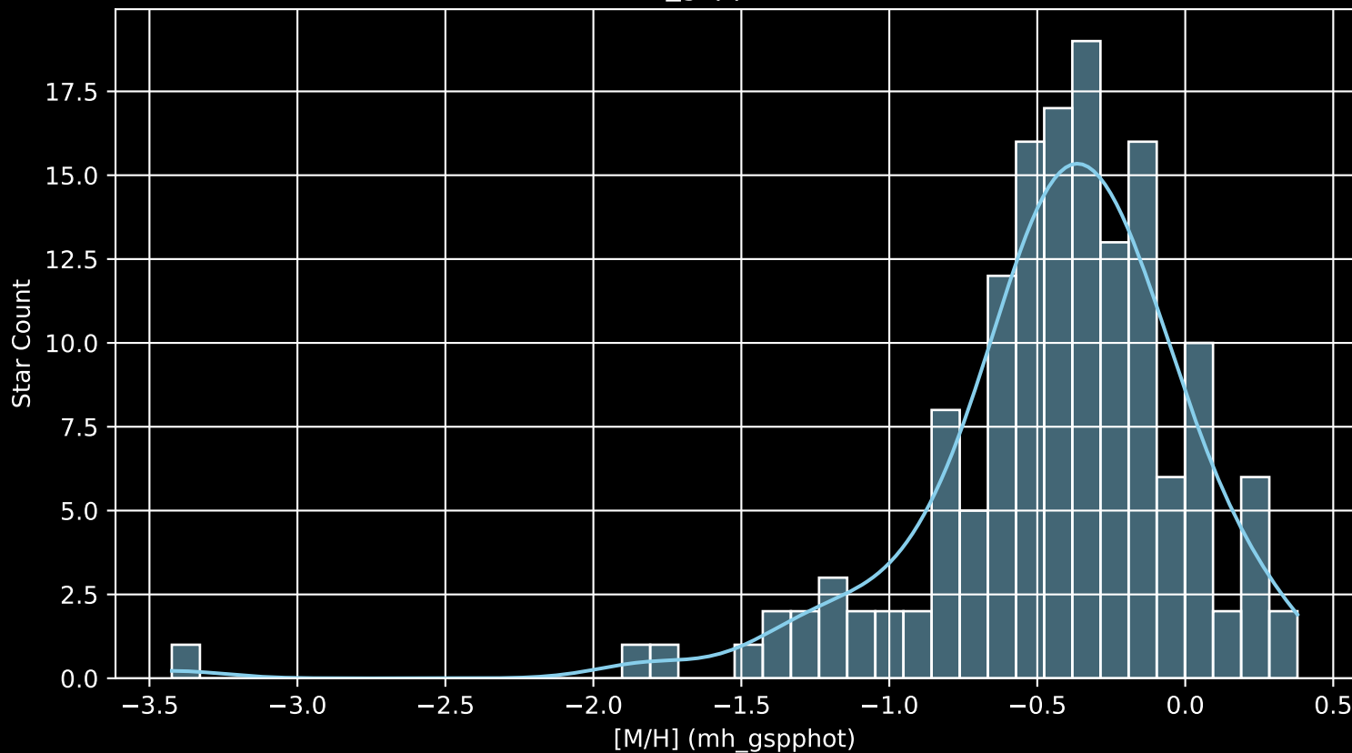
Gaia Cluster: [COIN-Gaia_12 [M/H] (mh_gspphot) (n= 149)
