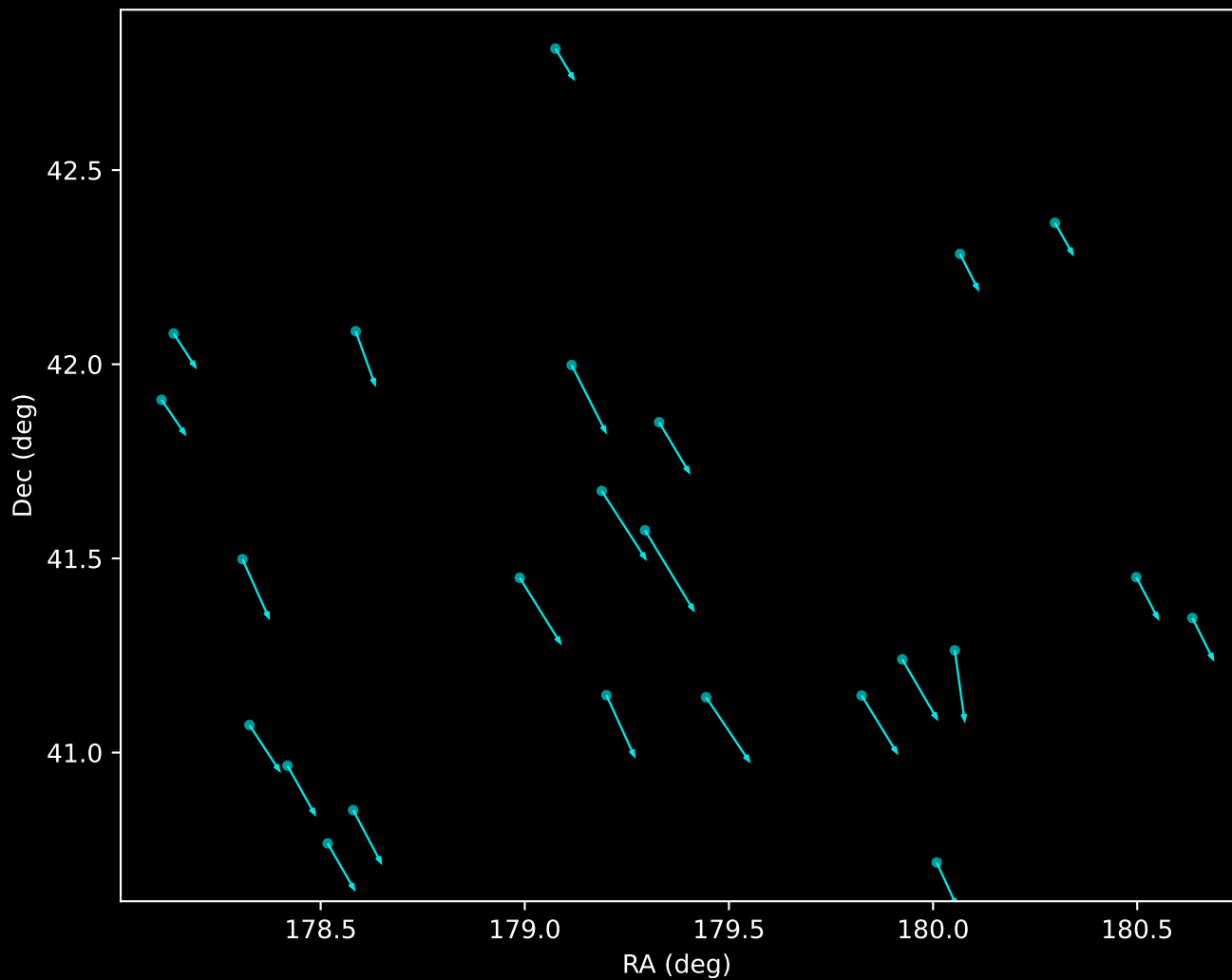
Gaia DR3 Noise Stream Proper Motion Vectors (n=24)
