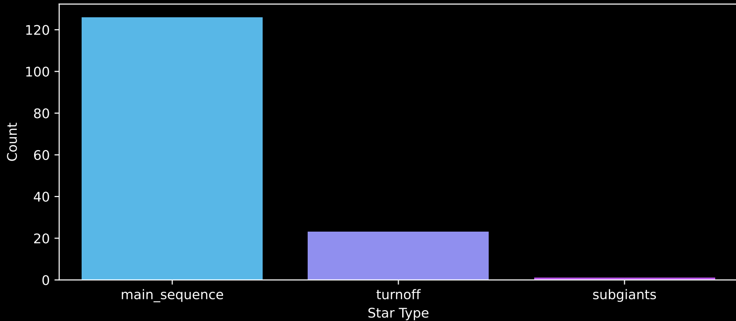
Gaia Cluster: [COIN-Gaia_12] Count plot of Star Type
