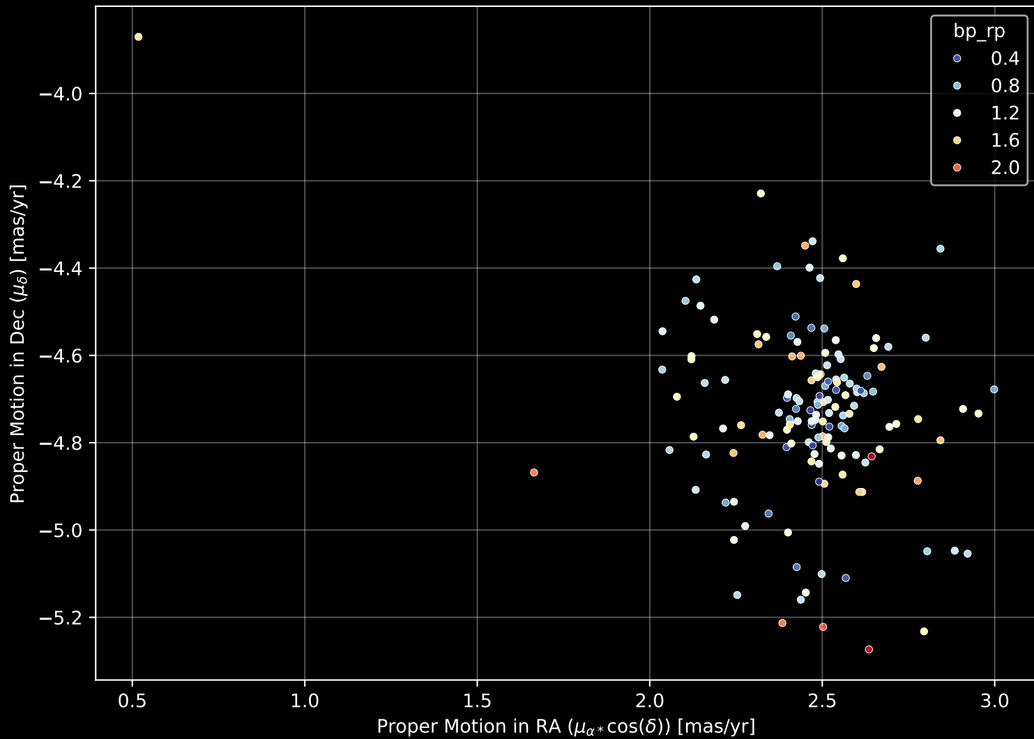
Gaia Cluster: [COIN-Gaia_12] Proper Motion Diagram (n= 150)
