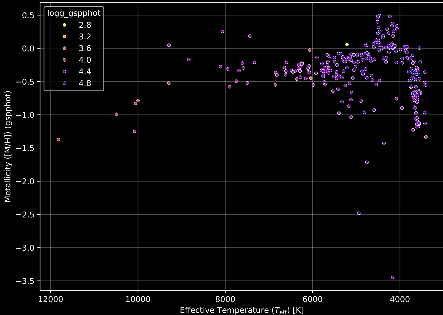
Gaia Cluster: [COIN-Gaia_13] Stellar Population Parameters (n= 268)
