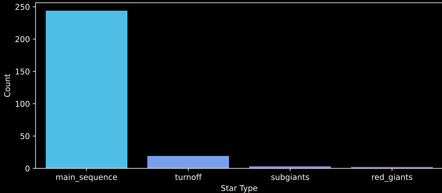
Gaia Cluster: [COIN-Gaia_13] Count plot of Star Type
