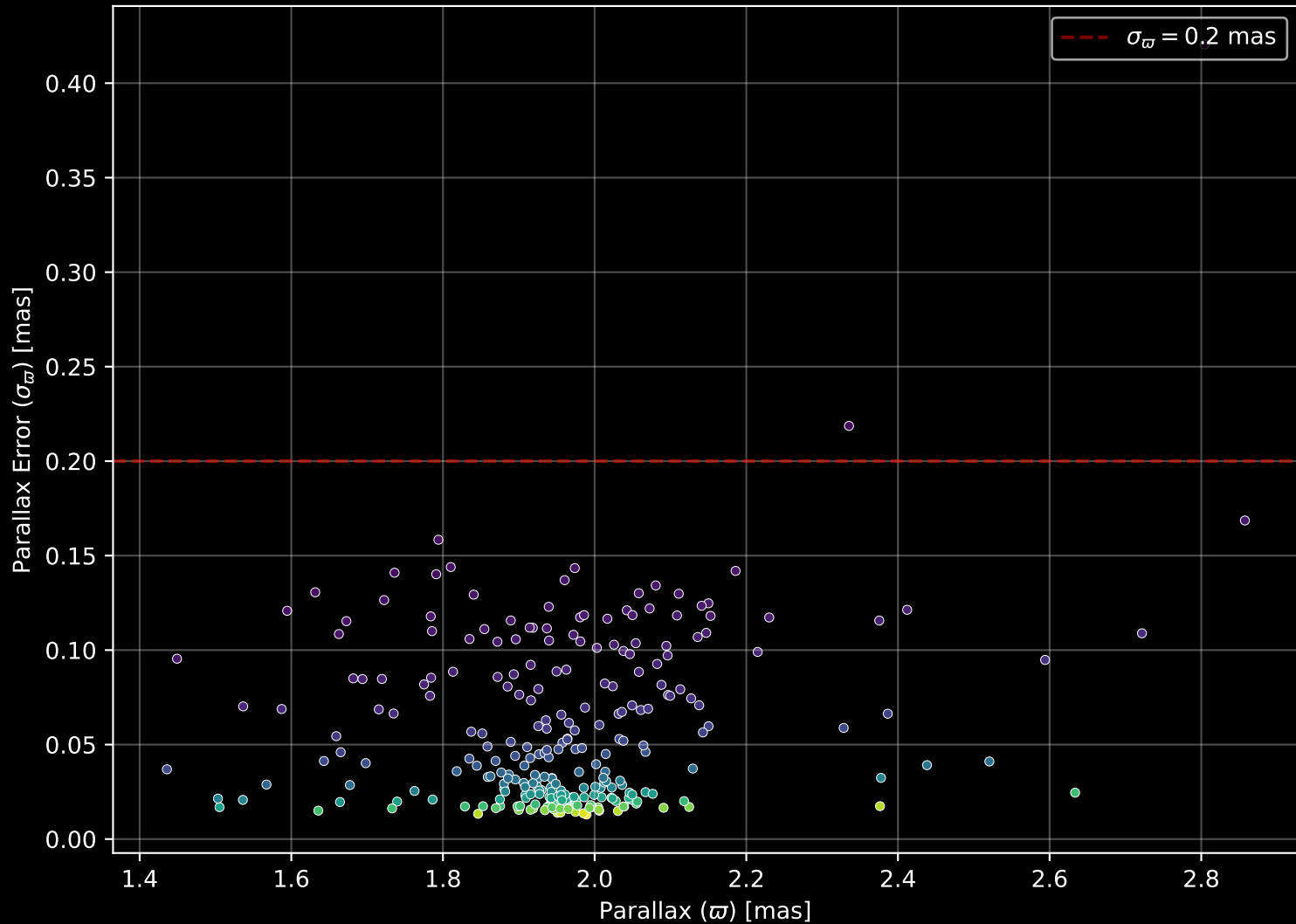
Gaia Cluster: [COIN-Gaia_13] Parallax Quality (n= 268)
