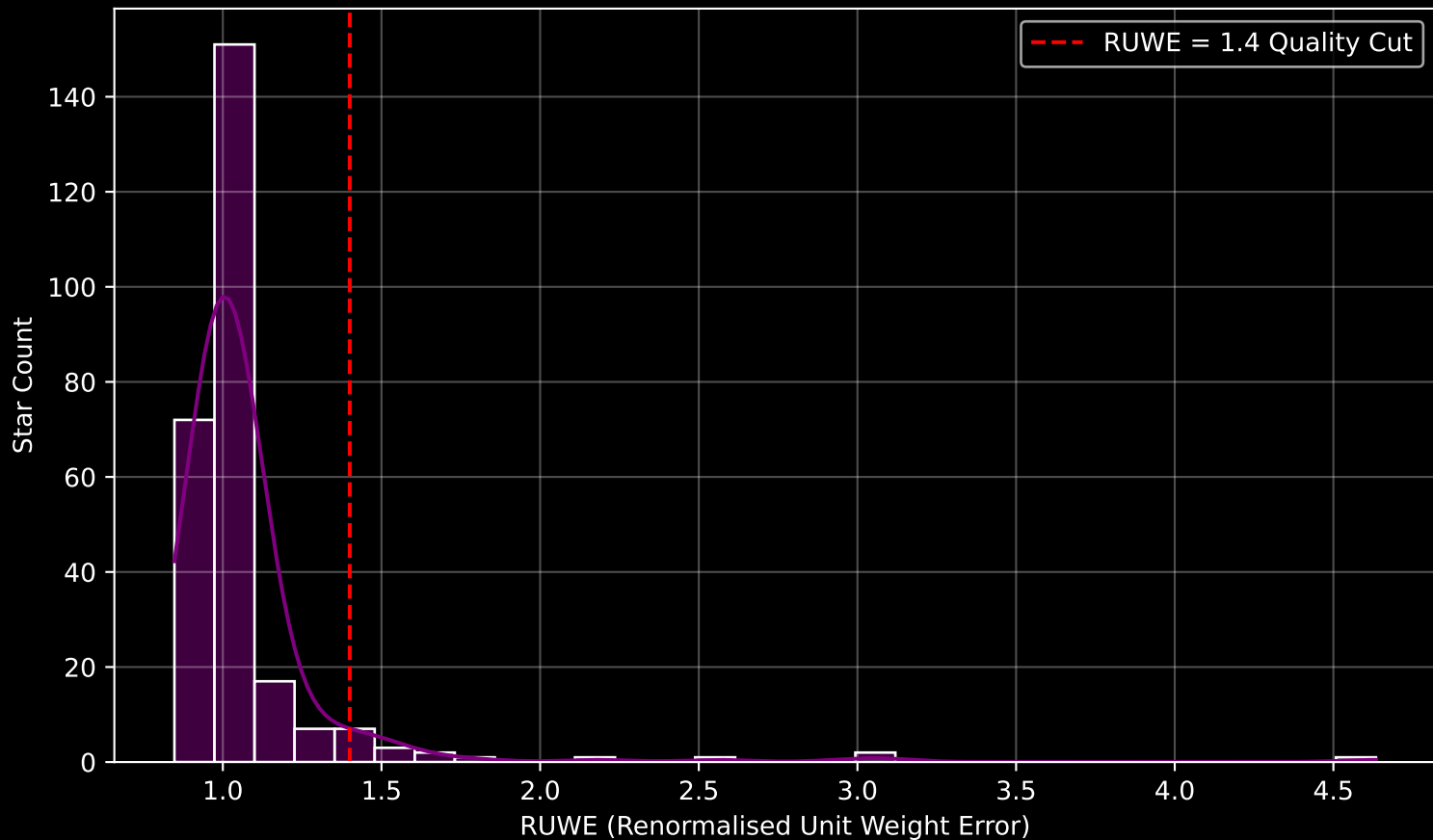
Gaia Cluster: [COIN-Gaia_13] RUWE Distribution (n= 265)
