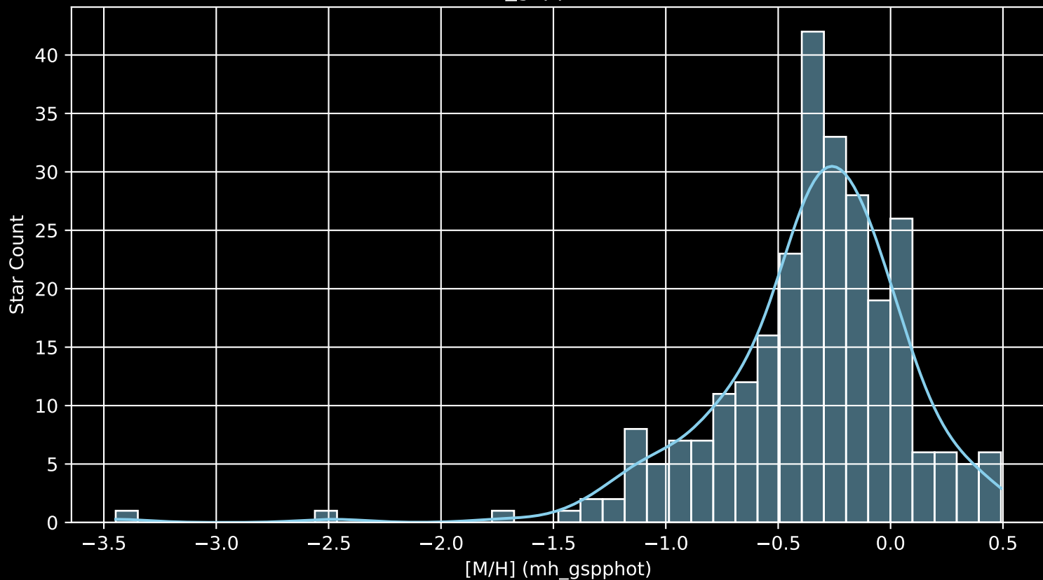
Gaia Cluster: [COIN-Gaia_13 [M/H] (mh_gspphot) (n= 268)
