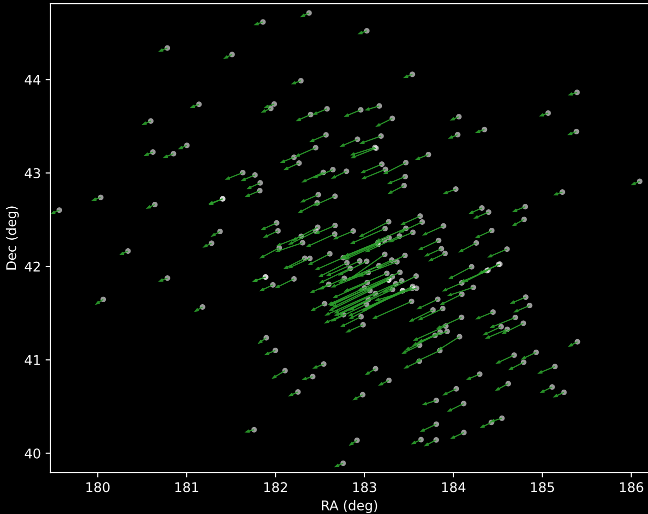
Gaia DR3 Cluster 4 Proper Motion Vectors (n=197)
