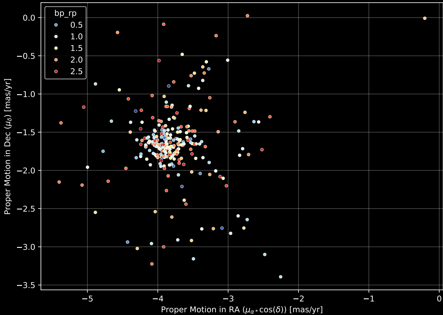
Gaia Cluster: [COIN-Gaia_13] Proper Motion Diagram (n= 268)
