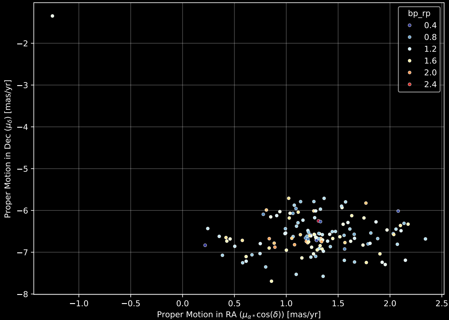
Gaia Cluster: [COIN-Gaia_14] Proper Motion Diagram (n= 139)
