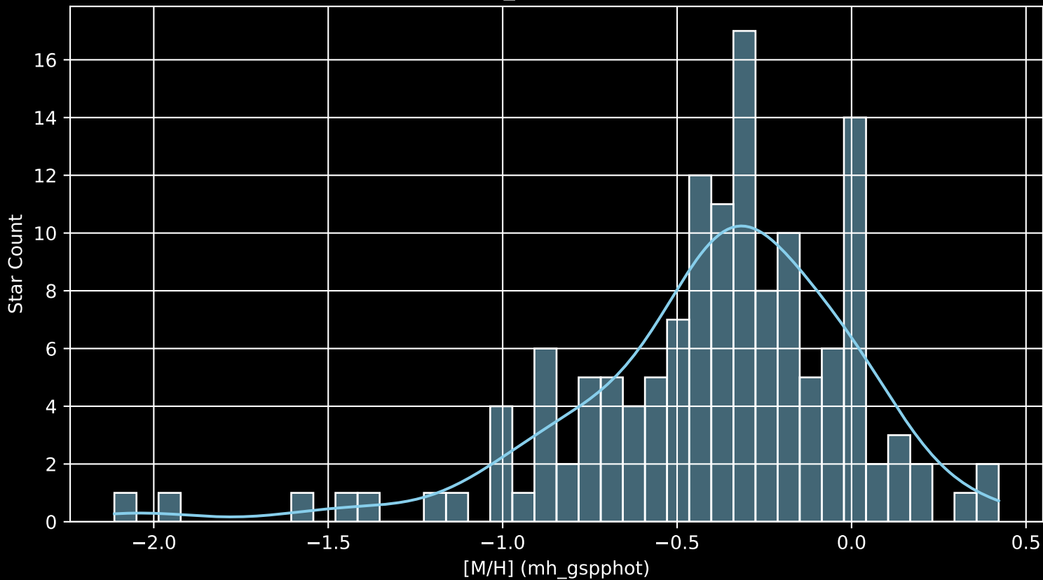
Gaia Cluster: [COIN-Gaia_14 [M/H] (mh_gspphot) (n= 139)
