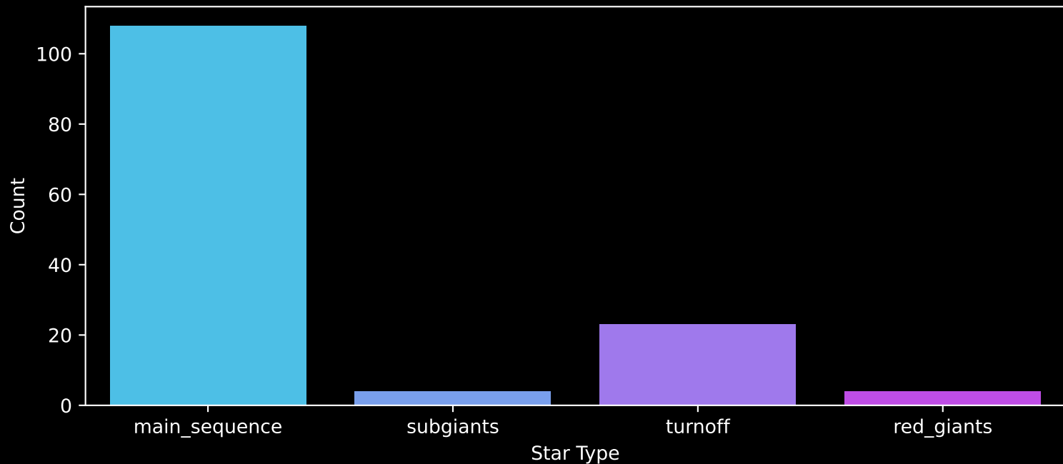
Gaia Cluster: [COIN-Gaia_14] Count plot of Star Type
