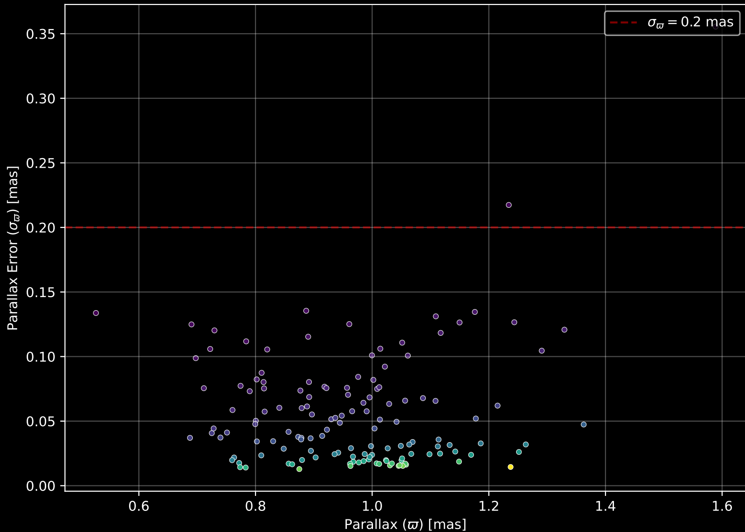
Gaia Cluster: [COIN-Gaia_14] Parallax Quality (n= 139)
