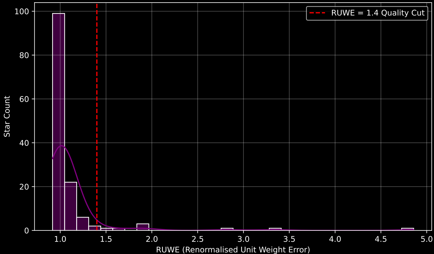
Gaia Cluster: [COIN-Gaia_14] RUWE Distribution (n= 137)
