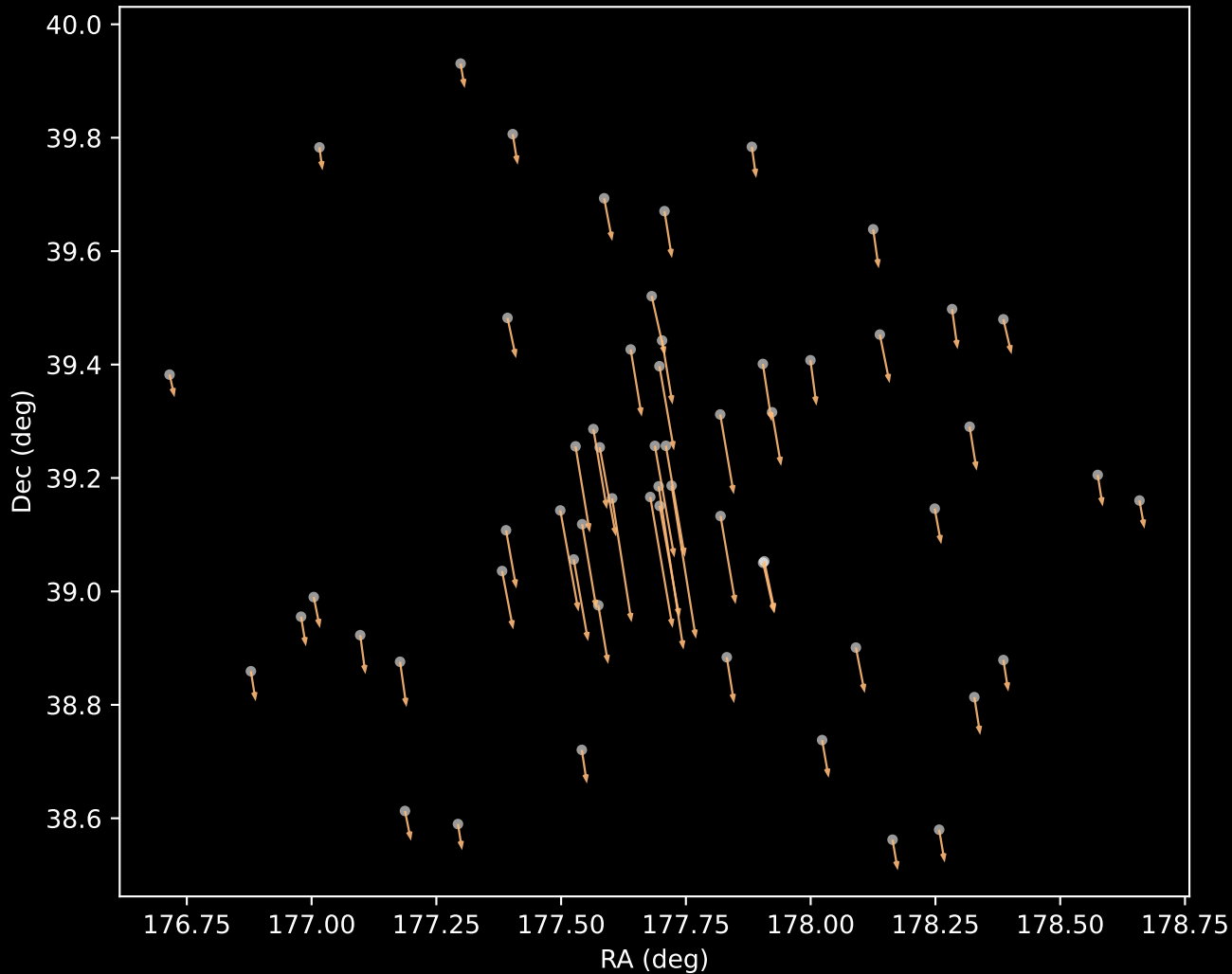
Gaia DR3 Cluster 3 Proper Motion Vectors (n=58)
