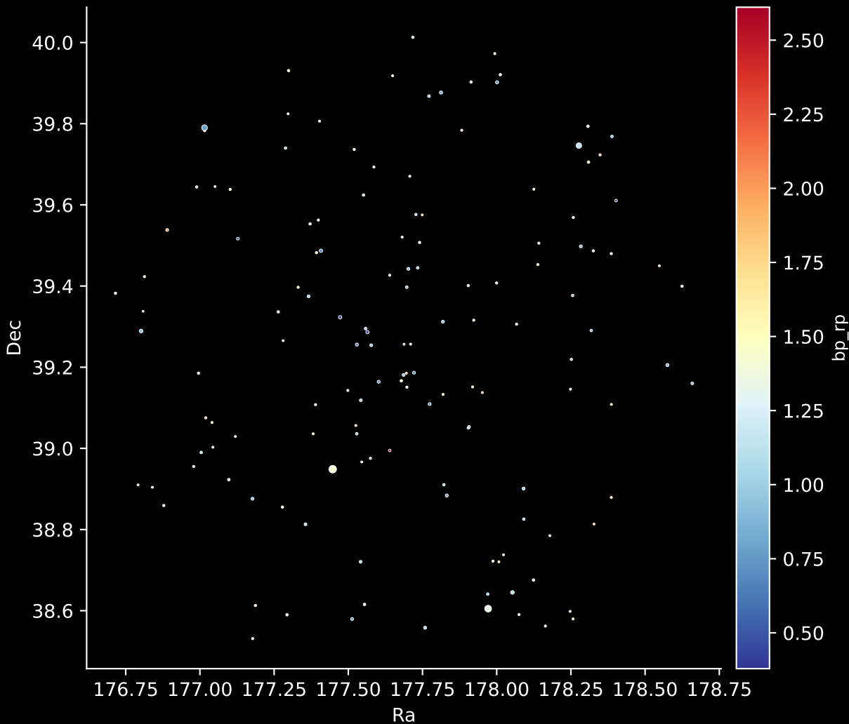
Gaia Cluster: [COIN-Gaia_14] Stars: 139
