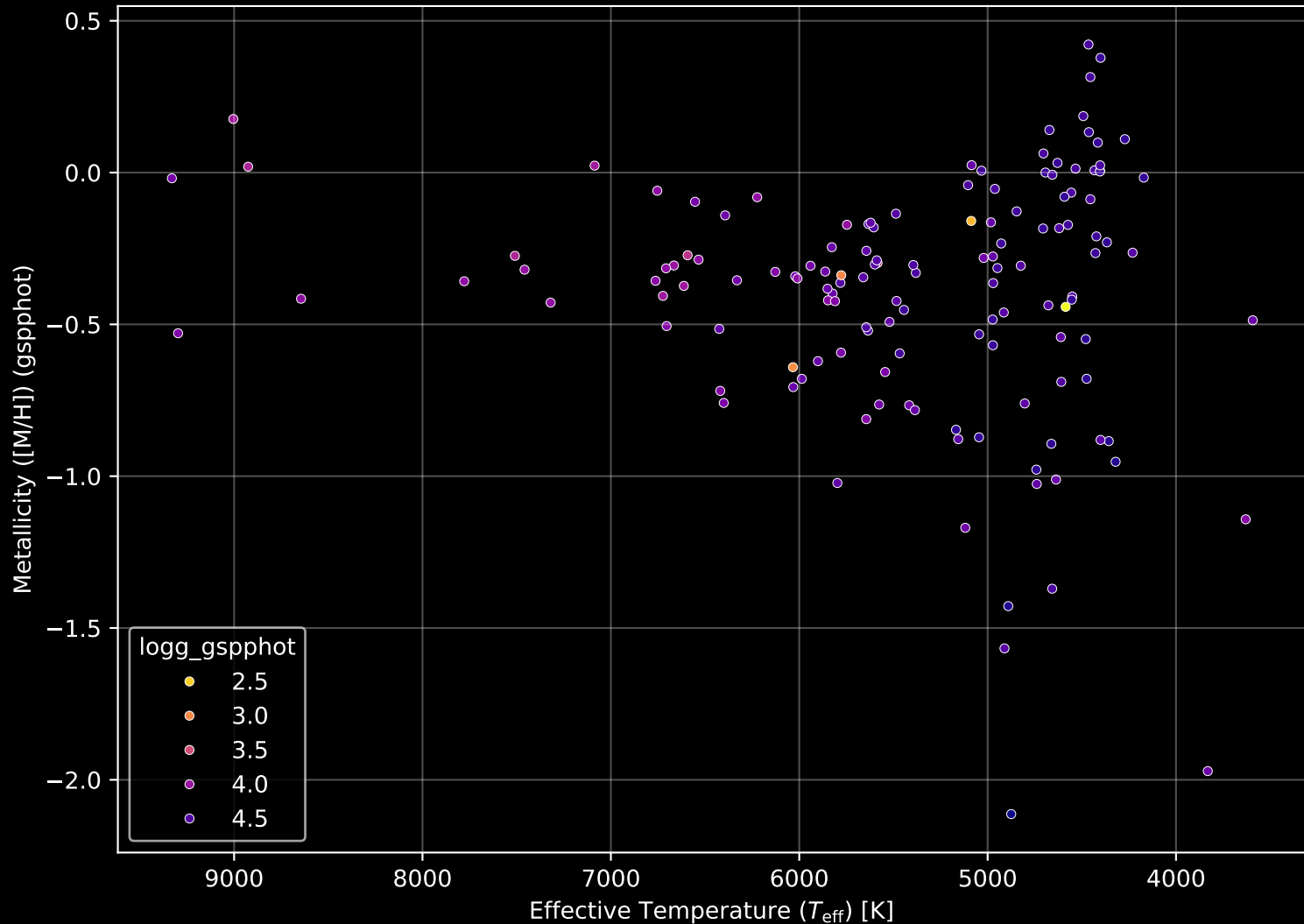
Gaia Cluster: [COIN-Gaia_14] Stellar Population Parameters (n= 139)
