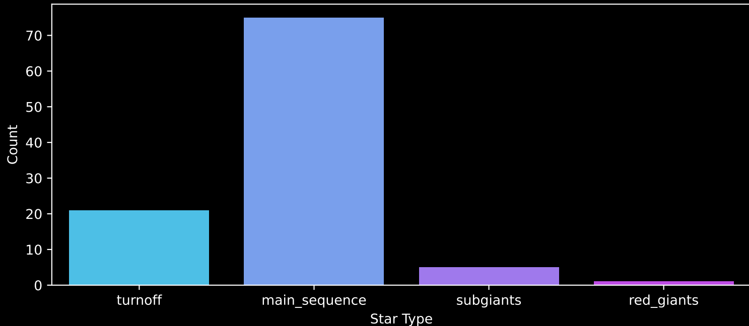
Gaia Cluster: [COIN-Gaia_16] Count plot of Star Type
