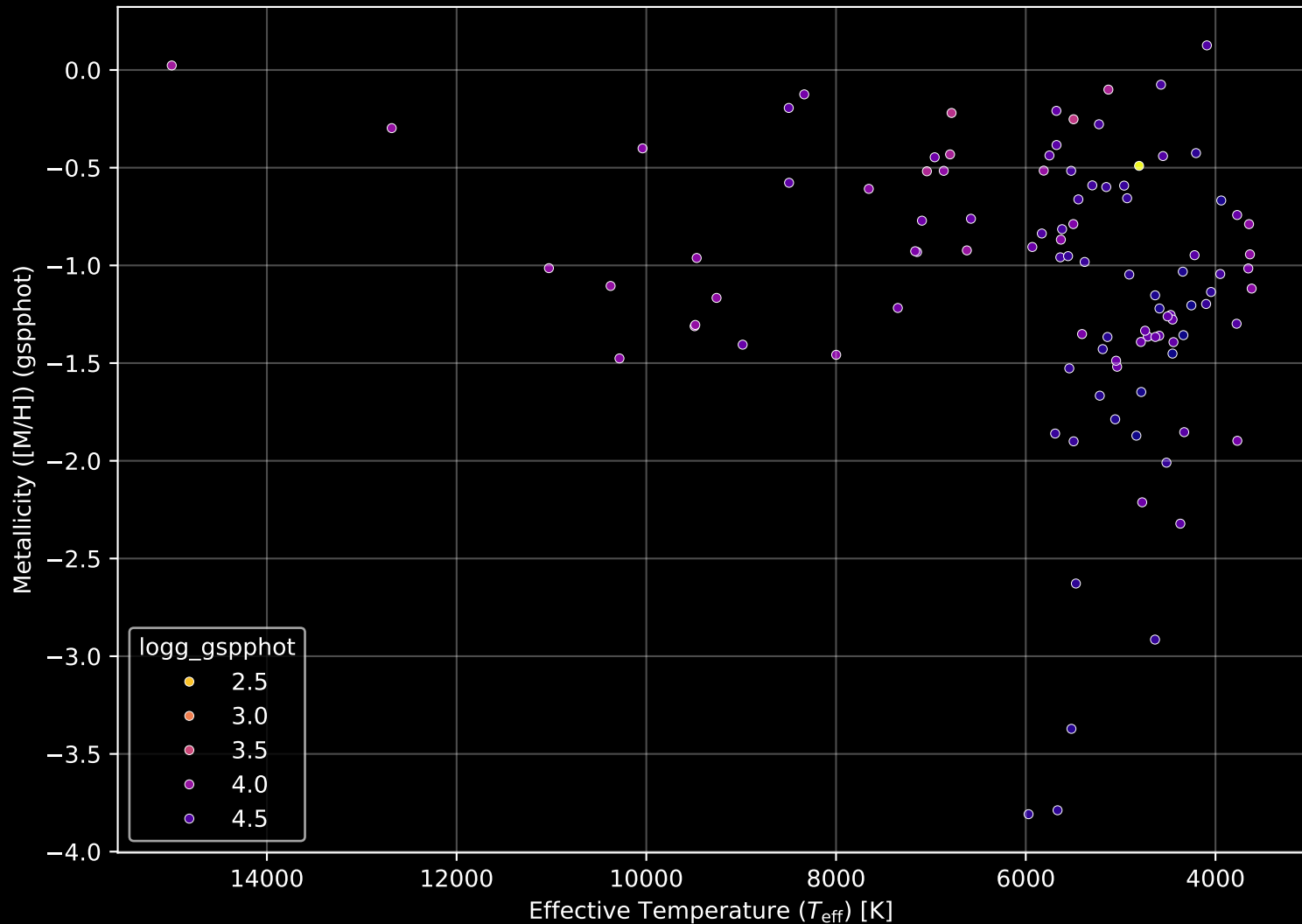
Gaia Cluster: [COIN-Gaia_16] Stellar Population Parameters (n= 102)
