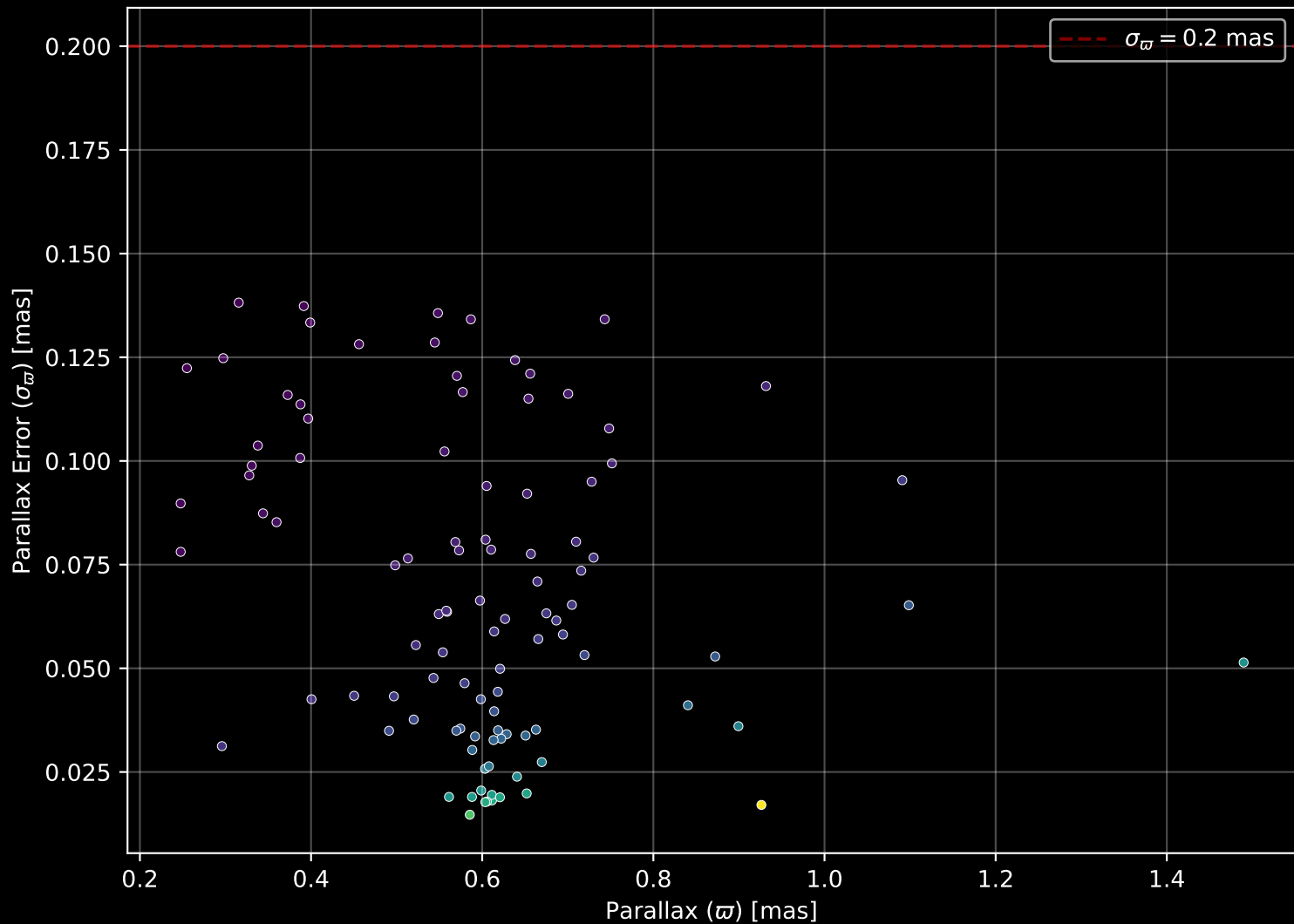
Gaia Cluster: [COIN-Gaia_16] Parallax Quality (n= 102)
