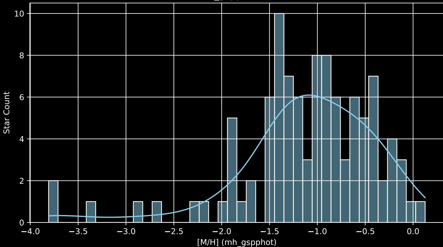
Gaia Cluster: [COIN-Gaia_16 [M/H] (mh_gspphot) (n= 102)
