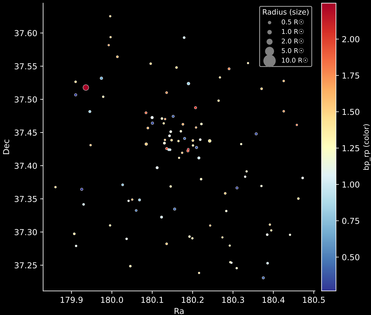
Gaia Cluster: [COIN-Gaia_16] Stars: 102
