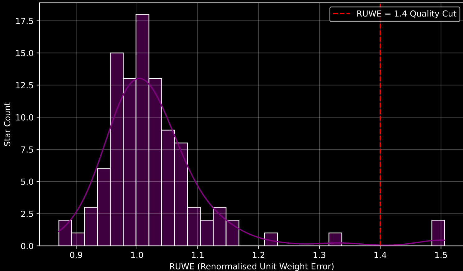
Gaia Cluster: [COIN-Gaia_16] RUWE Distribution (n= 102)
