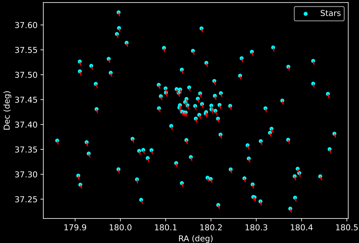
Gaia Cluster: [COIN-Gaia_16] Proper Motion Vectors for Gaia Star Field (n= 102)
