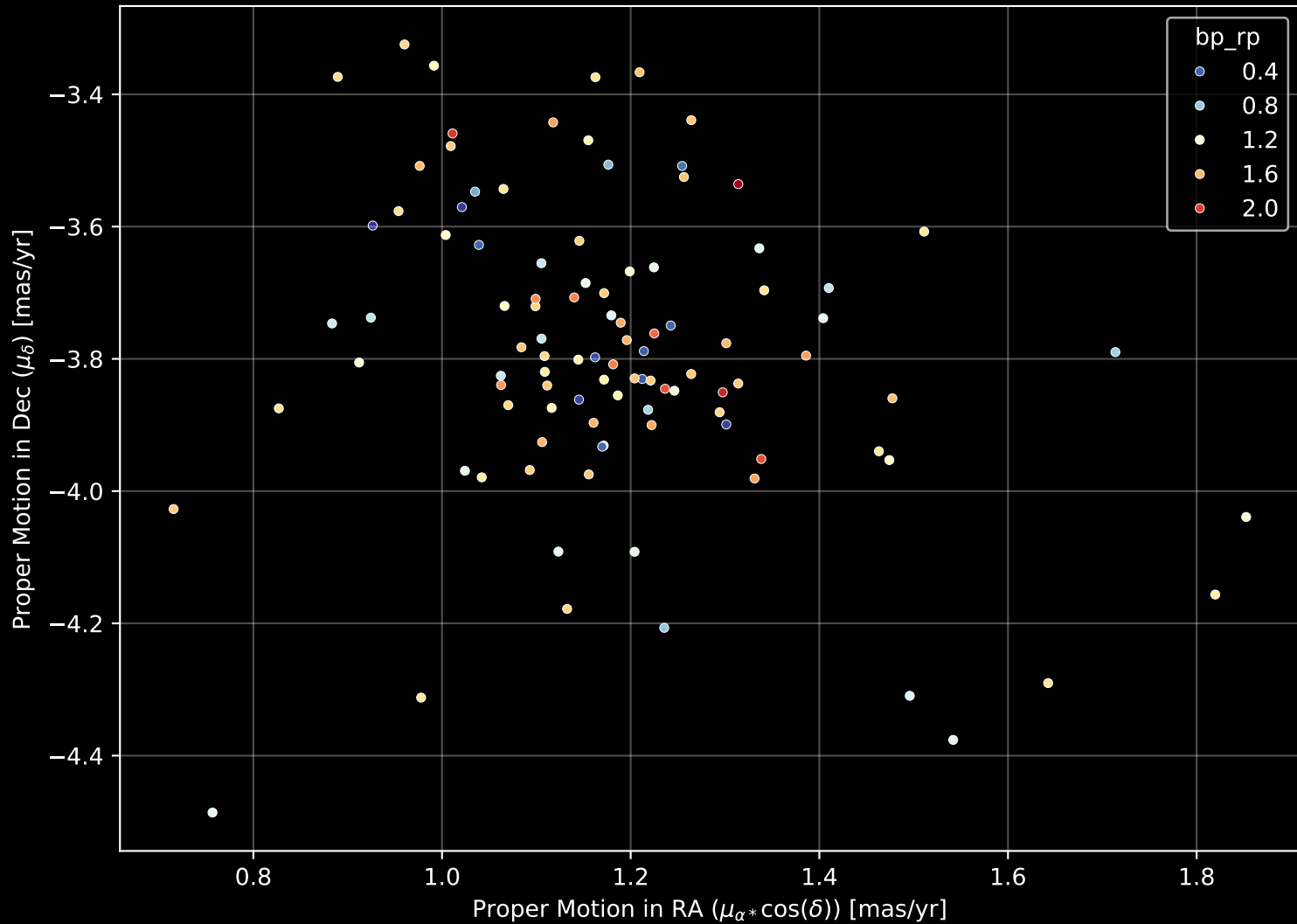
Gaia Cluster: [COIN-Gaia_16] Proper Motion Diagram (n= 102)
