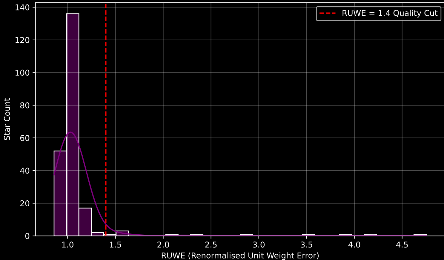
Gaia Cluster: [COIN-Gaia_24] RUWE Distribution (n= 218)
