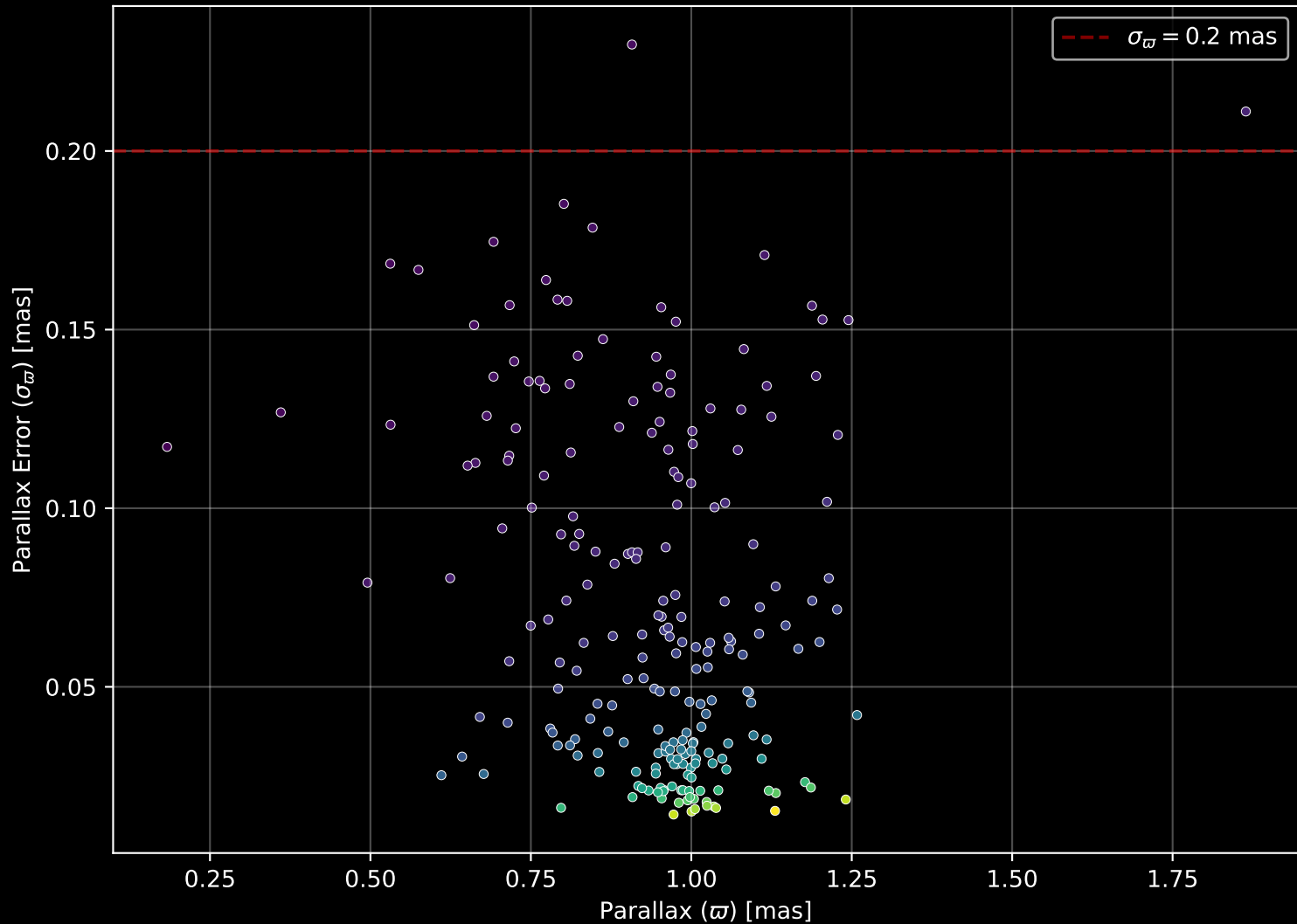
Gaia Cluster: [COIN-Gaia_24] Parallax Quality (n= 220)
