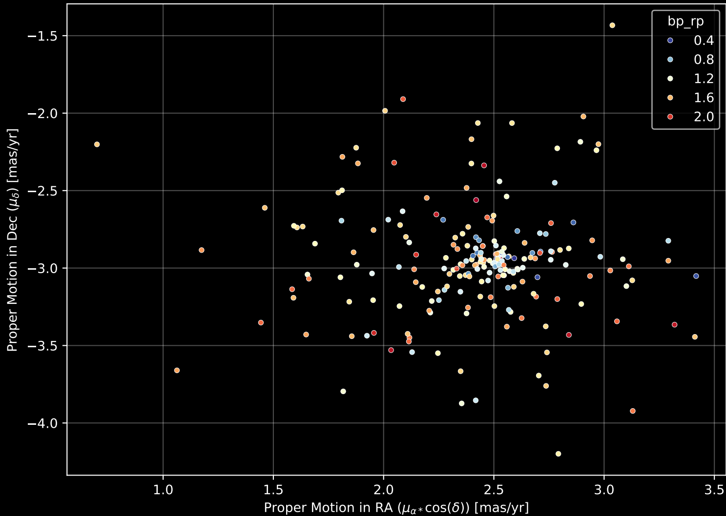
Gaia Cluster: [COIN-Gaia_24] Proper Motion Diagram (n= 220)
