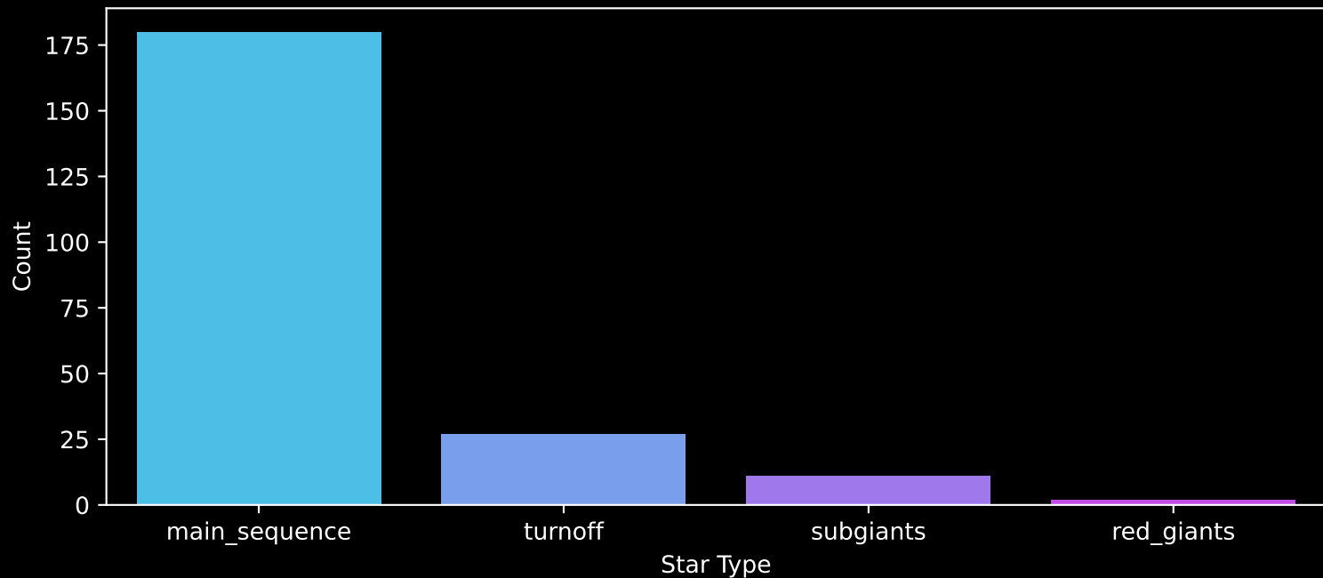
Gaia Cluster: [COIN-Gaia_24] Count plot of Star Type
