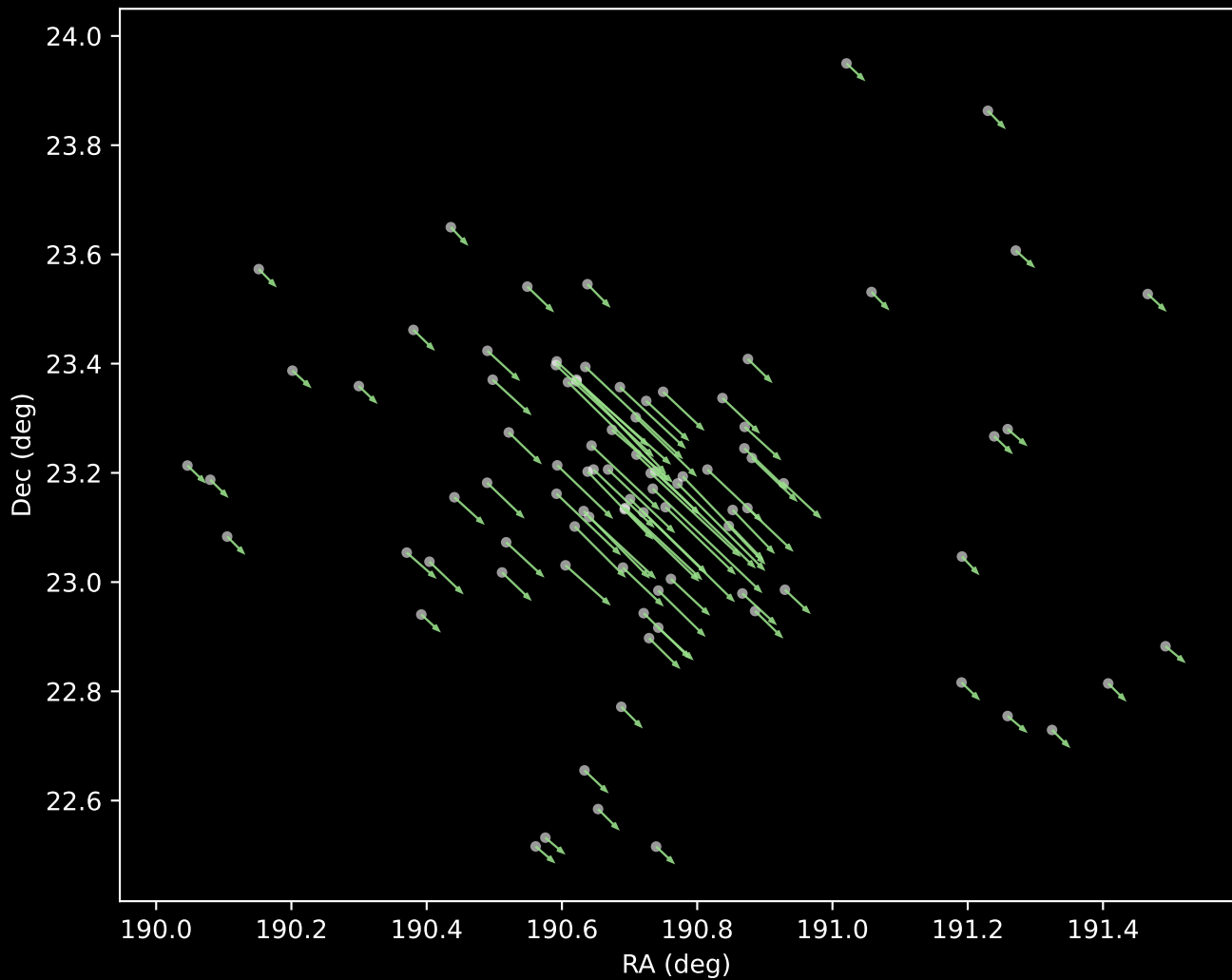
Gaia DR3 Cluster 5 Proper Motion Vectors (n=90)
