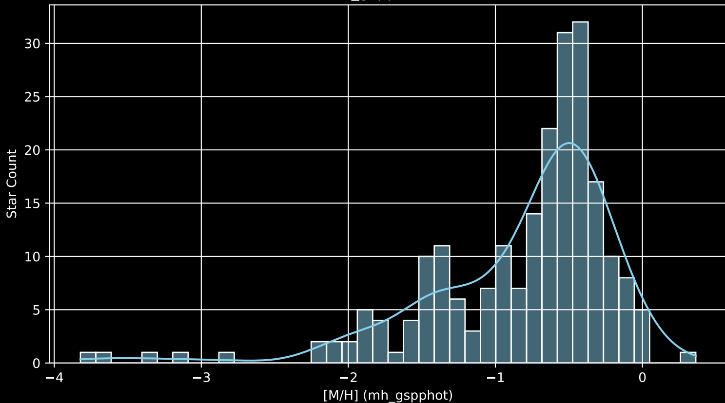
Gaia Cluster: [COIN-Gaia_24 [M/H] (mh_gspphot) (n= 220)
