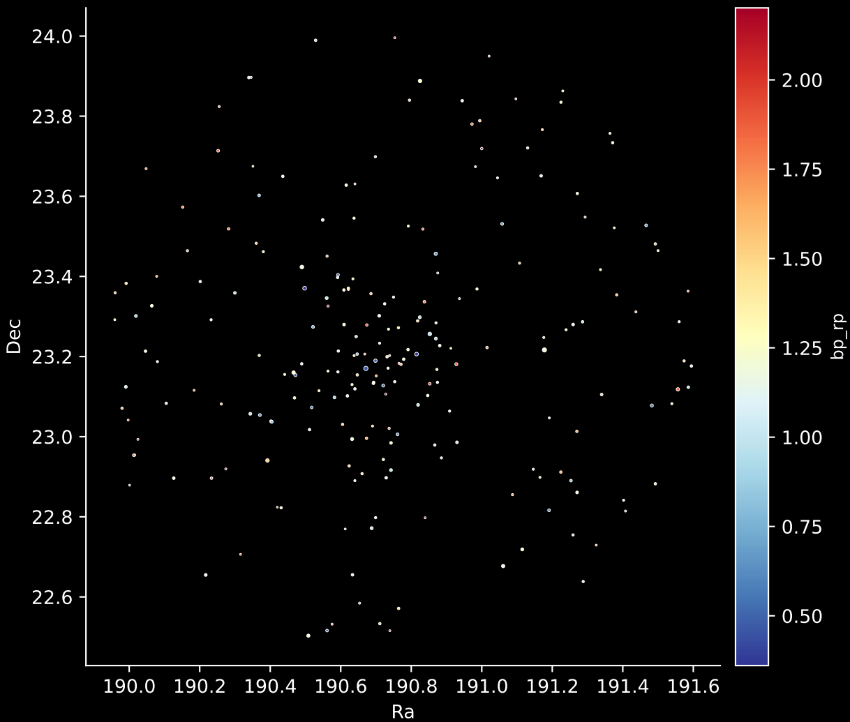
Gaia Cluster: [COIN-Gaia_24] Stars: 220
